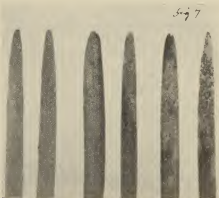
FIG. 7.—Relative effect of sulphur and copper dusts on the degree of infection caused by P. anomala . Leaves of Odessa barley inoculated with urediniospores and dusted immediately afterward. Left: dusted with sulphur. Centre: dusted with copper sulphate-lime dust. Right: control, not dusted.
