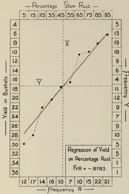
FIG. 22.—Regression of yield on percentage stem rust in plots of Marquis wheat from a 12 x 12 Latin Square experiment in 1930.
