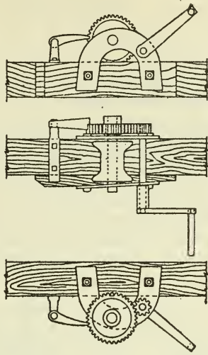
DETAIL OF WINCH AT "D" SCALE 1" = 4" inches
