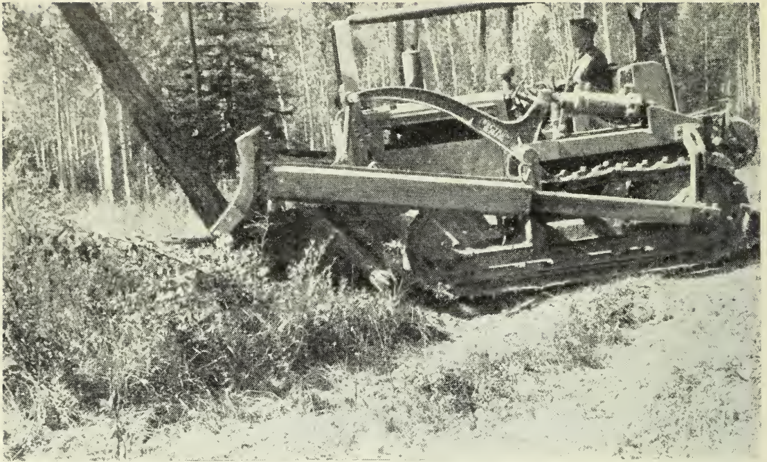
FIG. 7.—A bulldozer pushes a tree over.
