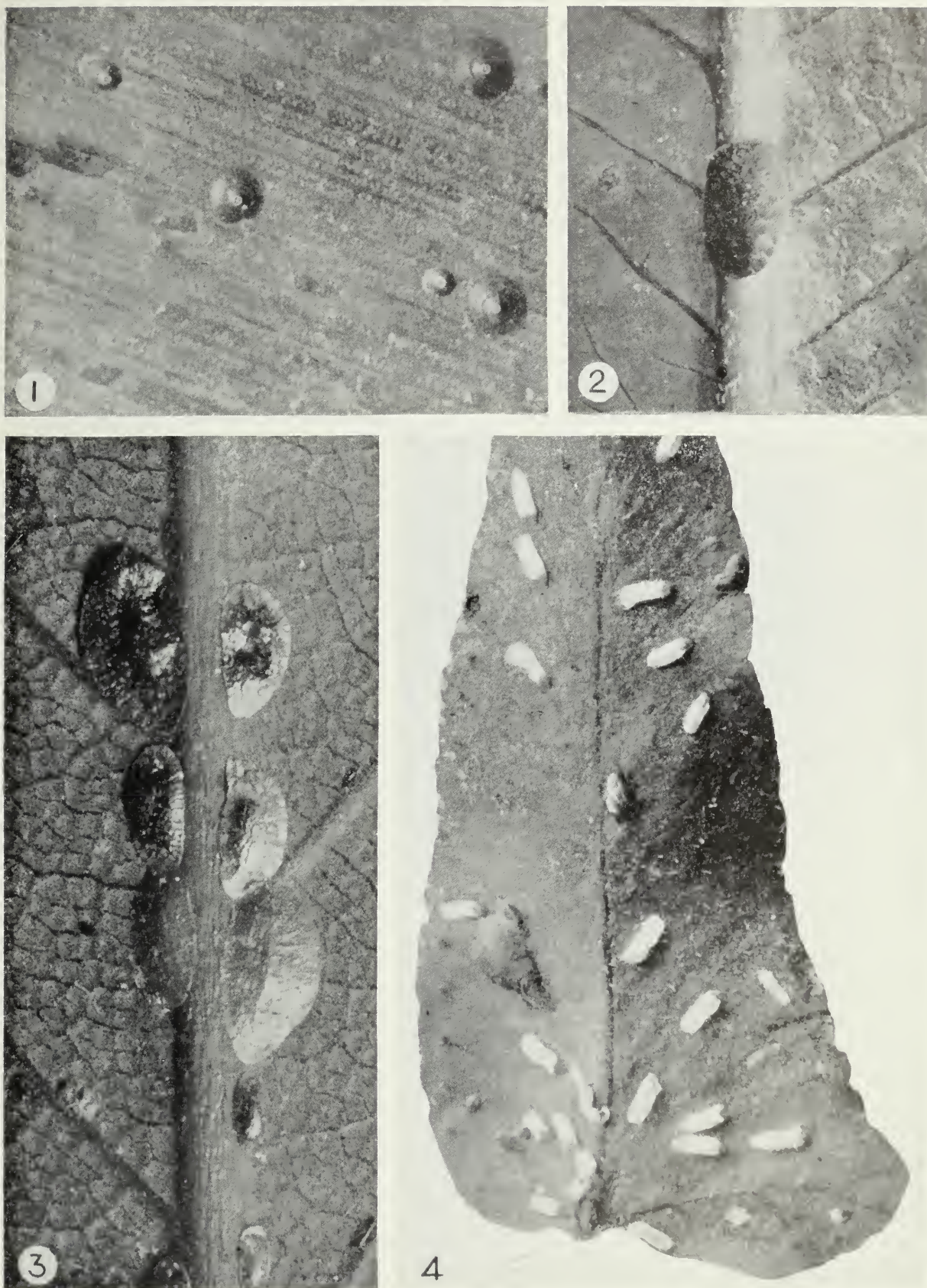
FIG. 1.—Florida red scale on palm leaf; 2, hemispherical scale on croton; 3, soft scale; 4, fern scale, males, females and young; all figures much enlarged (original).
