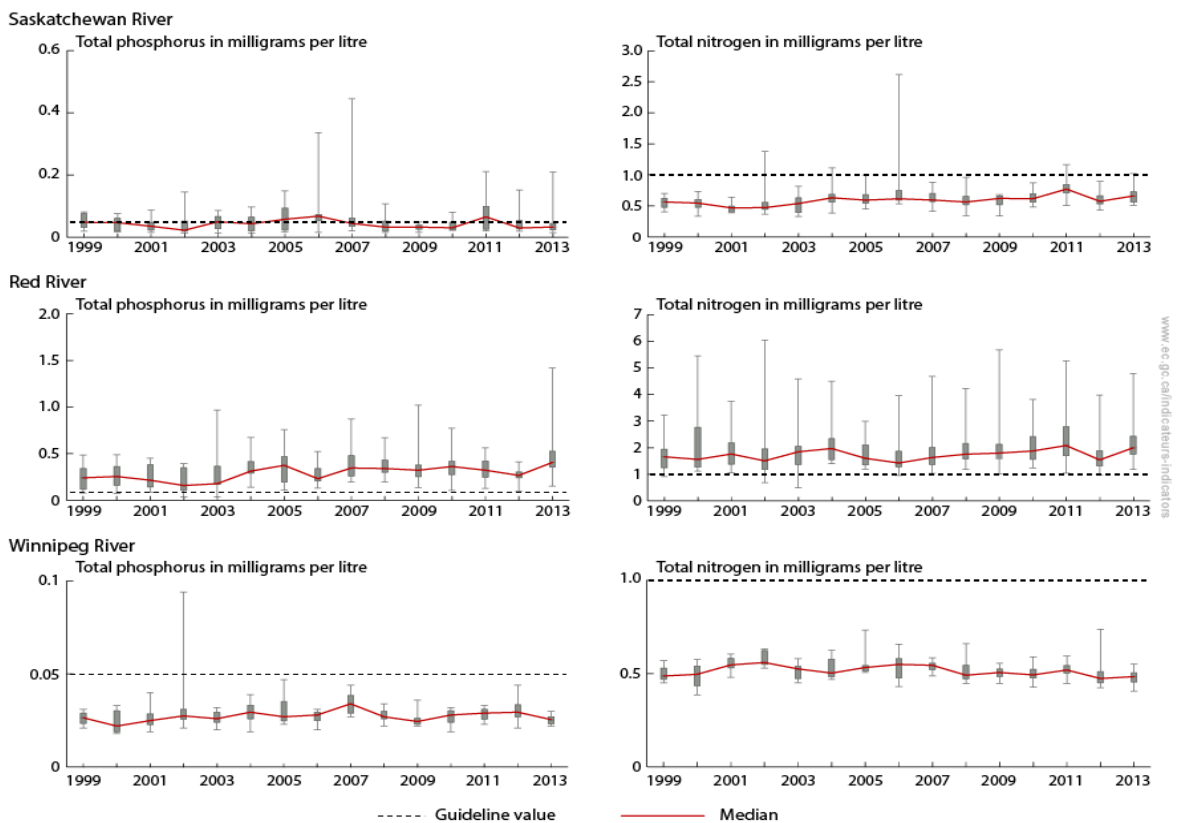
Figure 4. Annual total phosphorus and total nitrogen concentration box plots for the Red, Winnipeg and Saskatchewan rivers, Canada, 1999 to 2013
