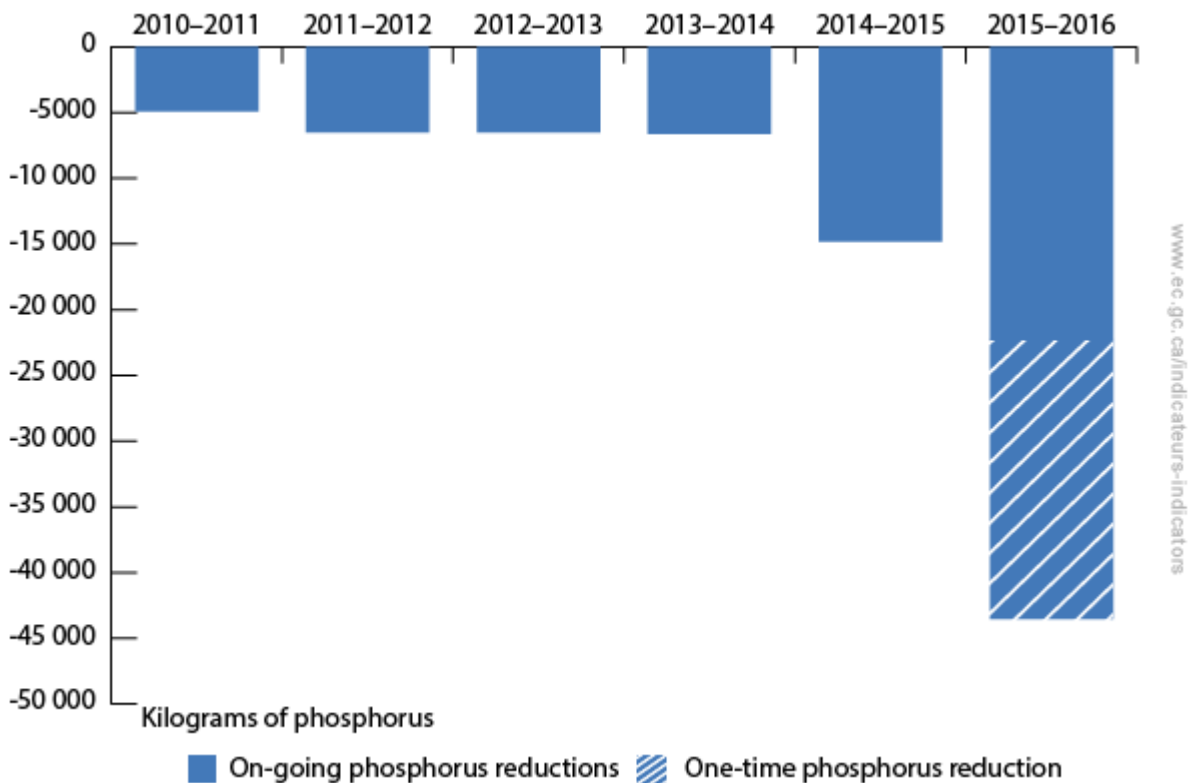
Figure 2. Cumulative, estimated reduction in the amount of phosphorus reaching Lake Winnipeg due to stewardship projects, April 2008 to March 2016
