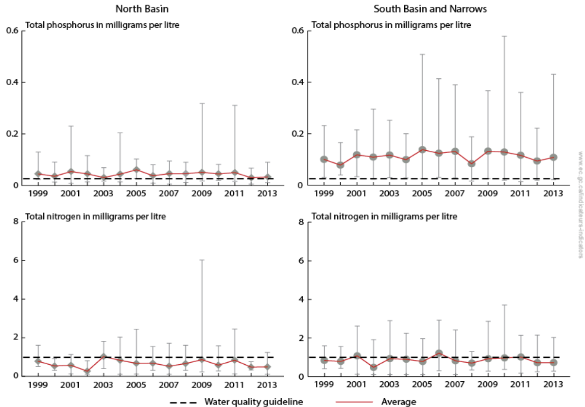
Figure 3. Annual seasonally weighted averages for total phosphorus and total nitrogen concentrations in Lake Winnipeg, Canada, 1999 to 2013
