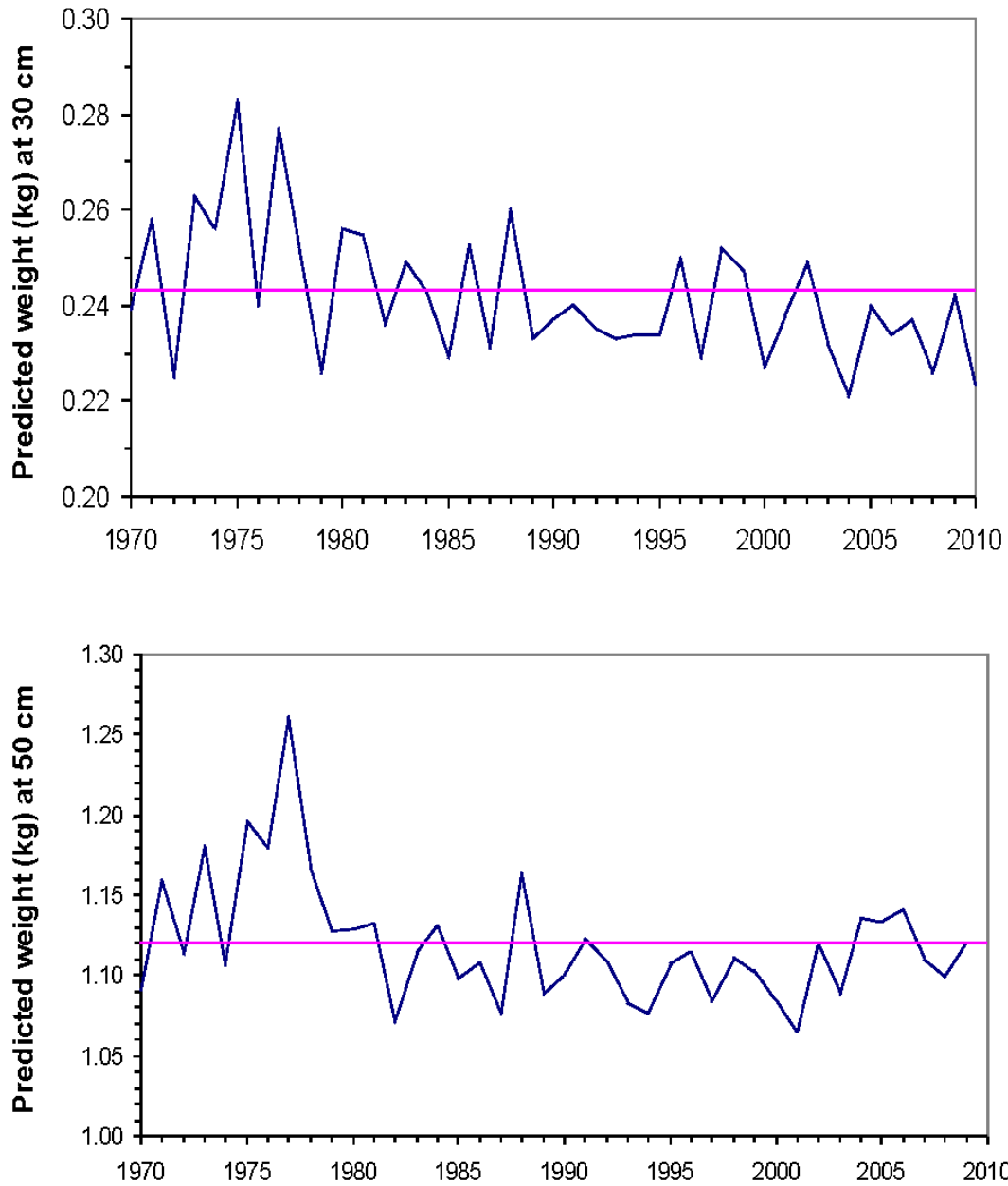
Figure 10. Condition (predicted weight at age) for 30 cm (top panel) and 50 cm (lower panel) NAFO Subdivision 4Vn (May-October) cod from the DFO summer RV survey. Horizontal line is the average from 1970-2009.
