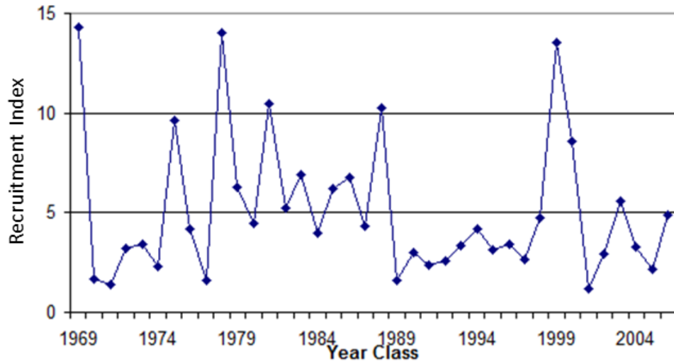
Figure 9a. Recruitment index of age 2-4 cohort numbers for NAFO Subdivision 4Vn cod (May-October) from the DFO summer RV survey.
