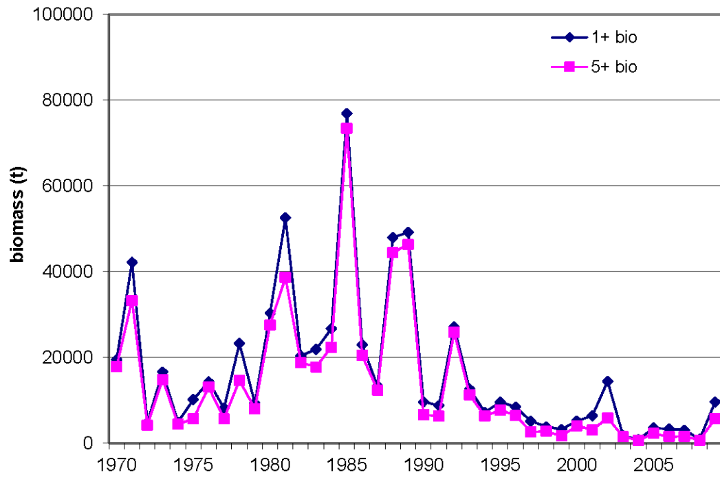
Figure 4. Numbers (upper panel) and biomass (lower panel) for 4Vn cod (May-October) for all ages (age 1+) and mature fish (age 5+) from the DFO summer RV survey.
