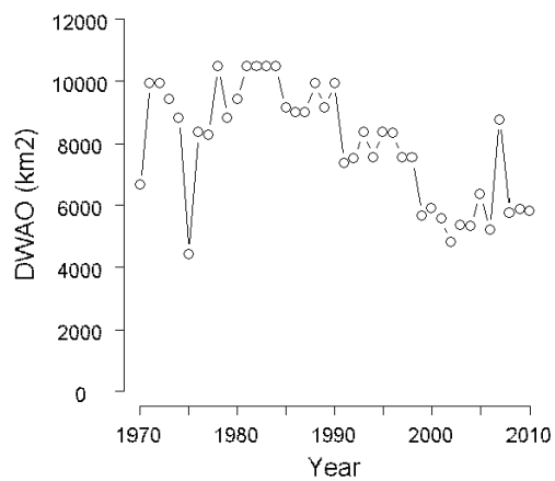
Figure 6. Design weighted area of occupancy ( \text{km}^2 ), or DWOA, for 4Vn (May-October) cod all sizes (upper panel), 1-38 cm (middle panel), and greater than 38 cm (lower panel) in NAFO Subdivision 4Vn from the DFO summer RV survey, 1970-2010.
