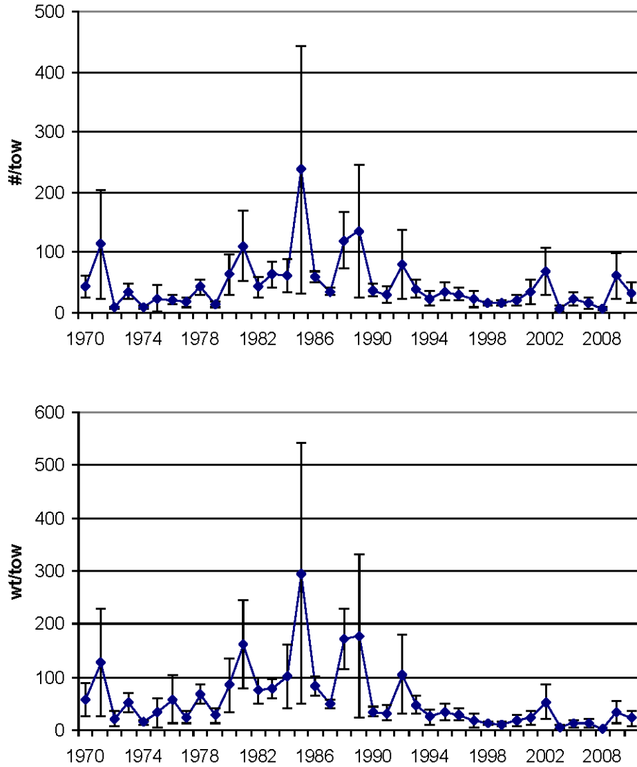
Figure 3. Numbers per tow (upper panel) and weight per tow (kg) (lower panel) for 4Vn cod (May-October) from the DFO summer RV survey.
