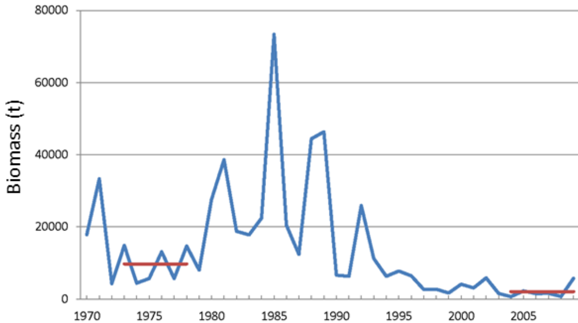
Figure 12. NAFO Subdivision 4Vn (May-October) estimated cod mature biomass (age 5+) from the DFO summer RV survey. The two horizontal lines represent the average of the time series for 1973-1978 and 2004-2009, respectively. The value reported in DFO (2011a, and 2011b) of 8,400 t for this similar calculation was for estimates not corrected for vessel effect in the 1973-1978 period. The conclusions of DFO (2011b) on status of the NAFO Subdivision 4Vn resident component and the potential for recovery are unchanged.
