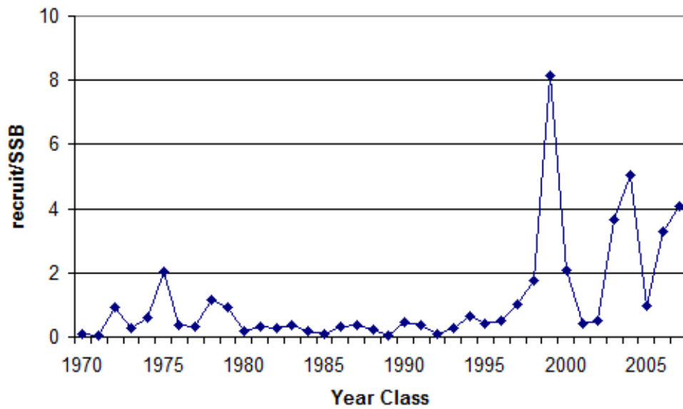
Figure 9b. Relationship between recruitment index (recruit) and spawning stock biomass (SSB) at age 5+ for NAFO Subdivision 4Vn cod (May-October) from the DFO summer RV survey.
