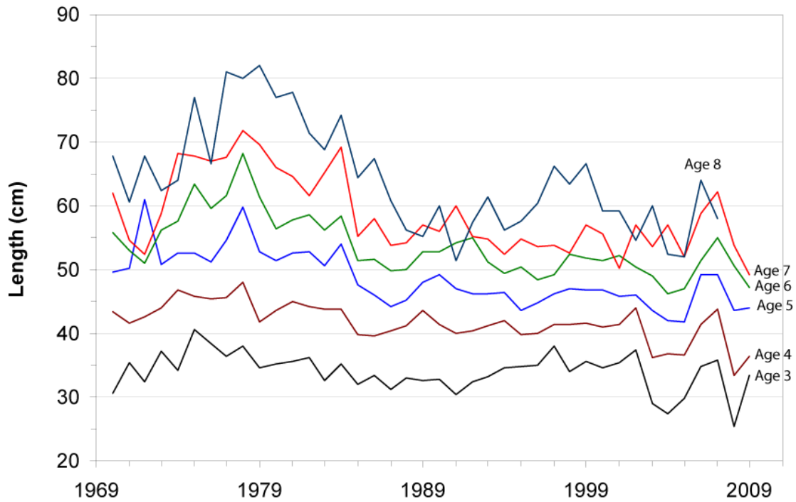
Figure 11. Length at age, for ages 3 to 8 years, for NAFO Subdivision 4Vn cod (May-October) from the DFO summer RV survey.
