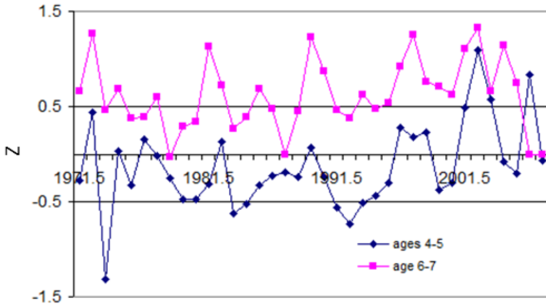
Figure 7. Estimates of total mortality ( Z ) by age class for NAFO Subdivision 4Vn (May-October) cod from the DFO summer RV survey.
