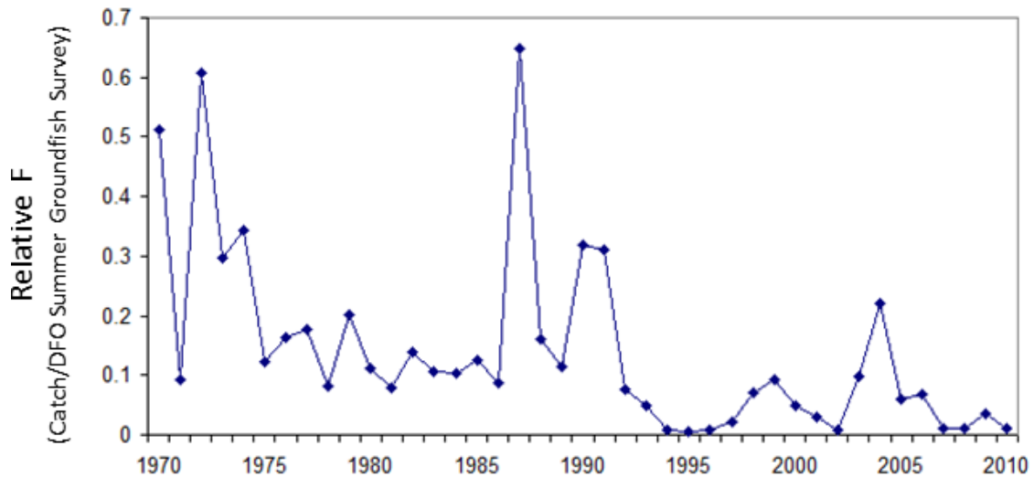
Figure 8. Relative fishing mortality ( F ) for NAFO Subdivision 4Vn cod (May-October) from the DFO summer RV survey.
