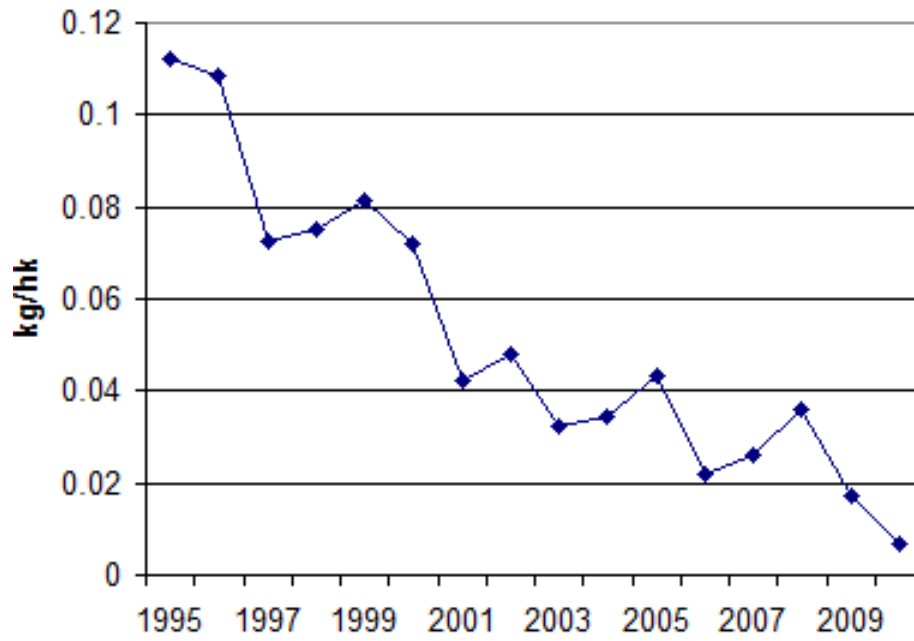
Figure 5. NAFO Subdivision 4Vn cod (May-October) abundance (kg/hook) from the September DFO-Industry fixed gear survey.
