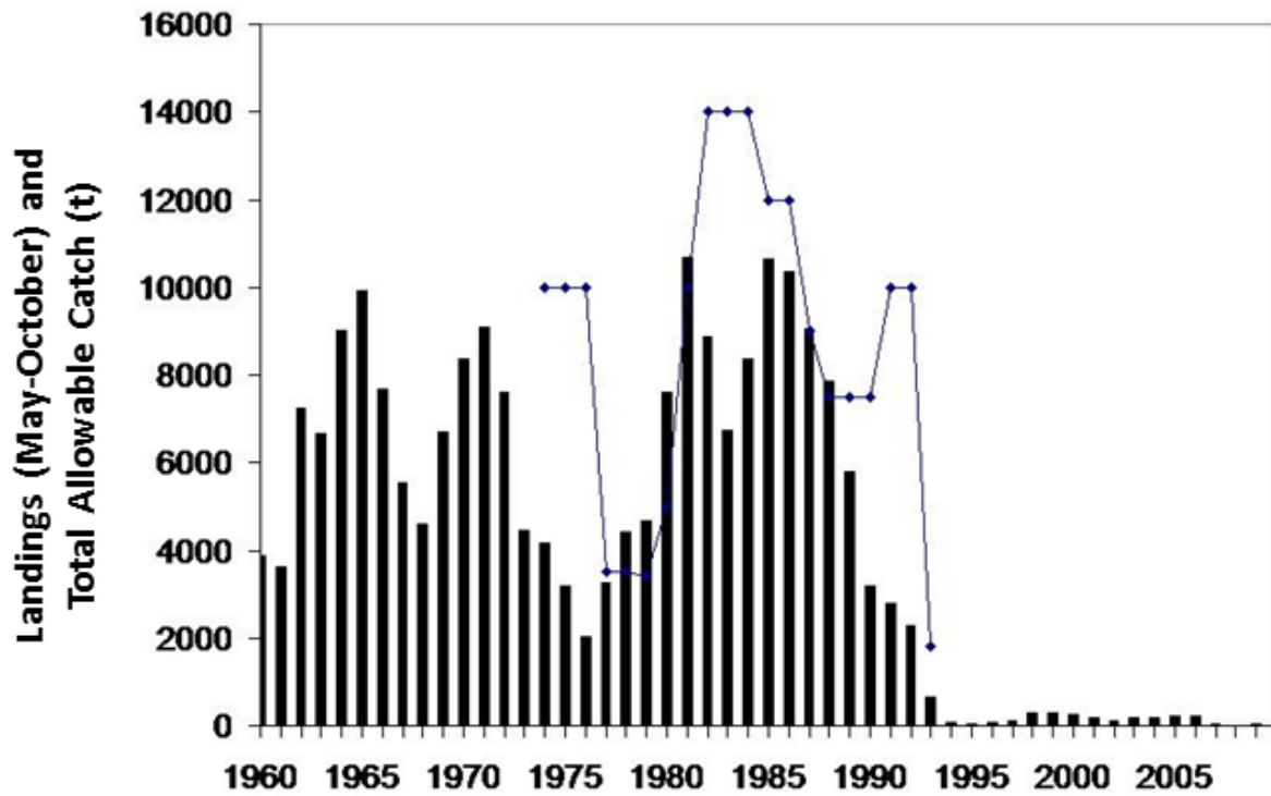
Figure 2. Landings (bars) and Total Allowable Catch (line) in tonnes for 4Vn cod (May-October) 1960 to 2010.
