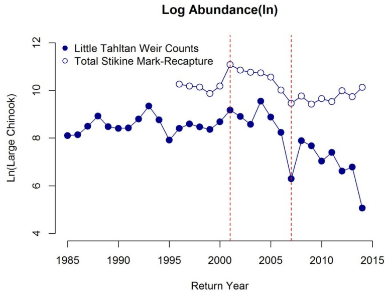
Figure 2. Relative spawner abundance time-series for Little Tahltan weir counts and total Stikine mark-recapture estimates by return year. Weir counts are available beginning in 1985 while mark-recapture estimates are available beginning in 1996. The leftmost vertical dashed line indicates the peak Stikine abundance year of 2001 that was followed by a period of declining abundance until 2007. The rightmost vertical dashed line indicates the return to increasing Stikine abundance beginning in 2007, but Little Tahltan weir counts continued to decline. Note that the obstruction created by the 2014 slide on the Tahltan River likely restricted fish passage to the Little Tahltan River. Note that the vertical axis is log-transformed.
