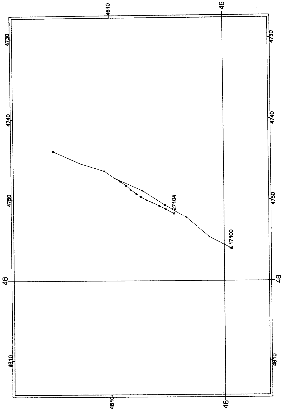
Figure II-3. Predicted trajectory at 1030 GMT, May 17, 1990
