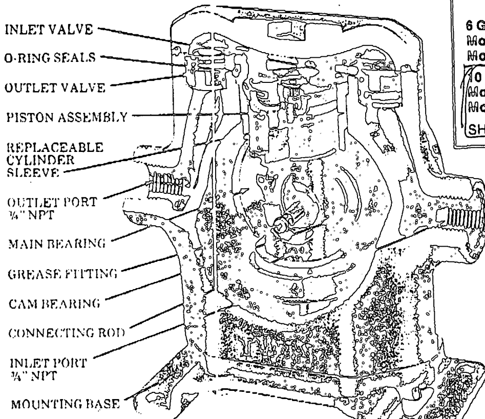
Cutaway view of Series 5200 pump is shown here without safety shield so piston parts and cam bearing can be seen. Do not operate pump without this shield in place.
