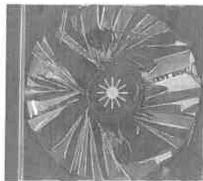
Figure 5. A recordable CD that was vacuum freeze-dried. The protective top layer and metal reflective layer have delaminated from the base of the disc.
