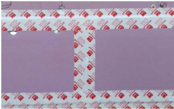
Figure 7: Close-up of the exterior air barrier system using extruded polystyrene rigid insulation with sealed joints used on a Winnipeg trial home, 2015. Photo credit: Gary Proskiw
