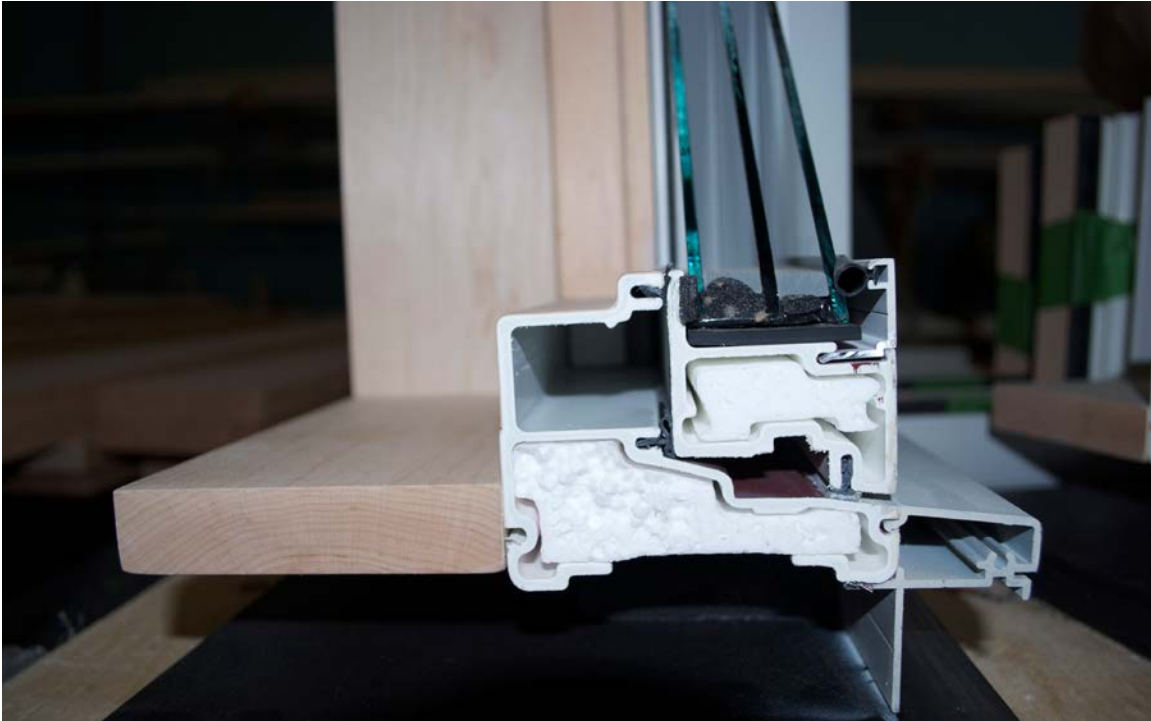
Figure 15: Image of a triple glazed high performance window. Photo: Natural Resources Canada
