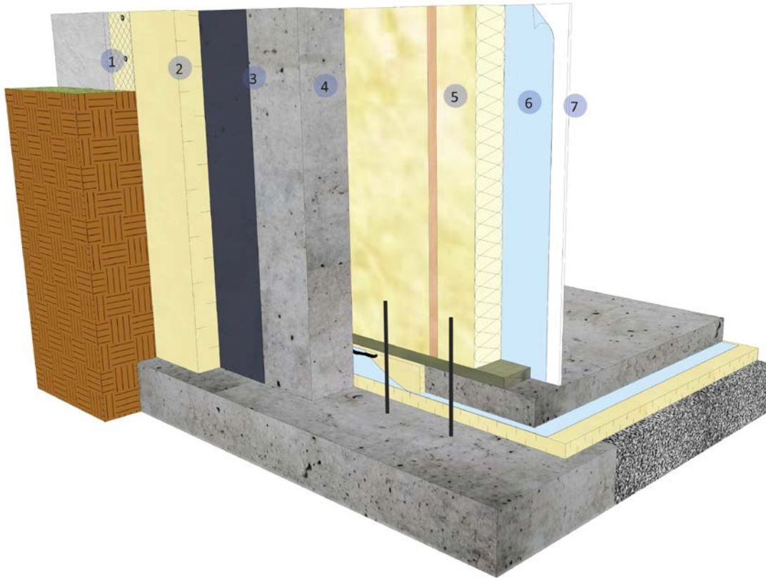
Figure 18: Approach 1 – Example of an exterior insulated foundation wall system. Contact the local manufacturer representative for specific application details. Illustration: Natural Resources Canada
