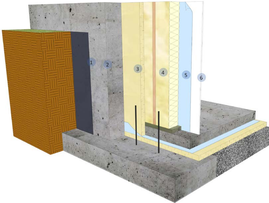
Figure 19: Approach 2 – Example of an interior insulated foundation wall employing rigid insulation materials. Contact the local manufacturer representative for specific application details. Illustration: Natural Resources Canada
