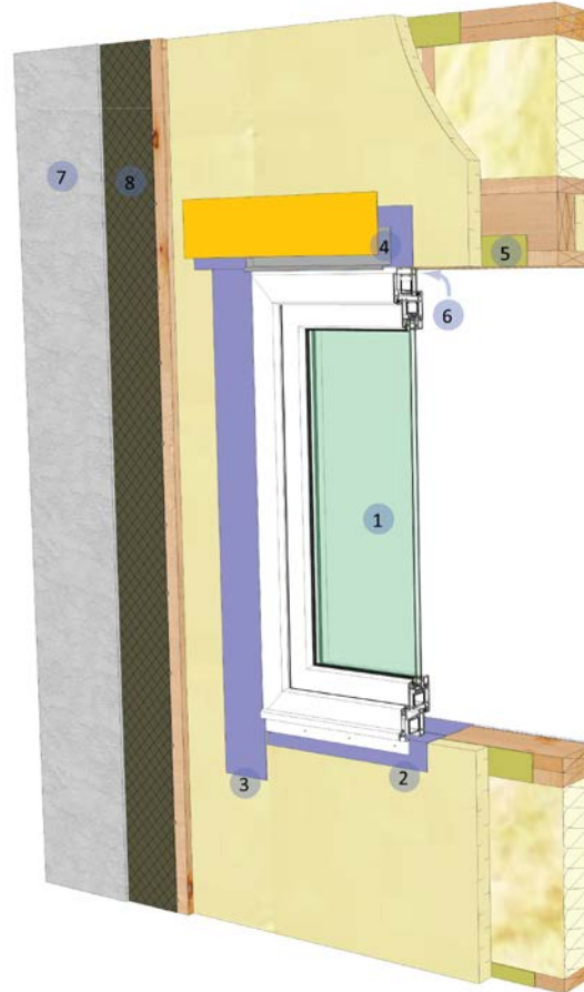
Figure13: Builders installed flange windows and fastened through insulation into framing. Illustration: Natural Resources Canada
