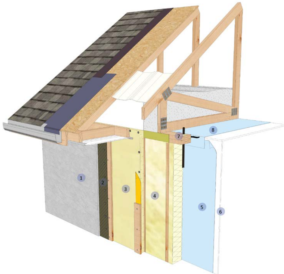
Figure 11: Simplified view of an above grade wall to roof transition as trialed by the Manitoba LEEP builder group with an exterior insulated and air sealed wall/roof system. Illustration: Natural Resources Canada
