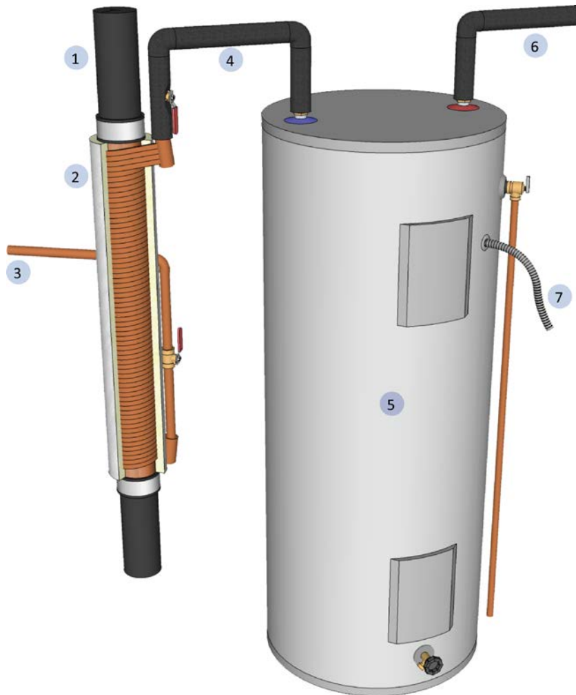
Figure 22: Illustration of a Drain Water Heat Recovery System (DWHR) Illustration: Natural Resources Canada
