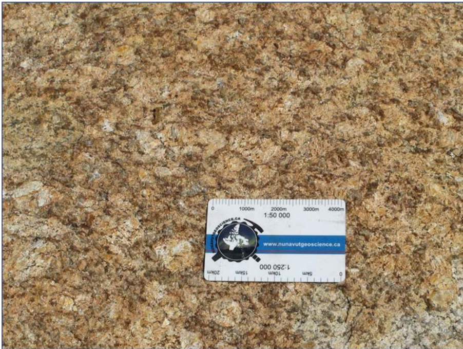
Figure 8. Biotite-orthopyroxene monzogranite with relict K-feldspar porphyroclasts (unit Pmg) on western Hall Peninsula, Baffin Island, Nunavut. Photograph by B.J. Dyck. 2015-032
