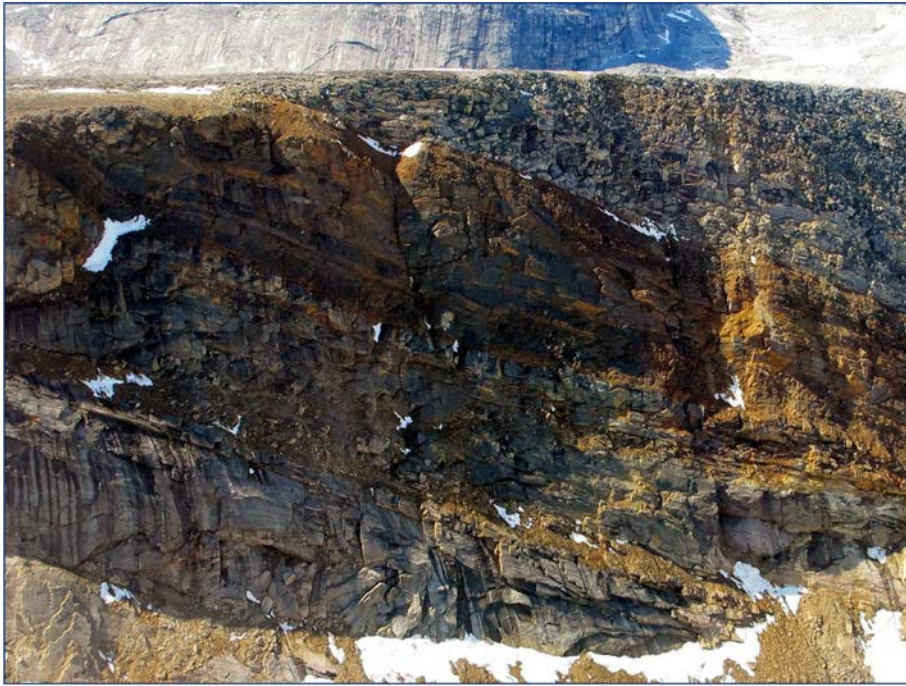
Figure 5. Archean biotite-hornblende tonalite orthogneiss (unit \bar{A}t ; top right) thrust over Paleoproterozoic metasedimentary rocks (unit PLHs; centre) that disconformably overlie another Archean tonalite orthogneiss layer. These thick-skinned T_2 thrust imbricates are east-verging, suggesting a dominant compressional force from the west during the Trans-Hudson Orogen on Hall Peninsula, Baffin Island, Nunavut. Looking southwest; the cliff section is approximately 175 m tall. Photograph by H.M. Steenkamp. 2015-042
