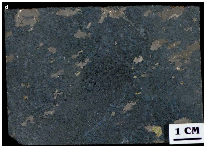
Figure SR4.3d. Stobie mine. Typical ore with 15% blebby pyrrhotite-pentlandite-chalcopyrite in medium-grained gabbro. Sample S14, Inco collection.
