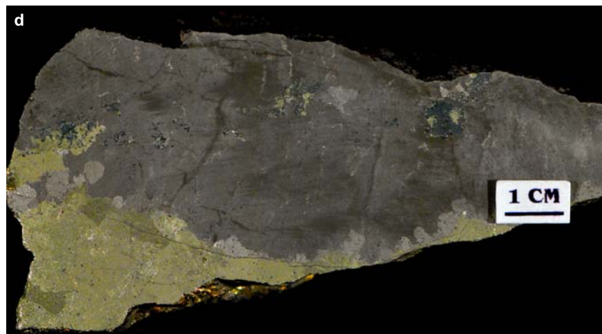
Figure SR1.8d. Little Stobie mine. Massive pyrrhotite with minor pentlandite cross-cut by a coarse chalcopyrite vein. Sample 01-AV-217, 1600, collected by Watkinson.
