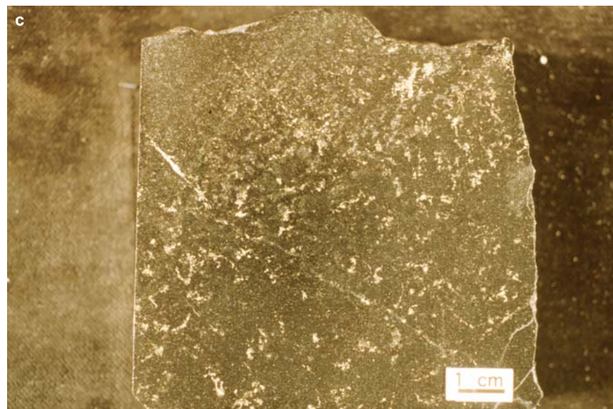
Figure SR4.3c. Stobie mine. Typical ore with 8% blebby pyrrhotite-chalcopyrite in fine-grained gabbro. Sample S11, Inco collection.
