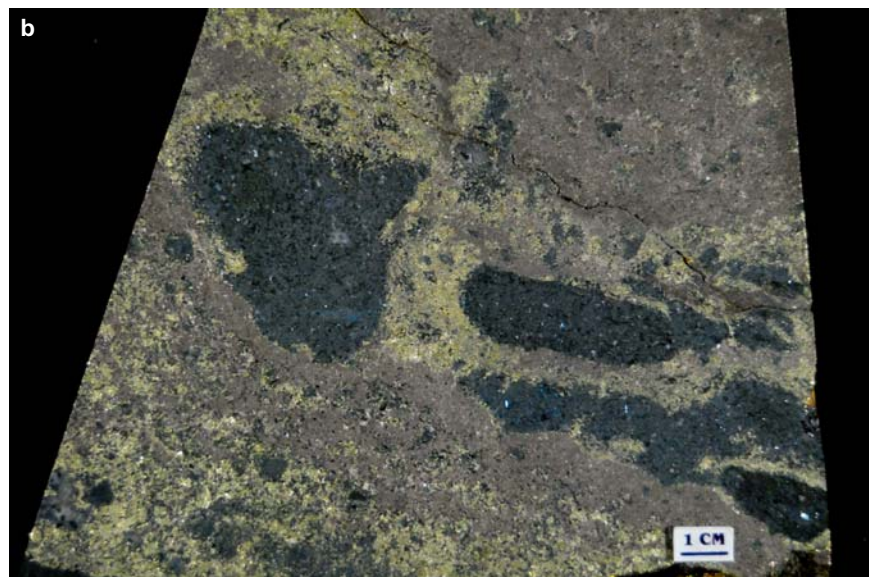
Figure SR1.8b. Little Stobie mine. Semi-massive sulphide coarse pyrrhotite-chalcopyrite in mafic Levack Gneiss Complex. Sample 01-AV-212, collected by Watkinson.
