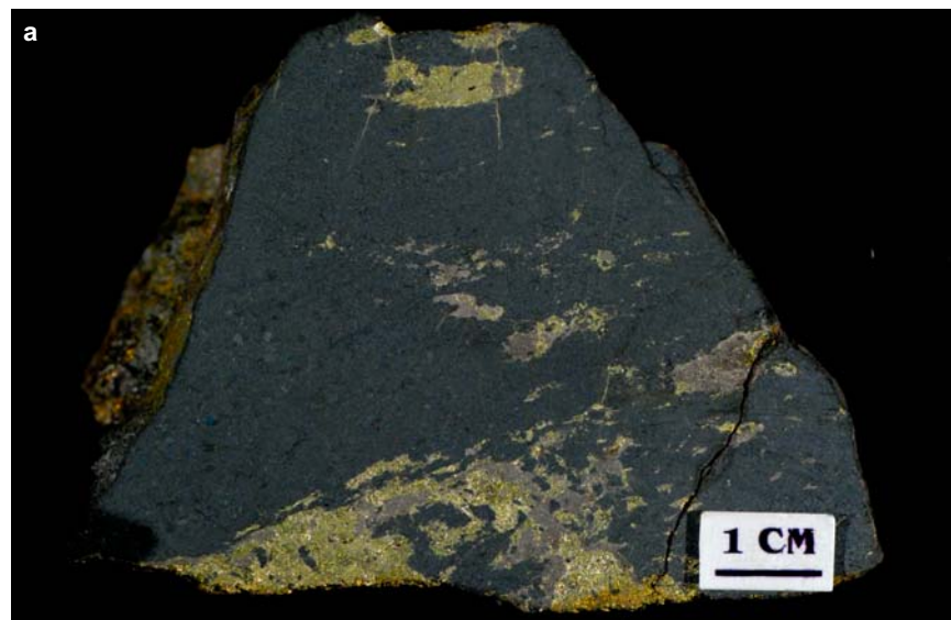
Figure SR1.9a. Mt Nickel deposit. Blebby to stringer and disseminated chalcopyrite-pyrrhotite in fine-grained mafic rock. Sample 02-AV-842.
