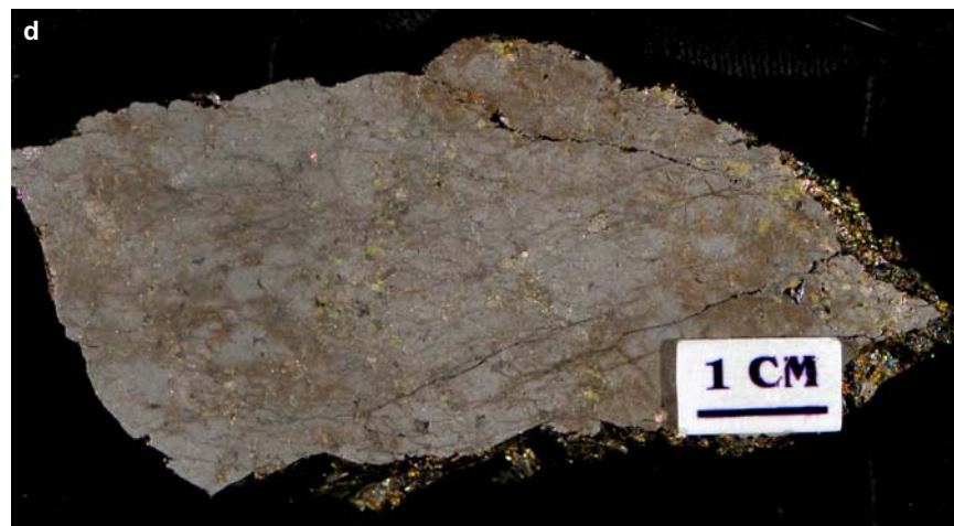
Figure SR1.3d. Crean Hill deposit. Massive pyrrhotite with minor blebby pentlandite and disseminated chalcopyrite stringers. Sample 98-AV-48, 3980 level 3980A.
