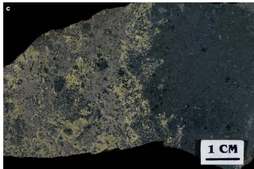
Figure SR1.8c. Little Stobie mine. Interstitial to semi-massive pyrrhotite-chalcopyrite-bornite in Levack Gneiss Complex. Sample 01-AV-214, collected by Watkinson.
