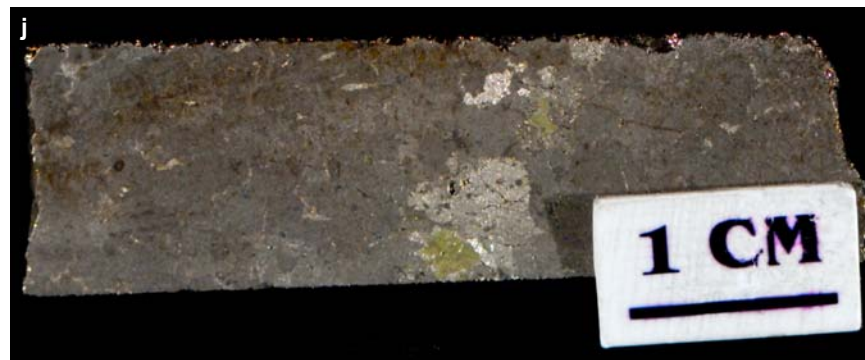
Figure SR3.1j. Copper Cliff deposit. Massive pyrrhotite-pentlandite-chalcopyrite. Sample 98-AV-58, bore hole 100505, 240-240.5 ft, 100 orebody.
