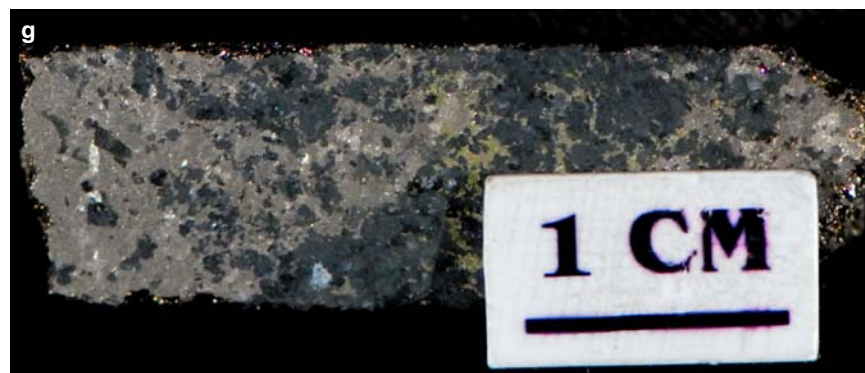
Figure SR3.1g. Copper Cliff deposit. Semi-massive pyrrhotite-chalcopyrite. Sample 98-AV-55, bore hole 100506, 248-248.5 ft, 100 orebody.
