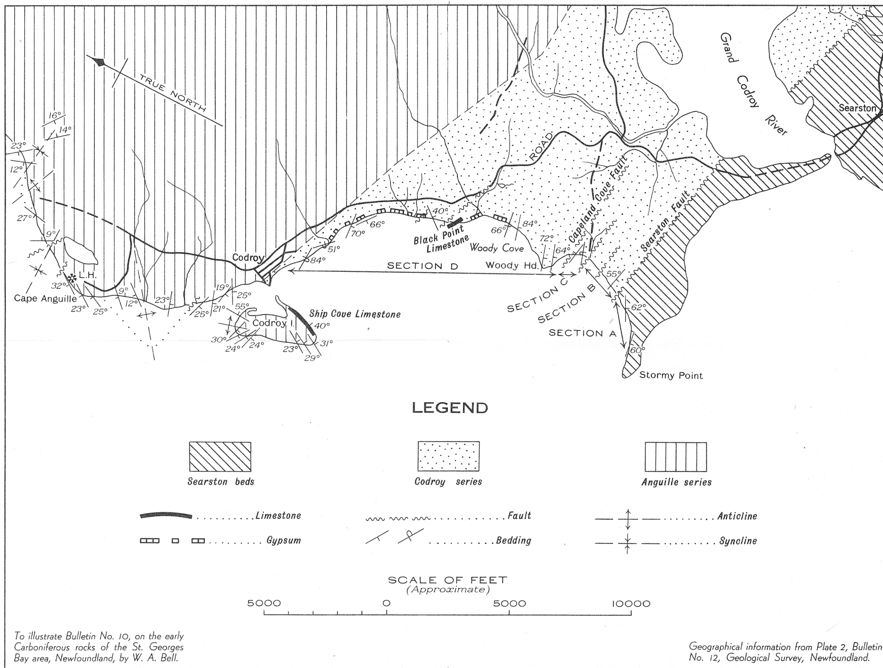
FIGURE 2. GEOLOGY OF THE CODROY AREA, NEWFOUNDLAND
