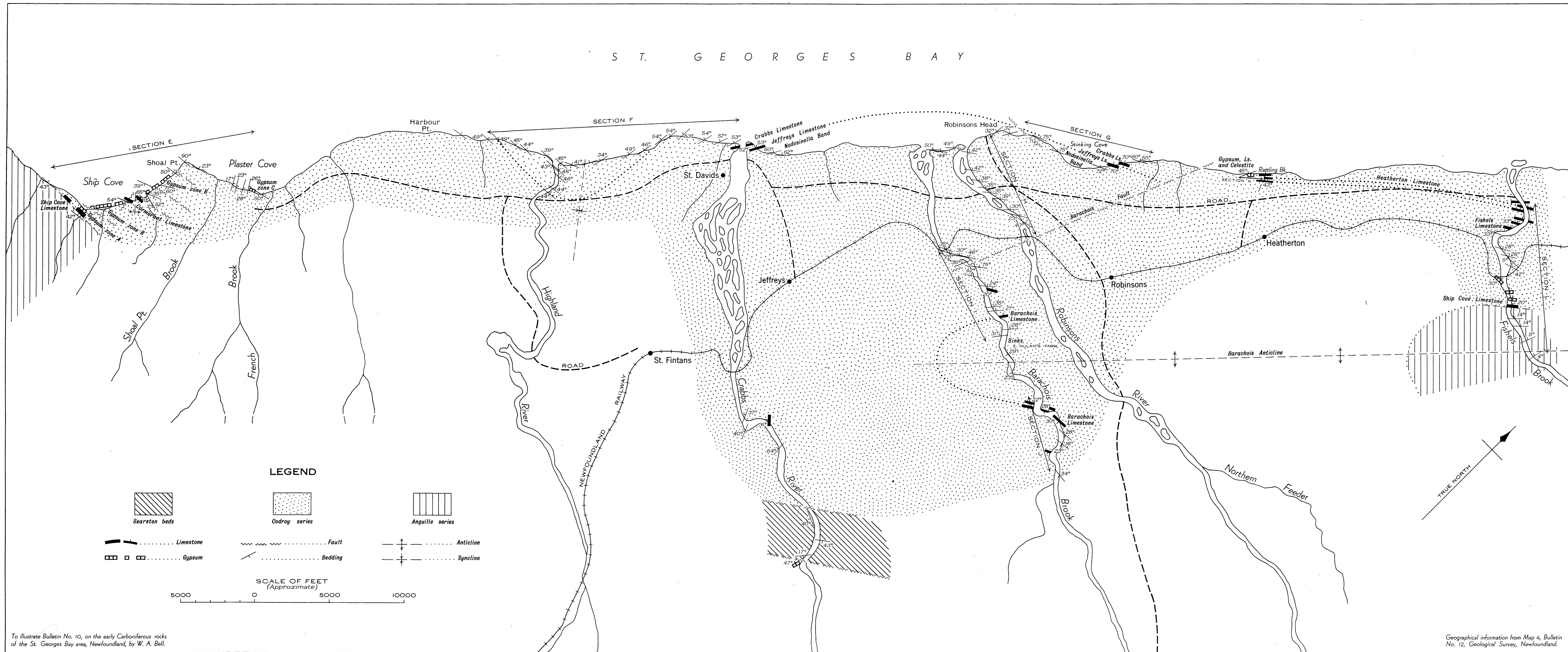
FIGURE No. 3 GEOLOGY OF PART OF THE SOUTHEAST COAST OF ST. GEORGES BAY, NEWFOUNDLAND
