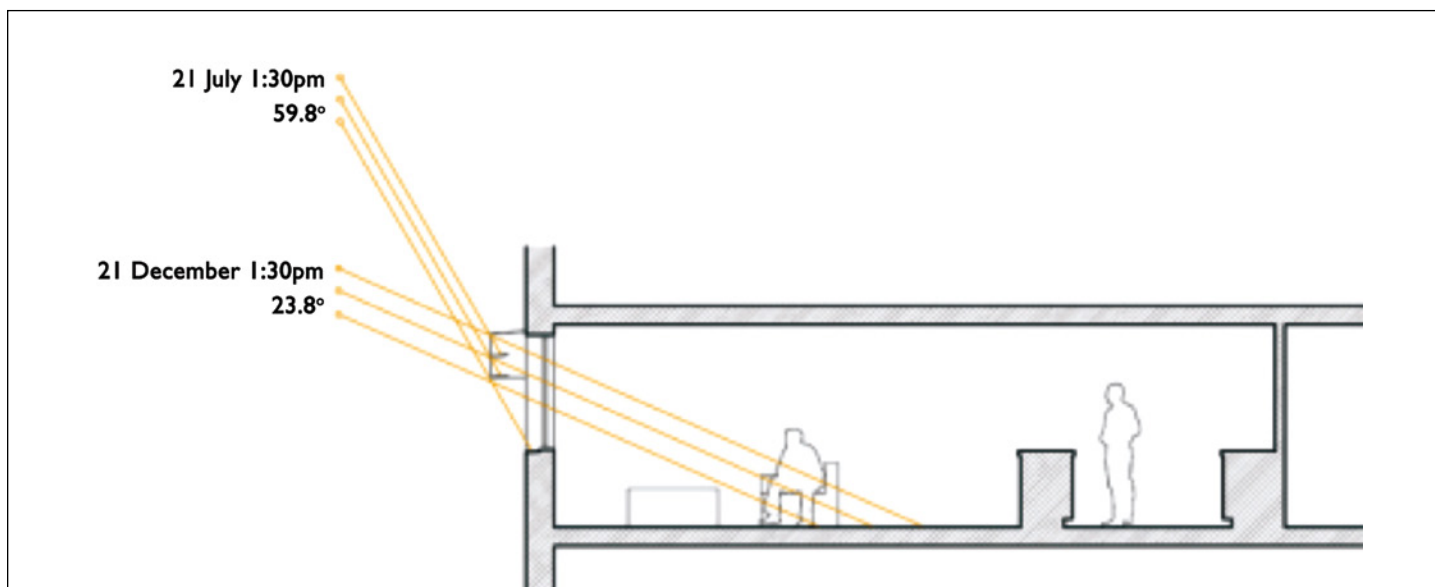
Figure 2 Solar penetration on July 21 and December 21 on the southwest facade
