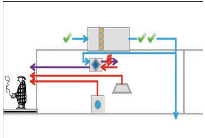
Figure 3 The proposed ventilation concept for Bois Ellen: the outside air intake is located at the roof, away from common smoking areas. Air is preconditioned by a large commercial system before being supplied to the individual unit HRVs. The roof-mounted system boasts high-efficiency filtration that improves outside air quality by removing fine particulates. (Clipart smoker: free.clipartof.com. Image concept: Frédéric Genest, Pageau Morel)
