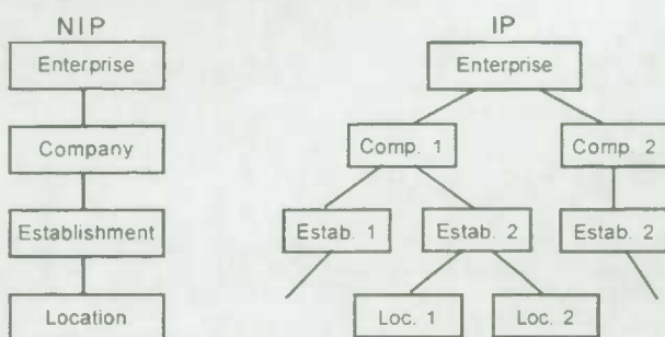
Diagram 2: Statistical Structures
