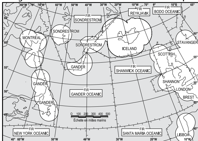
Figure 6.1 – Couverture VHF – NAT – 10 000 pi
