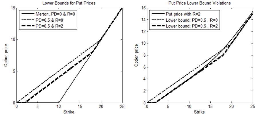
< Figure 2. Lower Bound for Put Prices >
