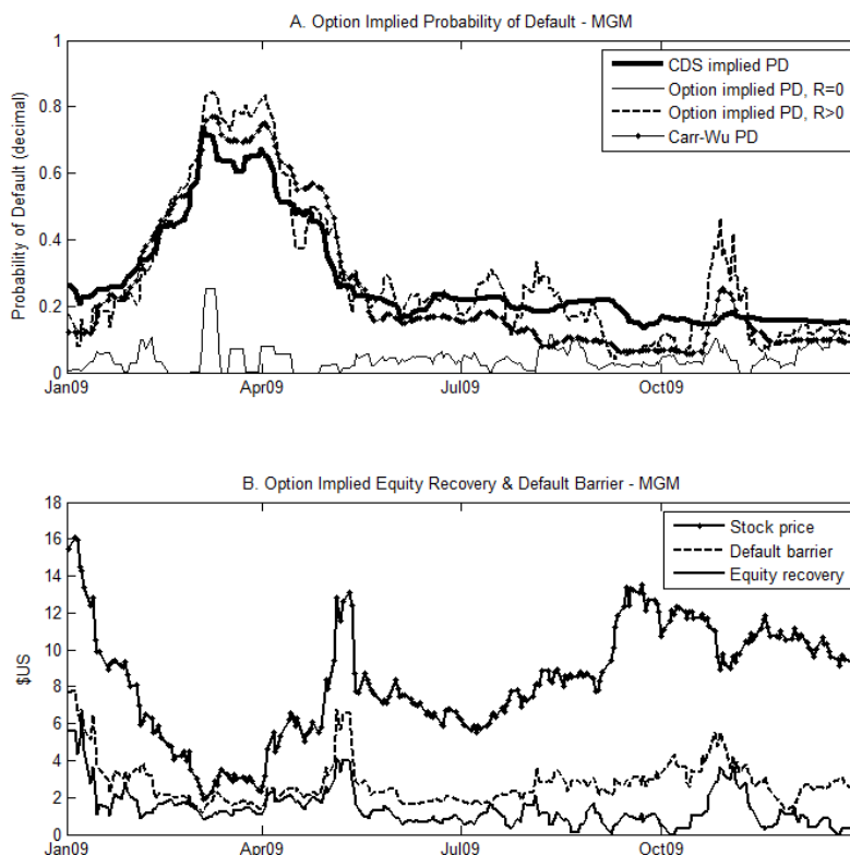
< Figure 4. Probability of Default, Equity Recovery, and Default Barrier: MGM >
