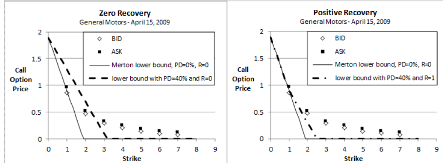
< Figure 3. Lower-Bound Violations: General Motors >
