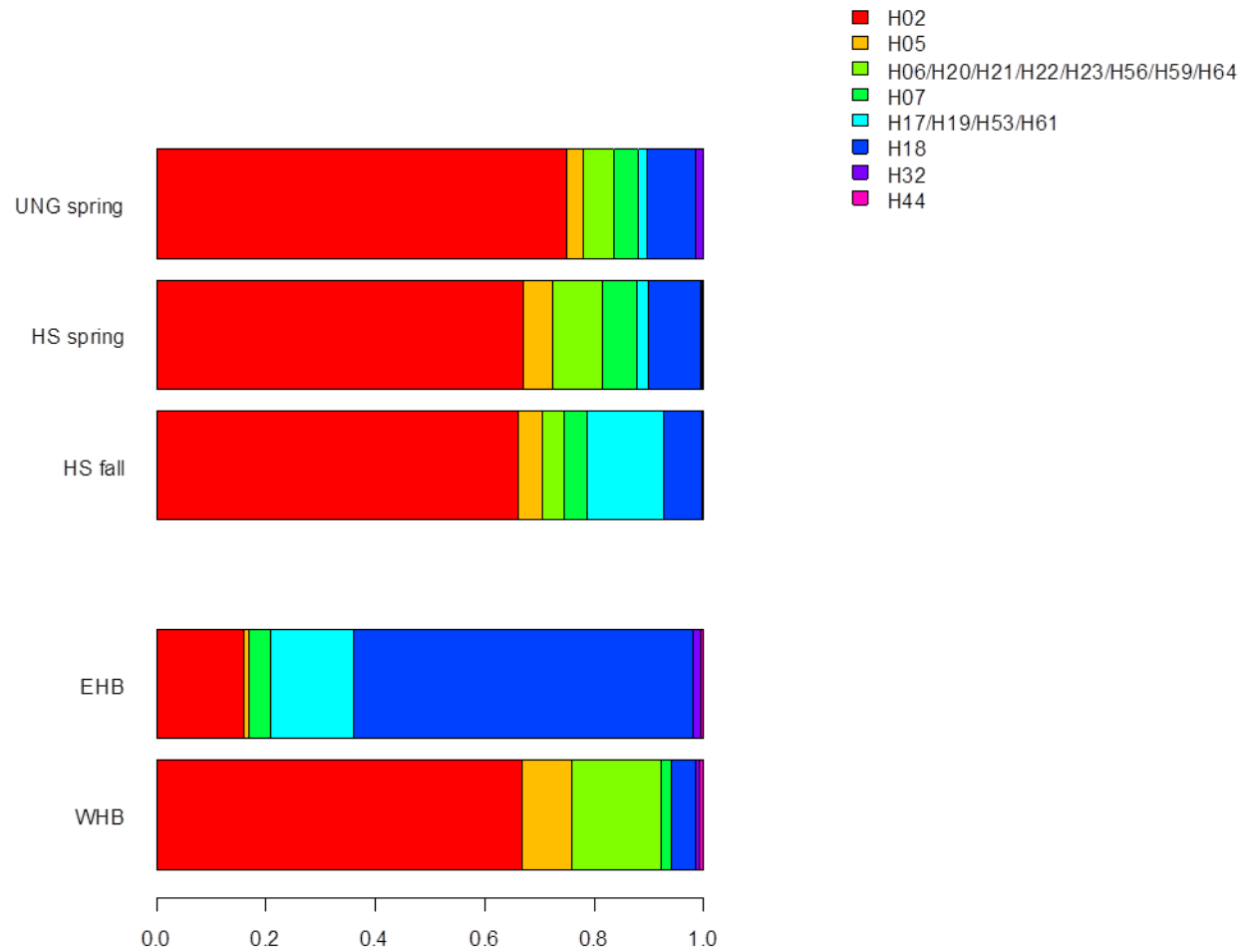
Figure 2. Frequency plot of haplotypes in source areas (bottom, EHB and WHB), and in mixed hunt areas (top). UNG spring, HS spring and HS fall are stated for Ungava spring harvest and Hudson Strait spring and fall harvests respectively. Colour legend shows haplotypes or groups of haplotypes.
