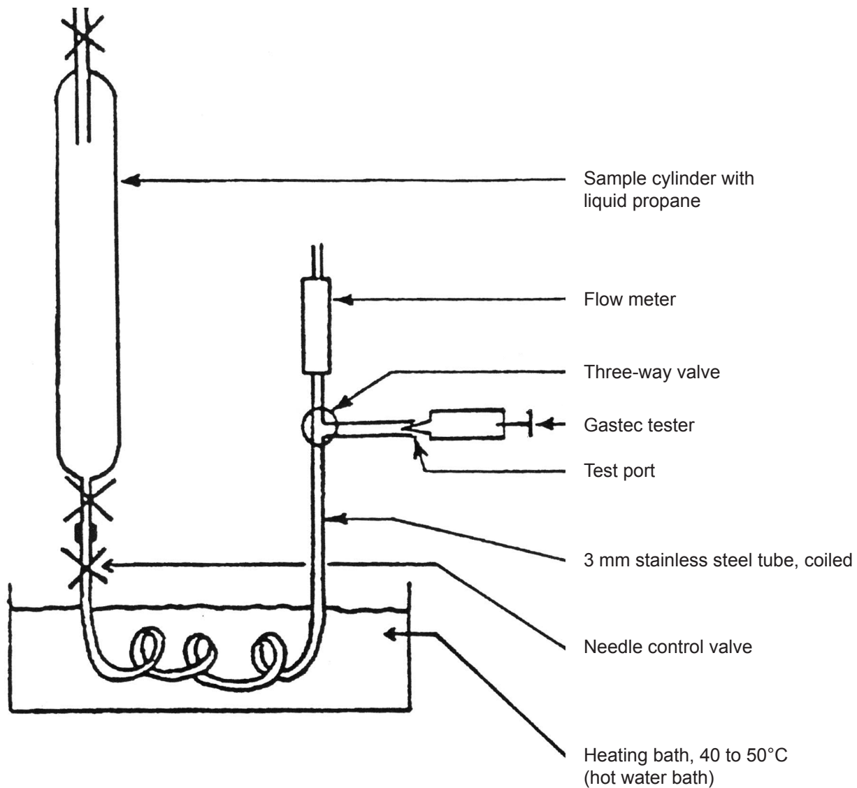
Figure 1 — Apparatus for procedure A — Flowing propane gas stream analysis
