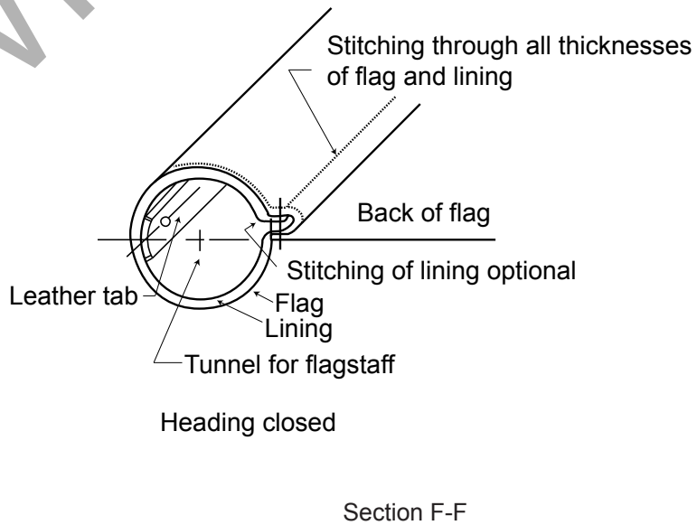
Figure 10 — Construction details for flag type — Subtype 3A flag
