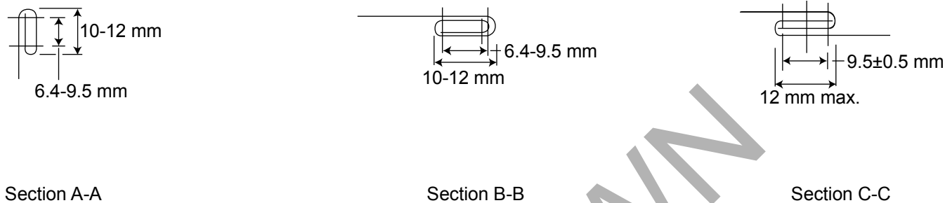
Figure 5 — Construction details
