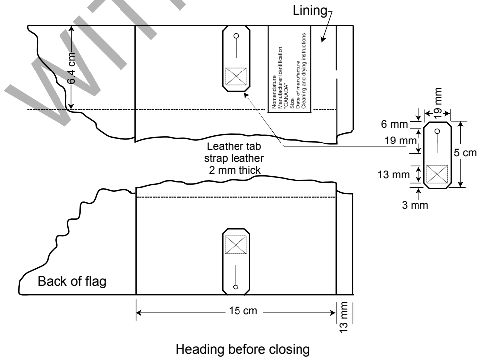
Figure 8 — Type 3 — Header, open-sleeve with leather tabs
