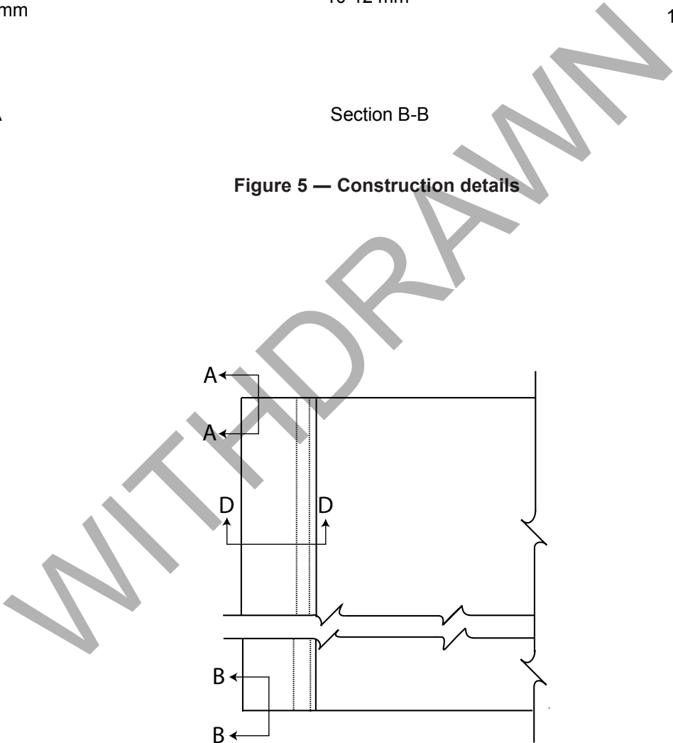
Figure 6 — Type 1 — Header, open-sleeve
