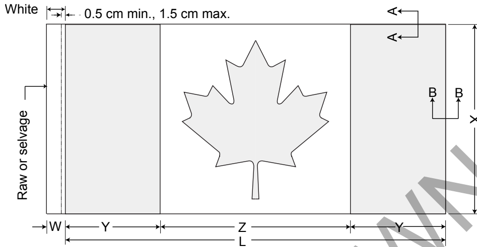
Figure 2 — One-piece flag construction
