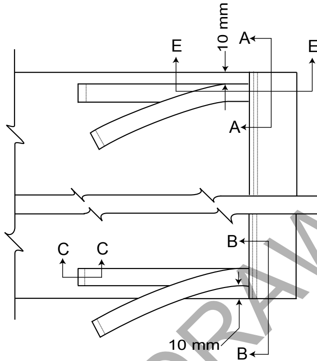
Figure 7 — Type 2 — Header, open-sleeve with tie tapes
