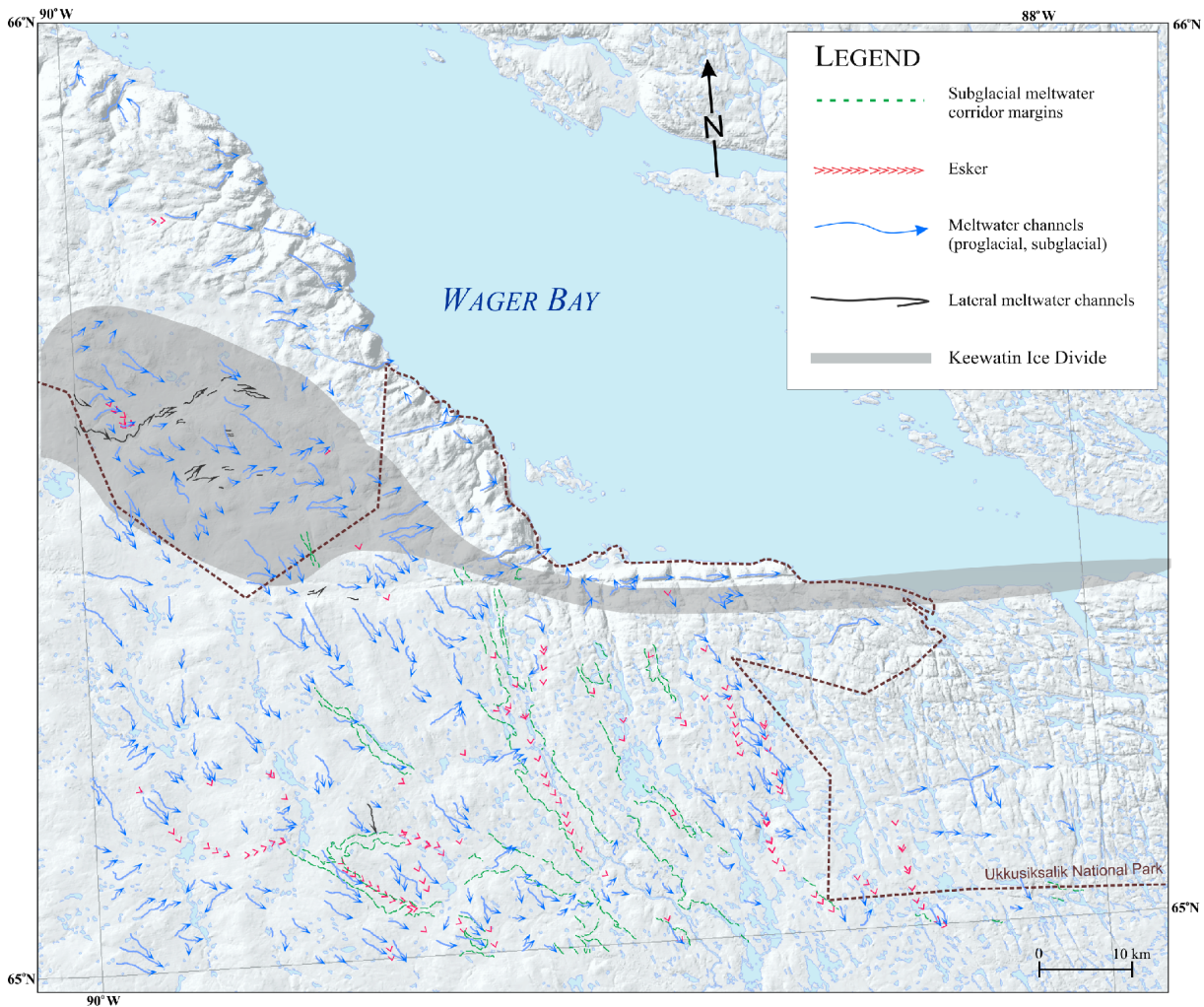
Figure 2. Ice-retreat features including subglacial meltwater corridors, eskers, proglacial/subglacial meltwater channels, and lateral meltwater channels. Location of Keewatin Ice Divide is approximate.
