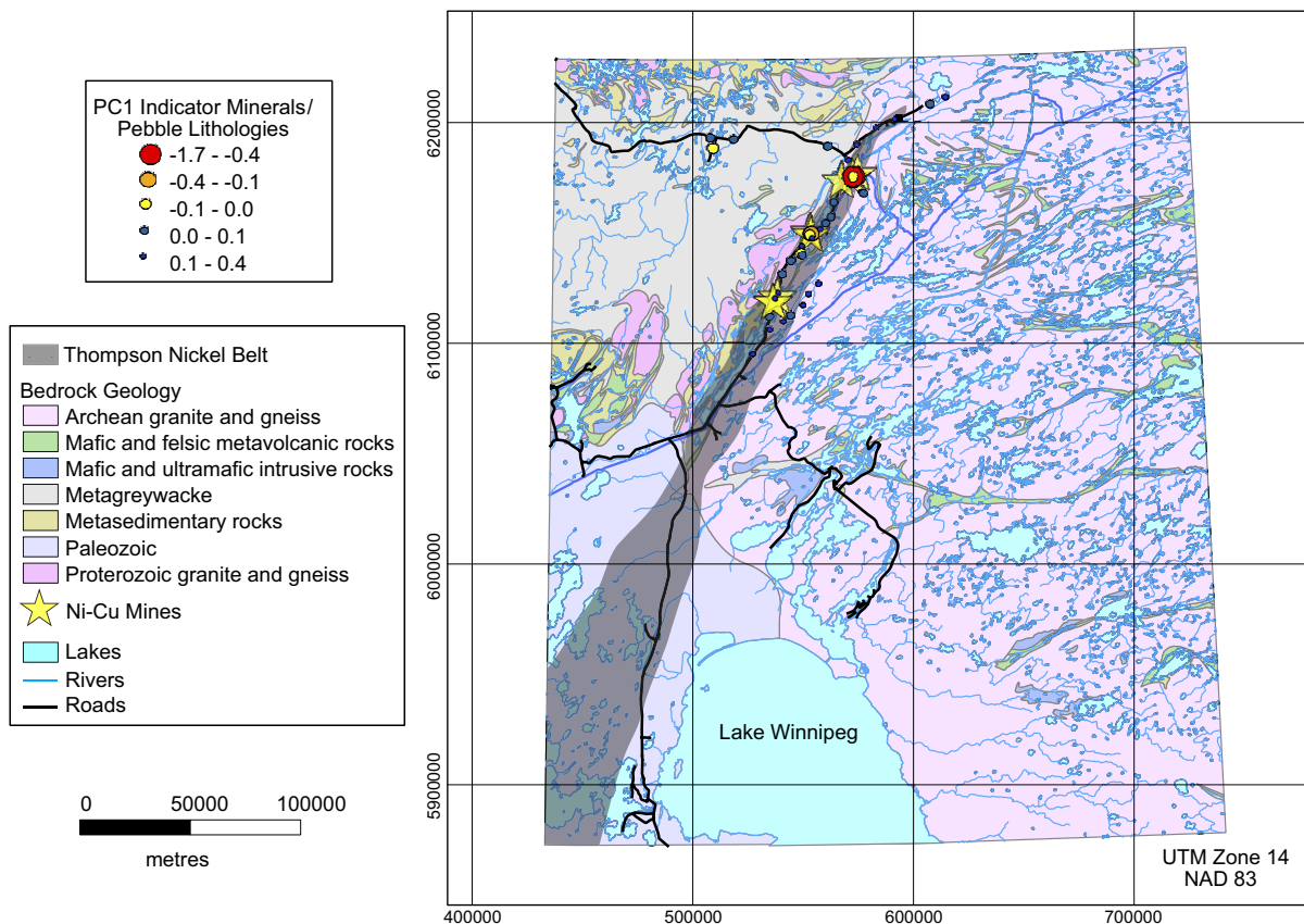
Figure 7. Map showing the distribution of the first principal component scores derived from the combined indicator mineral and pebble-lithology data.
