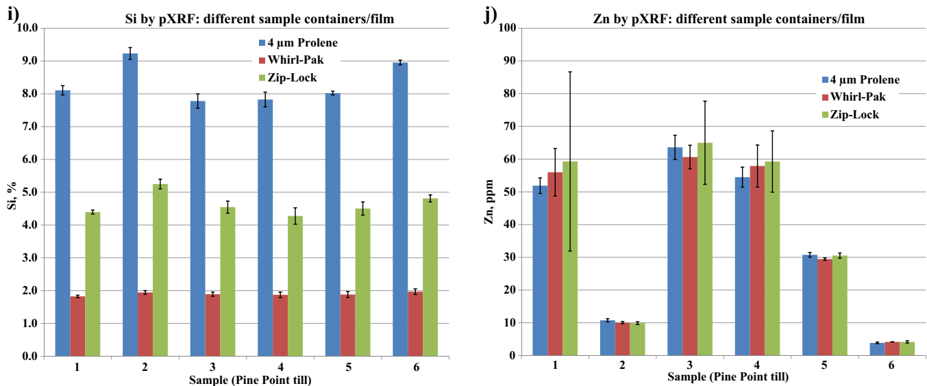
Figure 2 continued. i) Silicon by pXRF using different sample containers/film. ii) Zinc by pXRF using different sample containers/film.
