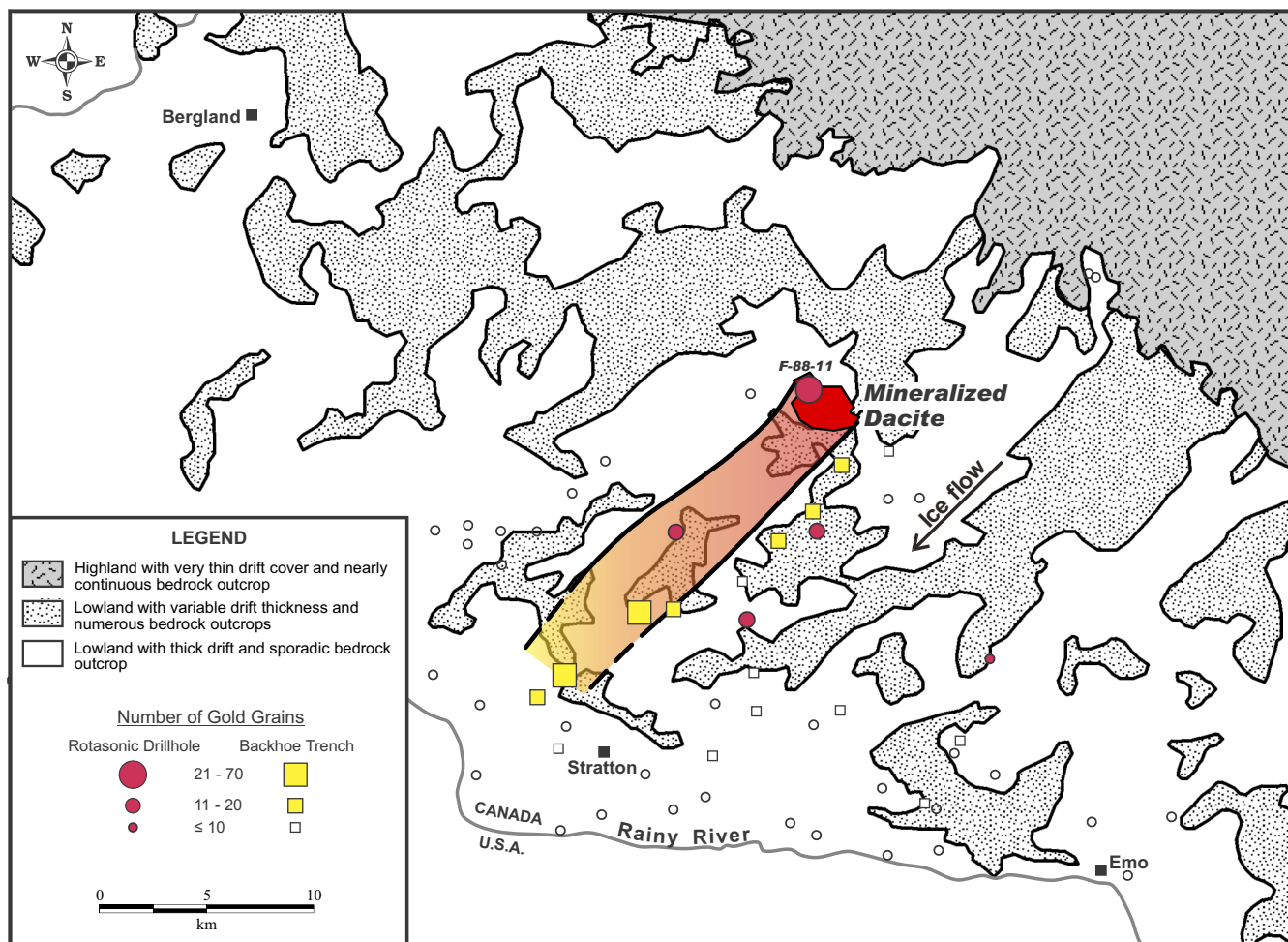
Figure 5. Approximate limits of the gold-grain dispersal train from the broadly mineralized dacite hosting the Rainy River gold deposit. Most till samples collected within the train contained >10 gold grains per 7.5 kg of -2 mm matrix.
