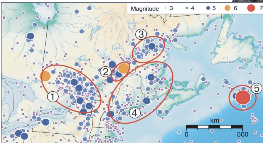
Zones of earthquake activity. This map shows the distribution pattern of earthquakes M3 or greater between 1900 - 2004.
