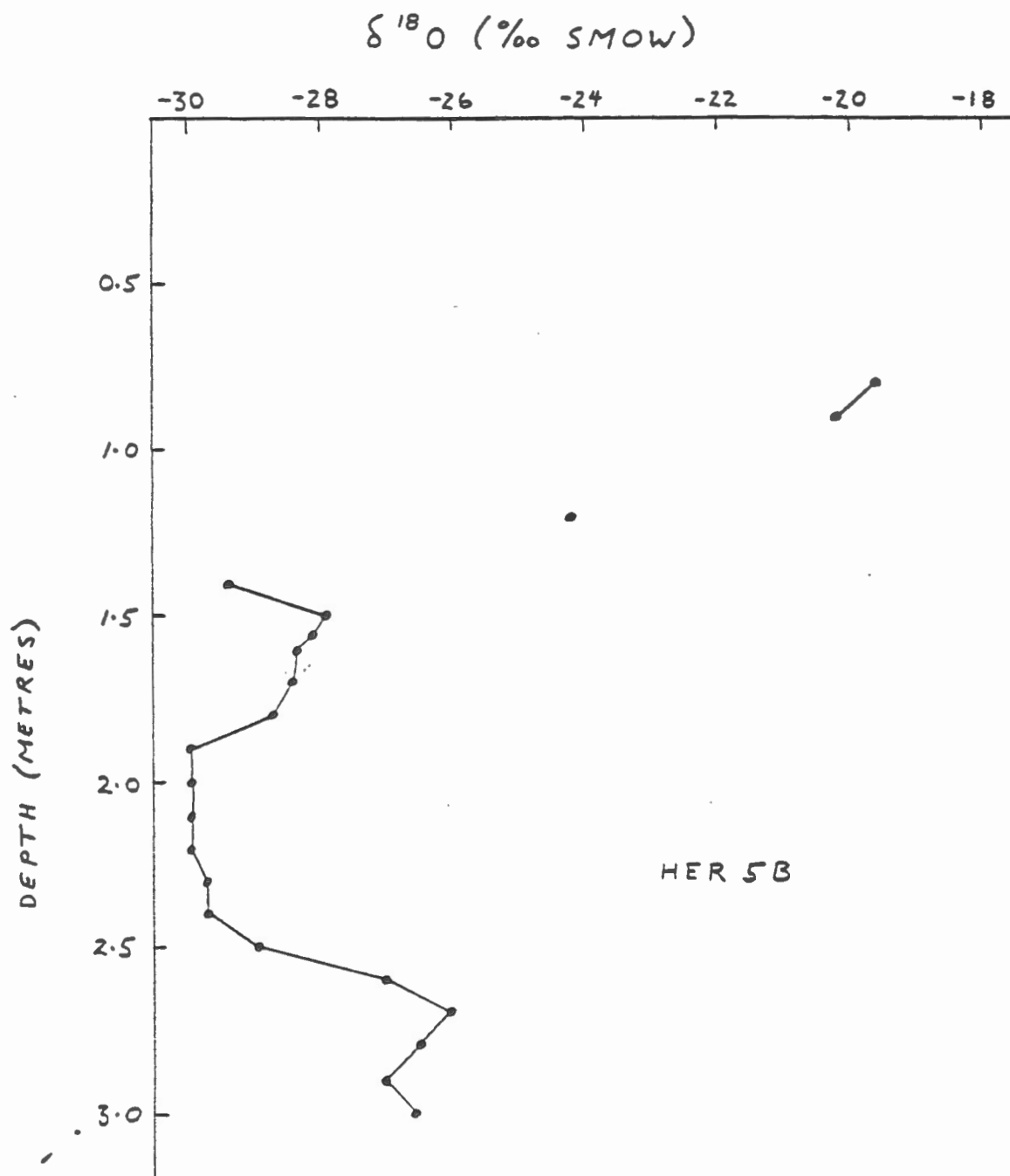
Figure 2.14 Variation in ^{18}\text{O} content with depth for section HER 5B.
