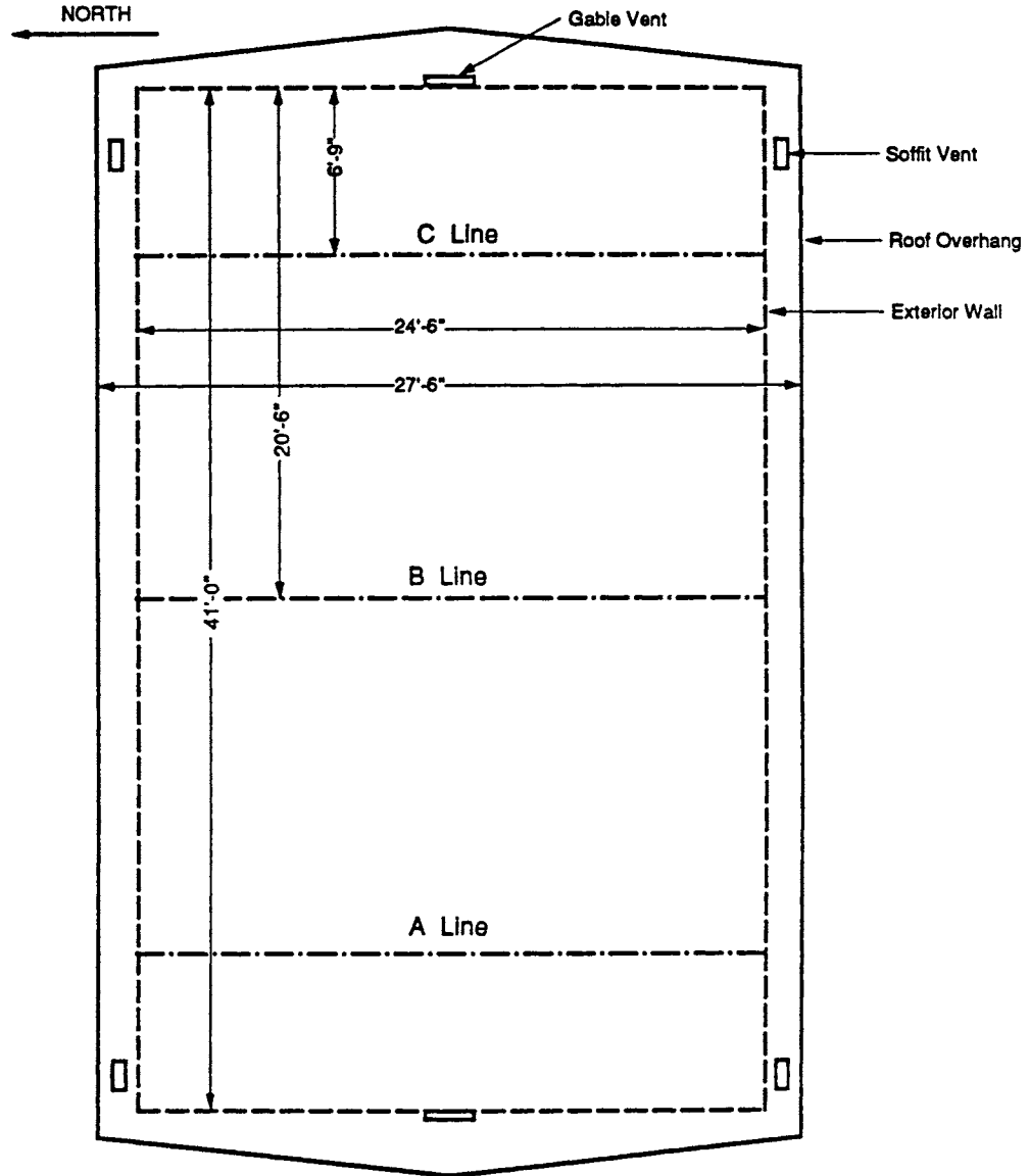
Plan View of Attic
