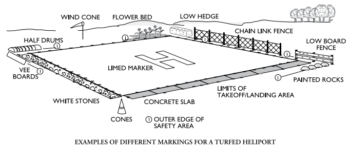
Figure 5.8—FATO Safety Area Marker Examples
