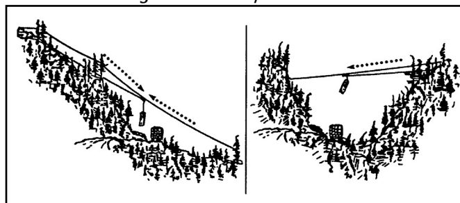
Figure 2.2 – Skyline Crane
