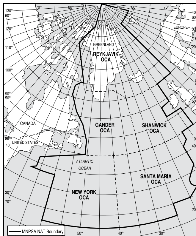
Figure 1.2—NAT HLA Between FL 285 and FL 420
