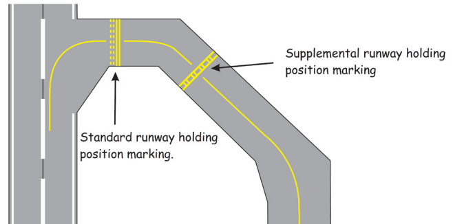
Figure 5.7—Runway Holding Position Markings
