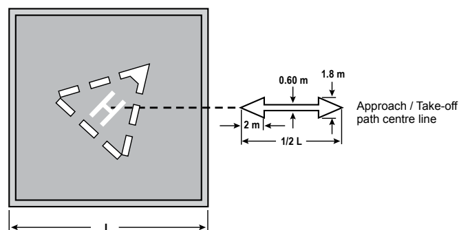
Figure 5.11—Approach and Take-Off Direction Marking
