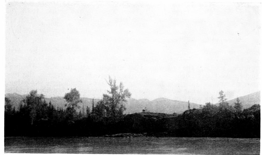
51A. The lava bed, looking southward from the canyon of the Nass River toward Lava Lake.
