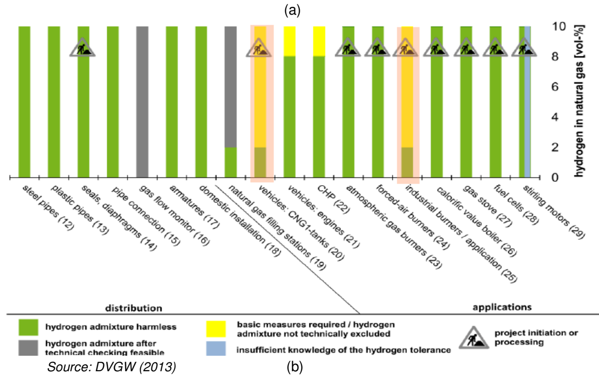
Figure 11: Preliminary H 2 -tolerance information resulted from DVGW project, including the H 2 -tolerance of 29 components belonging to 5 categories of (a) transport, gas storage, measurement and control, (b) distribution, and applications [53]
