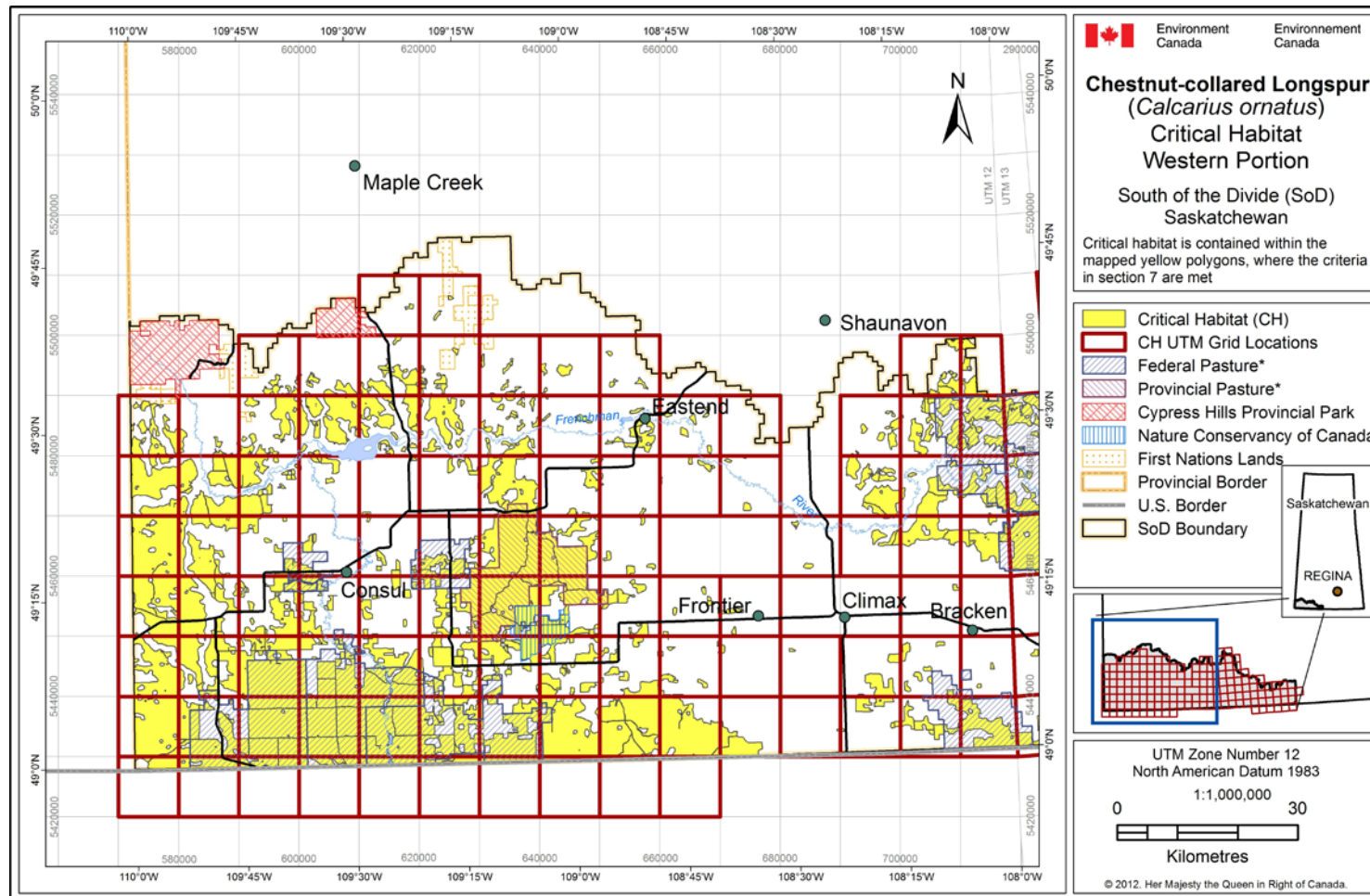
Figure 5. Critical habitat for the Chestnut-collared Longspur in the western portion of southwestern Saskatchewan is represented by the yellow shaded polygons comprising 489,078 ha, where the criteria and methodology set out in Section 7.1 are met. The 10 km x 10 km UTM grid overlay shown on this figure is a standardized national grid system that indicates the general geographic area containing critical habitat. Areas outside of the yellow shaded units do not contain critical habitat. *indicates community pasture boundaries as of August, 2015. Most federal pastures are in the process of being transferred to the province.
