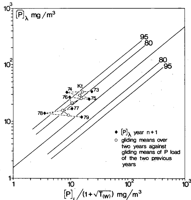
Figure VII 13. Mean total phosphorus concentration (one and two years later) in relation to flushing corrected inflow total phosphorus concentration: Kootenay
