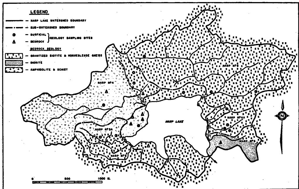
Figure III 1.10 Bedrock geology, sampling sites and basin designation of the Harp Lake watershed
