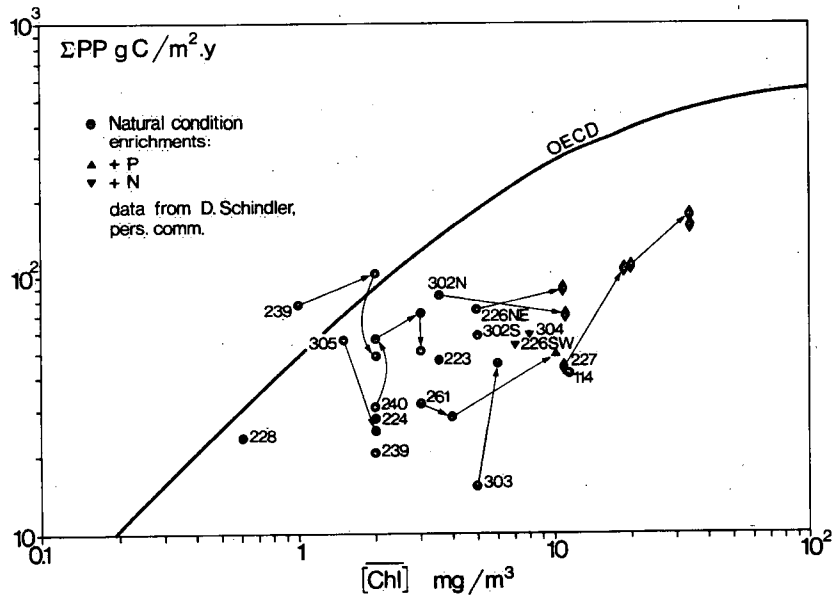
Figure V 15. Annual areal primary production in relation to annual mean chlorophyll a concentration (Schindler)
