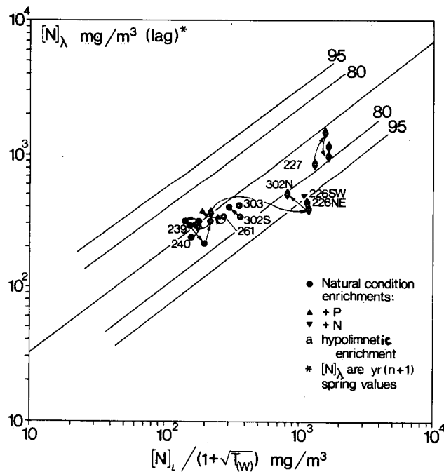
Figure 11. Total nitrogen concentration (one year after inflow measurements) in relation to flushing corrected inflow total nitrogen concentrations
