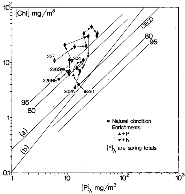
Figure V. 4. Enrichment condition: annual mean chlorophyll a concentration in relation to spring total phosphorus concentration
