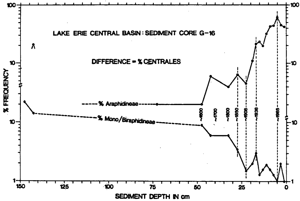
Figure VIII 7. Long term changes of diatoms in the sediments of Lake Erie; from Harris and Vollenweider, 1981.
