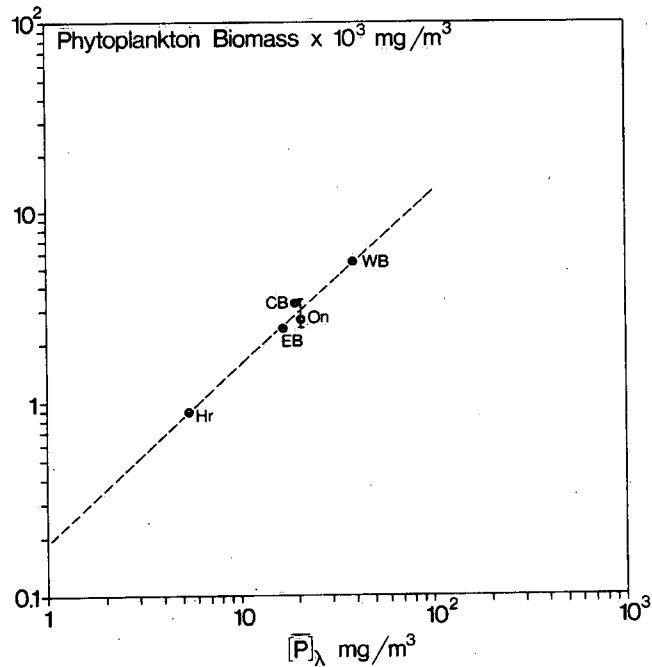
Figure IV 3. Annual mean surface phytoplankton biomass in relation to annual mean total phosphorus concentration
