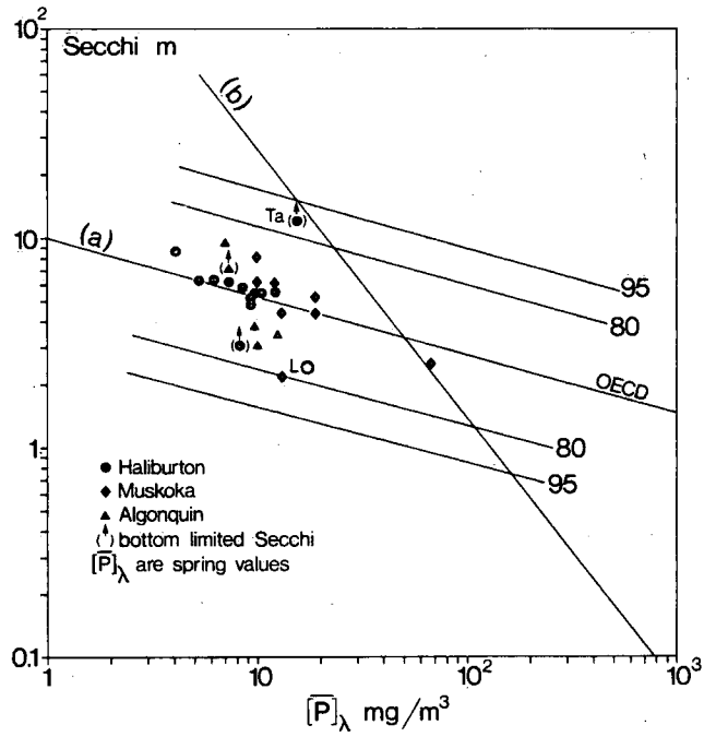
Figure III 14. Secchi transparency in relation to spring total phosphorus concentration
