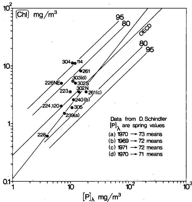
Figure V.2. Natural condition: annual mean chlorophyll a concentration in relation to spring total phosphorus concentration (Schindler)
