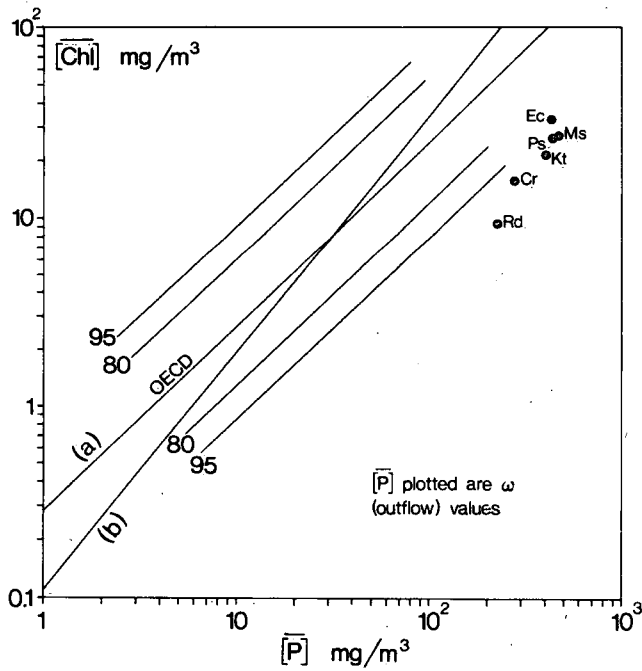
Figure VI 9. Several year mean chlorophyll a concentration in relation to average outflow total phosphorus concentration
