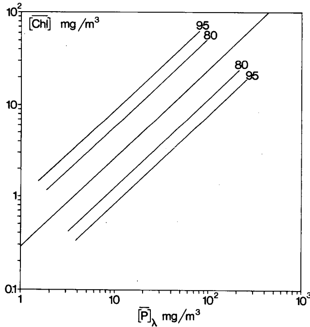
Figure A 1.2 OECD Standard Regression: Annual mean chlorophyll a concentration in relation to annual mean total phosphorus lake concentration: 80 and 95% confidence limits for the a-line
