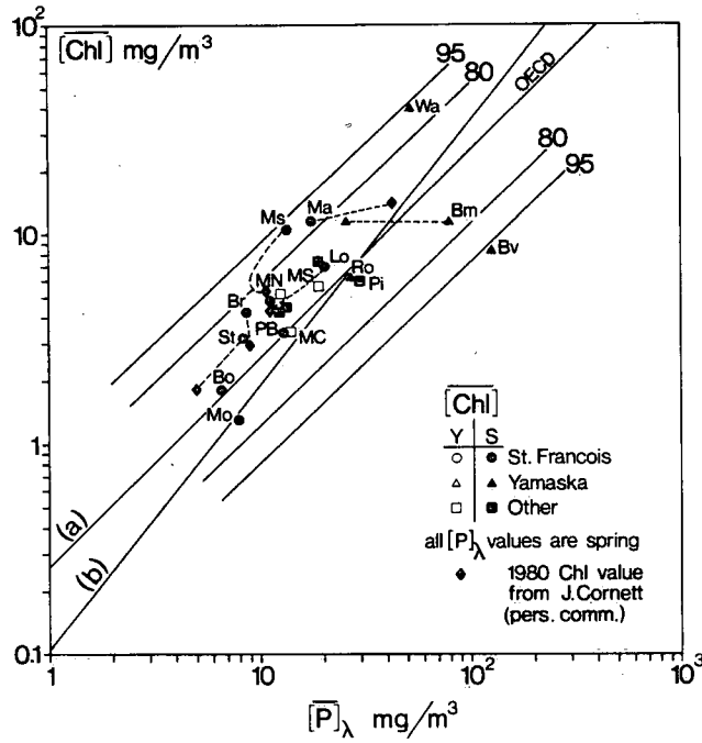
Figure II.3. Annual mean chlorophyll a concentration in relation to spring total phosphorus concentration
