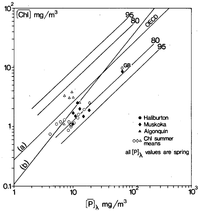
Figure III 4. Annual mean chlorophyll a concentration in relation to spring total phosphorus concentration
