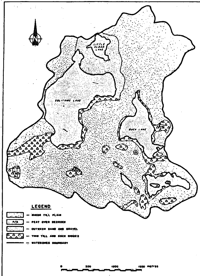
Figure III 2.2 Surficial geology of the Solitaire, Buck and Little Clear Lakes watershed
