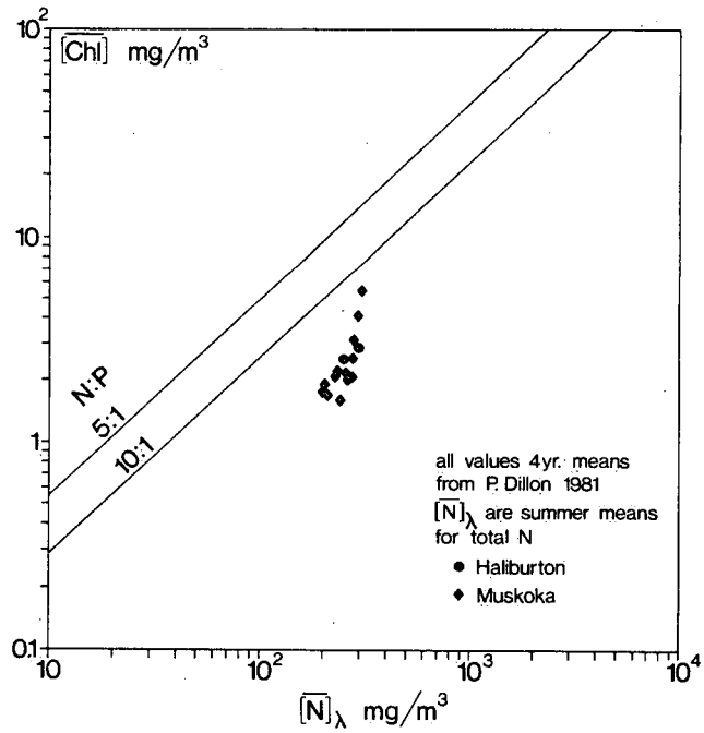
Figure III 9. Annual mean chlorophyll a in relation to total nitrogen concentration of the growing season, 4 year means
