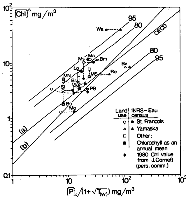
Figure I 6. Mean summer chlorophyll a in relation to flushing corrected inflow total phosphorus concentration
