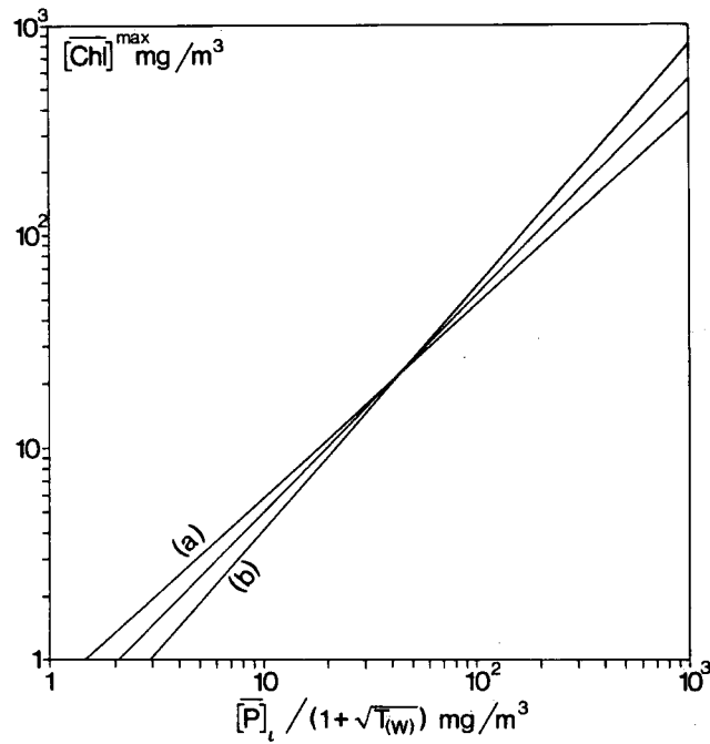
Figure A 1.9 OECD Standard Regression: Maximum chlorophyll a concentration in relation to flushing corrected annual mean total phosphorus inflow concentration: a-, b- and intermediate lines
