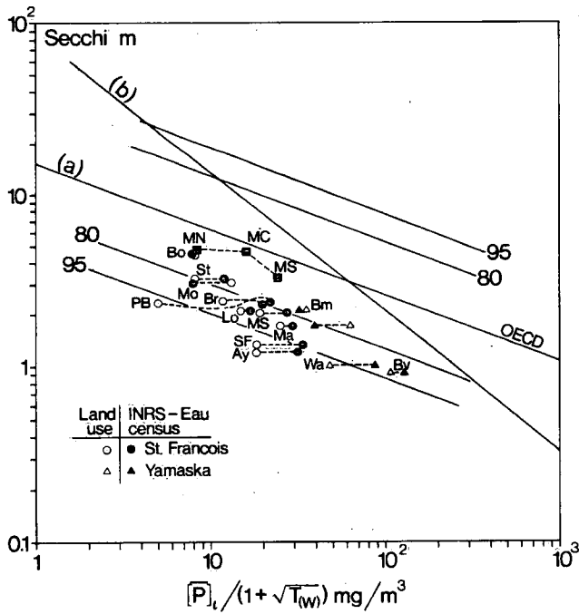
Figure I 10. Secchi transparency in relation to flushing corrected inflow total phosphorus concentration
