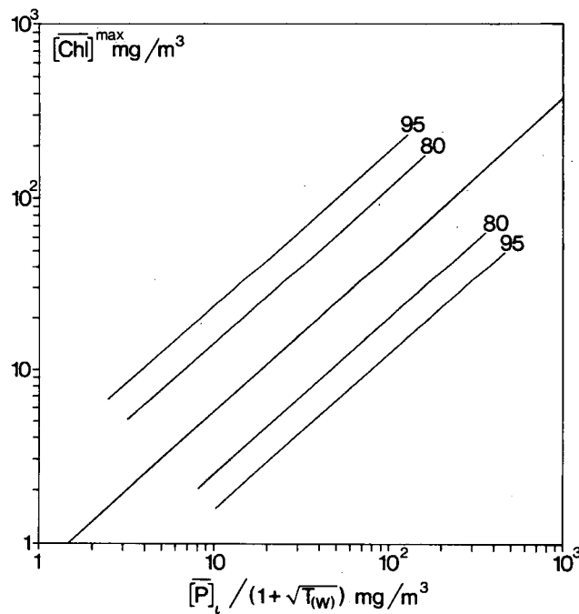
Figure A 1.10 OECD Standard Regression: Maximum chlorophyll a concentration in relation to flushing corrected annual mean total phosphorus inflow concentration: 80 and 95% confidence limits for the a-line
