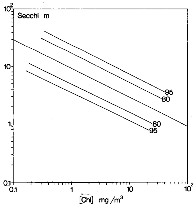
Figure A 1.12 OECD Standard Regression: Annual mean Secchi transparency in relation to annual mean chlorophyll a concentration: 80 and 95% confidence limits for the a-line
