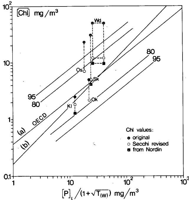
Figure VII 9. Annual mean chlorophyll a concentration in relation to flushing corrected inflow total phosphorus concentration
