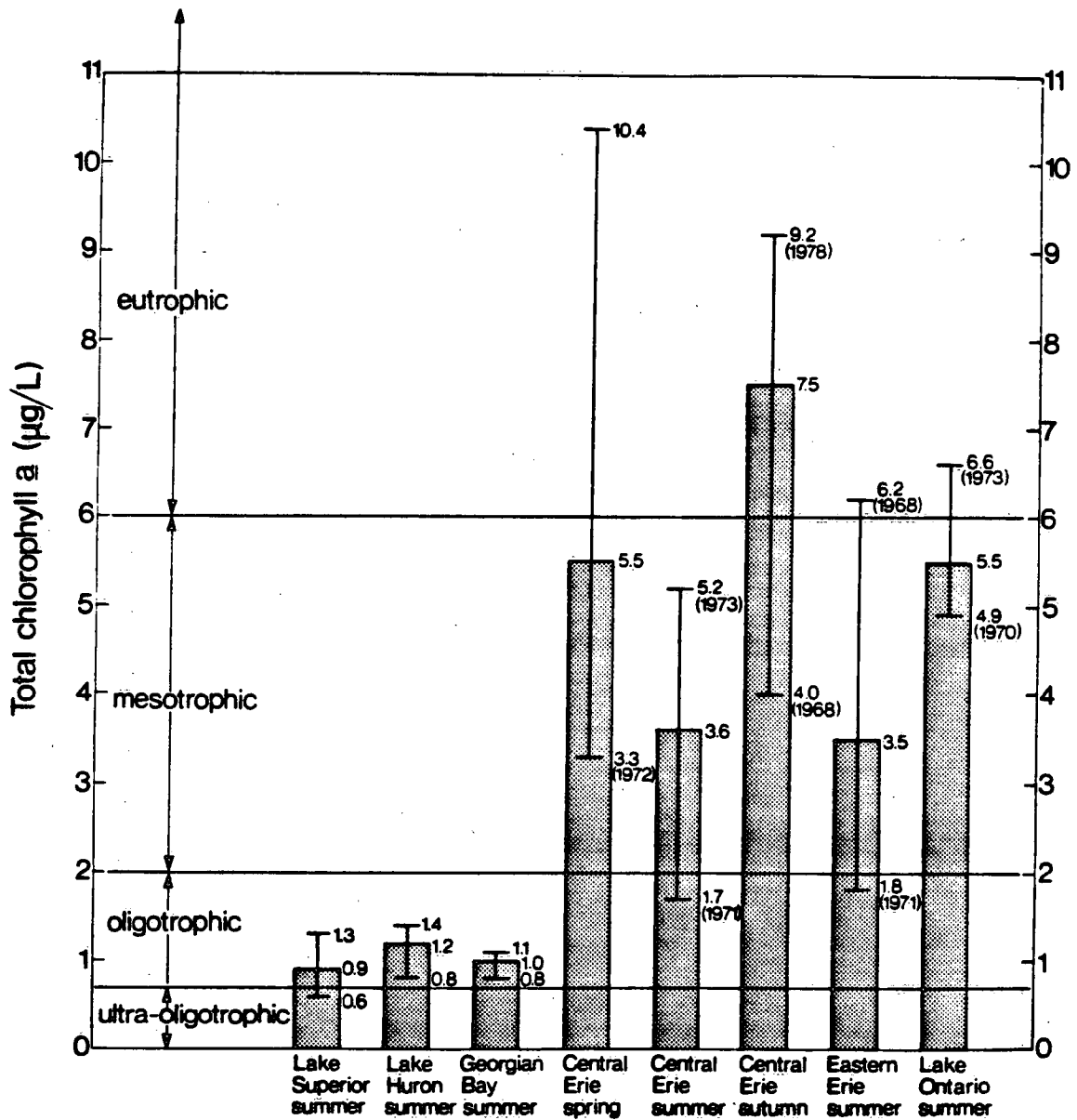
Figure VIII 2. Trophic conditions of the Laurentian Great Lakes in the 1960s and 1970s: Summary of chlorophyll a in offshore surface waters. (Limits are mean values in different years)
