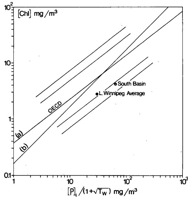
Figure VI 2. Several year mean chlorophyll a concentration in relation to flushing corrected annual mean total phosphorus inflow concentration, Lake Winnipeg
