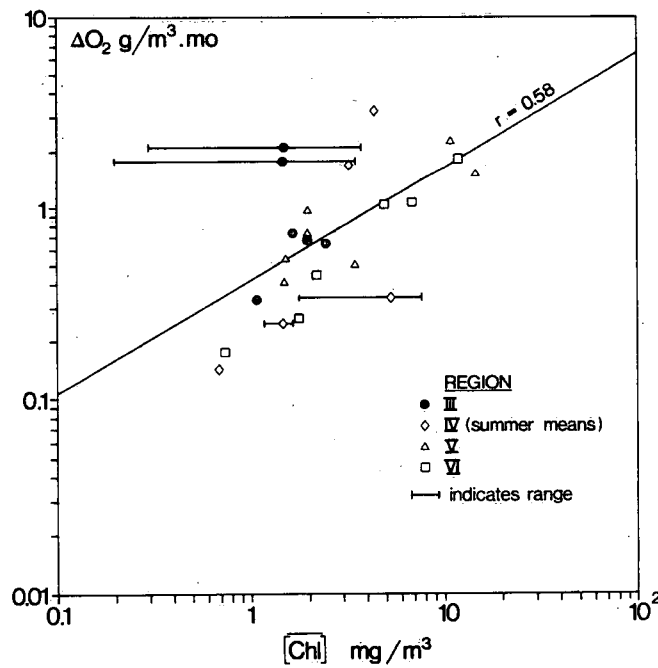
Figure V. 19. Mean monthly hypolimnetic oxygen depletion rate in relation to annual mean chlorophyll a concentration
