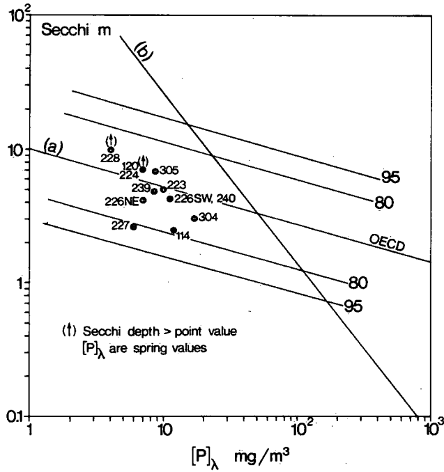
Figure V 14. Secchi transparency in relation to spring total phosphorus concentrations
