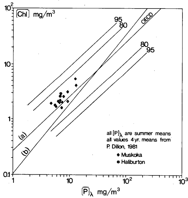
Figure III 7. Annual mean chlorophyll a concentration in relation to mean total phosphorus concentration, 4 year means
