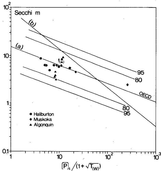
Figure III 17. Secchi transparency in relation to flushing corrected inflow total phosphorus concentration
