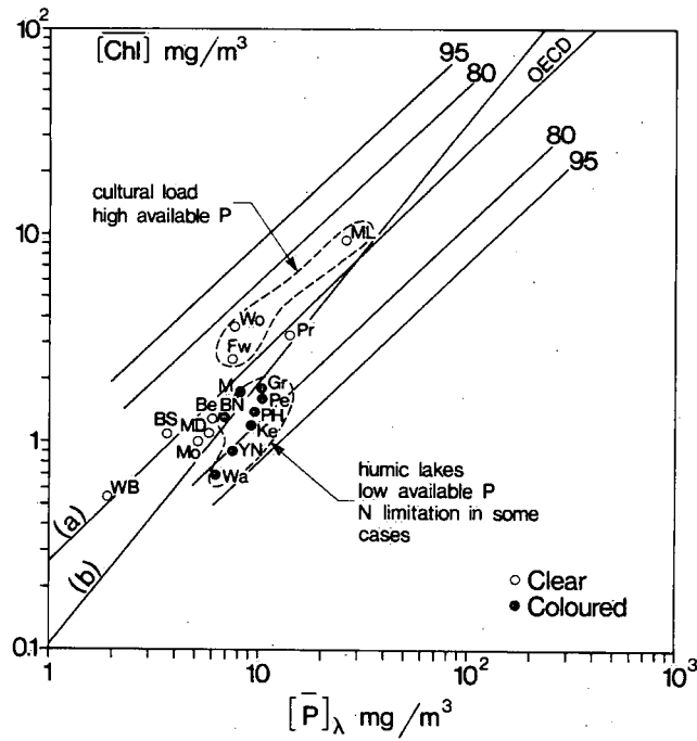
Figure 12. Annual mean chlorophyll a concentration in relation to annual mean total phosphorus concentration.
