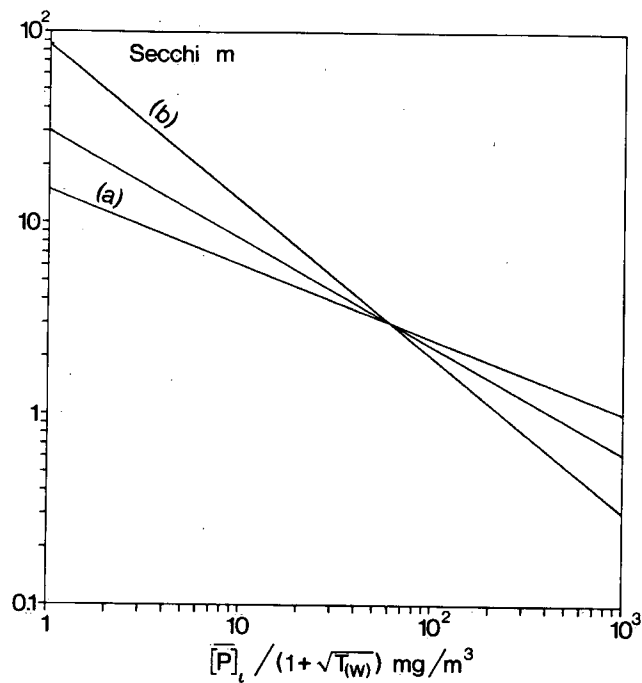
Figure A 1.15 OECD Standard Regression: Annual mean Secchi transparency in relation to flushing corrected annual mean total phosphorus inflow concentration: a-, b- and intermediate lines
