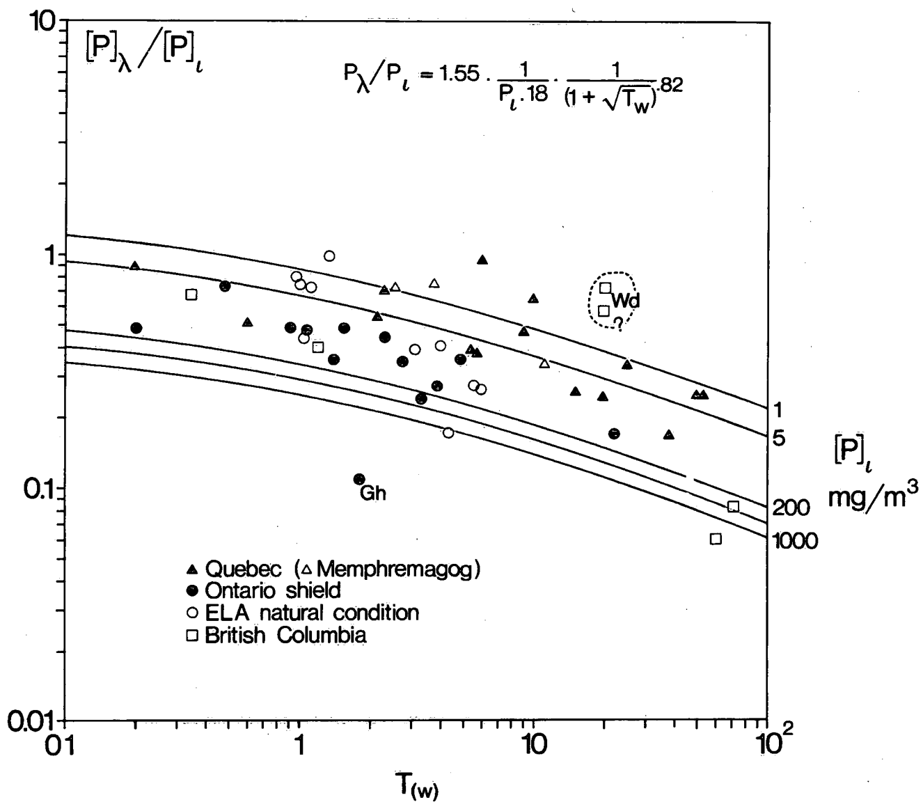
Figure A2.1 Annual mean total phosphorus lake concentration/inflow concentration ratio in relation to theoretical water residence time
