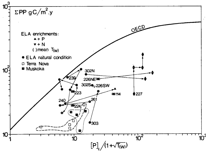
Figure V 16. Annual areal primary production in relation to flushing corrected inflow total phosphorus concentration
