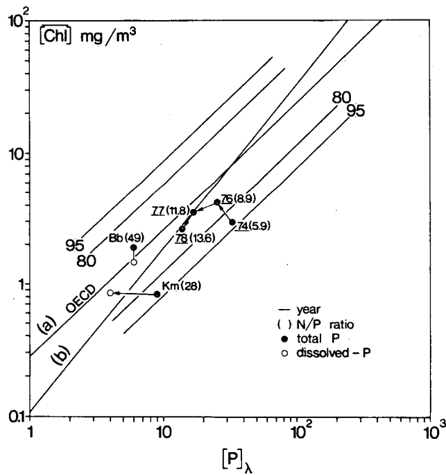
Figure VII 10 Annual mean chlorophyll a concentration in relation to mean phosphorus concentration ( dissolved and total): Kootenay, Kamloops and Babine
