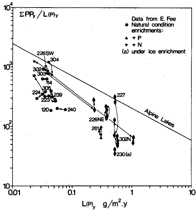
Figure V. 18. Annual areal primary production/annual total phosphorus loading ratio in relation to annual total phosphorus loading
