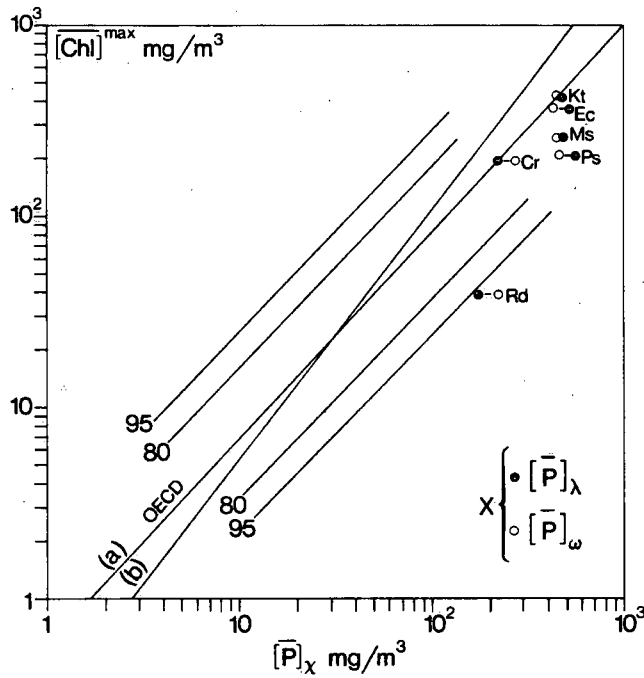
Figure VI 10. Peak chlorophyll a concentration in relation to average inlake and outflow total phosphorus concentration
