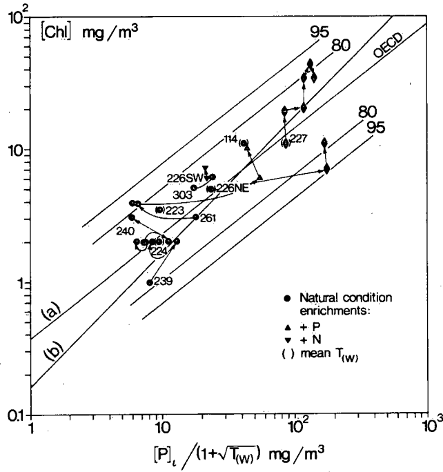
Figure 12. Annual mean chlorophyll a concentration in relation to flushing corrected inflow total phosphorus concentration
