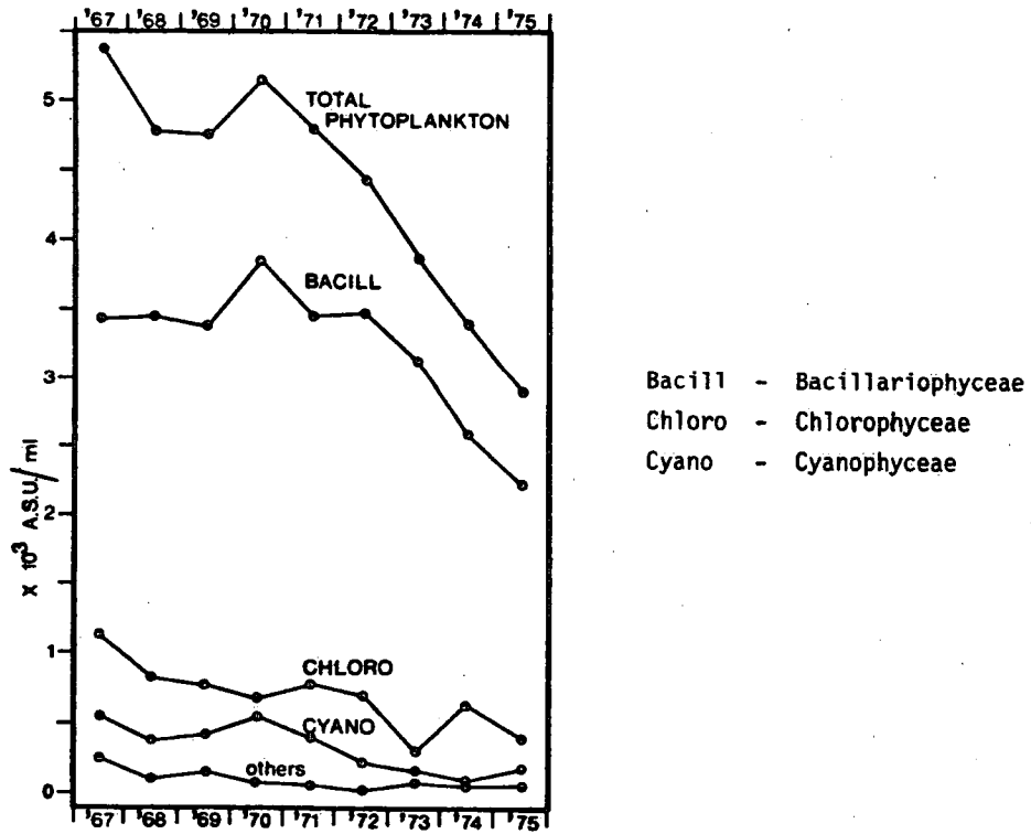
Figure VIII 8. Recent trends in Western Lake Erie phytoplankton - from Nicholls et al., 1977
