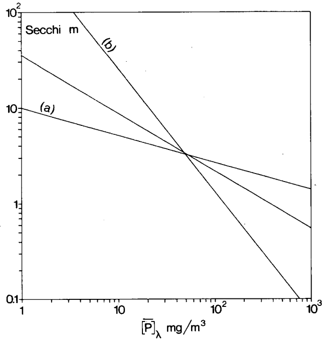
Figure A 1.13 OECD Standard Regression: Annual mean Secchi transparency in relation to annual mean total phosphorus lake concentration: a-, b- and intermediate lines
