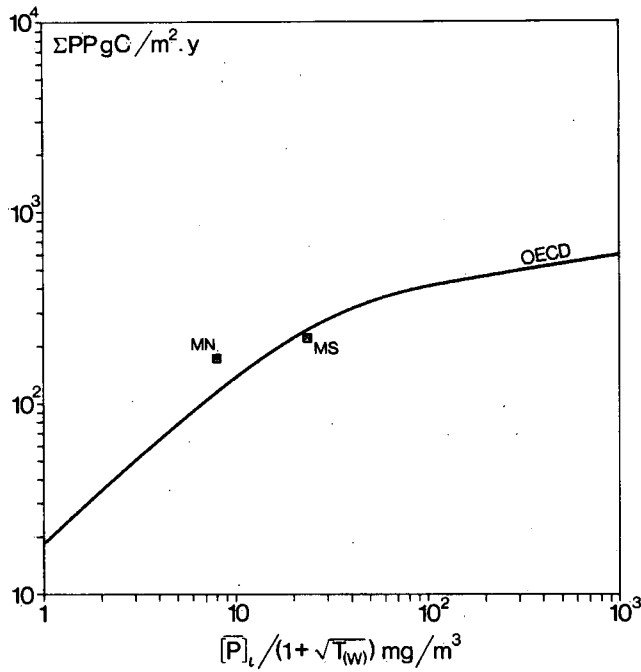
Figure I 7. Annual area primary production in relation to flushing corrected inflow total phosphorus concentration
