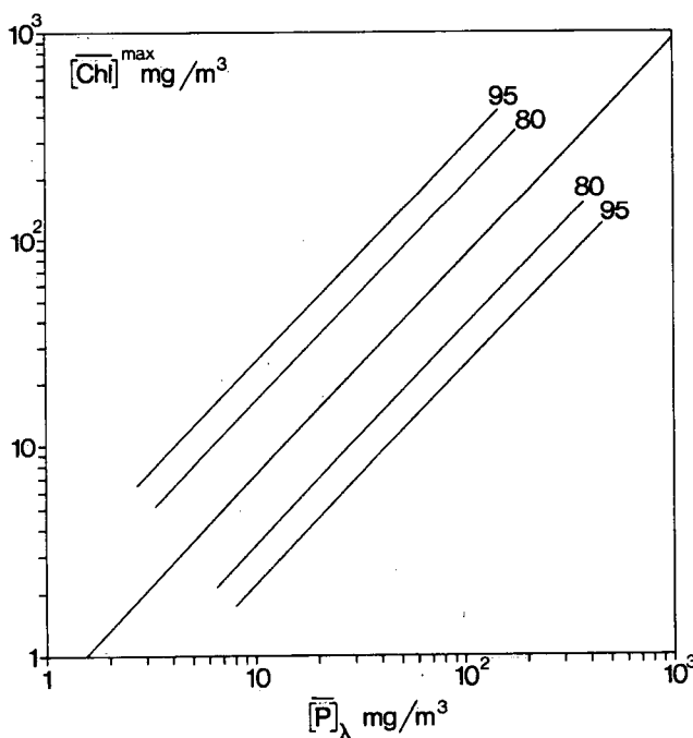
Figure A 1.4 OECD Standard Regression: Maximum chlorophyll a concentration in relation to annual mean total phosphorus lake concentration: 80 and 95% confidence limits for the a-line
