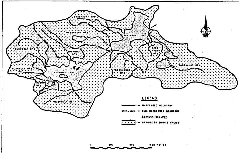
Figure III 1.1 Bedrock geology and basin designation of the Basshaunt Lake watershed
