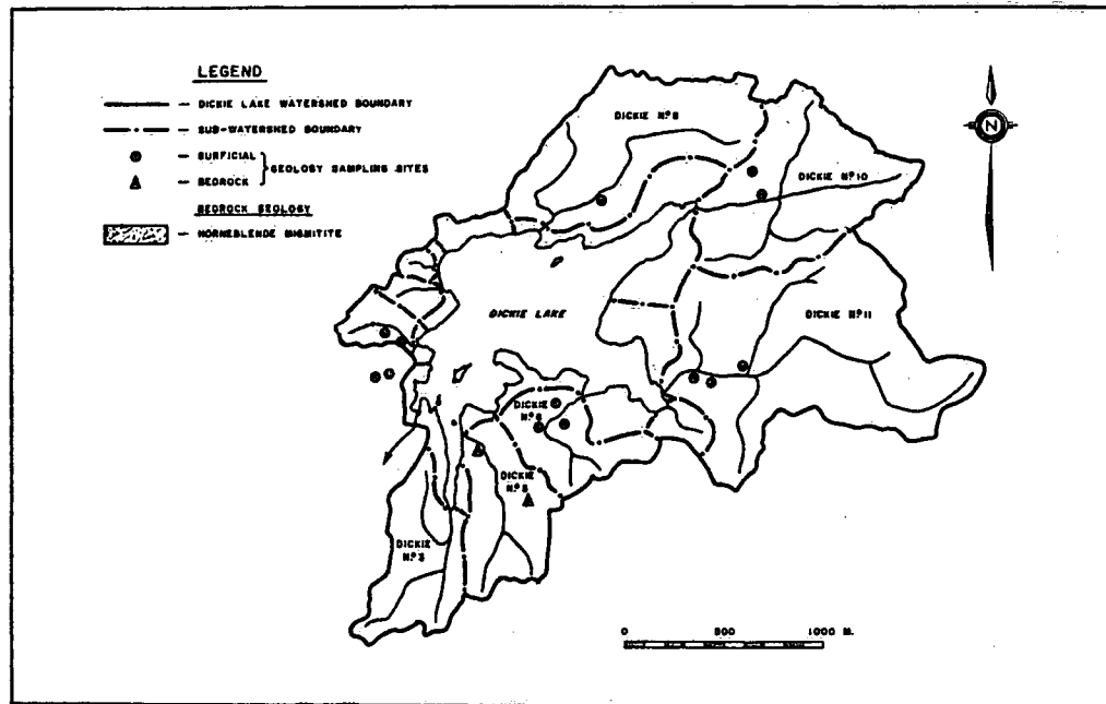
Figure III 1.7 Bedrock geology, sampling sites and basin designation of the Dickie Lake watershed
