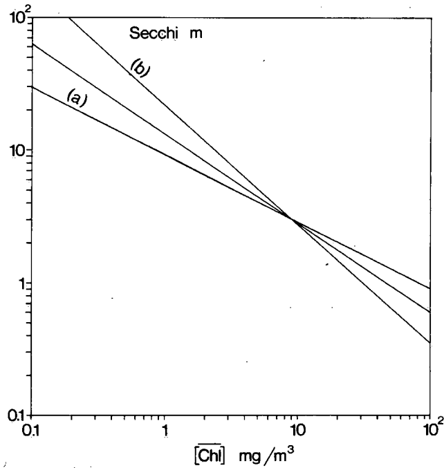
Figure A 1.11 OECD Standard Regression: Annual mean Secchi transparency in relation to annual mean chlorophyll a concentration: a-, b- and intermediate lines
