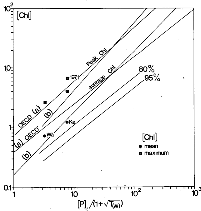
Figure I 5 Annual mean chlorophyll in relation to flushing corrected annual mean inflow total phosphorus concentration.
