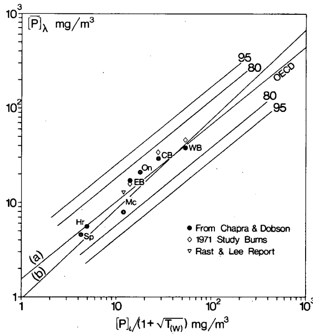
Figure IV 4. Annual mean total phosphorus concentration in relation to the flushing corrected annual mean inflow total phosphorus concentration
