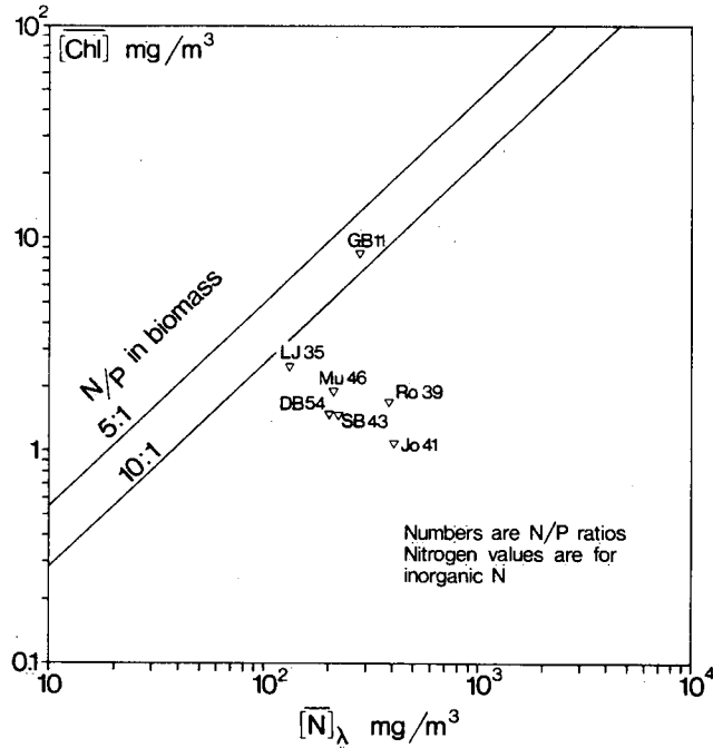
Figure III 8. Annual mean chlorophyll a concentration in relation to mean inorganic nitrogen concentration
