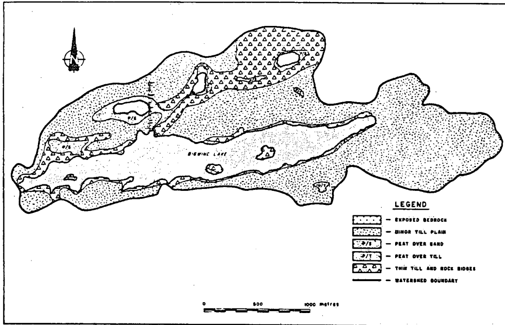
Figure III 2.3 Surficial geology of the Bigwind Lake watershed
