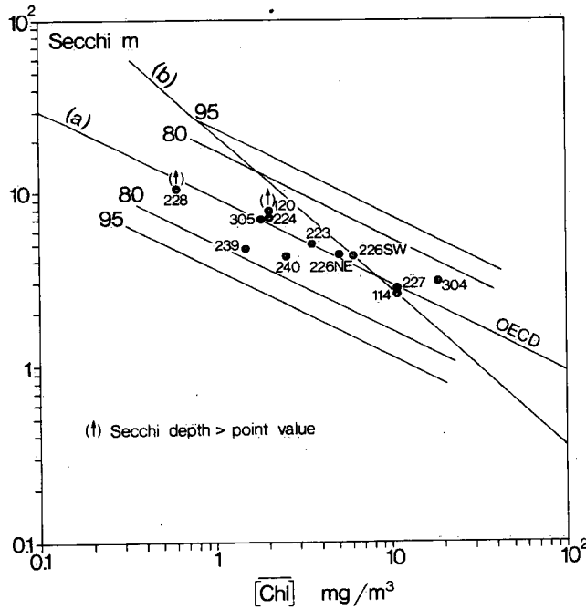
Figure 13. Secchi transparency in relation to annual mean chlorophyll a concentration
