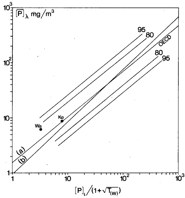
Figure I 4. Annual mean total phosphorus concentration in relation to the flushing corrected annual mean inflow total phosphorus concentration.
