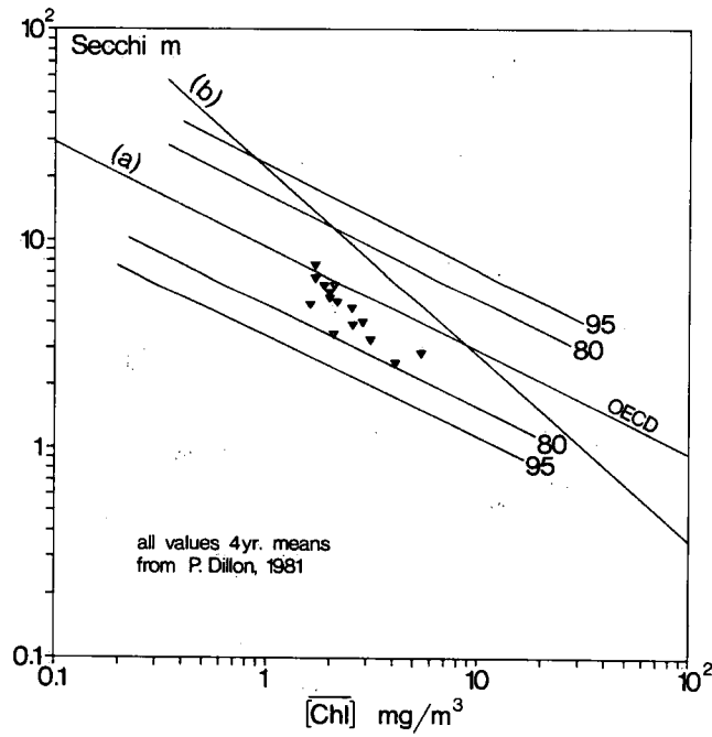
Figure III 13. Secchi transparency in relation to annual chlorophyll a concentration, 4 year means
