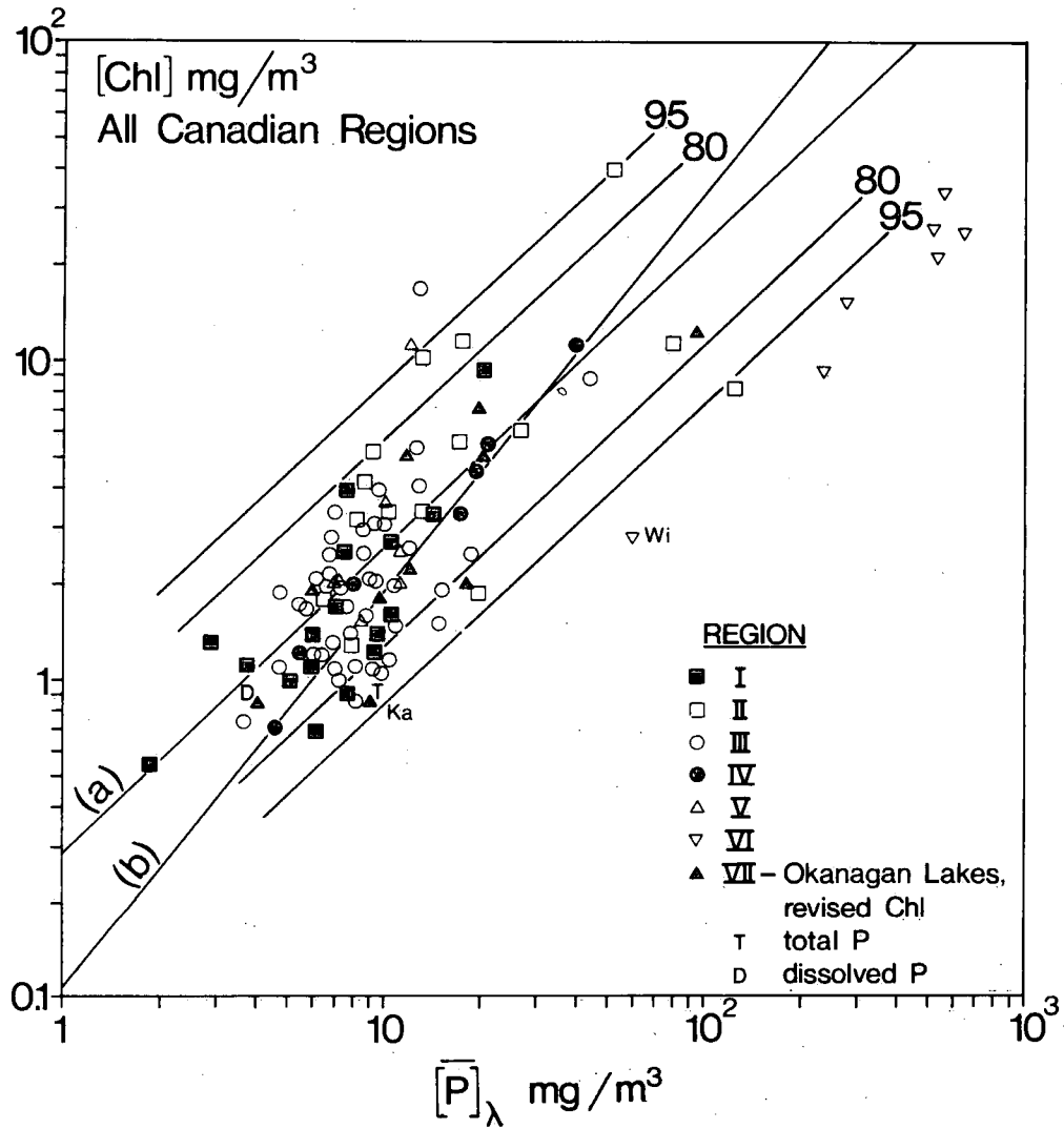
Figure IX 1. Annual mean chlorophyll a concentration in relation to annual mean phosphorus lake concentration
