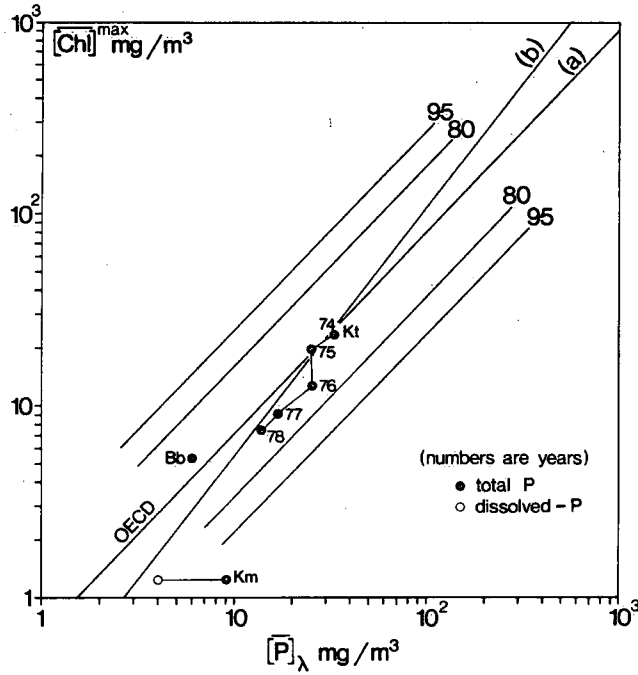
Figure VII 11. Peak chlorophyll a concentration in relation to mean Total phosphorus: Kootenay, Kamloops and Babine
