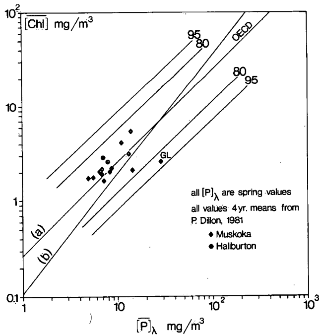
Figure III 5. Annual mean chlorophyll a concentration in relation to spring total phosphorus concentration, 4 year means
