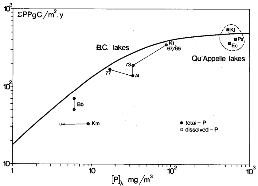
Figure VII 18. Annual areal primary production in relation to mean total phosphorus concentration: Kootenay, Kamloops and Babine
