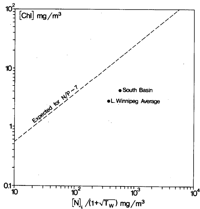
Figure VI 3. Several year mean chlorophyll a concentration in relation to flushing corrected annual mean total nitrogen inflow concentration, Lake Winnipeg
