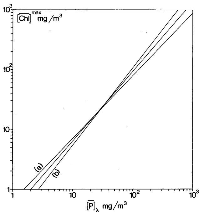
Figure A 1.3 OECD Standard Regression: Maximum chlorophyll a concentration in relation to annual mean total phosphorus lake concentration: a-, b- and intermediate lines
