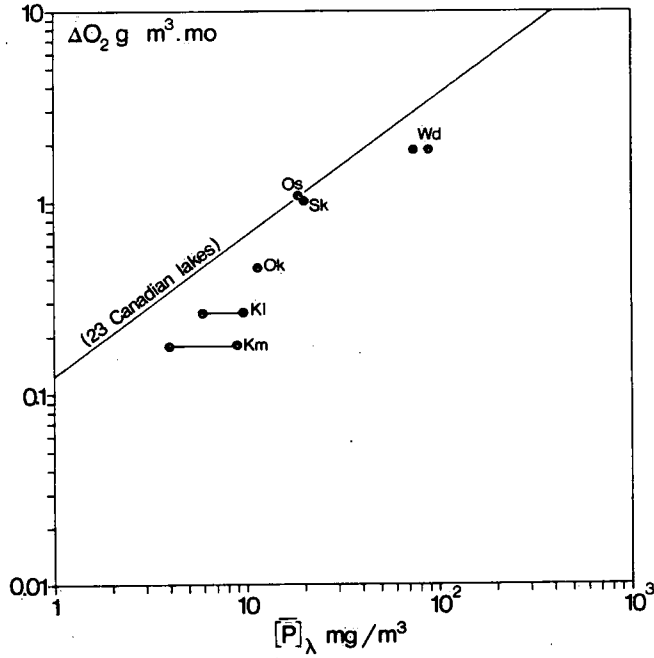
Figure VII 19. Monthly hypolimnetic oxygen demand in relation to mean total phosphorus concentration: B. C. lakes
