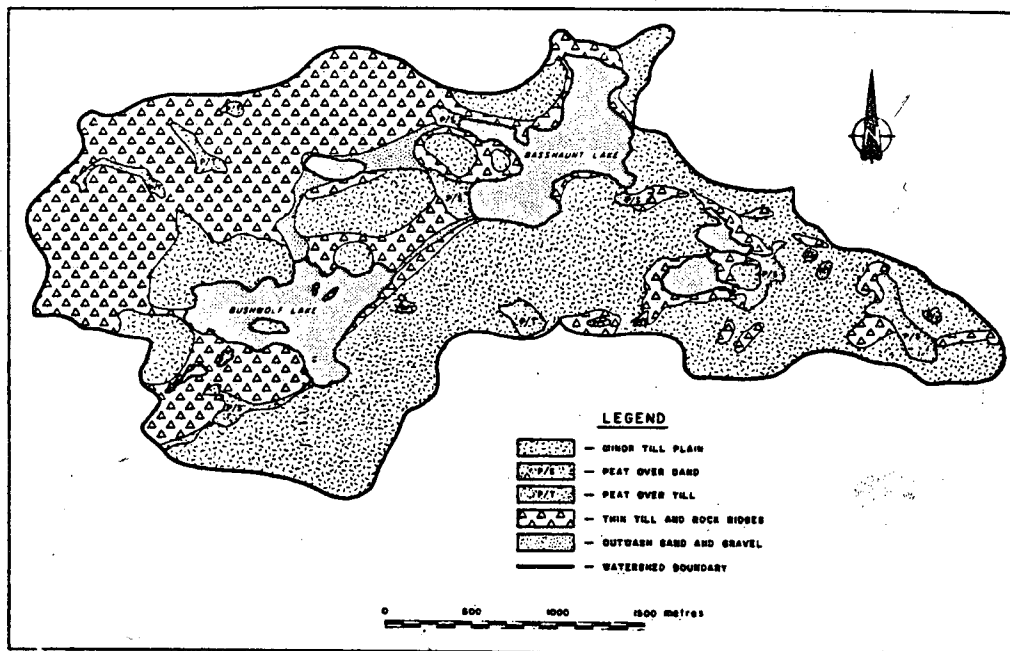
Figure III 2.4 Surficial geology of the Basshaunt-Lake watershed
