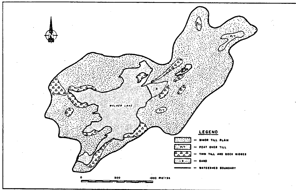
Figure III 2.12 Surficial geology of the Walker Lake watershed
