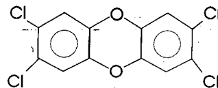
2,3,7,8-tetrachlorodibenzodioxin
