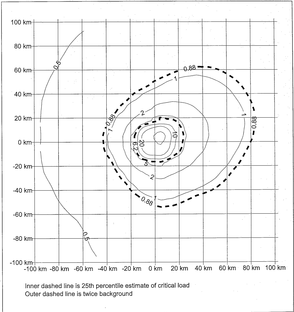
FIGURE 3 Ninety-fifth percentile of total soluble deposition rates ( \text{mg}/\text{m}^2/\text{a} ) estimated by dispersion modelling for copper emitted from a generic copper smelter
