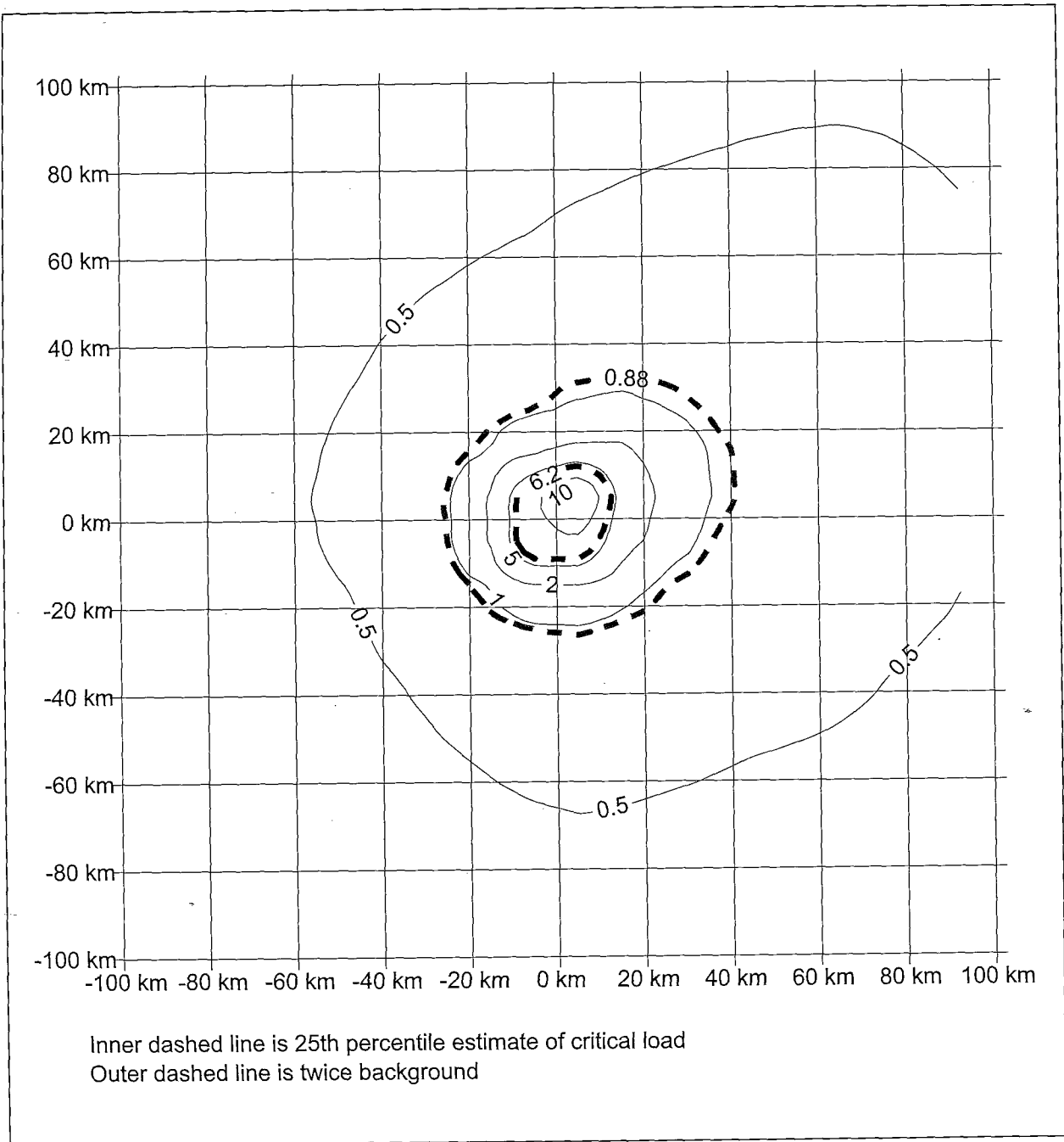
FIGURE 2 Fiftieth percentile of total soluble deposition rates ( \text{mg}/\text{m}^2/\text{a} ) estimated by dispersion modelling for copper emitted from a generic copper smelter
