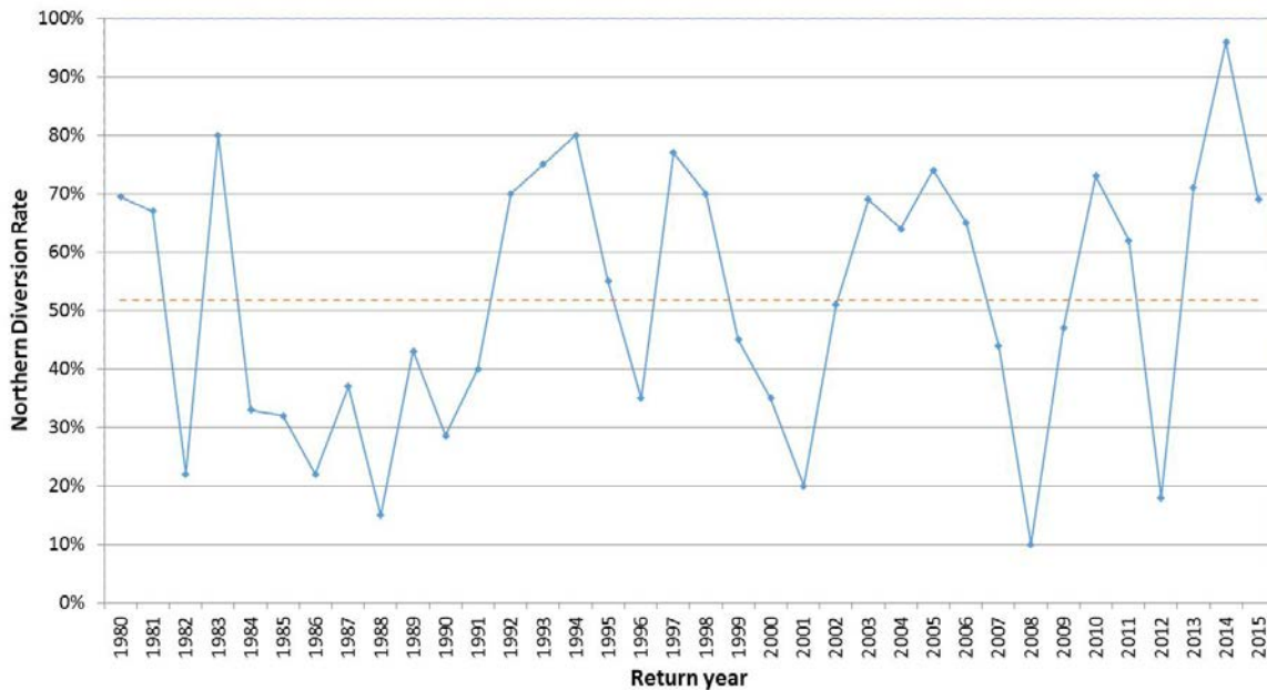
Figure 3. Northern diversion rate of returning Fraser River Sockeye Salmon. The dashed line represents the average percentage ( 52\% \pm 22\% , average \pm standard deviation) of northern diversion between 1980 and 2015. Data provided by the Pacific Salmon Commission, 2015.
