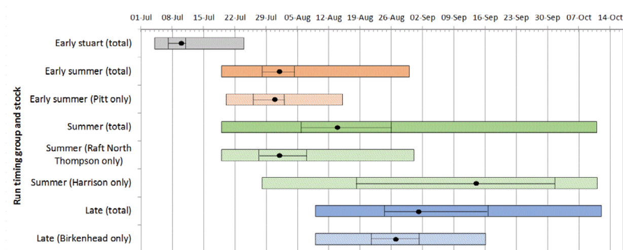
Figure 4. Range at which 50% of the Fraser River Sockeye Salmon Management Groups escaped past Mission (1977 to 2014). The black dots indicate the medians for each Management Group or stock while the vertical bars represent the first and third quartile. Data provided by the Pacific Salmon Commission, 2015.
