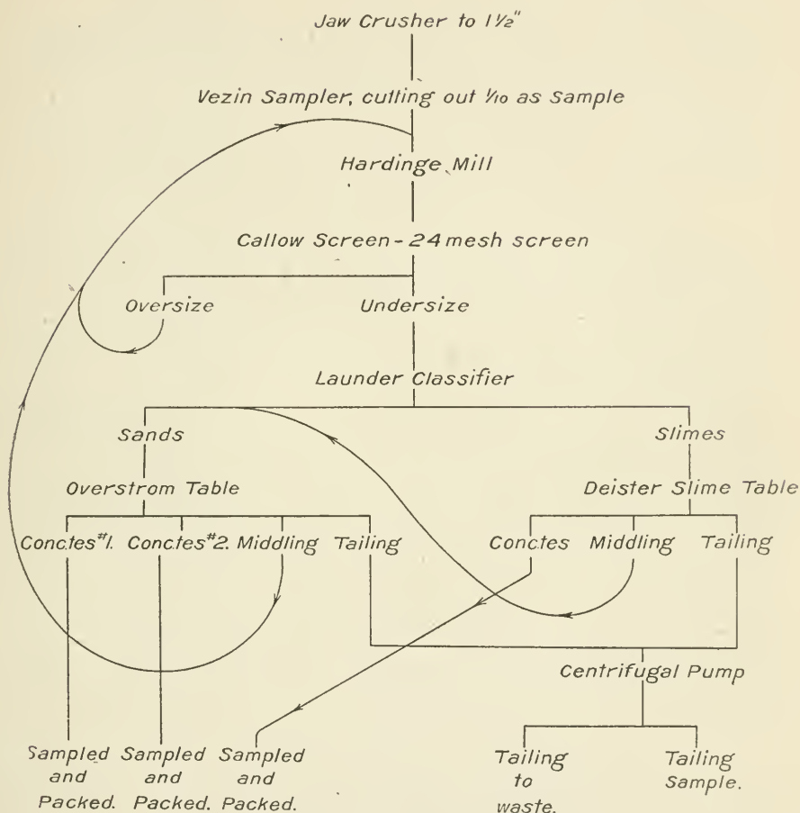
Fig. 3.—Flow sheet, concentration test, Chromite Ore.
