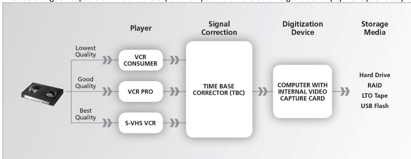
Figure 19. Workflow diagram for Digitization Set-up Three.
