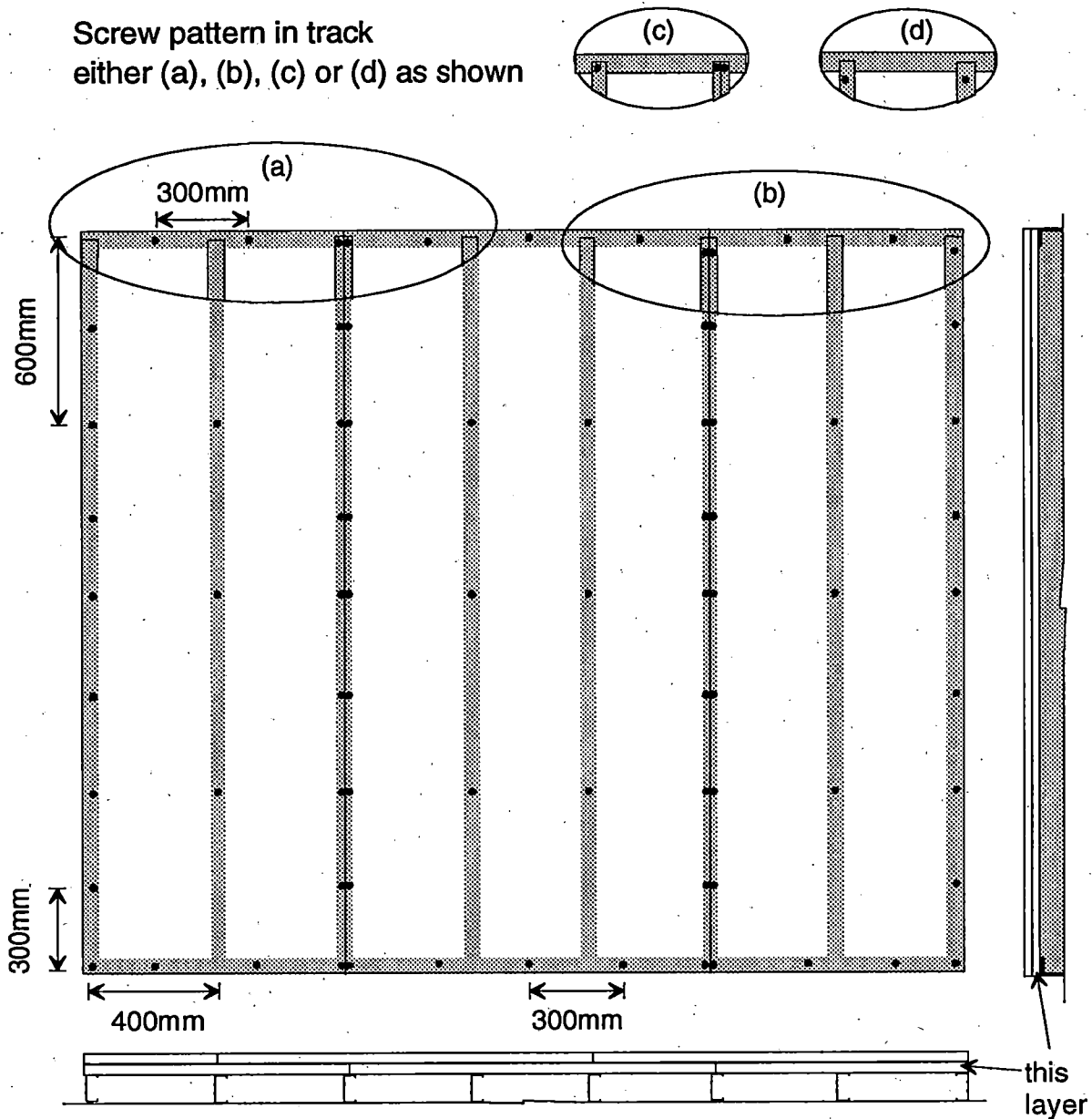
Figure A-23: Base-ply of two-ply gypsum board attached parallel to steel studs at 400 mm o.c., single tracks at top and bottom.. Pattern (a) and (b) meet requirements of CAN/CSA-A82.31-M91, Clause 12.2.3.1, and National Building Code of Canada, Section 9.29.5.9. Drawing not to scale.
