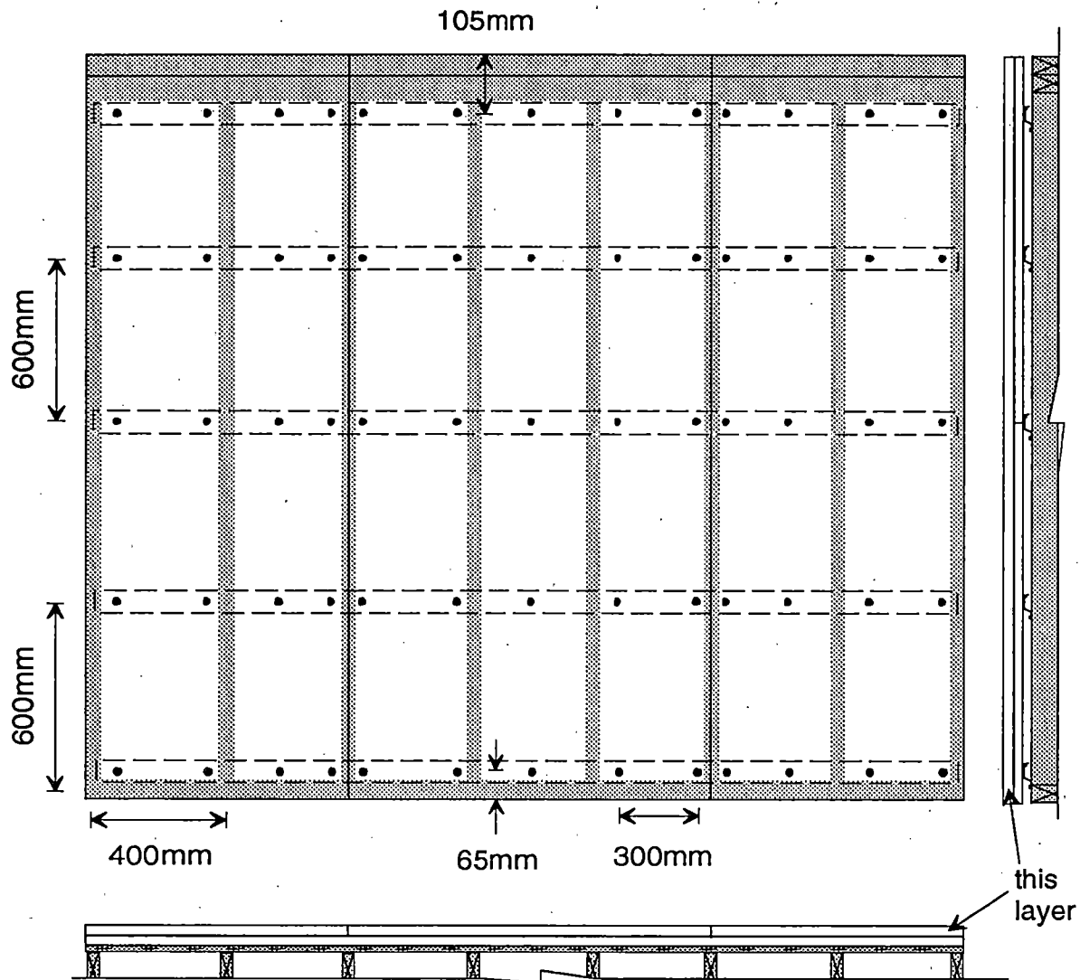
Figure A-12: Face-ply of two-ply gypsum board attached perpendicular to resilient furring channels. Resilient channels attached perpendicular to studs at 600 mm o.c.. Studs at 400 mm o.c.. Meets requirements of CAN/CSA-A82.31-M91, Clause 12.2.3.1. Note that screw spacing was shifted from ideal locations to avoid contact with studs. Drawing not to scale.
