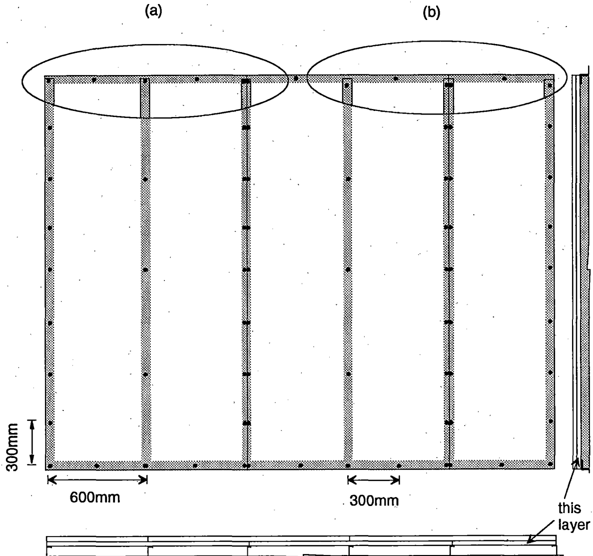
Figure A-20: Base-ply of two-ply gypsum board attached parallel to steel studs at 600 mm o.c., single single tracks at top and bottom. Meets requirements of CAN/CSA-A82.31-M91, Clause 12.2.3.2. Pattern (b) is required for fire resistance (Clause 18.2.6 of CAN/CSA-A82.31-M91 and National Building Code of Canada, Section 9.24.3.2).
