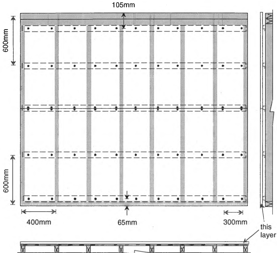
Figure A-10: Single-ply gypsum board attached parallel to resilient furring channels. Studs at 400 mm o.c. Resilient furring channels attached perpendicular to studs at 600 mm o.c.. Note that screw spacing was shifted from ideal locations to avoid contact with studs. Meets requirements of CAN/CSA-A82.31-M91, Clause 12.2.3.1. Drawing not to scale.
