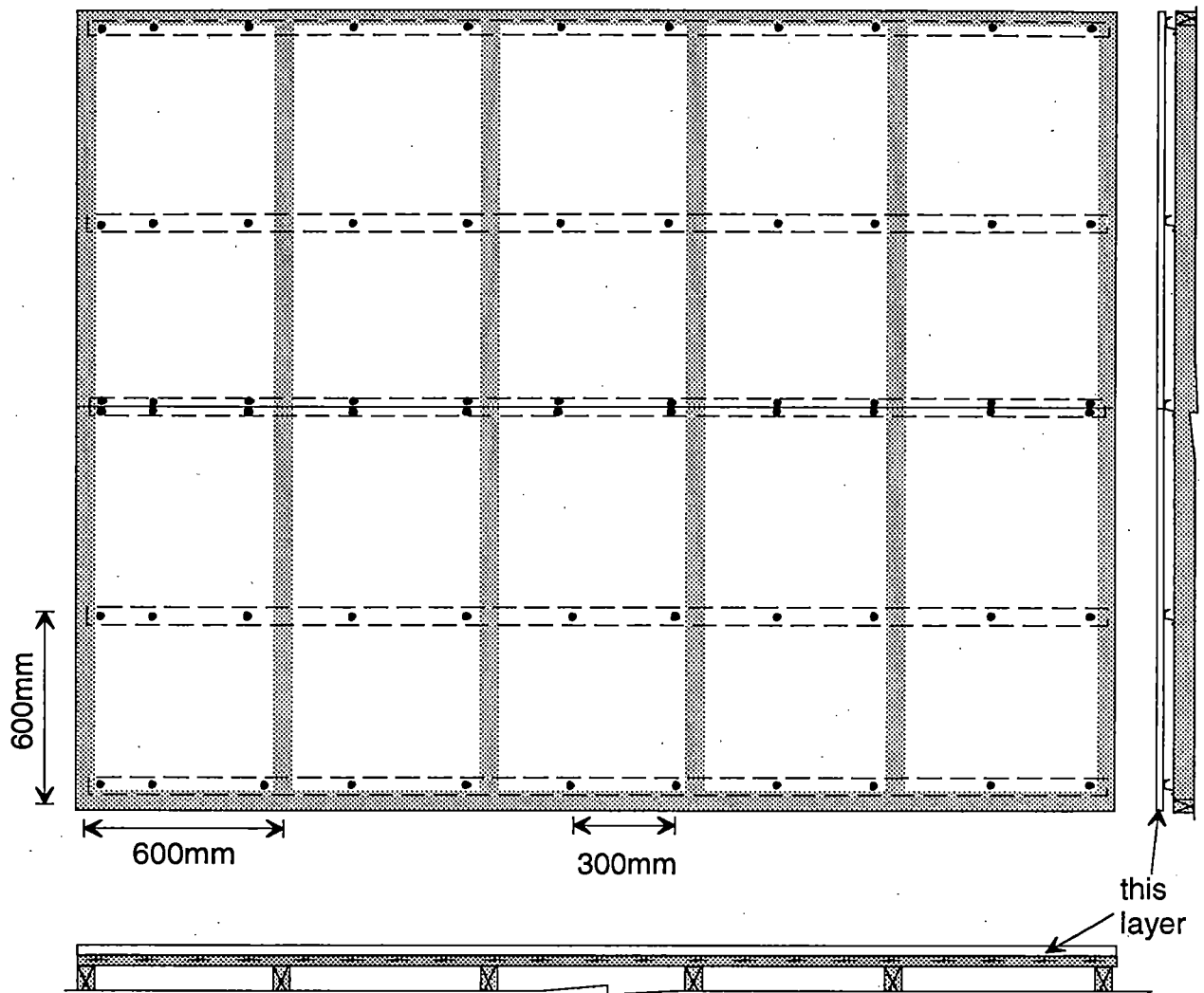
Figure A-7: Single-ply gypsum board attached parallel to resilient furring channels. Resilient channels attached perpendicular to studs at 600 mm o.c.. Wood studs spaced 600 mm o.c., with single plates at top and bottom. Meets requirements of CAN/CSA-A82.31-M91, Clause 12.2.3.1, and National Building Code of Canada, Section 9.29.5.9. Note that screw spacing was shifted from ideal locations to avoid contact with studs. Drawing not to scale.
