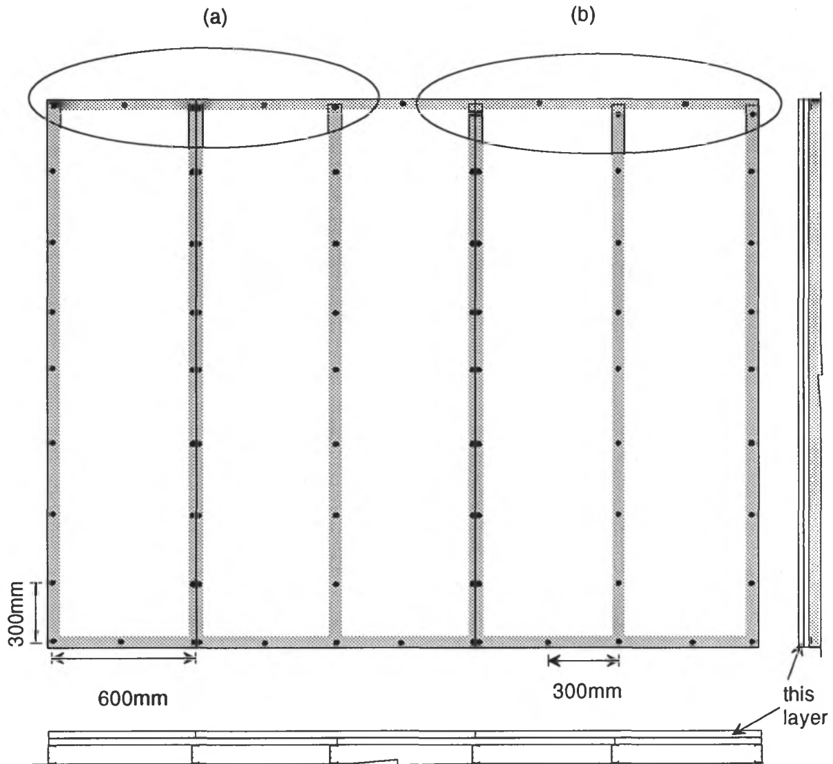
Figure A-21: Face-ply of two-ply gypsum board attached parallel to steel studs at 600 mm o.c., single tracks at top and bottom. Meets requirements of CAN/CSA-A82.31-M91, Clause 12.2.3.1. Pattern (b) is required for fire resistance (Clause 18.2.6 of CAN/CSA-A82.31-M91 and National Building Code of Canada, Section 9.24.3.2).
