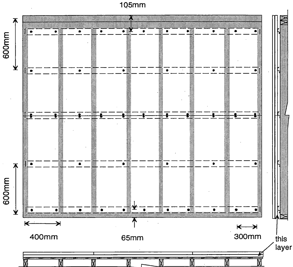
Figure A-11: Base-ply of two-ply gypsum board attached parallel to resilient furring channels. Resilient channels attached perpendicular to studs at 600 mm o.c.. Studs at 400 mm o.c. Meets requirements of CAN/CSA-A82.31-M91, Clause 12.2.3.2. Note that screw spacing was shifted from ideal locations to avoid contact with studs. Drawing not to scale.
