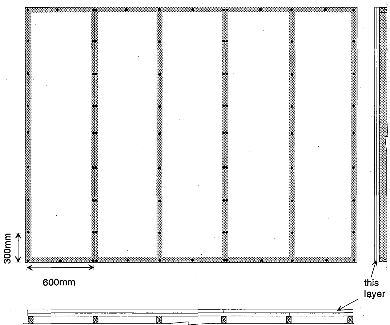
Figure A-3: Face-ply of two-ply gypsum board attached parallel to wood studs at 600 mm o.c., single plates at top and bottom. Meets requirements of CAN/CSA-A82.31-M91, Clause 7.3.4. Drawing not to scale.
