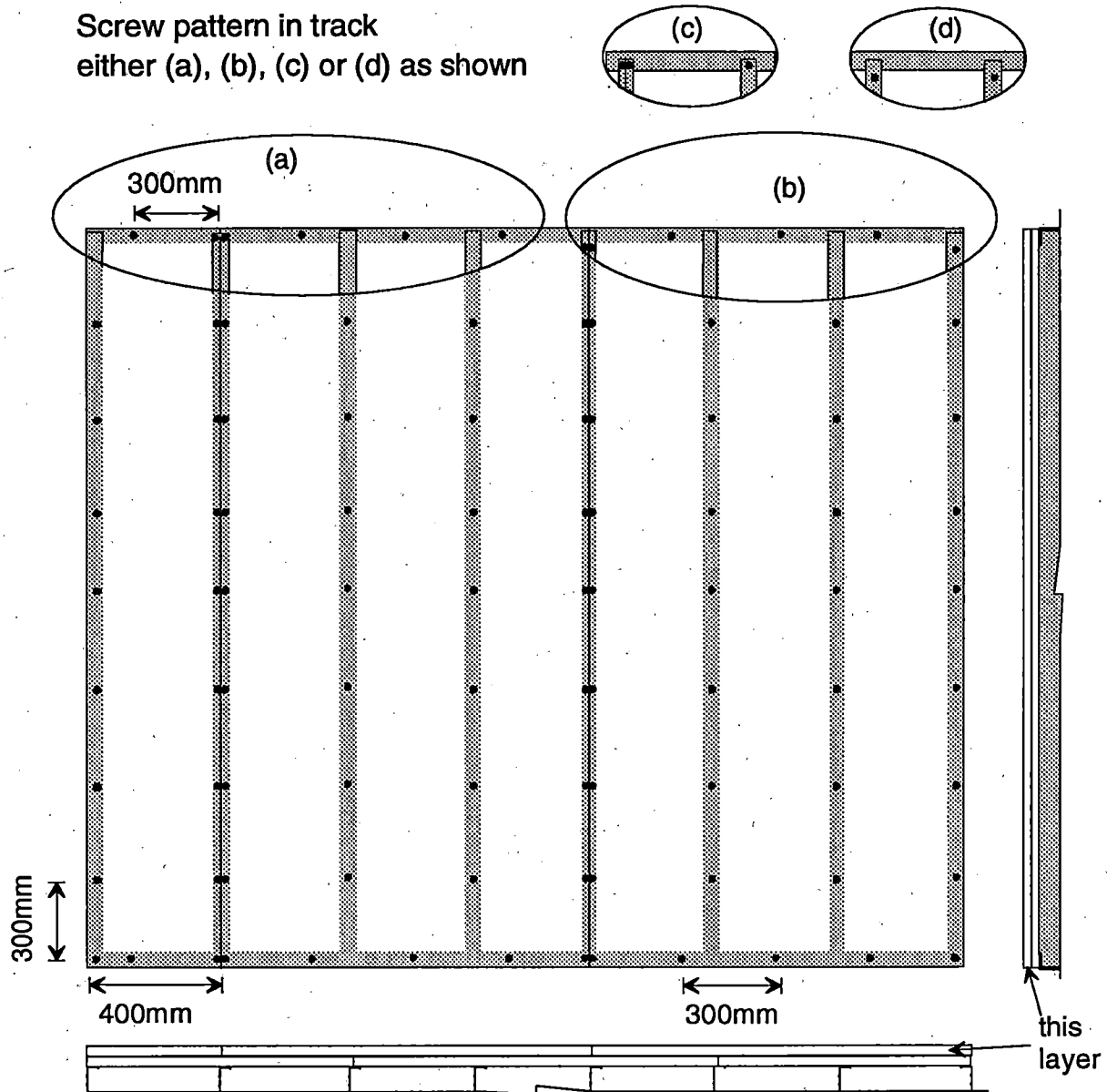
Figure A-24: Face-ply of two-ply gypsum board attached parallel to steel studs at 400 mm o.c., single tracks at top and bottom. Meets requirements of CAN/CSA-A82.31, Clause 12.2.3.1. Drawing not to scale.
