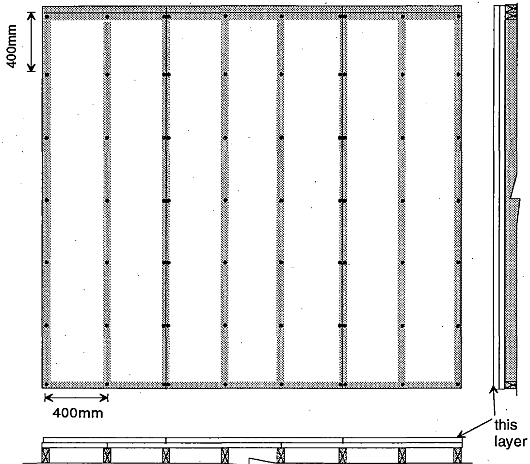
Figure A-6: Face-ply of two-ply gypsum board attached parallel to wood studs at 400 mm o.c., double plate at top, single plate at bottom. Meets requirements of CAN/CSA-A82.31-M91, Clause 7.3.4. Drawing not to scale.
