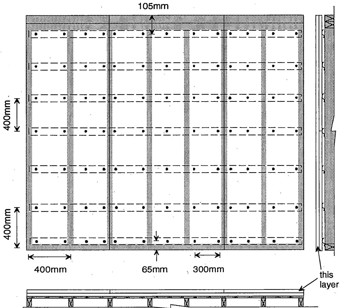
Figure A-18: Face-ply of two-ply gypsum board attached perpendicular to resilient furring channels. Resilient channels attached perpendicular to studs at 400 mm o.c.. Studs at 400 mm o.c., double plate at top, single plate at bottom. Meets requirements of CAN/CSA-A82.31-M91, Clause 12.2.3.1. Note that screw spacing was shifted from ideal locations to avoid contact with studs. Drawing not to scale.
