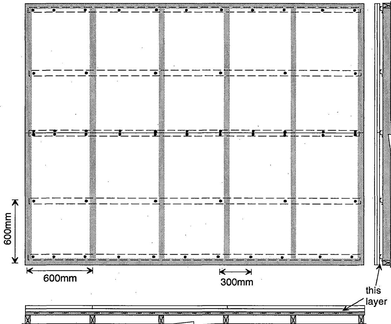
Figure A-8: Base-ply of two-ply gypsum board attached parallel to resilient furring channels. Resilient channels attached perpendicular to studs at 600 mm o.c. Wood studs at 600 mm o.c., with single plates at top and bottom. Meets requirements of CAN/CSA-A82.31-M91, Clause 12.2.3.2. Note that the screw spacing was shifted from ideal locations to avoid contact with studs. Drawing not to scale.
