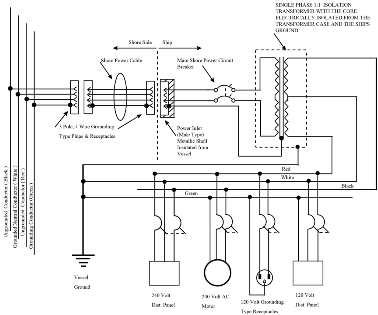
FIGURE 11-1: Isolation Transformer System with Single Phase
