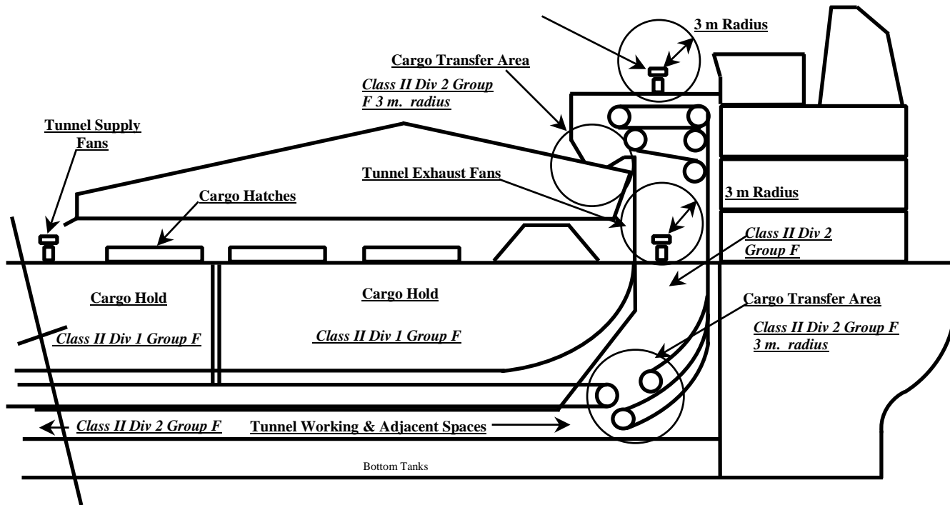
Self Unloader Elevation
