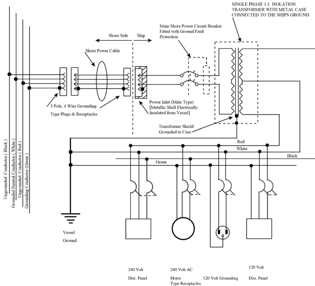
FIGURE 11-2 : Isolation Transformer System with Single Phase 240 Volt Input and 120/240 Volt Single Phase Output with GF Protection of Transformer Primary
