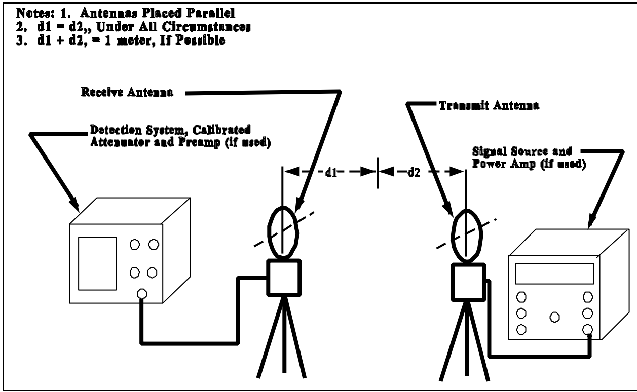
Figure 4 – Test Set-up for Magnetic Field Reference Measurement
