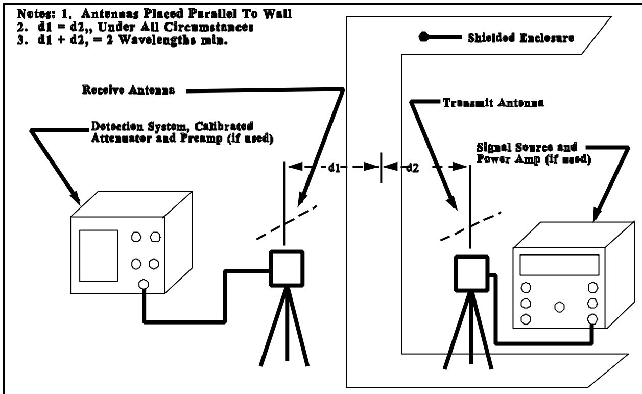
Figure 7 – Test Set-up for Plane-wave Measurement
