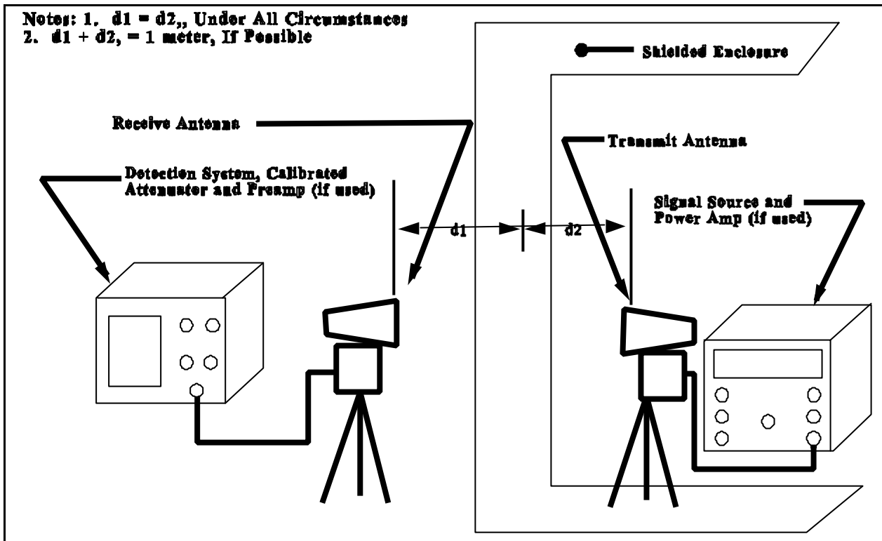
Figure 8 – Test Set-up for Plane-wave Measurement
