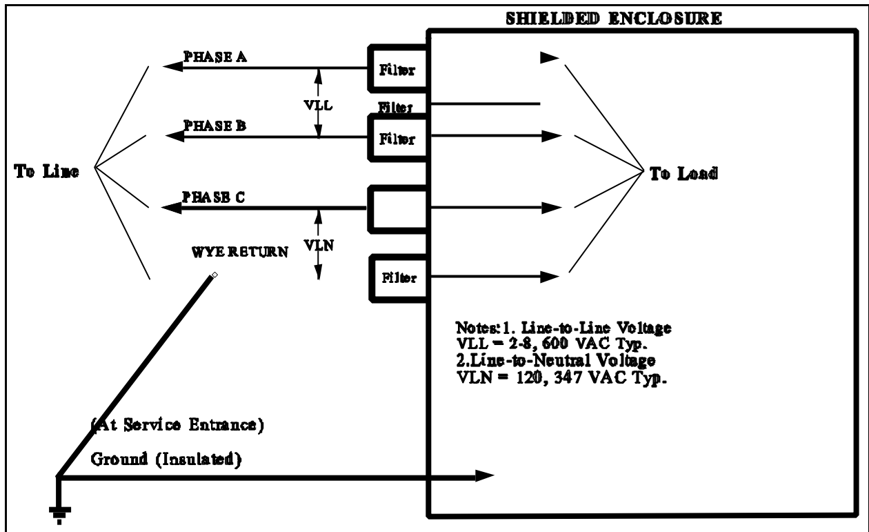
Figure 12 – Typical Power Line Configuration for 3 Phase, WYE
