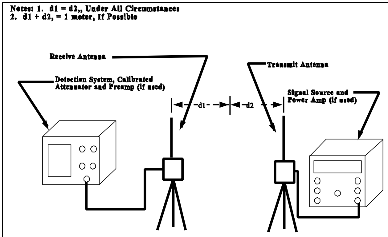
Figure 6 – Test Set-up for Electric Field Reference Measurement
