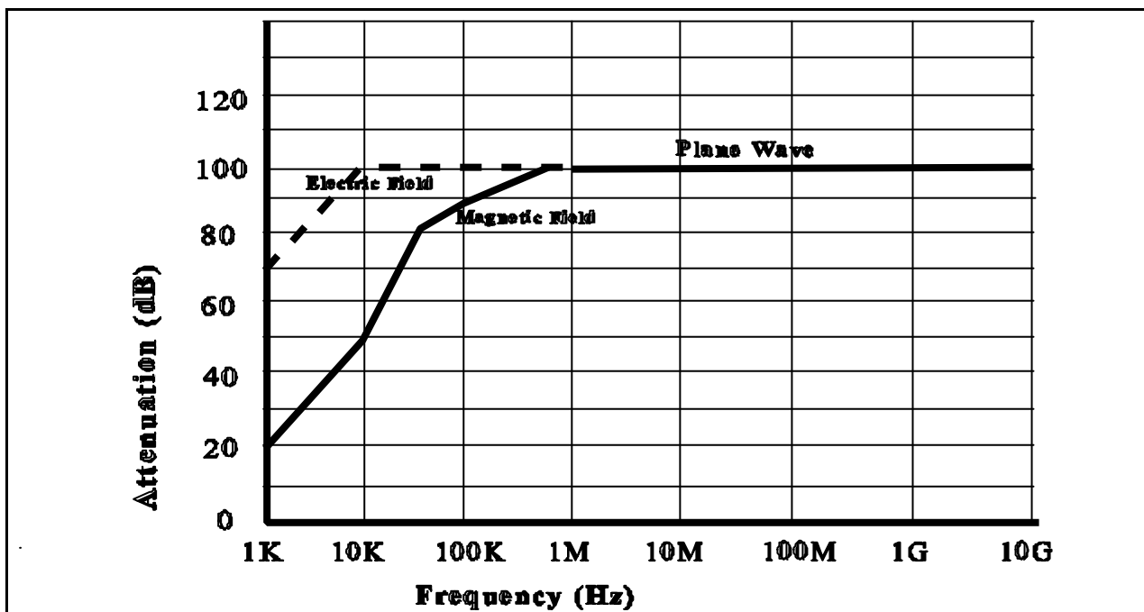
Figure 2 – Electromagnetic Attenuation Required
