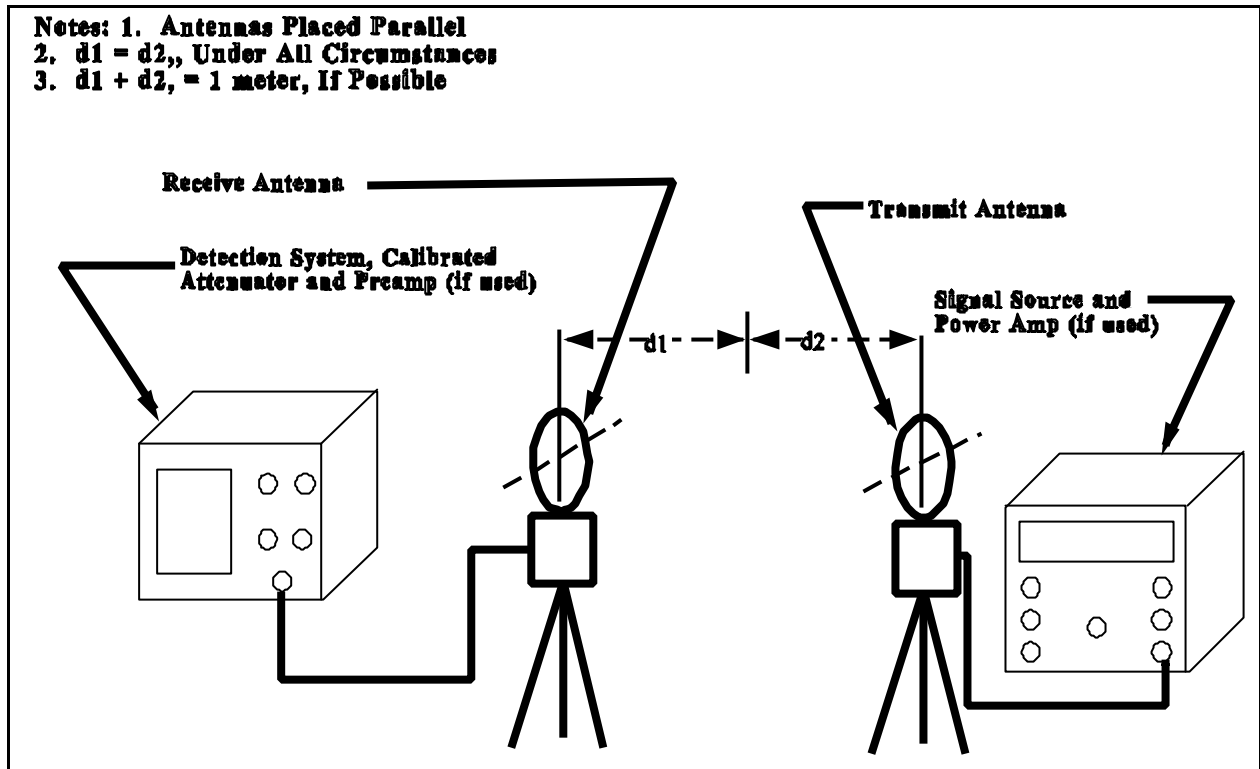
Figure 5 – Test Set-up for Electric Field Measurements
