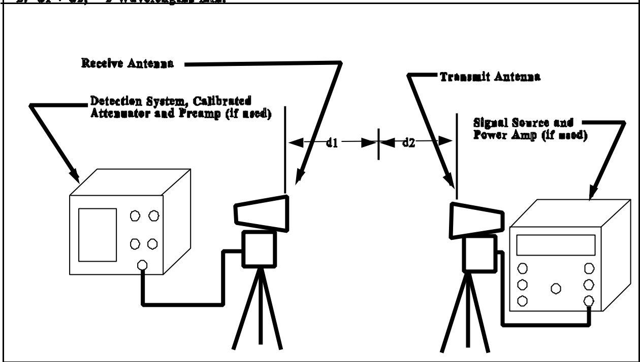
Figure 9 – Test Set-up for Plane-wave Reference Measurement
