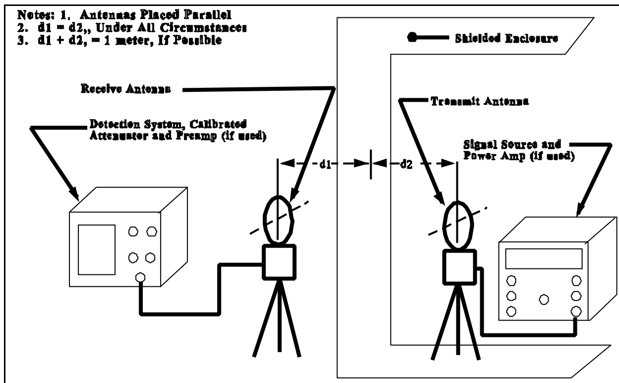
Figure 3 – Test Set-up for Magnetic Field Measurements
