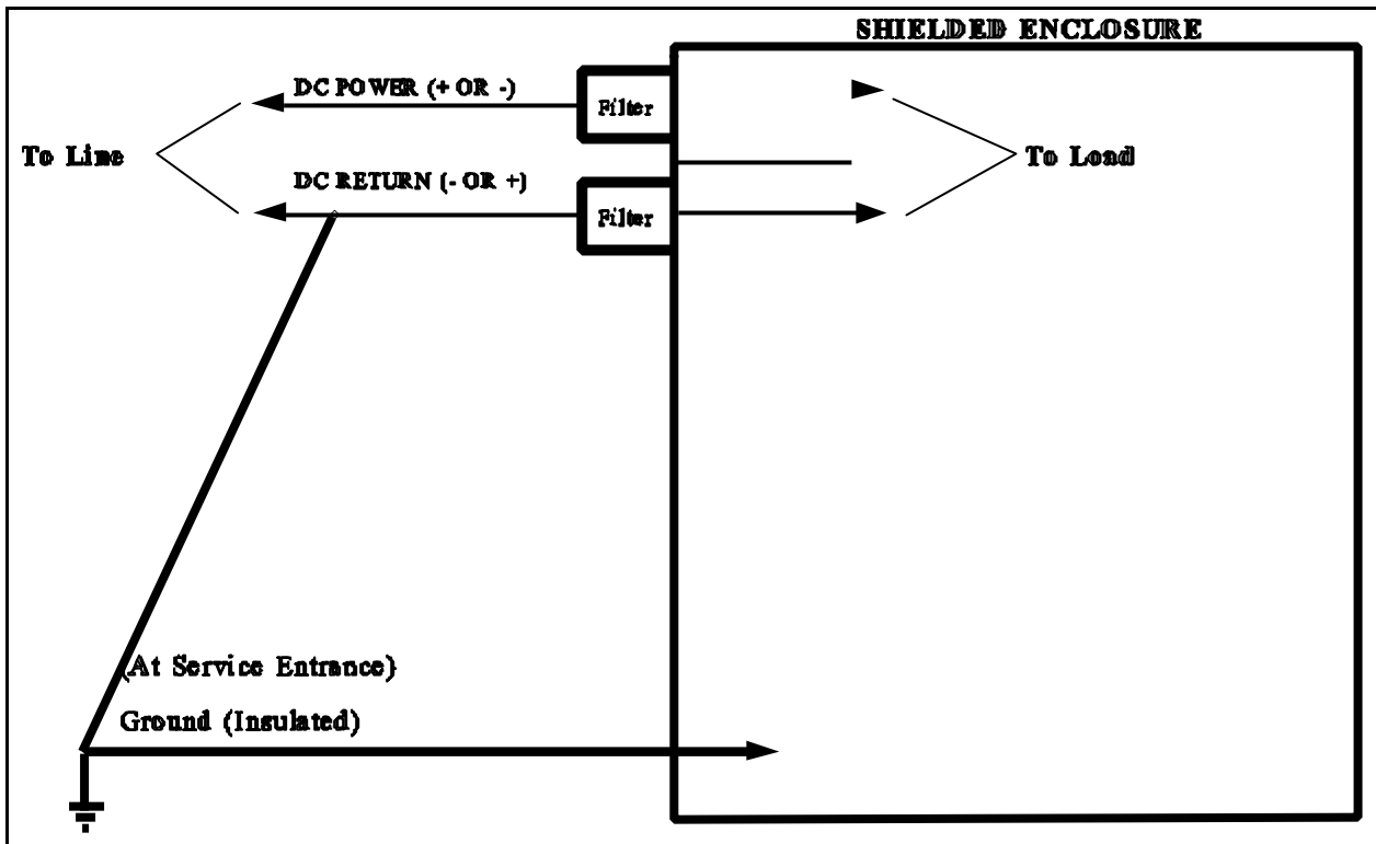
Figure 14 – Typical Power Line Configuration for DC Power
