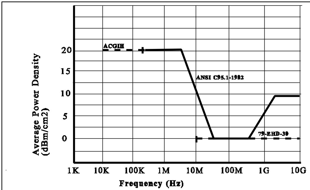
Figure 1 – Guidelines for Personnel Exposure to Electromagnetic Radiation
