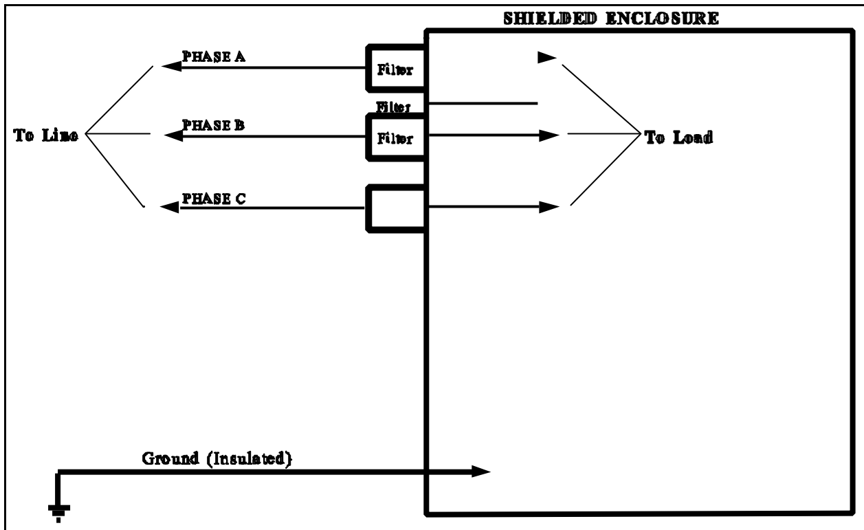
Figure 13 – Typical Power Line Configuration for 3 Phase, Delta
