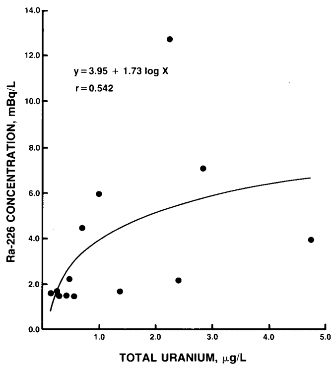
Figure A-1. Relationship of total uranium and Ra-226 concentrations in surface waters (13 sampling stations).
