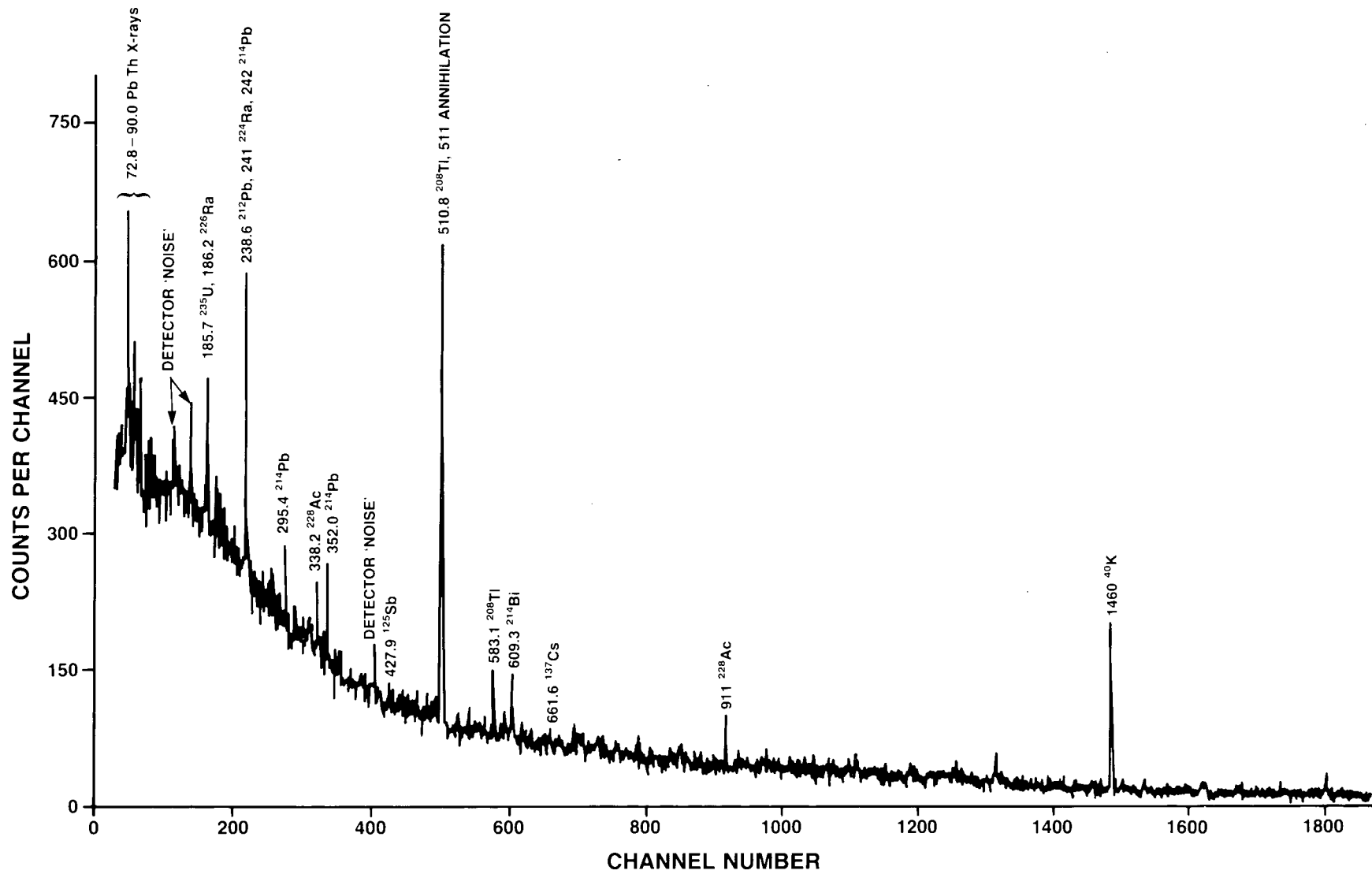
Figure 4. Gamma-ray spectrum of a 1984 Niagara River water sample showing prominent photopeaks with their energies (keV).
