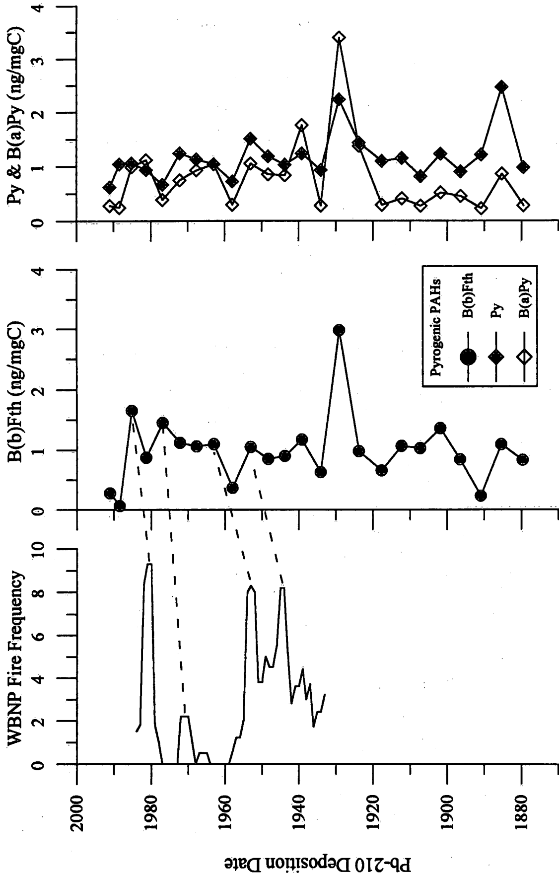
Figure 35: Pyrogenic PAHs Related to WBNP Fire Frequency. Normalized to TOC, the peaks in these three PAHs relate well to a reconstructed forest fire frequency curve for WBNP after the data from Larsen (1989). Dashed lines indicate speculative correlations assuming a lag in arrival of PAHs to the sediments.
