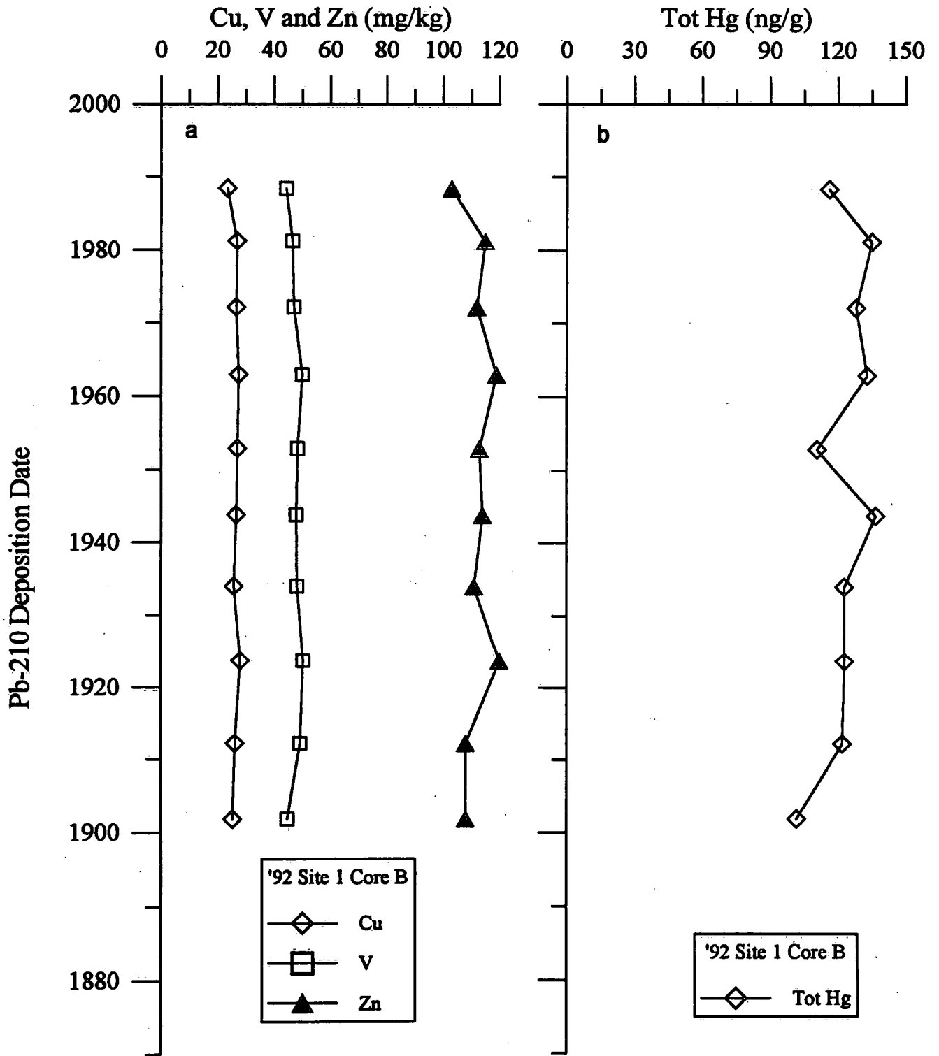
Figure 39: Copper, Vanadium, Zinc and Total Mercury in 1992 Site 1 Core B.
