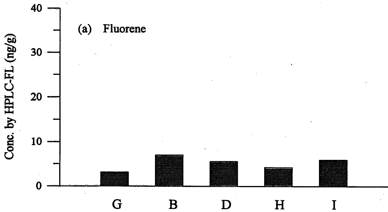
Figure 13: Fl, Fth and B(ghi)Per in 1992 Surficial Samples.
