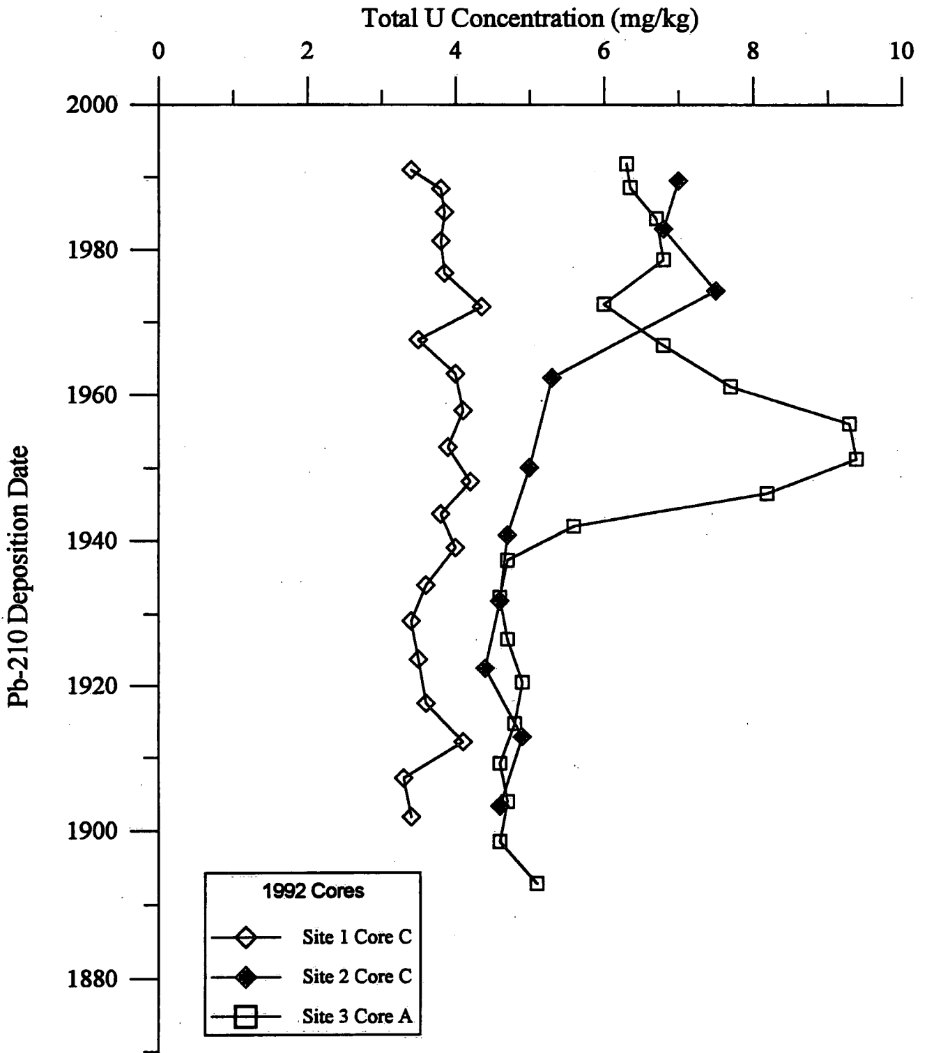
Figure 28: Total Uranium Distribution in Cores from Three Sites - 1992.
