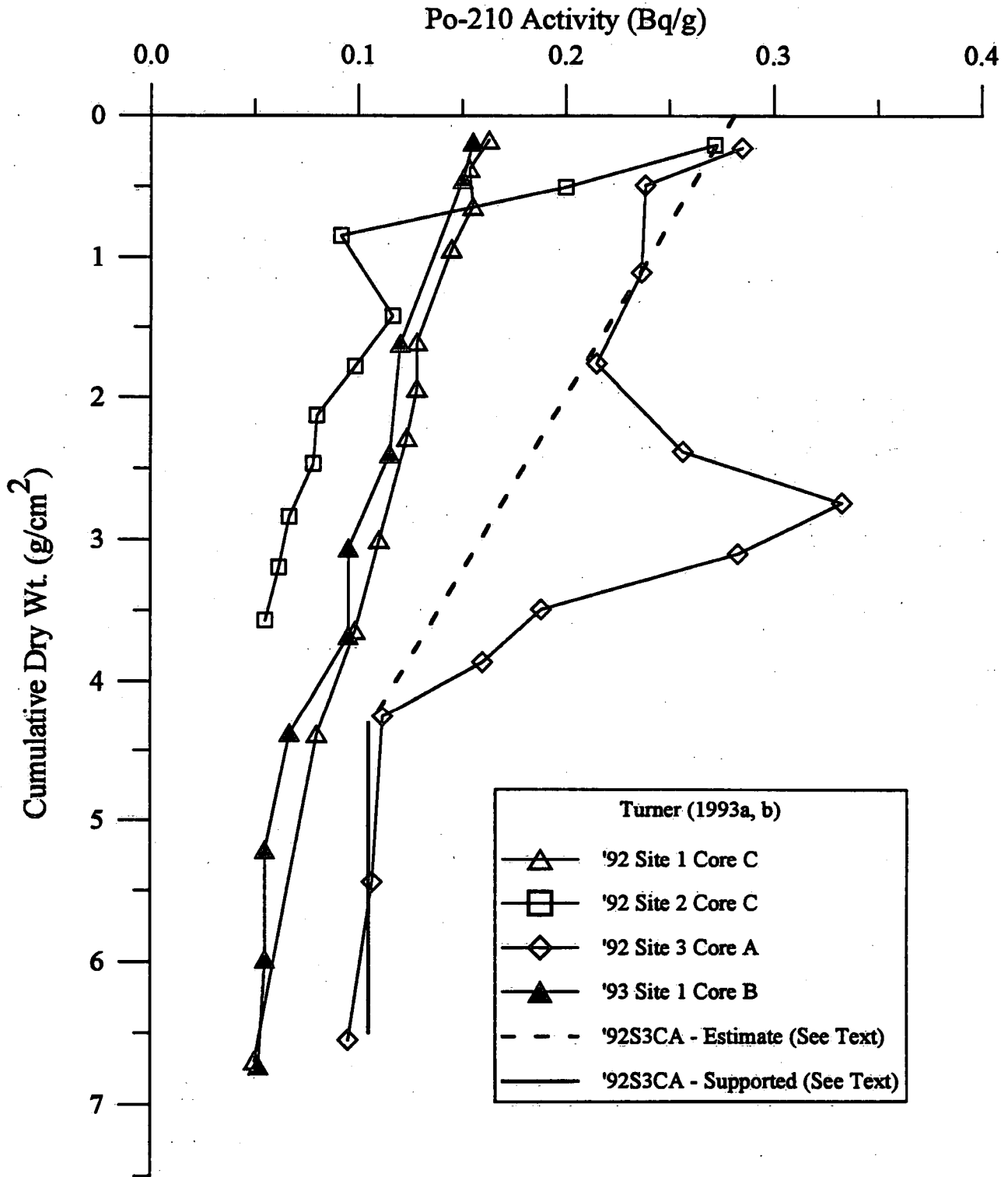
Figure 18: Po-210 Activities, Turner Data. Activity of Po-210 plotted against cumulative dry weight. All cores determined as part of the Pb-210 dating method. See text for discussion of regression lines.
