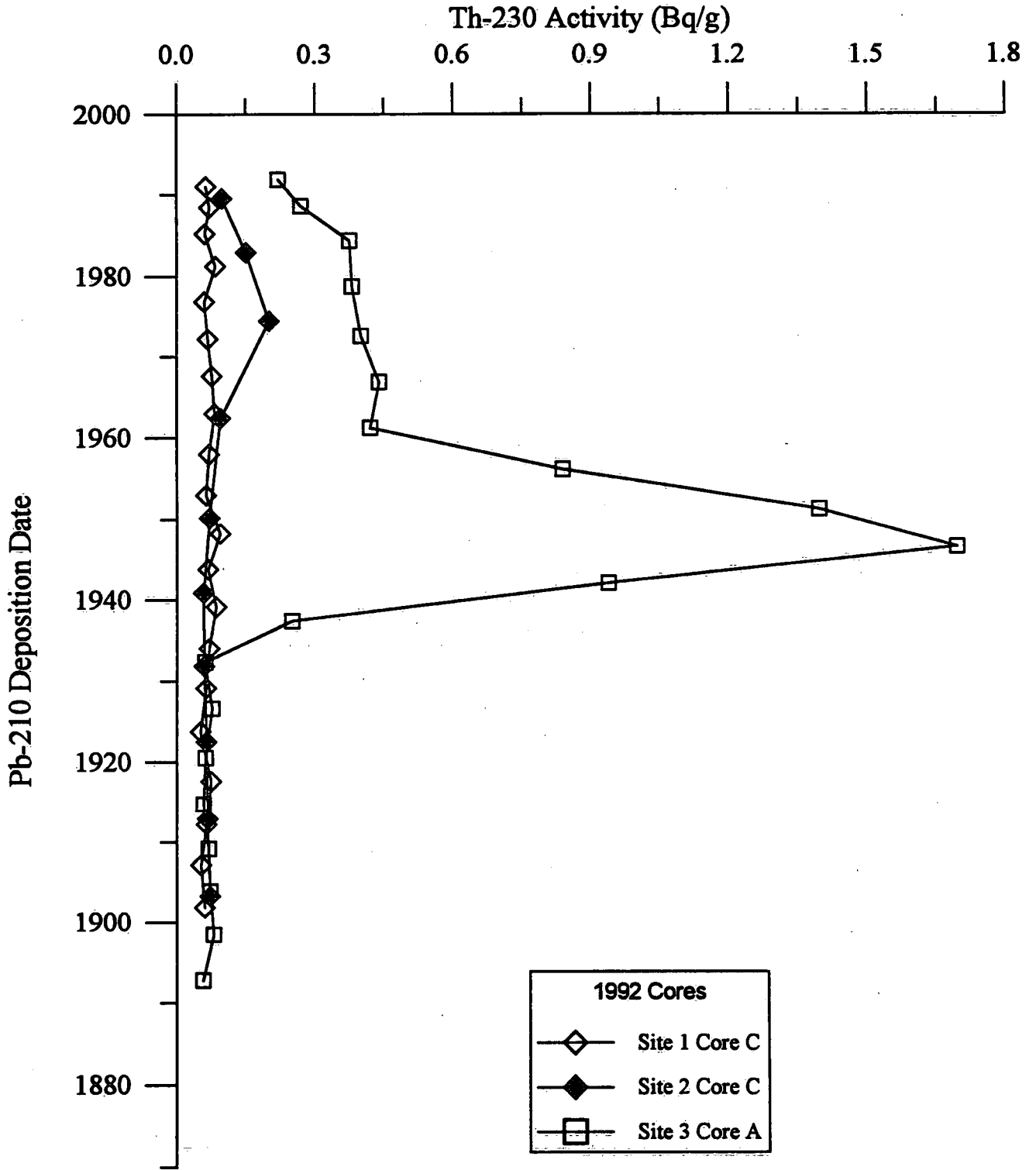
Figure 27: Thorium-230 Distribution in Cores from Three Sites - 1992.
