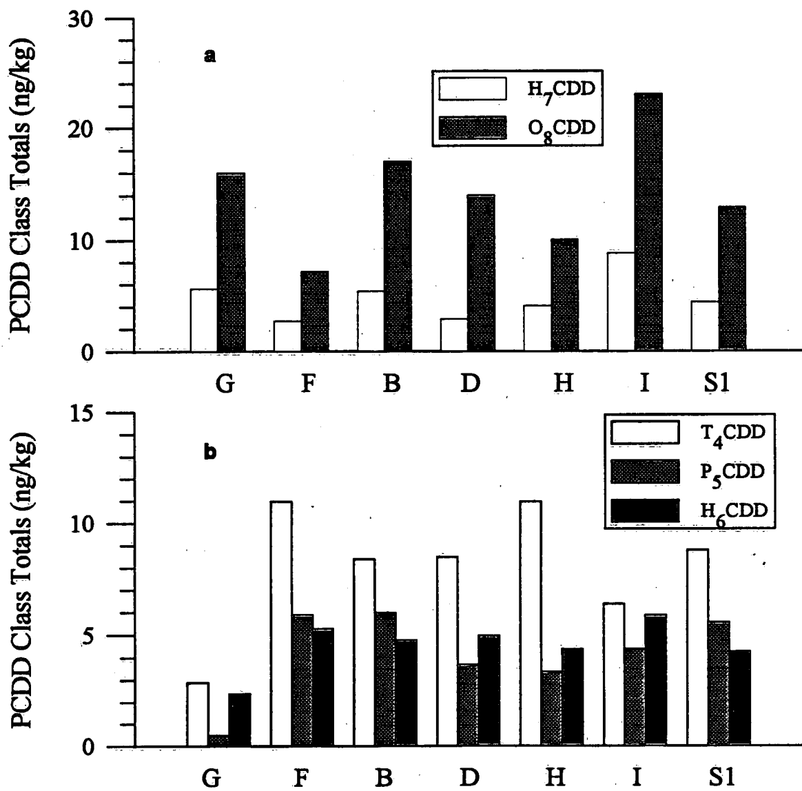
Figure 4: Totals of PCDD classes for 1992 Surficial Sediments.
