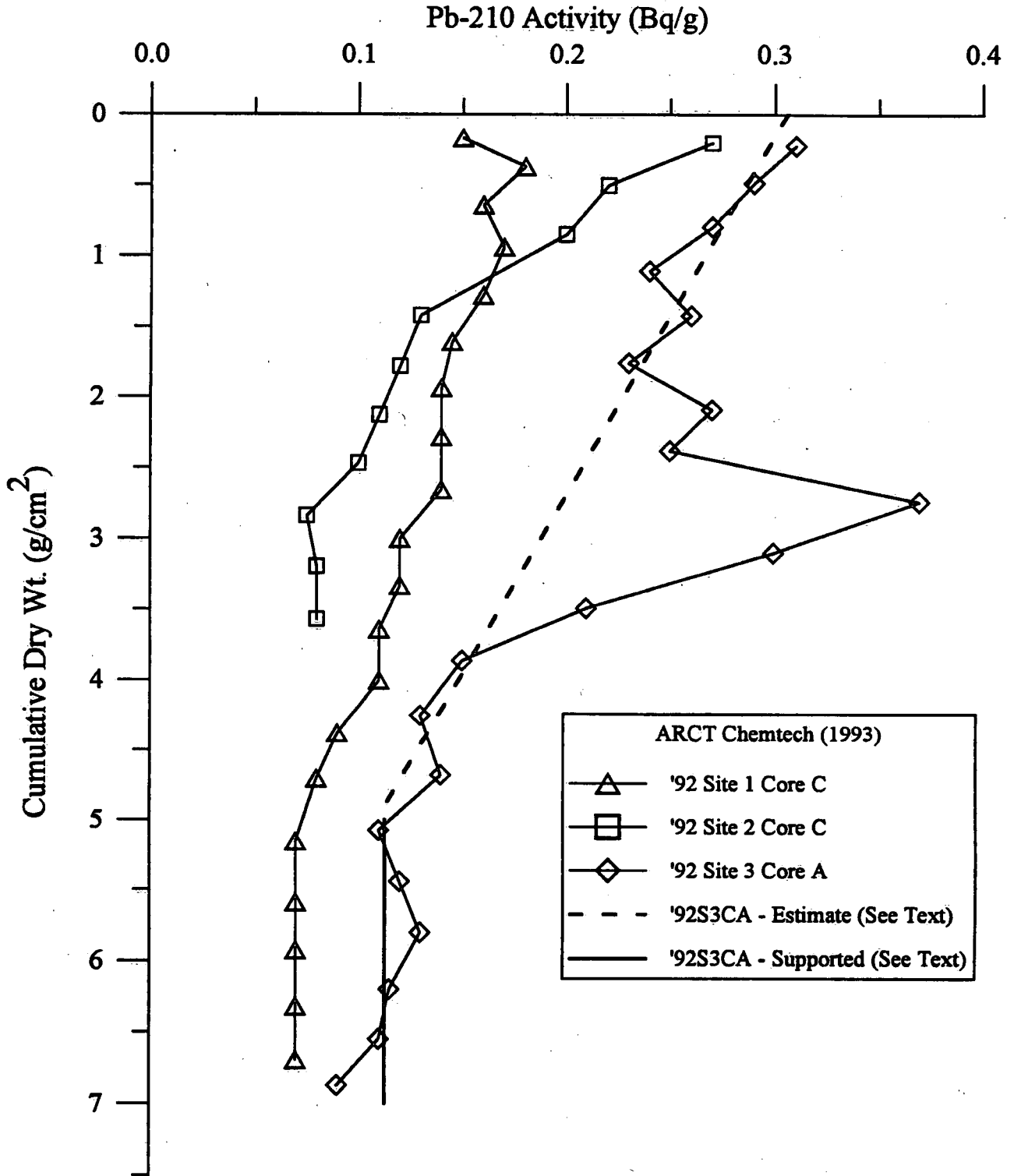
Figure 19: Pb-210 Activities, ARCT Chemtech Data. Activity of Pb-210 plotted against cumulative dry weight. All cores determined by direct gamma counting. See text for discussion of regression line.
