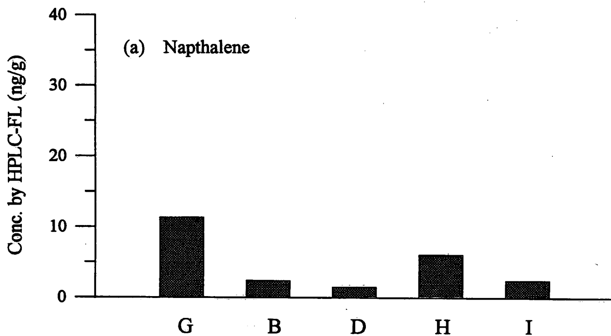
Figure 11: Naph, 1-MeNpth and 2-MeNpth in 1992 Surficial Samples.
