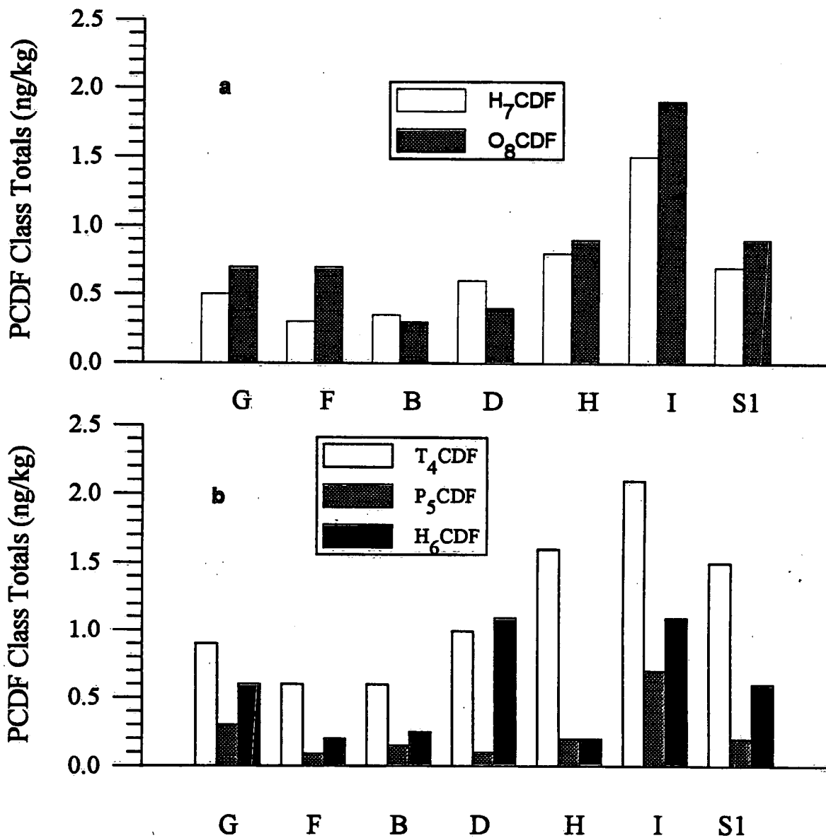
Figure 5: Totals of PCDF Classes for 1992 Surficial Sediments.
