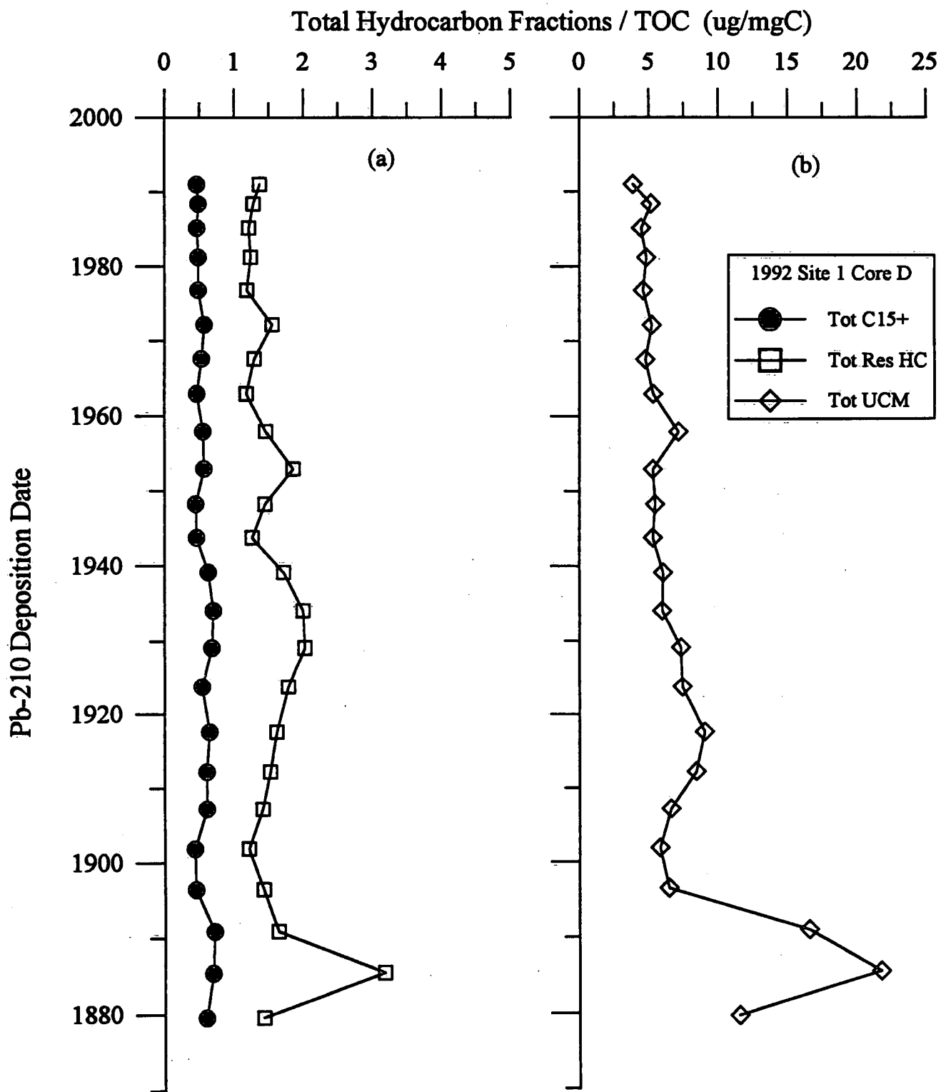
Figure 41: Total Hydrocarbon Fractions Normalized to TOC - 1992 Site 1 Core D. Values from GLC-FID, TOC data reported in Section 5.2 (92 S1 CC).
