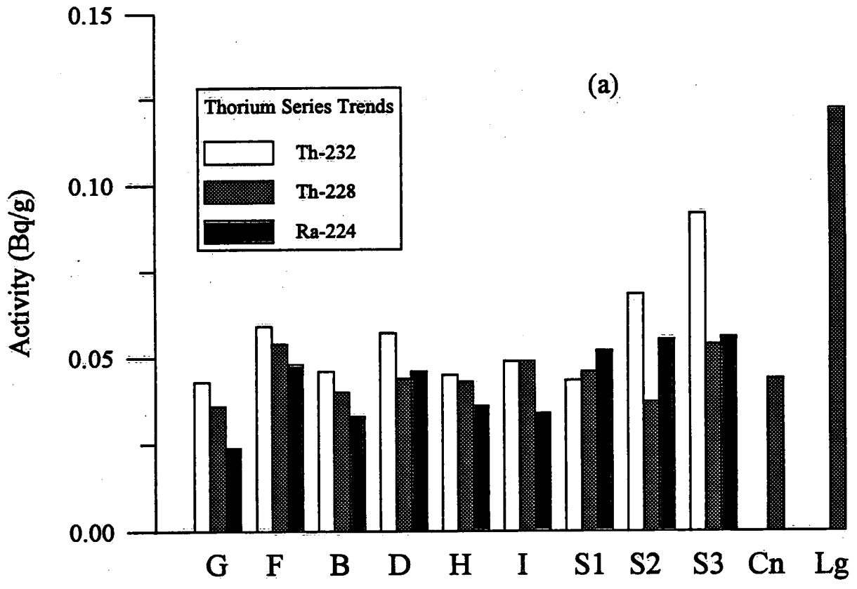
Figure 2: Thorium and Uranium Series Radionuclides - Surficial Sediments 1992.
