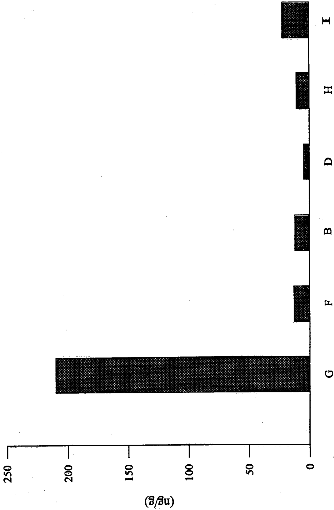
Figure 8: Dehydroabietic Acid (DHA) Concentrations in 1992 Surficial Sediment.
