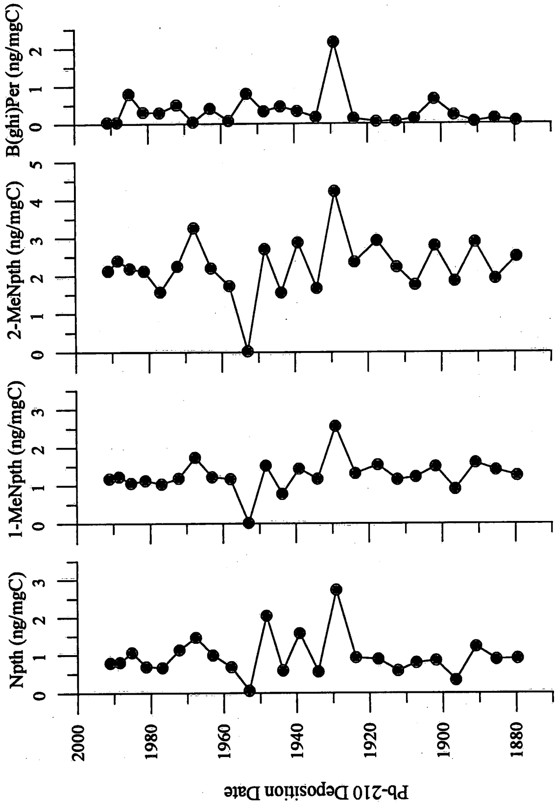
Figure 32: Site 1 TOC Normalized PAH Data - Npth, 1-MeNpth, 2-Npth and B(ghi)Per. Fluorescence HPLC data only are shown. Values from Table 13 are divided by TOC (Section 5.2).
