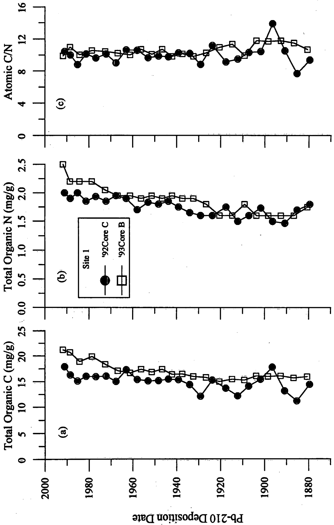
Figure 24: Site 1 Organic Carbon & Nitrogen. Concentrations of total organic C, total "organic" N and atomic C/N ratio for cores taken in 1992 and 1993. Values are plotted against deposition date determined for each core by the Pb-210 method.
