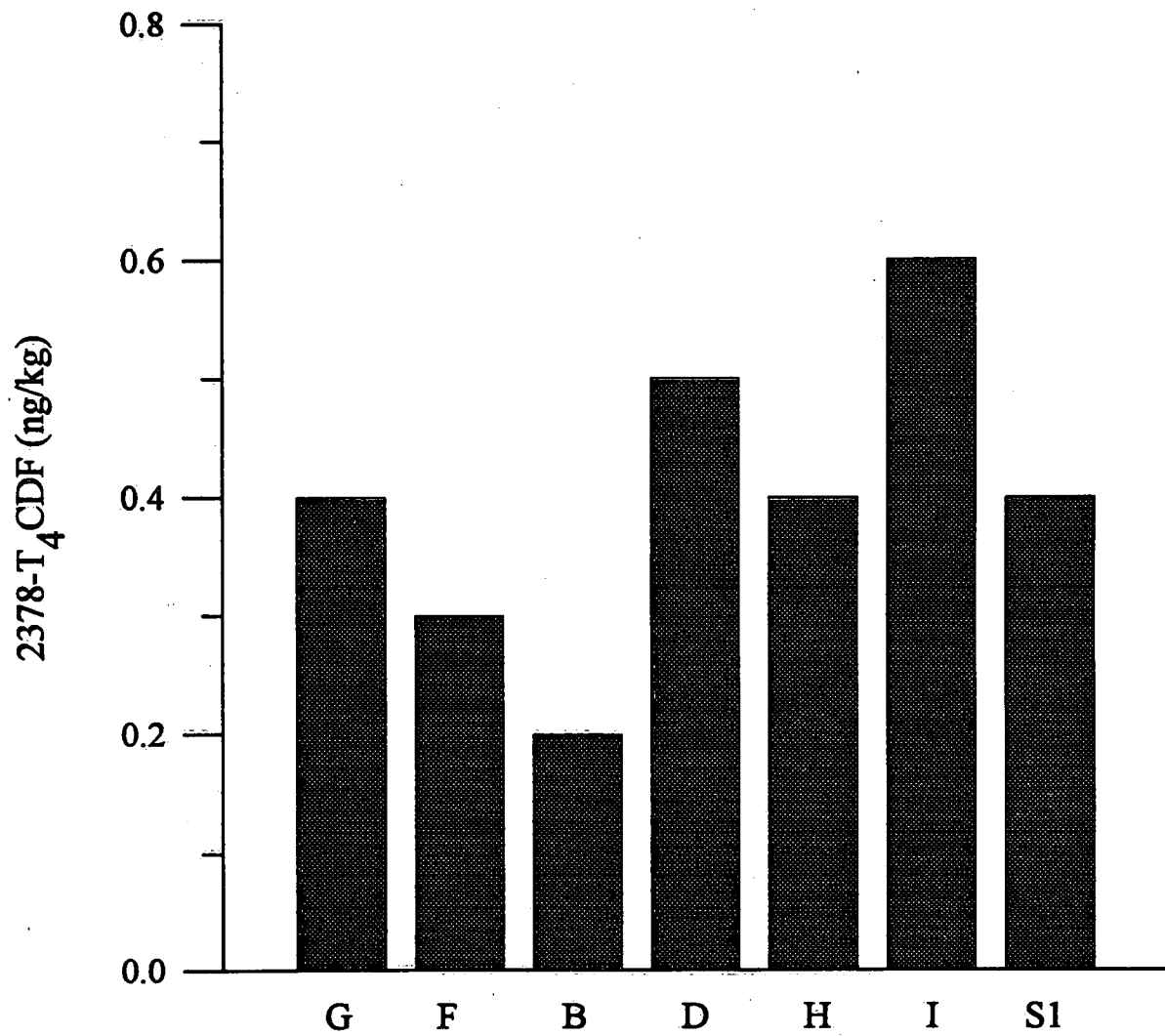
Figure 6: ^{2378}\text{-T}_4\text{CDF} Concentrations in 1992 Surficial Sediments
