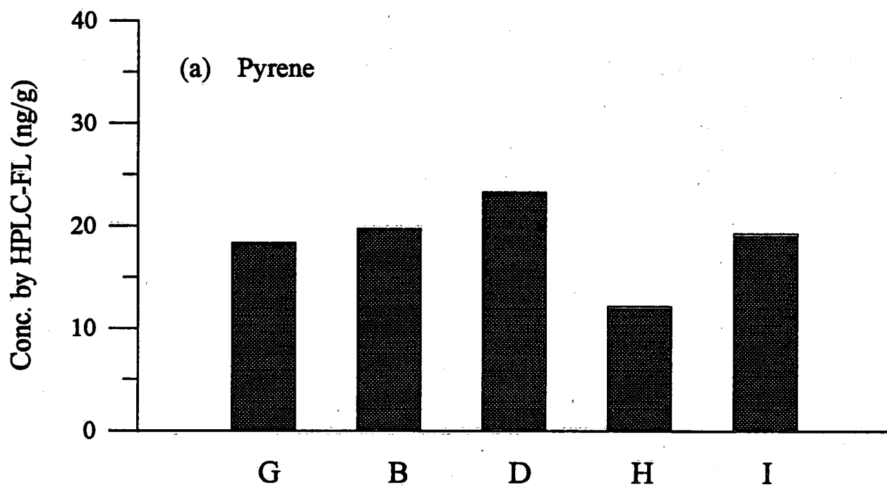
Figure 12: Py, B(b)Fth and B(a)Py in 1992 Surficial Samples.
