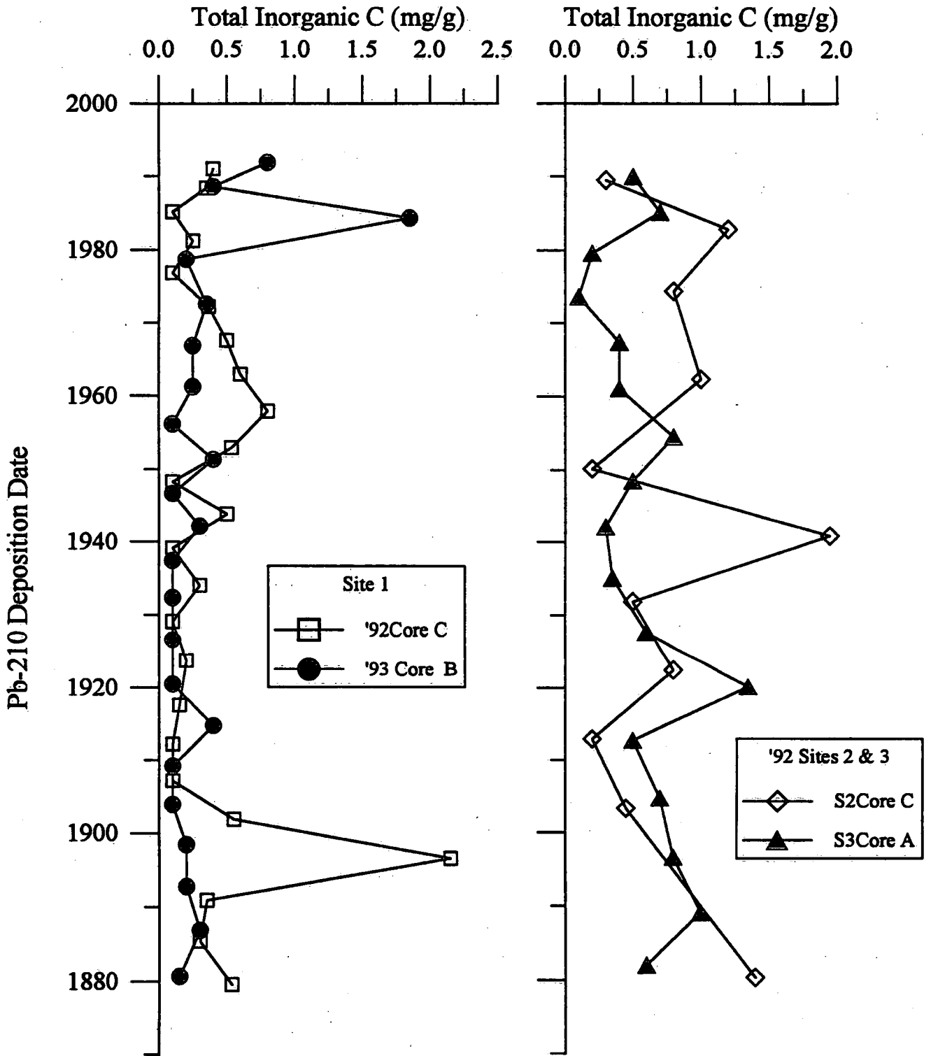
Figure 23: Inorganic Carbon, All Sites. Concentrations of TIC for '92 and '93 cores. Values are plotted against Pb-210 deposition date, see Section 5.1. For non-detectable values, the MDL was plotted (see Table 10).
