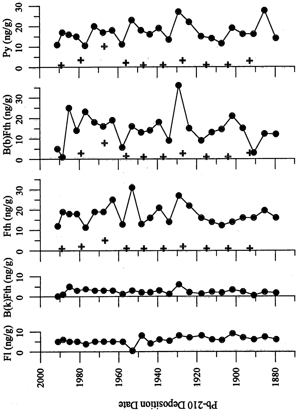
Figure 30: Site 1 PAH Data - Fl, B(k)Fth, Fth, B(b)Fth and Py. Fluorescence HPLC data shown by solid circles and GCMS data by crosses. SDLs are plotted whenever an ND occurred, as are "tr" values, see Tables 13 and 14.
