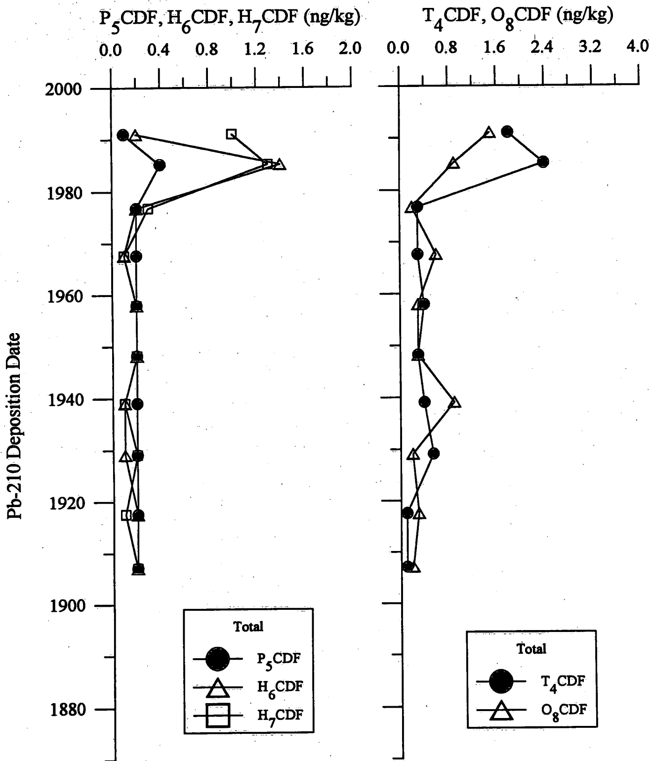
Figure 37: Distribution of PCDF Class Totals - 1992 Site 1 Core B.
