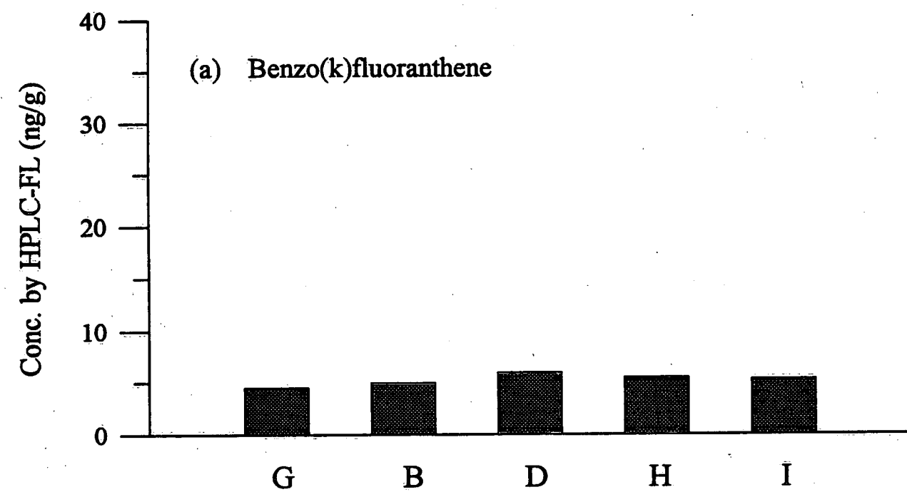
Figure 14: B(k)Fth and Ph in 1992 Surficial Samples.
