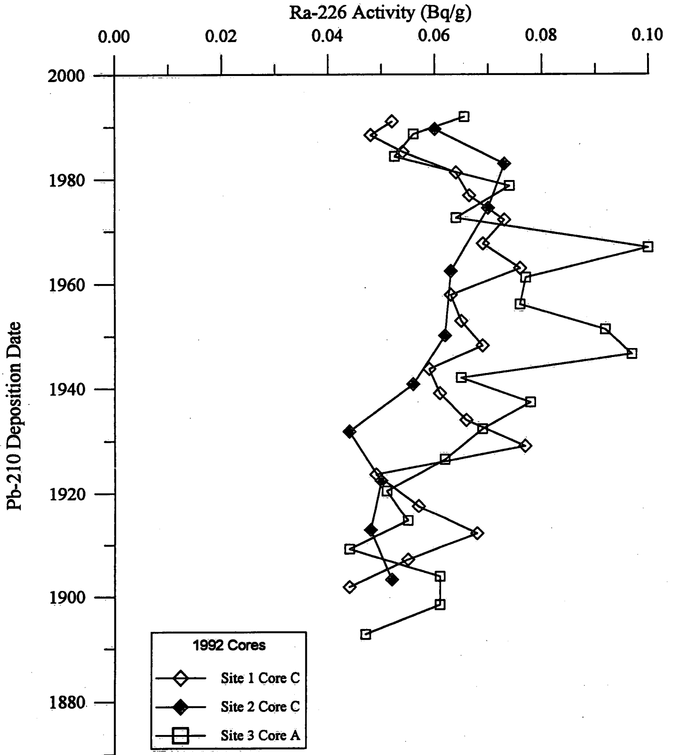
Figure 26: Radium-226 Distribution in Cores from Three Sites - 1992.
