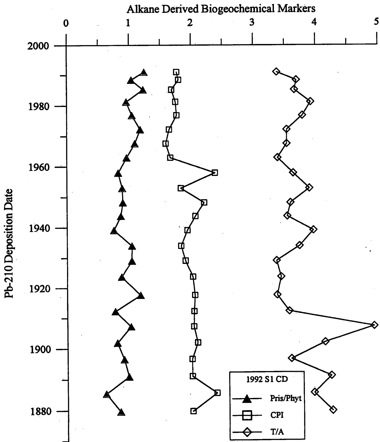
Figure 42: Alkane Derived Biogeochemical Markers for 1992 Site 1 Core D. Ratios derived from individual n-alkane concentrations from GLC-FID runs, no blank corrections necessary.
