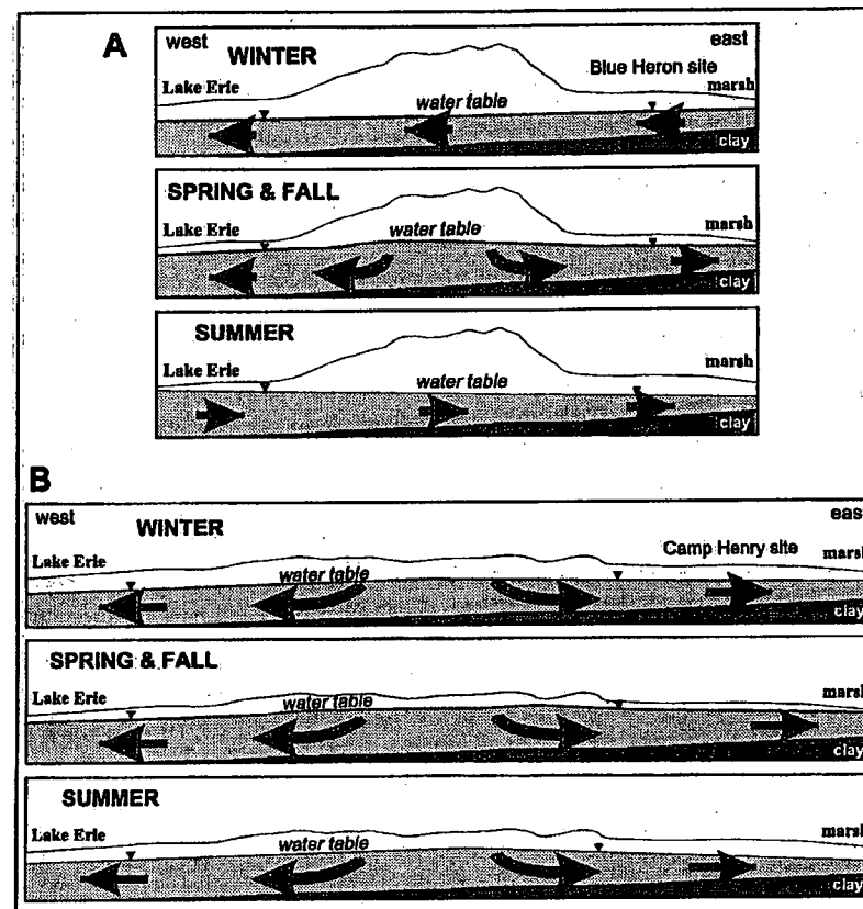
Figure 2: Conceptual model of seasonal changes in the direction of groundwater flow at (A) the northern part of Point Pelee (e.g., Northwest Beach/Blue Heron area), and (B) the southern portion of Point Pelee (e.g., Camp Henry site).
