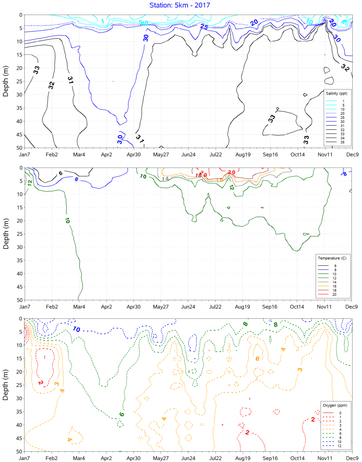
Figure 90. Station 5KM, 2017. Annual flux in mean Salinity (top), Temperature (middle), and Dissolved Oxygen (bottom) at depth.
