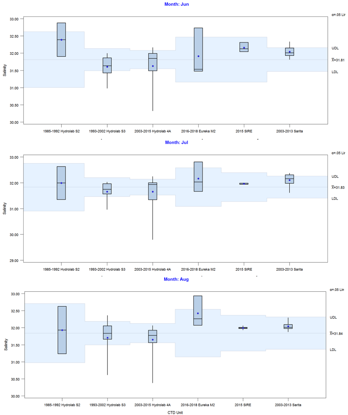
Figure 97. Analysis of mean sub-halocline salinity (depth 30 m) for CTD units after adjustments to Hydrolab Surveyor 3 and Hydrolab 4A salinity readings indicating no significant differences between monthly means.
