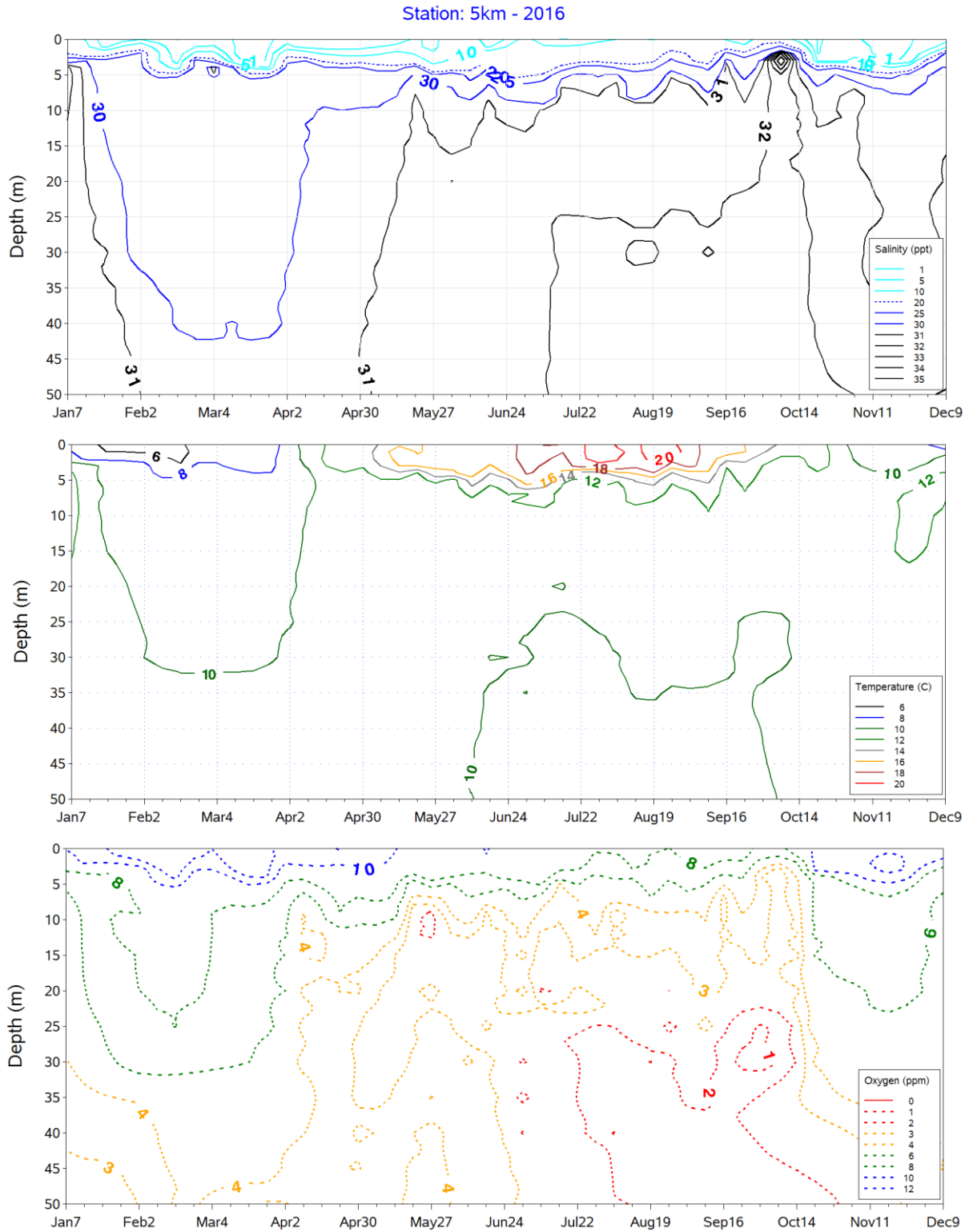
Figure 89. Station 5KM, 2016. Annual flux in mean Salinity (top), Temperature (middle), and Dissolved Oxygen (bottom) at depth.
