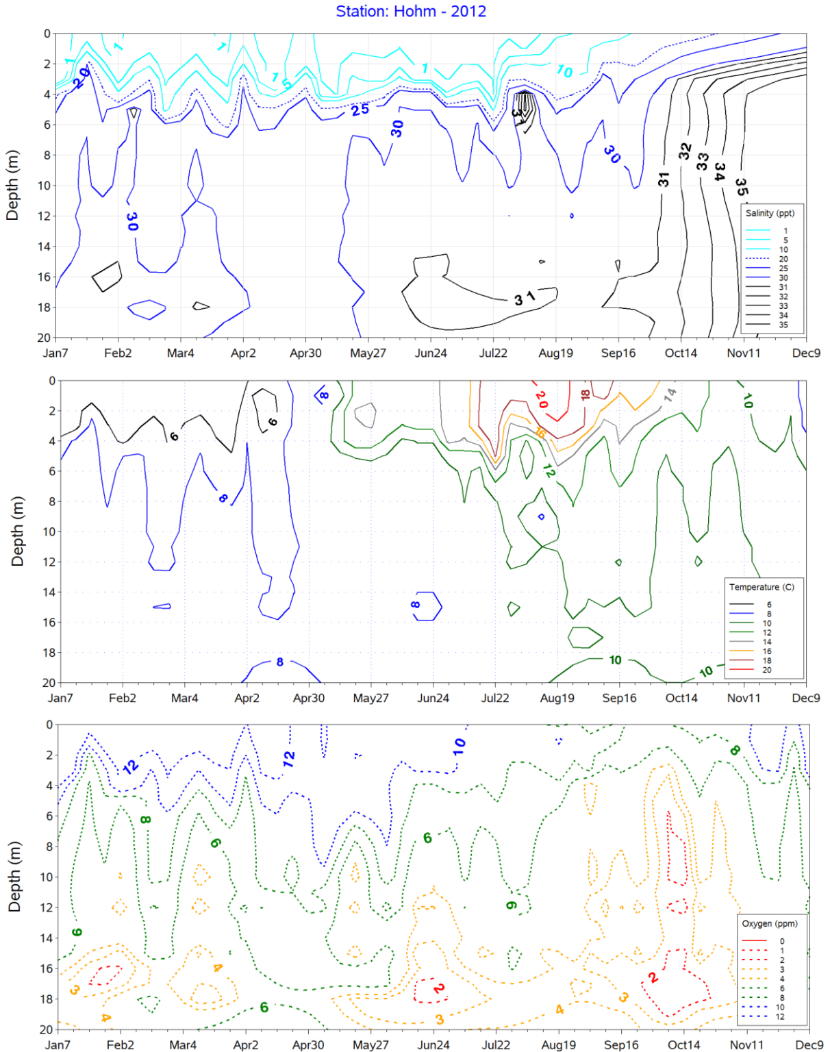
Figure 56. Hohm Station, 2012. Annual flux in mean Salinity (top), Temperature (middle), and Dissolved Oxygen (bottom) at depth.
