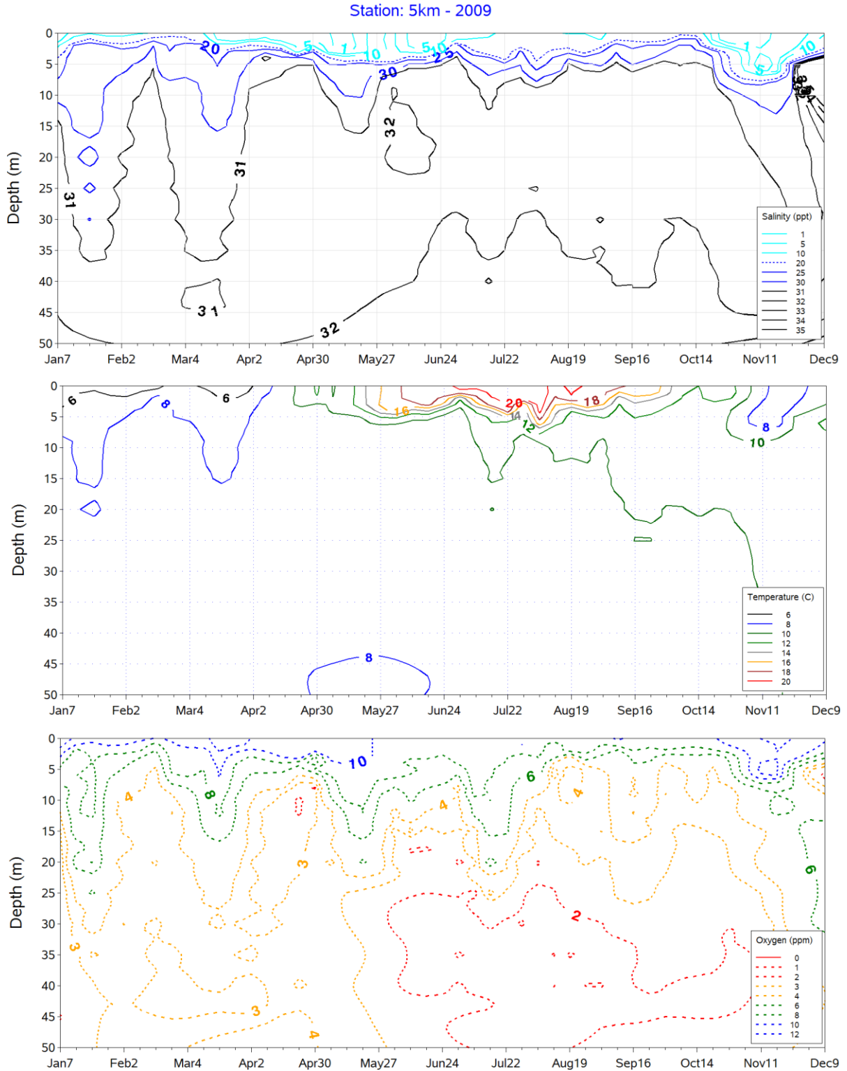
Figure 82. Station 5KM, 2009. Annual flux in mean Salinity (top), Temperature (middle), and Dissolved Oxygen (bottom) at depth.
