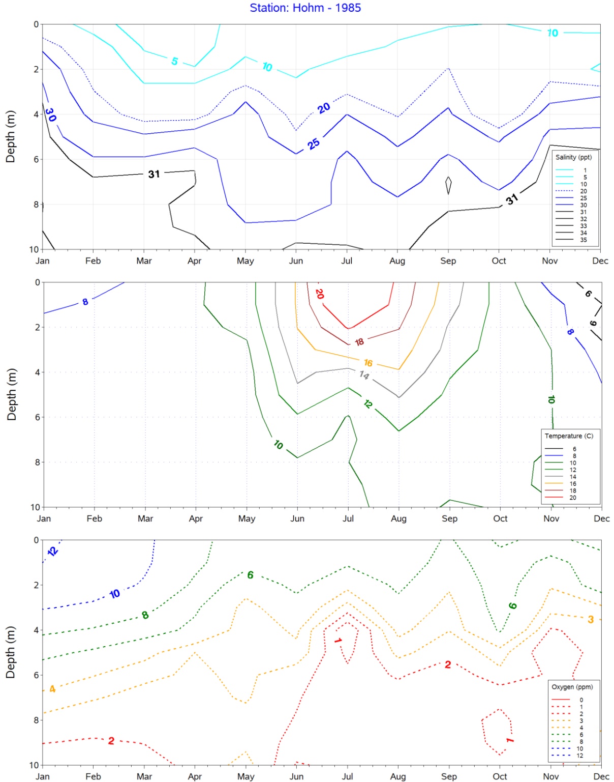
Figure 30. Hohm Station, 1985. Annual flux in mean Salinity (top), Temperature (middle), and Dissolved Oxygen (bottom) at depth.
