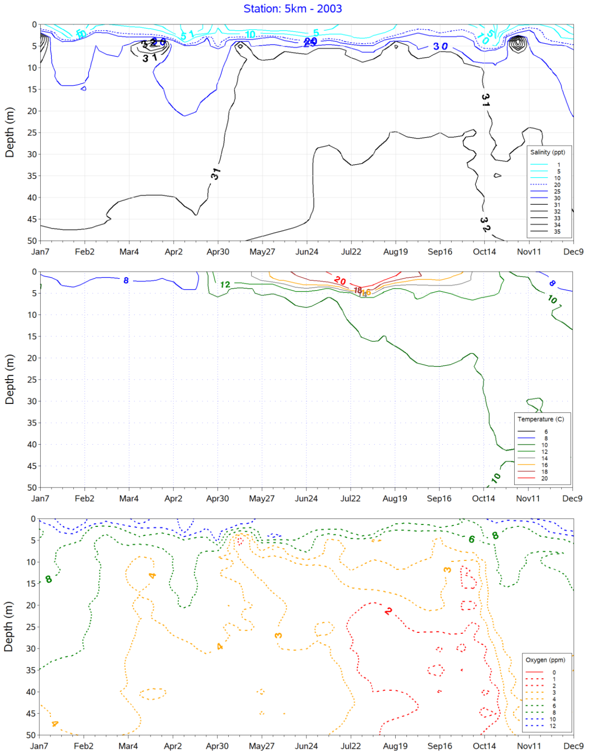
Figure 76. Station 5KM, 2003. Annual flux in mean Salinity (top), Temperature (middle), and Dissolved Oxygen (bottom) at depth.
