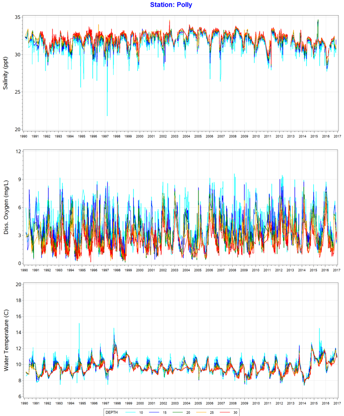
Figure 10. Salinity (top), DO (middle) and Temperature (bottom) at depth at Polly Point (PP-2) Station, 1990-2017.
