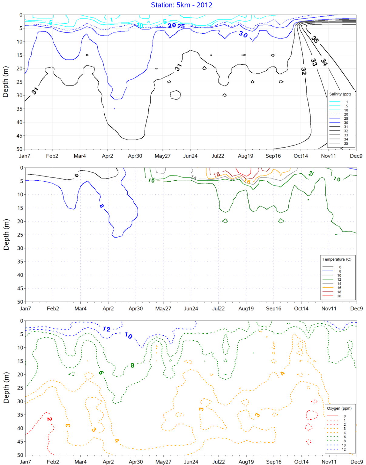
Figure 85. Station 5KM, 2012. Annual flux in mean Salinity (top), Temperature (middle), and Dissolved Oxygen (bottom) at depth.
