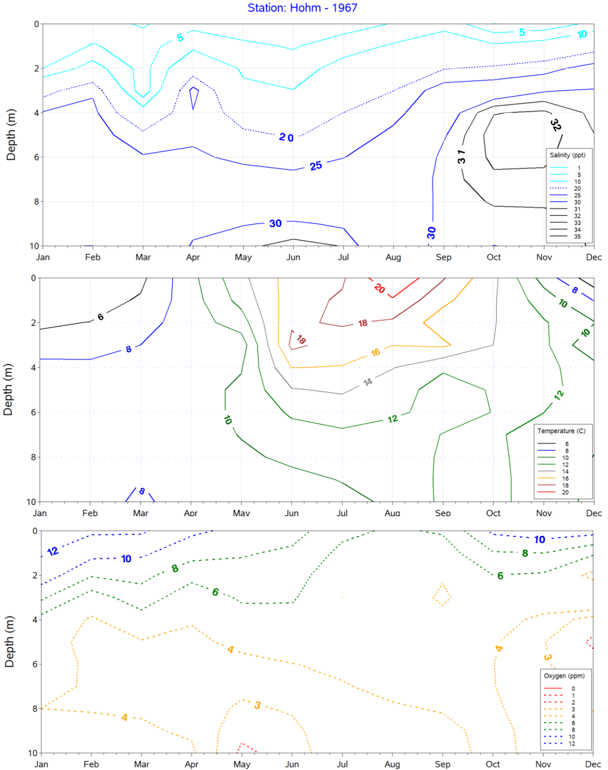
Figure 22. Hohm Station, 1967. Annual flux in mean Salinity (top), Temperature (middle), and Dissolved Oxygen (bottom) at depth.
