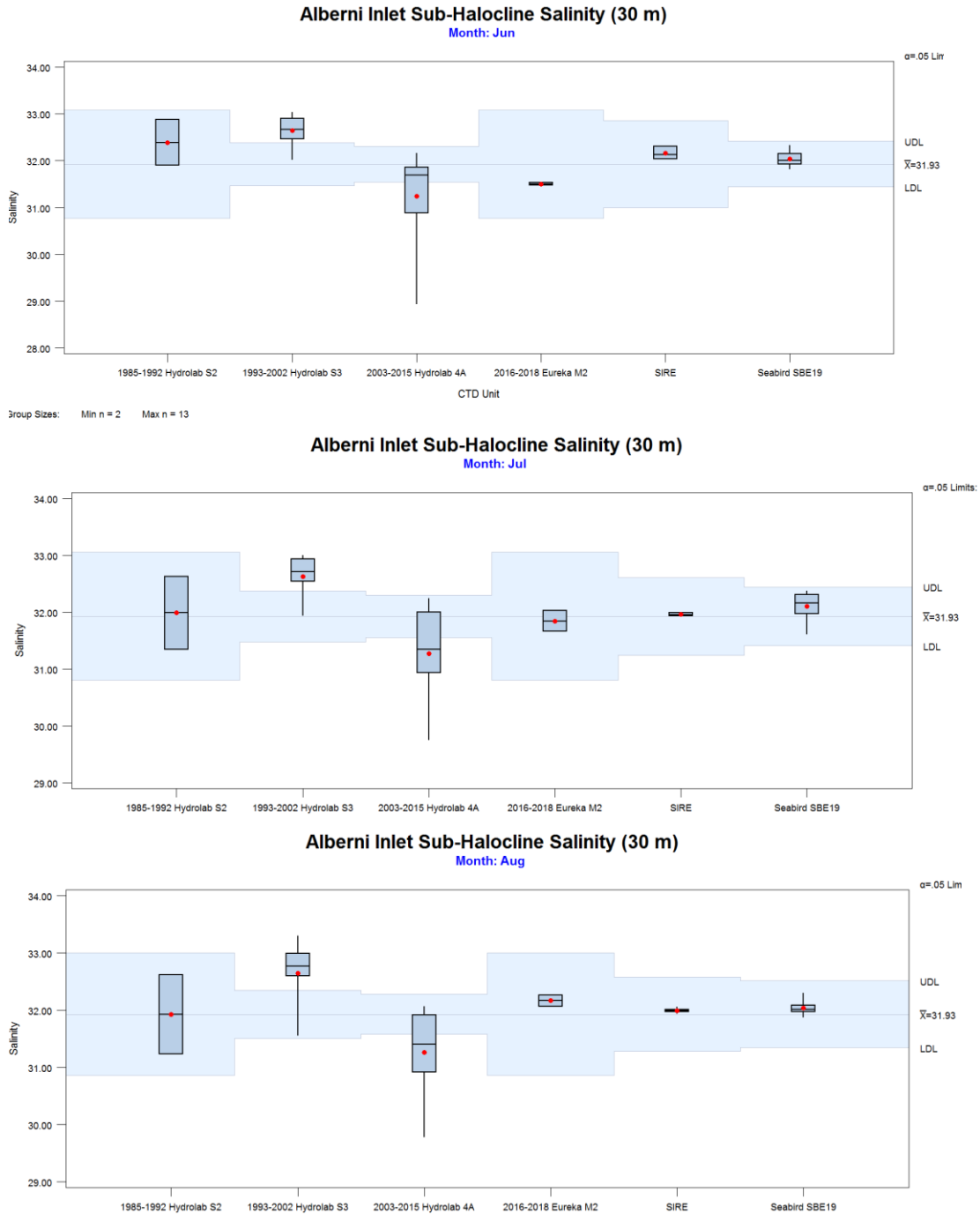
Figure 93. Salinity readings for most months associated with CTD units Hydrolab Surveyor 3 appear to be biased high (1993-2002), and Hydrolab Surveyor 4A appear to be biased low for some years (2009-2015), relative to other DOMP CTD units, including independent data (Seabird SBE19) spanning 2004-2013, and DFO SIRE data surveyed in 2015.
