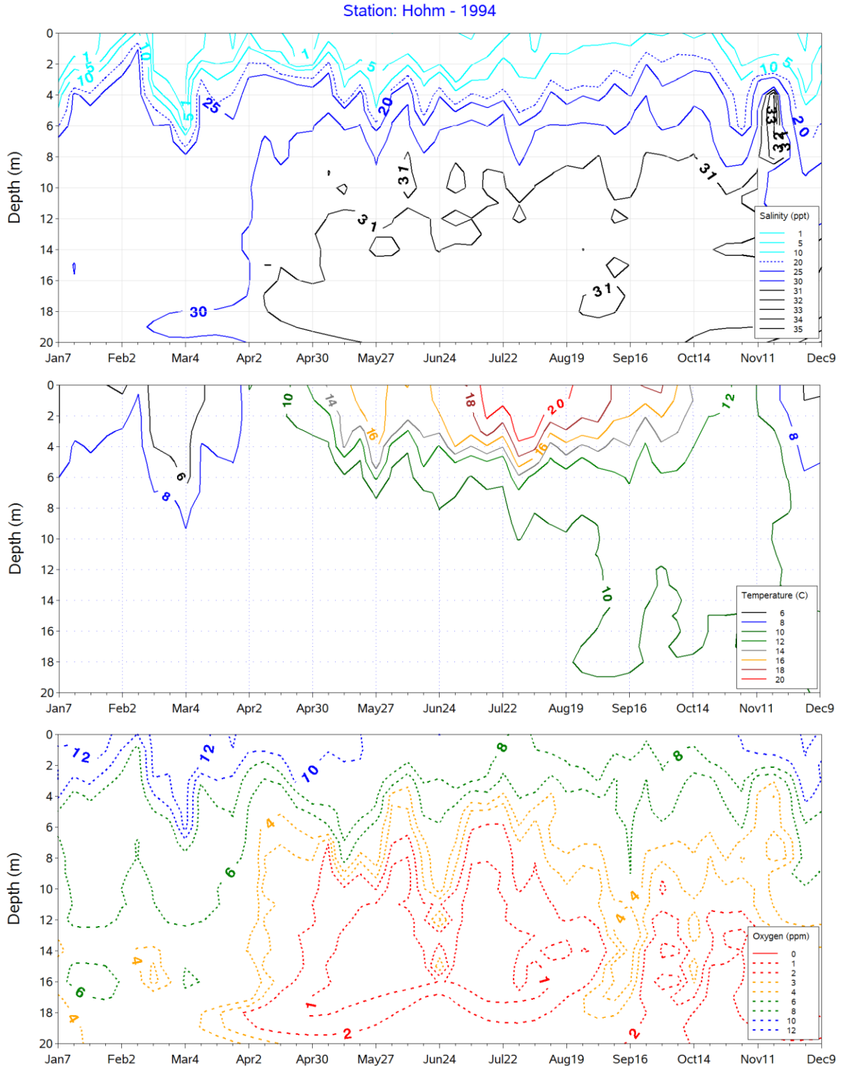
Figure 38. Hohm Station, 1994. Annual flux in mean Salinity (top), Temperature (middle), and Dissolved Oxygen (bottom) at depth.
