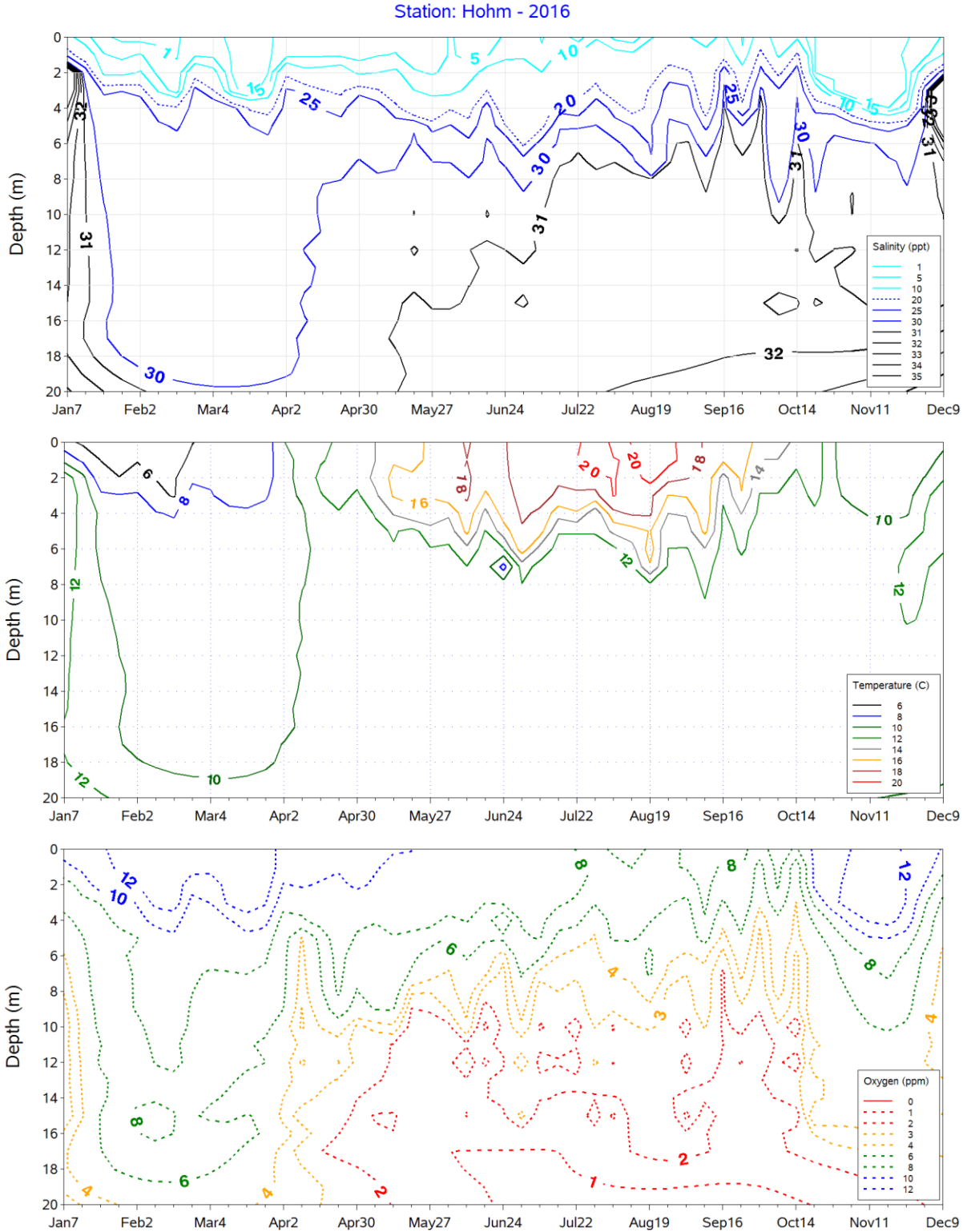
Figure 60. Hohm Station, 2016. Annual flux in mean Salinity (top), Temperature (middle), and Dissolved Oxygen (bottom) at depth.
