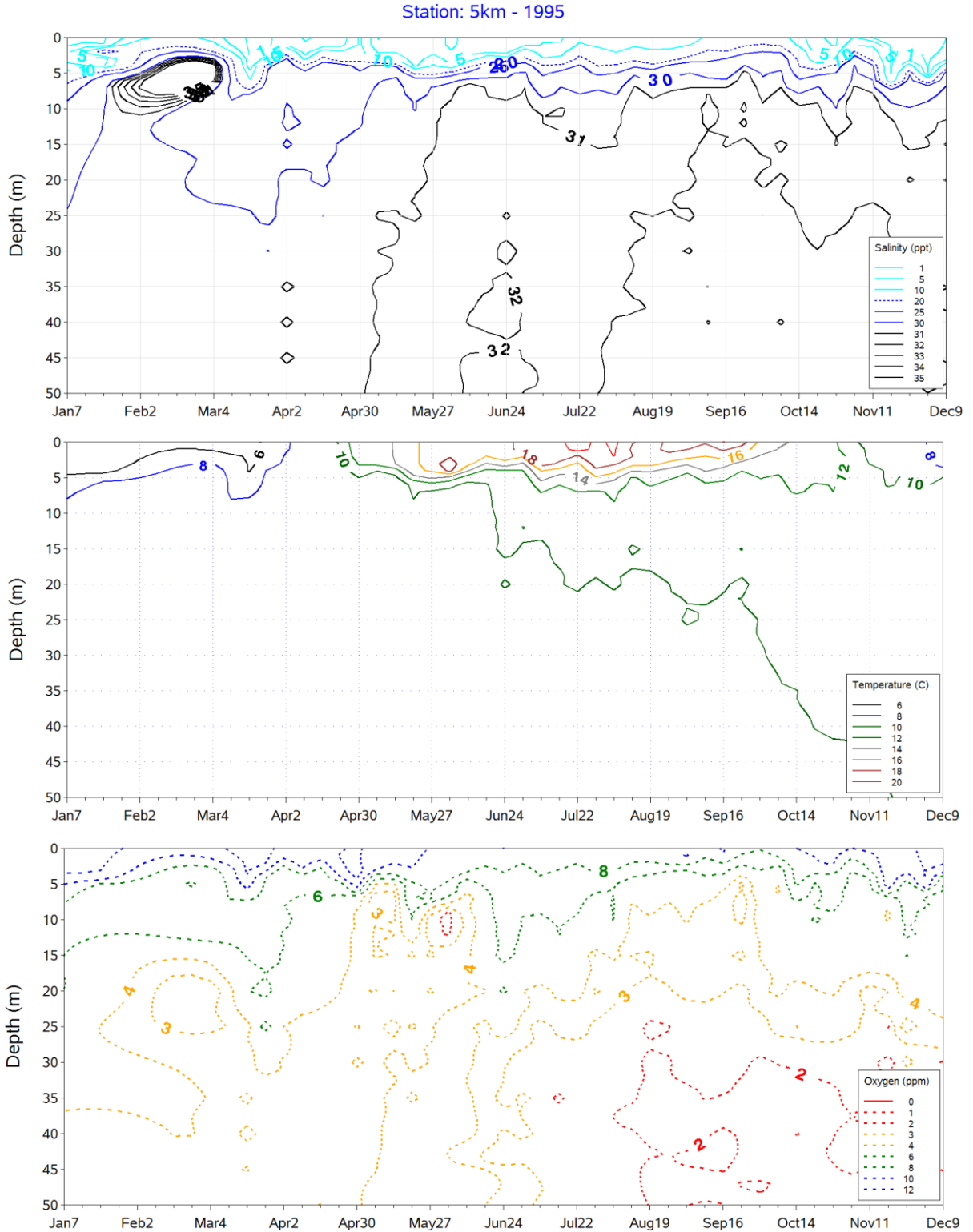
Figure 68. Station 5KM, 1995. Annual flux in mean Salinity (top), Temperature (middle), and Dissolved Oxygen (bottom) at depth.
