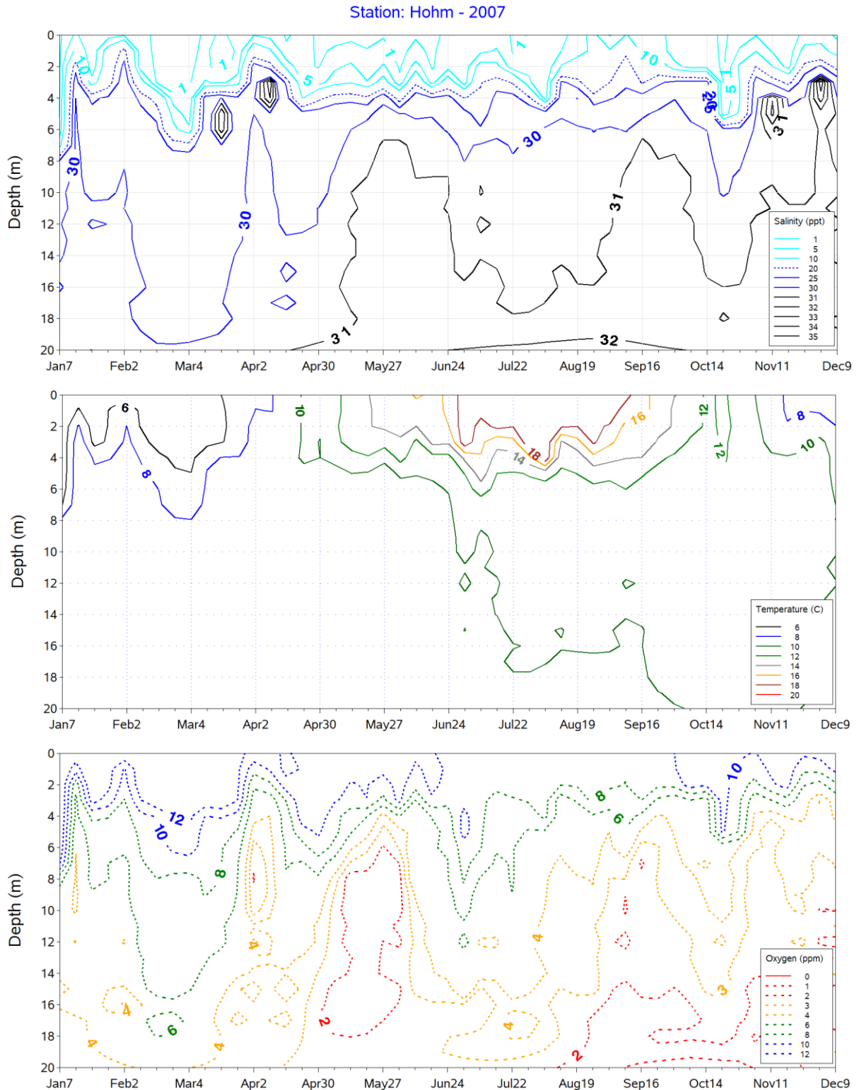
Figure 51. Hohm Station, 2007. Annual flux in mean Salinity (top), Temperature (middle), and Dissolved Oxygen (bottom) at depth.
