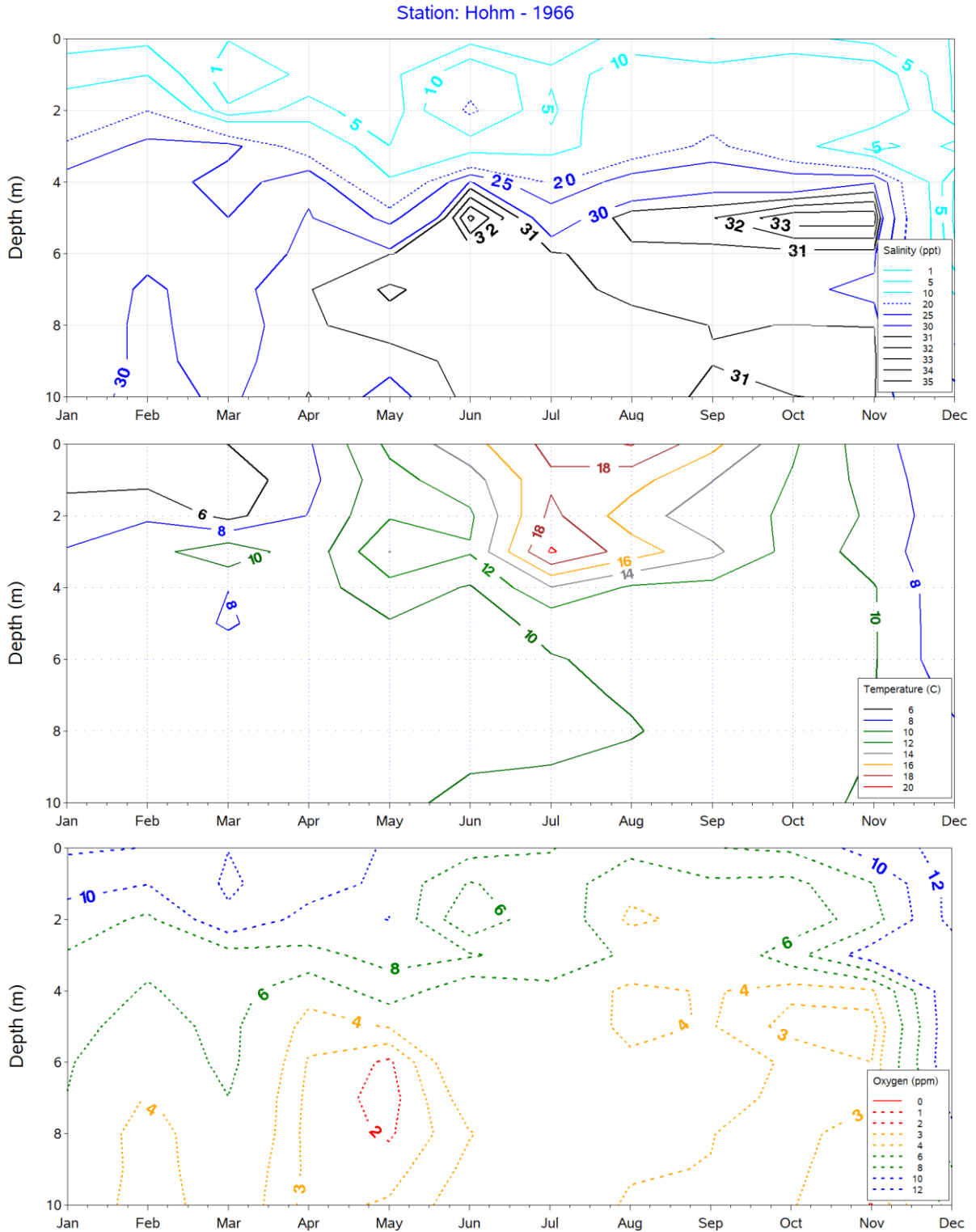
Figure 21. Hohm Station, 1966. Annual flux in mean Salinity (top), Temperature (middle), and Dissolved Oxygen (bottom) at depth.
