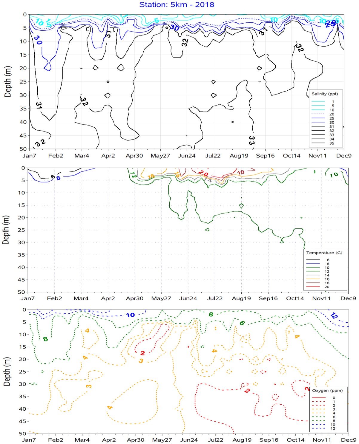
Figure 91. Station 5KM, 2018. Annual flux in mean Salinity (top), Temperature (middle), and Dissolved Oxygen (bottom) at depth.
