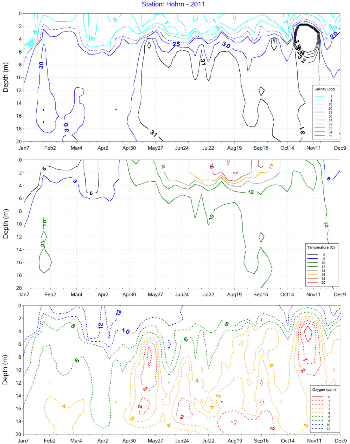
Figure 55. Hohm Station, 2011. Annual flux in mean Salinity (top), Temperature (middle), and Dissolved Oxygen (bottom) at depth.
