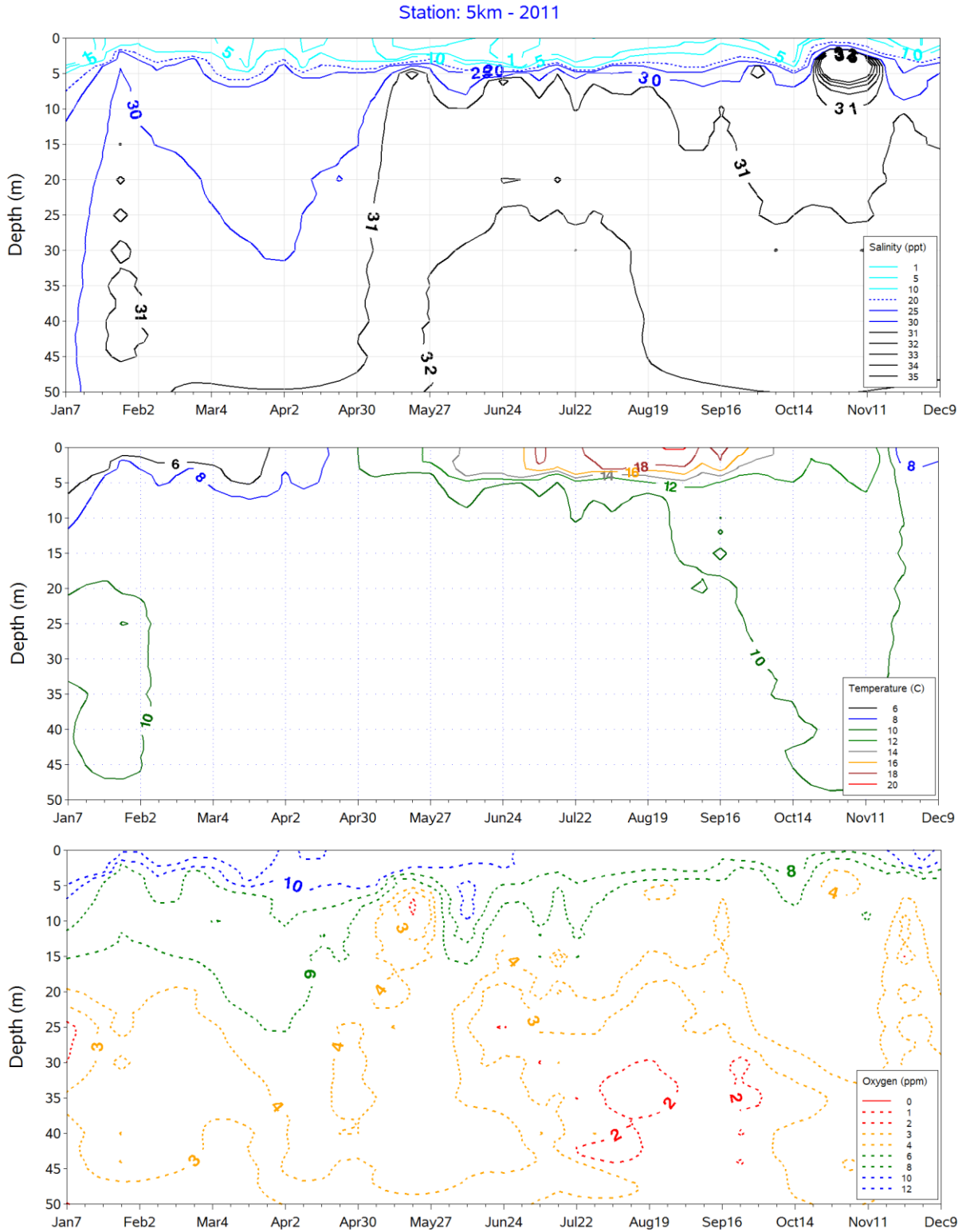
Figure 84. Station 5KM, 2011. Annual flux in mean Salinity (top), Temperature (middle), and Dissolved Oxygen (bottom) at depth.
