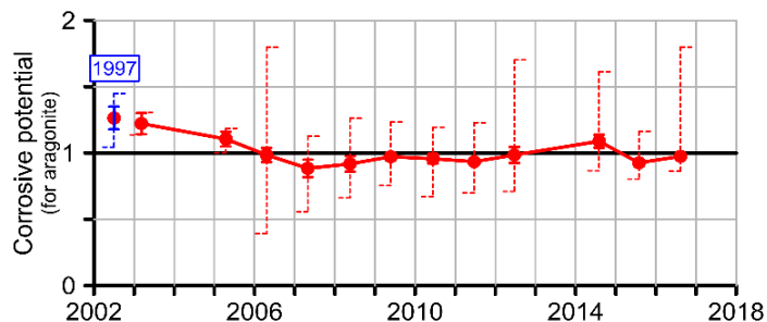
Figure 52. Values of an index \Omega in surface seawater of the Canada Basin. \Omega represents the corrosive effect of seawater on hard-shelled organisms, here for a limestone called aragonite. The threshold for damage is 1. Dashed lines span each year's range of variation across the basin. Unpublished data courtesy of Y. Zhang.
