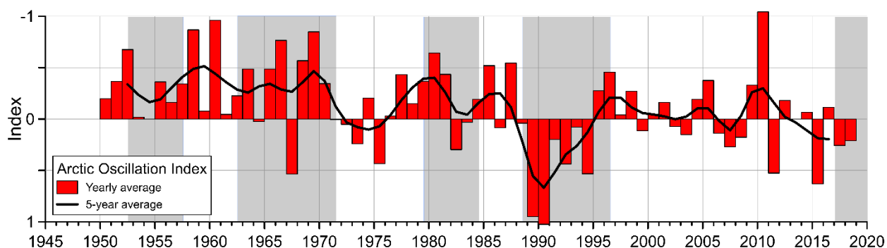
Figure 45. Variation of the Arctic Oscillation index over time. For ease of interpretation (and later comparisons), the index is plotted with negative values up-going. Grey-shaded panels denote periods of interest in the Beaufort region.
