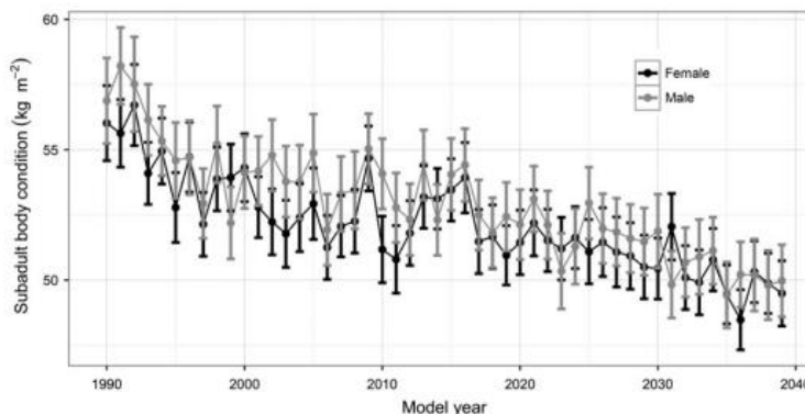
Figure 82. Across years, subadult body condition of polar bears is predicted to decrease in both males and females (source: Dey et al. 2017).
