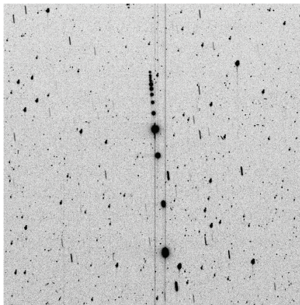
Fig.11 ( Top left ): Stack of NEOSSat frames of Orbcomm FM-20 during its conjunction with NEOSSat. ( Top right ): Photometry of Orbcomm FM 20 showing a departure from an inverse square brightness fit. ( Bottom left ): Iridium 17 stack showing the fade-out of the object just after TCA. ( Bottom right ): Photometry of Iridium 17 suggesting possible rotational motion of the secondary.
