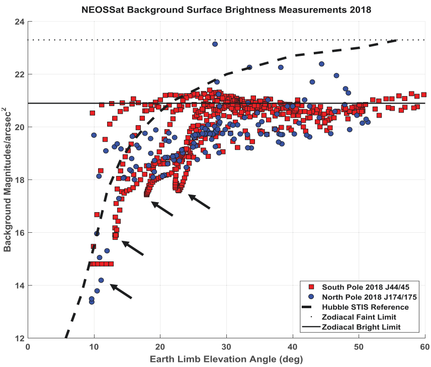
Fig.10 (Top left): NEOSSat test star fields in the CVZ. (Right Column): Images from NEOSSat during a South pole pass showing strong background surface brightness increase during polar crossings at 10° ELA. (Bottom Left): Surface brightness measurements by NEOSSat during Southern (Red) and Northern (Blue) polar crossings. The Hubble Space Telescope Imaging Spectrograph background brightness guideline [8] is shown for comparison.
