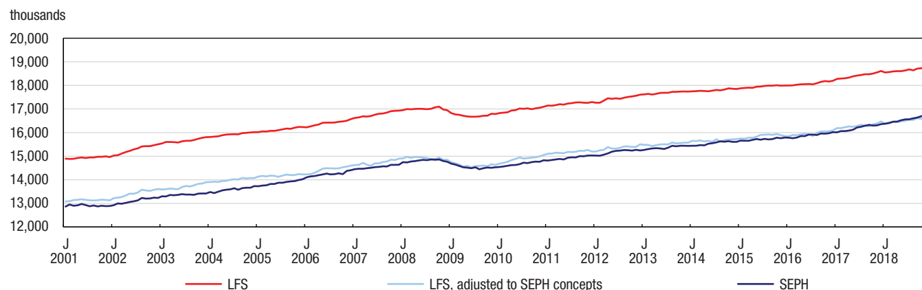
Chart 8.1 Labour Force Survey (LFS) and Survey of Employment, Payrolls and Hours (SEPH) employment levels, January 2001 to December 2018, seasonally adjusted
