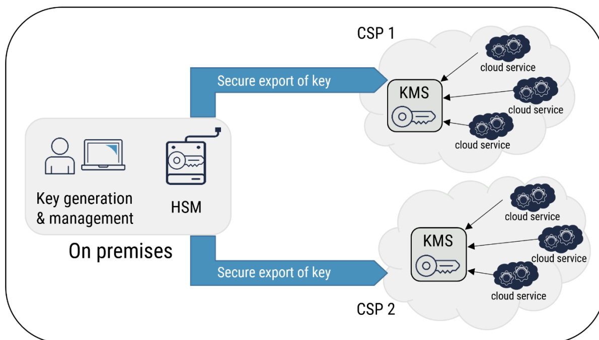
Figure 5: Service Mobility with BYOK
