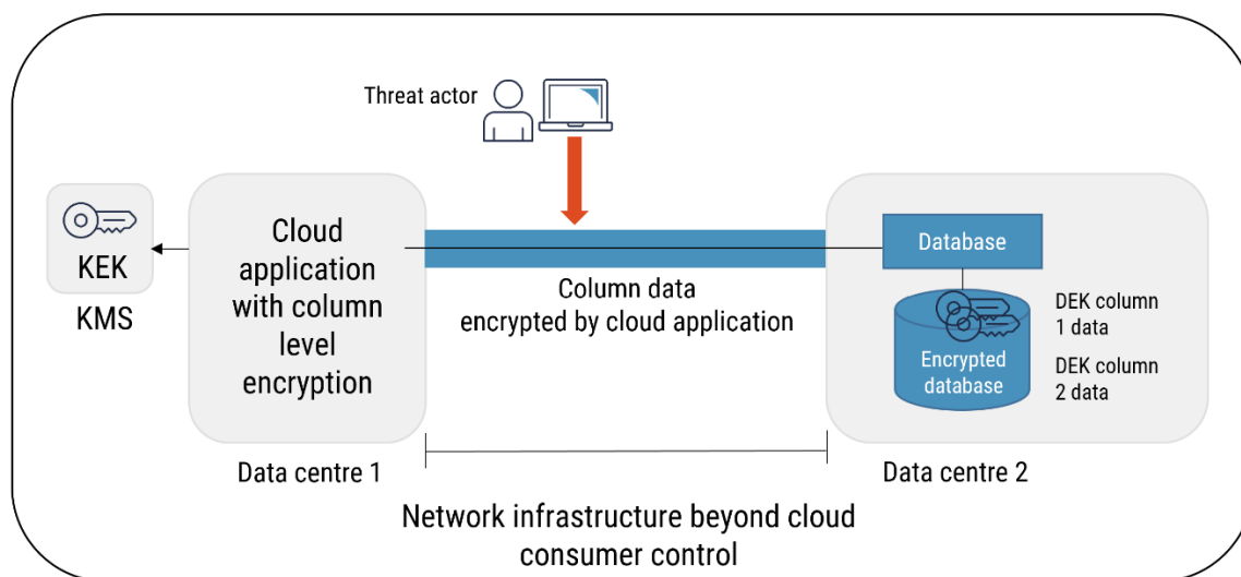
Figure 9: Column-Level Data Encryption
