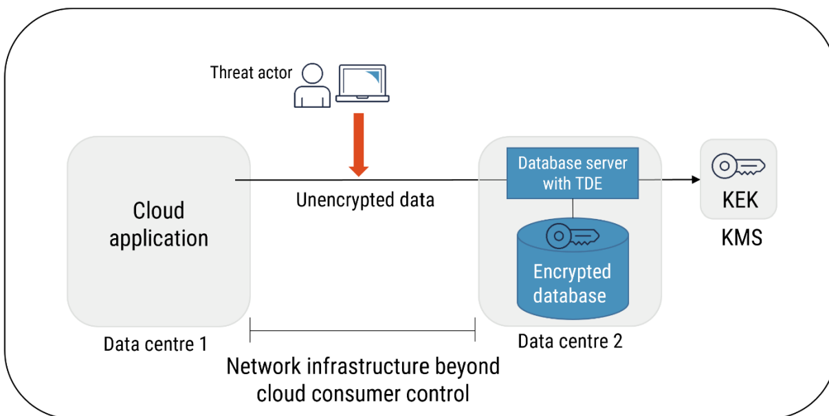
Figure 7: TDE without Encryption of Data in Transit
