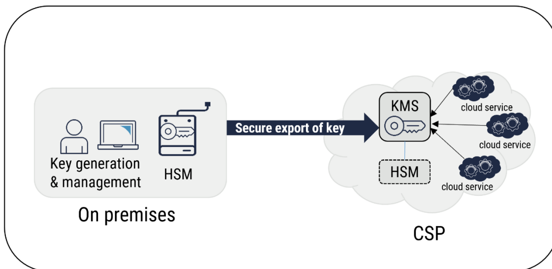
Figure 3: BYOK Concept
