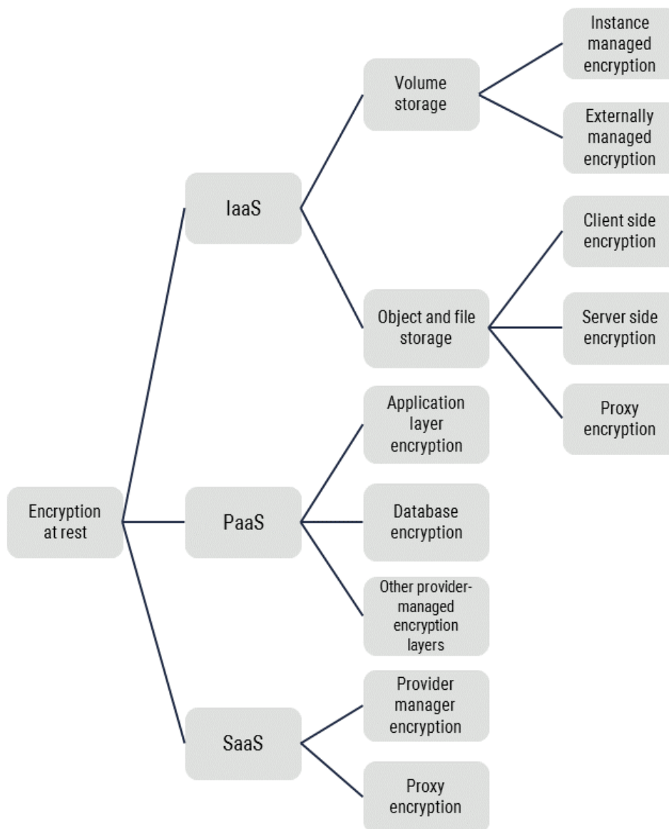
Figure 2: Encryption Options 9
