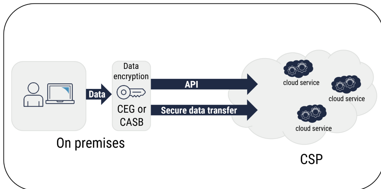
Figure 4: Data Encryption Using a CEG or a CASB
