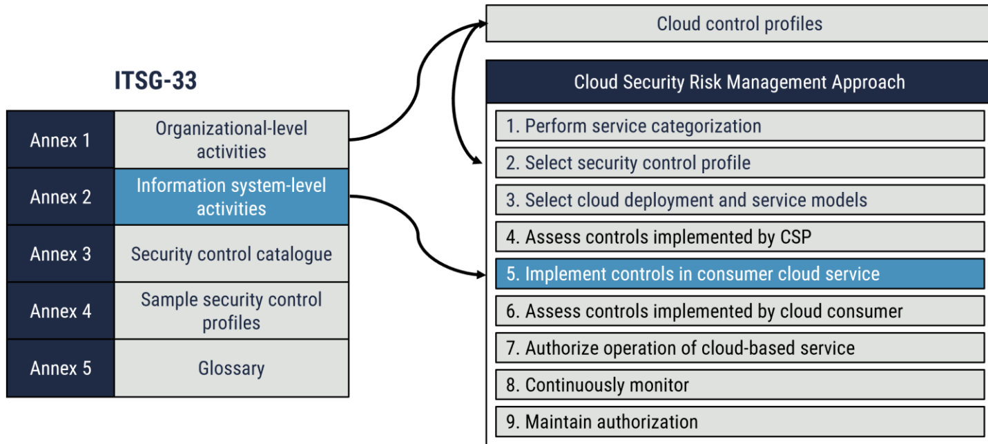
Figure 1: Relationship of Cloud Service Cryptography to IT Security Risk Management
