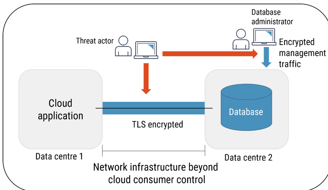
Figure 6: Encryption of Data in Transit
