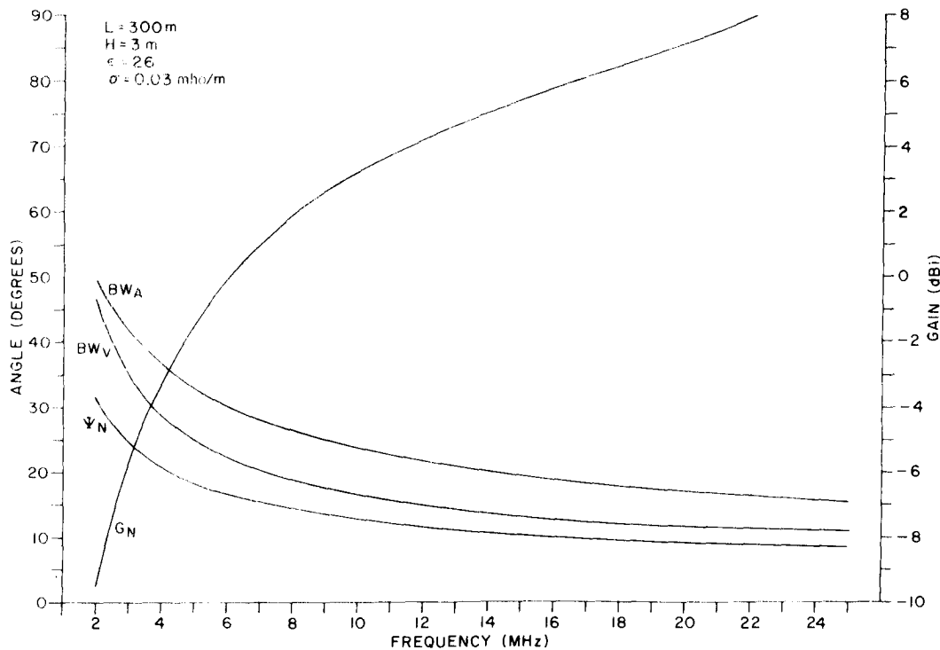
Figure II-43. Design Parameters for Wet Rich Soil, H = 2\text{ m} , L = 300\text{ m} .
