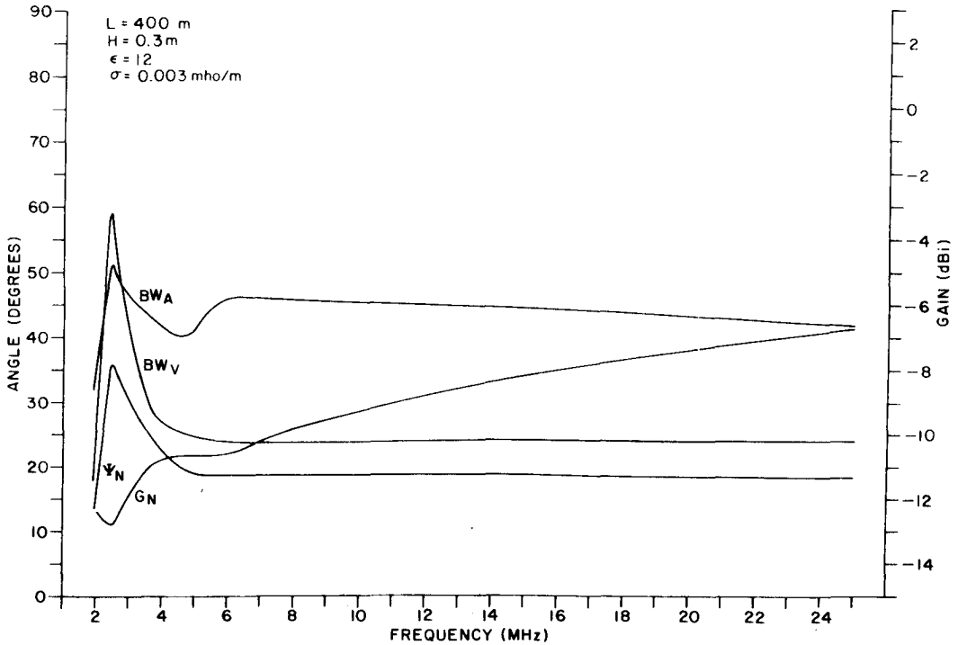
Figure II-20. Design Parameters for Average Soil (Dry), H = 0.3\text{m} , L = 400\text{m} .
