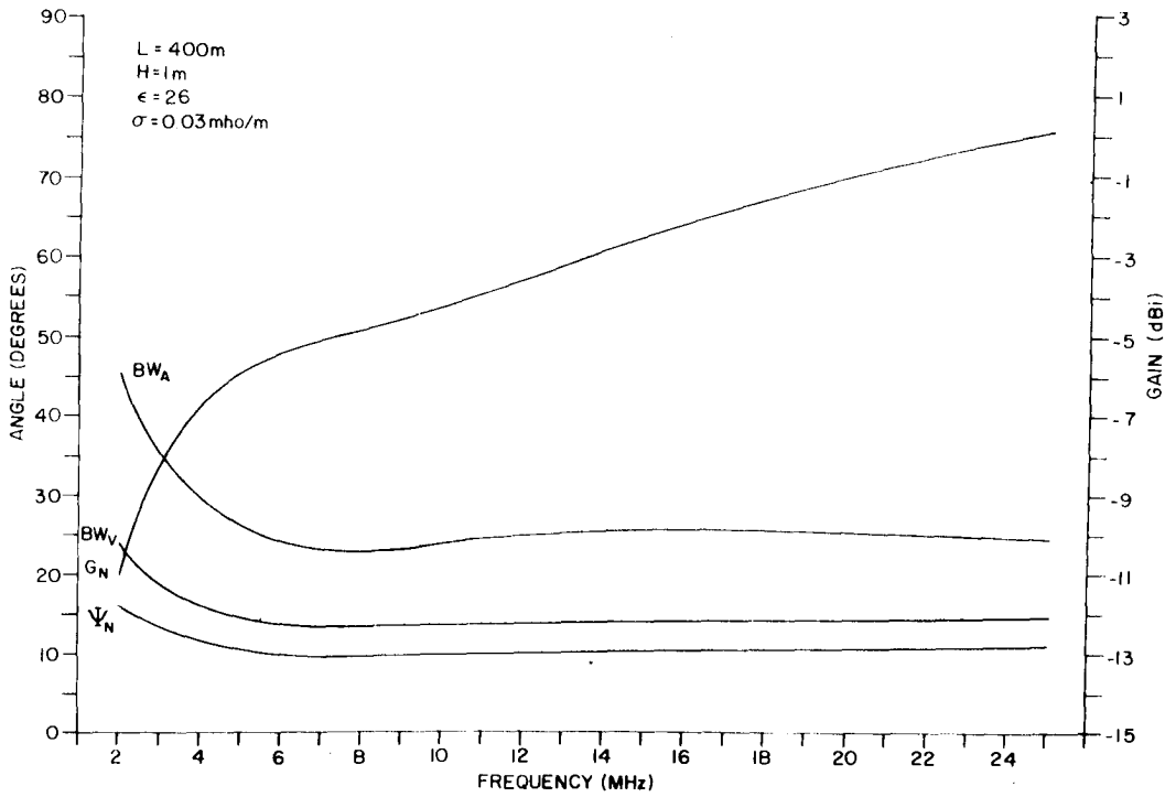
Figure II-40. Design Parameters for Wet Rich Soil, H = 1\text{m} , L = 400\text{m} .
