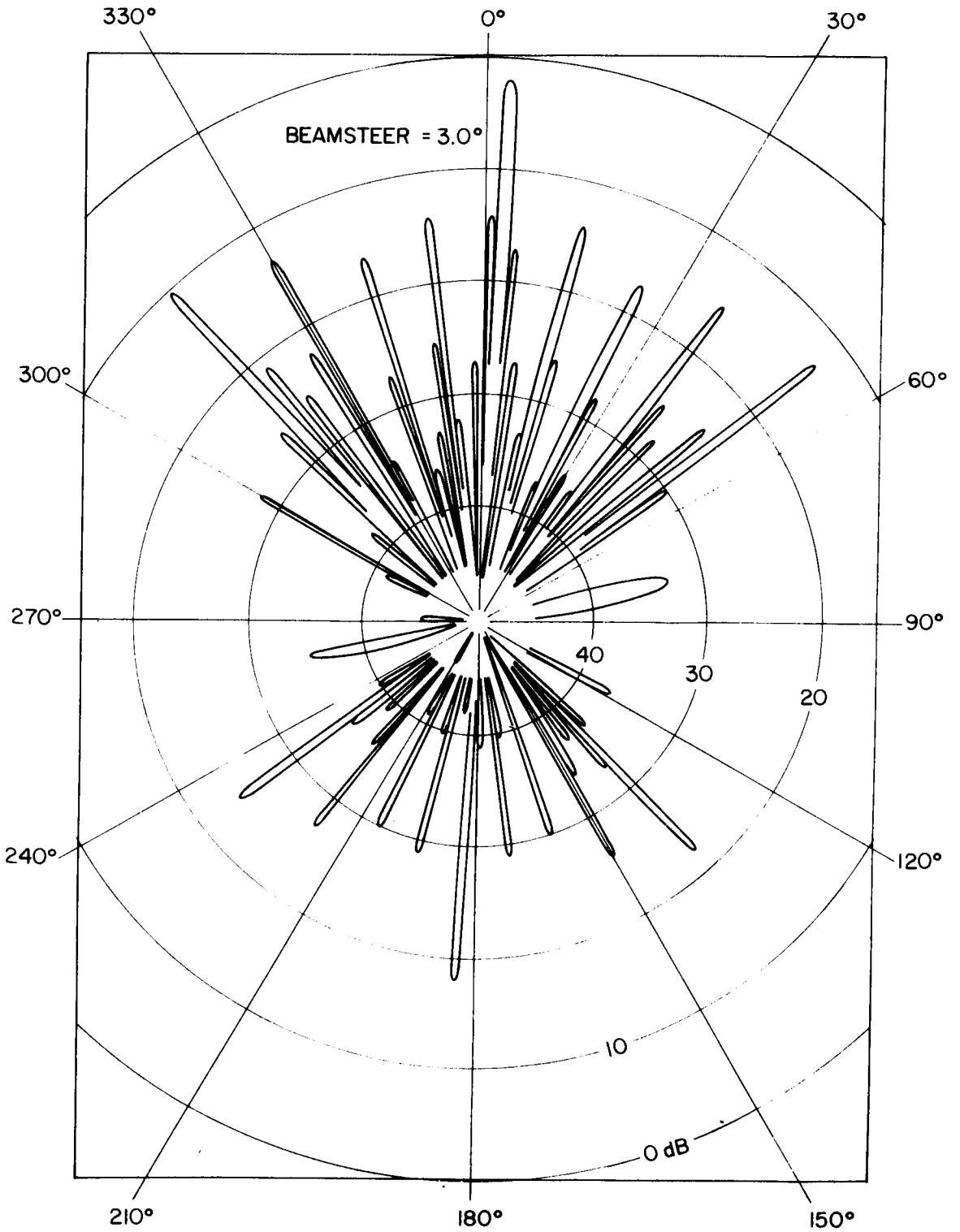
Figure IV-11. Polar Plot for Beamsteer = 3.0°
