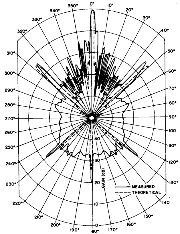
(b) Comparison of the theoretical and measured radiation patterns of the Cambridge Bay linear array at 9.75 MHz.
