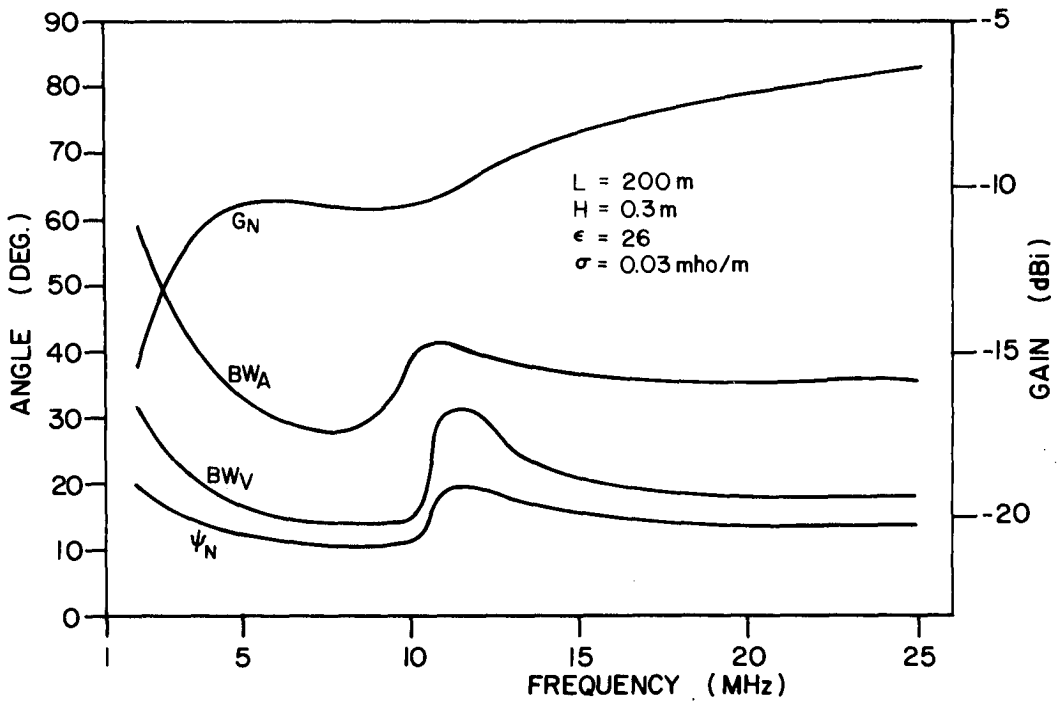
Figure II-34. Design Parameters for Wet Rich Soil, H = 0.3\text{m} , L = 200\text{m} .
