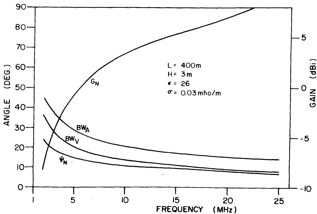
Figure II-48. Design Parameters for Wet Rich Soil, H = 3\text{m} , L = 400\text{m} .
