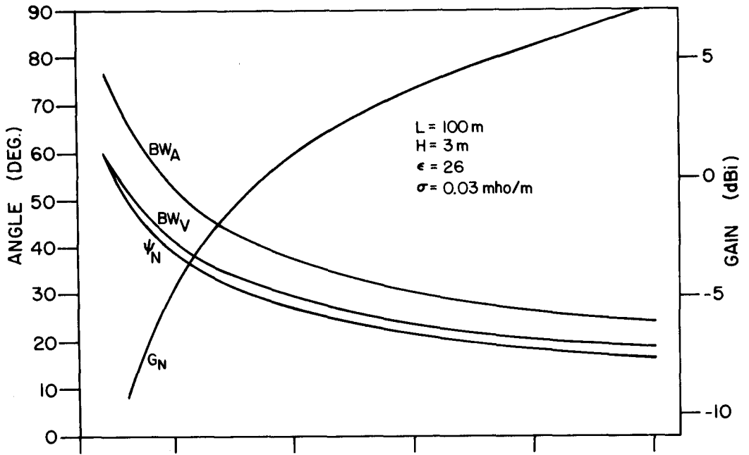
Figure II-45. Design Parameter for Wet Rich Soil, H = 3\text{m} , L = 100\text{m} .
