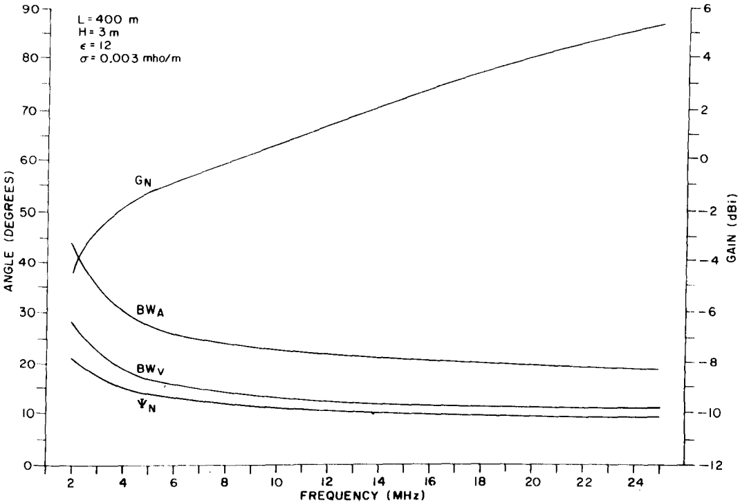
Figure II-32. Design Parameters for Average Soil (Dry), H = 3\text{m} , L = 400\text{m} .
