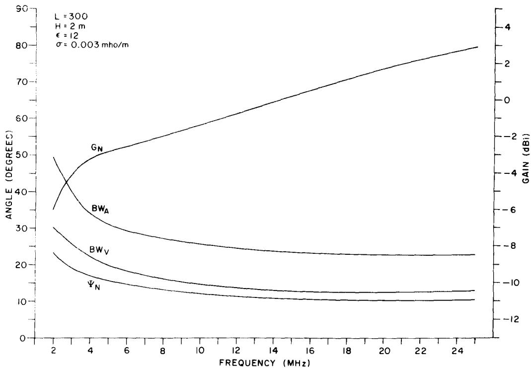
Figure II-27. Design Parameters for Average Soil (Dry), H = 2\text{m} , L = 300\text{m} .
