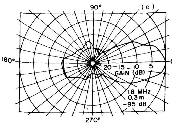
(c) Azimuthal pattern for Beverage antenna, L=110\text{m} , H=0.3\text{m} and f=18\text{MHz} .
