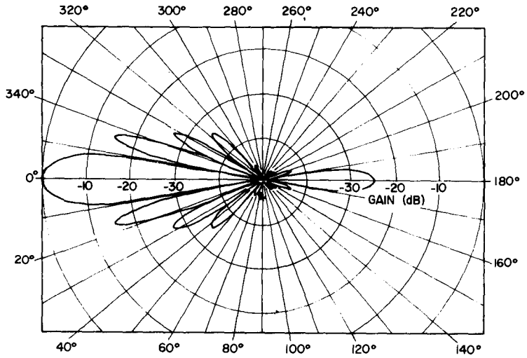
Figure 51. Theoretical 10 MHz azimuthal pattern for a Beverage antenna array with a 150m aperture. The elements are 110m long and their height above ground is 2m.
