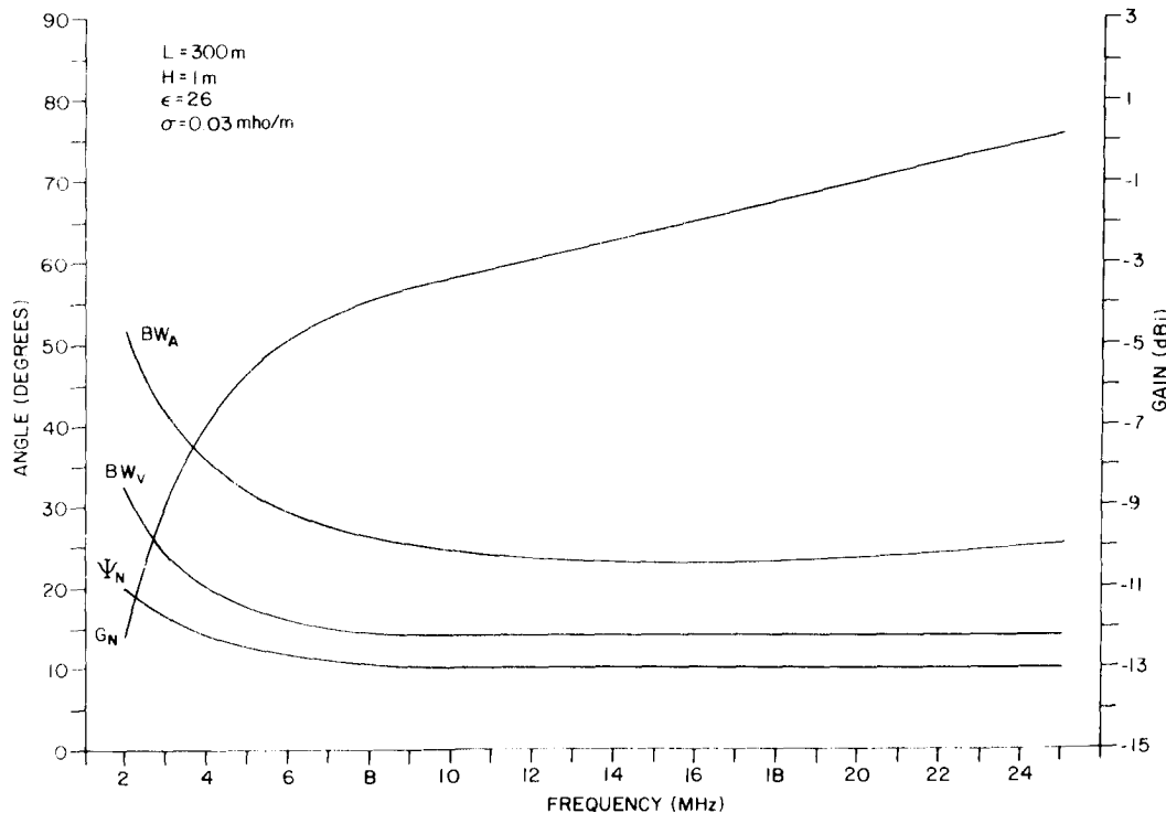
Figure II-39. Design Parameters for Wet Rich Soil, H = 1\text{m} , L = 300\text{m} .
