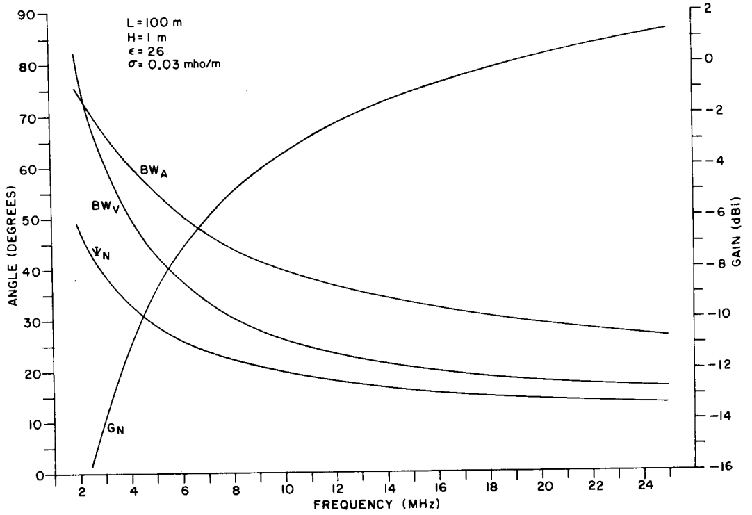
Figure II-37. Design Parameters for Wet Rich Soil, H = 1 \text{ m} , L = 100 \text{ m} .
