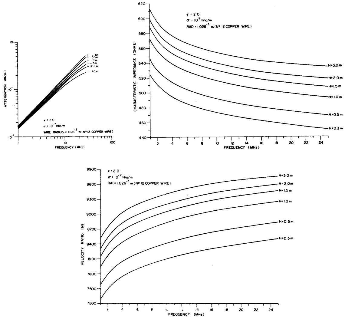
Figure I-1. Theoretical Values for Attenuation, Impedance and Wave Velocity for a Beverage Antenna on Dry Granite.
