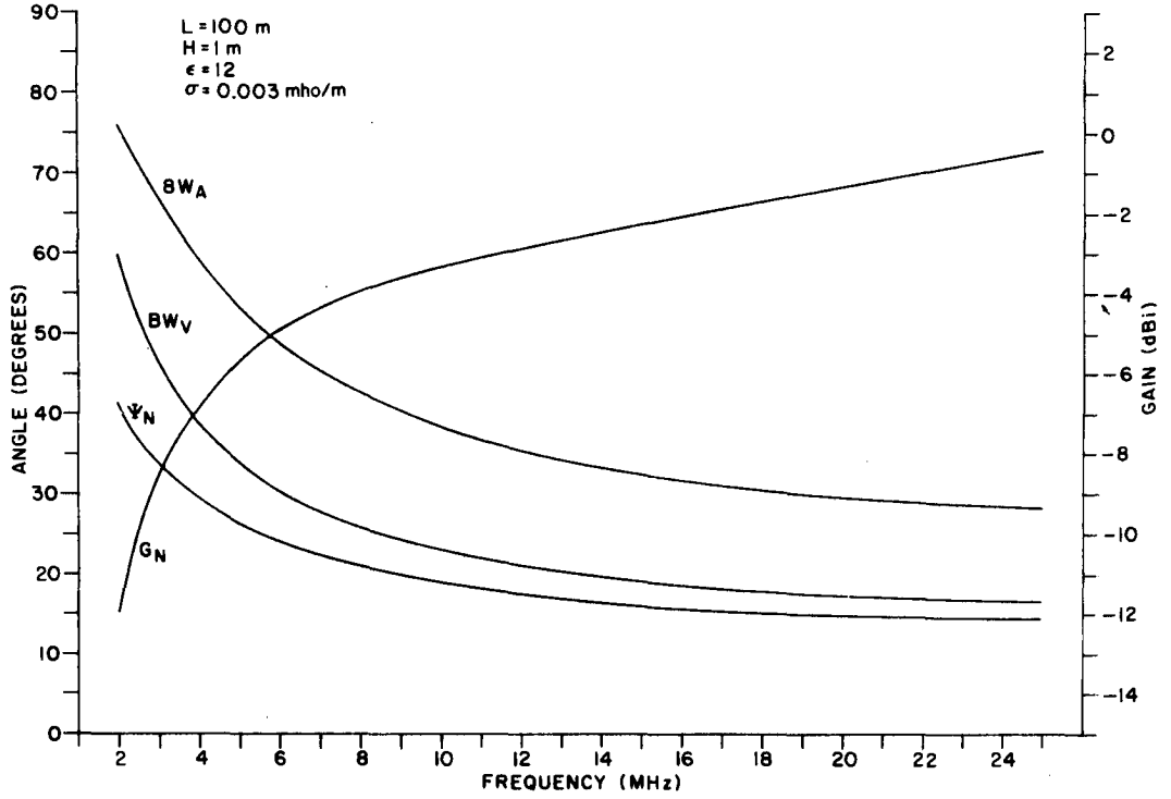
Figure II-21. Design Parameters for Average Soil (Dry), H = 1\text{m} , L = 100\text{m} .
