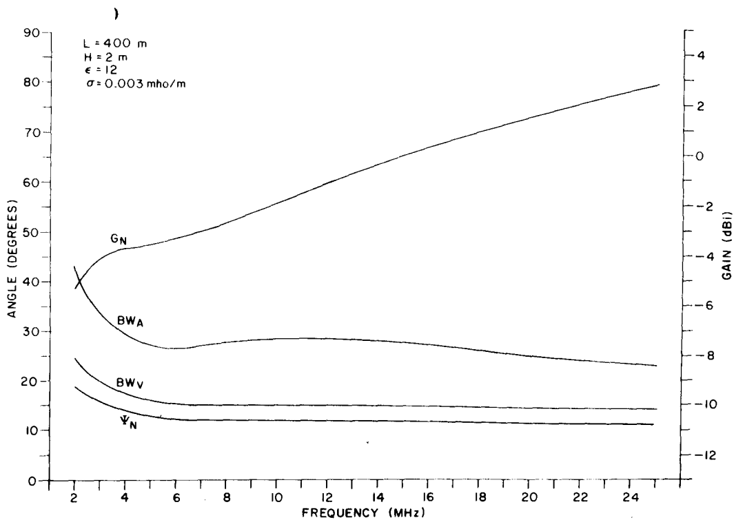
Figure II-28. Design Parameters for Average Soil (Dry), H = 2\text{m} , L = 400\text{m} .
