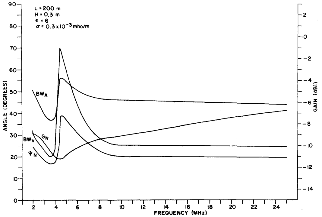
Figure II-2. Design Parameters for Poor Soil (Dry), H = 0.3\text{m} , L = 200\text{m} .
