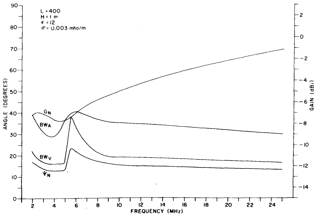
Figure II-24. Design Parameters for Average Soil (Dry), H = 1 \text{ m} , L = 400 \text{ m} .
