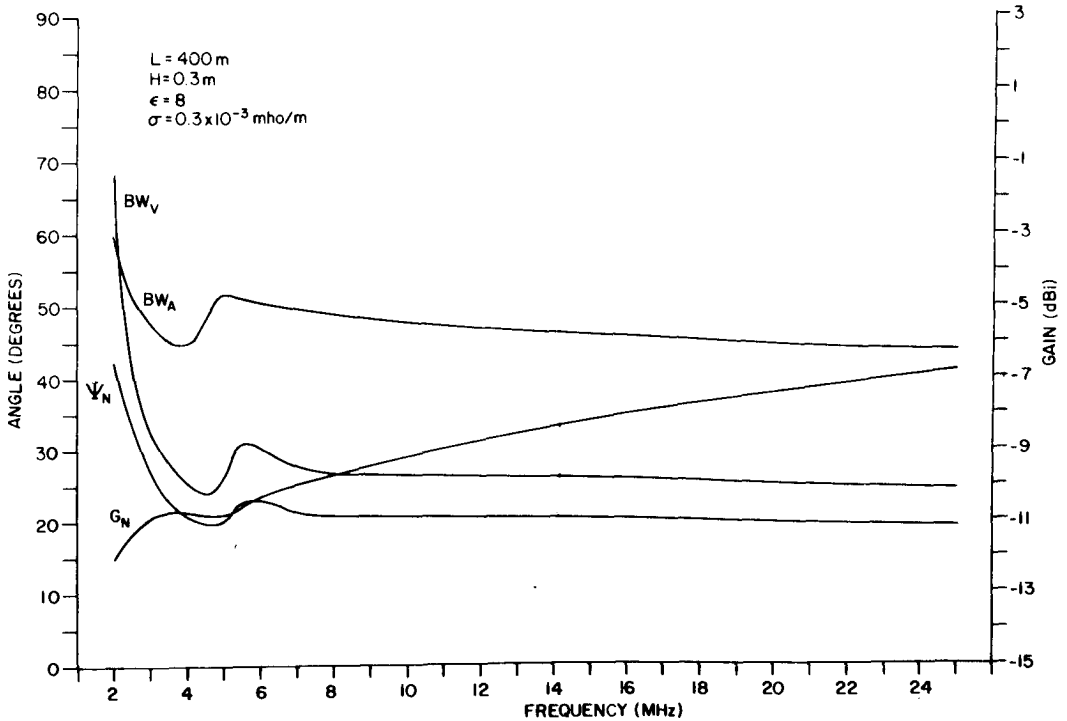
Figure II-4. Design Parameters for Poor Soil (Dry), H = 0.3\text{m} , L = 400\text{m} .
