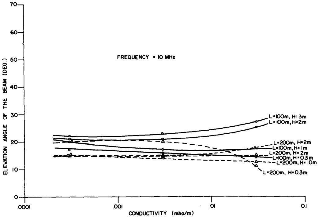
Figure 22. Vertical Beamwidth and Take-off Angle of a Beverage Antenna at 10 MHz as a Function of Soil Conductivity, Length and Height.
