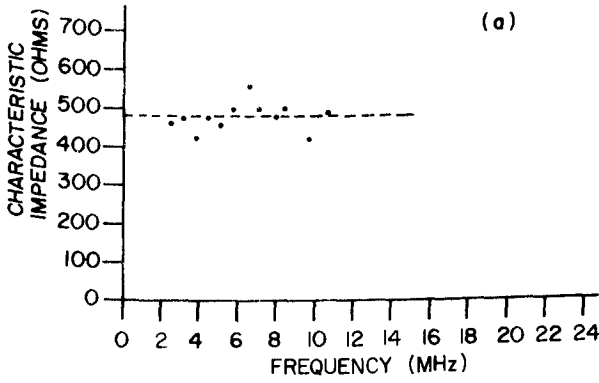
(a) Characteristic input impedance of element #1 derived from open and short circuit input impedance measurements.
