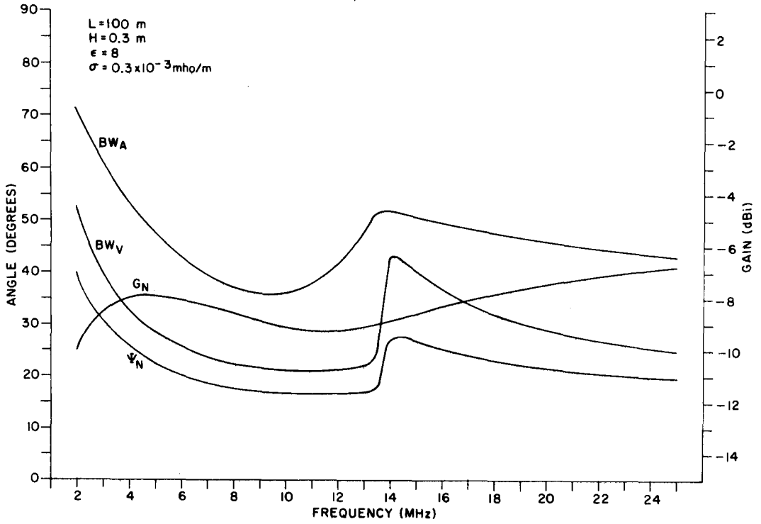
Figure II-1. Design Parameters for Poor Soil (Dry), H = 0.3\text{m} , L = 100\text{m} .
