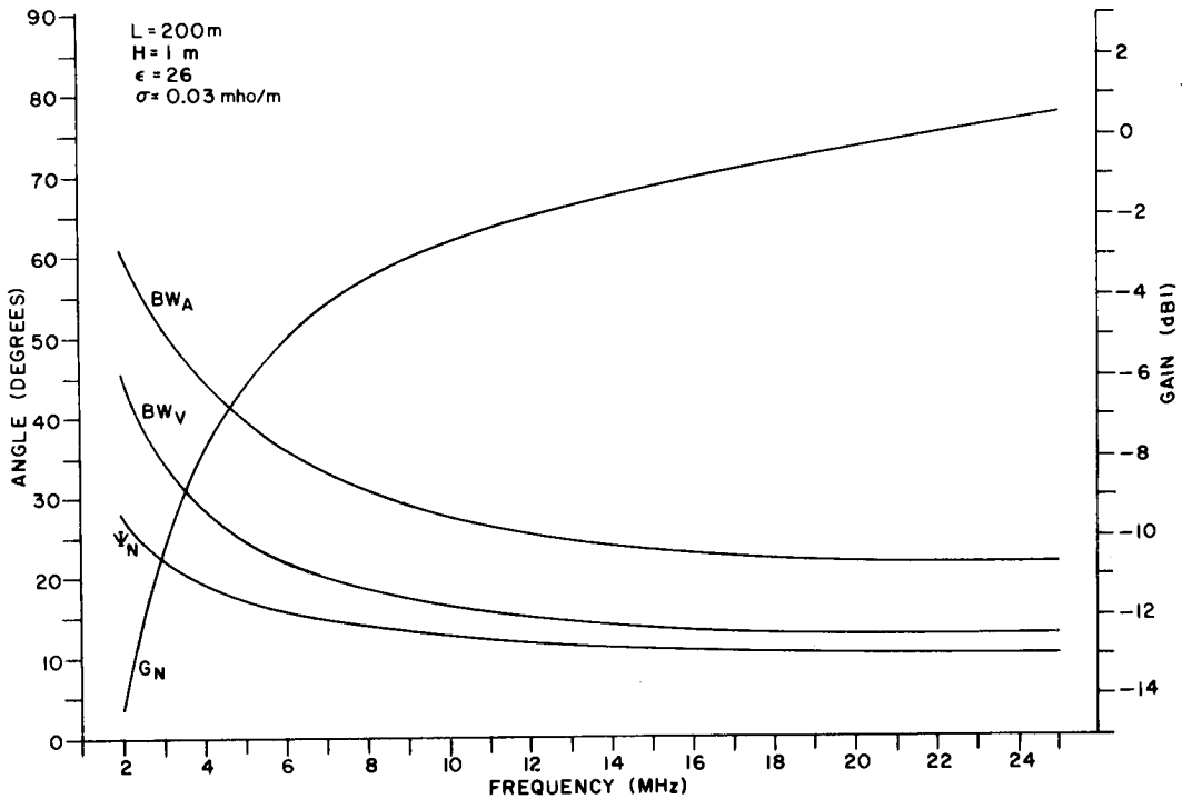
Figure II-38. Design Parameters for Wet Rich Soil, H = 1 \text{ m} , L = 200 \text{ m} .
