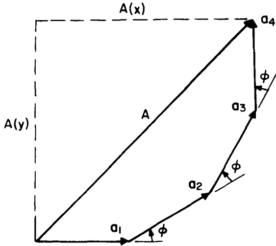
Figure IV-7. Phasor Diagram of One Segment of 4 Elements.
