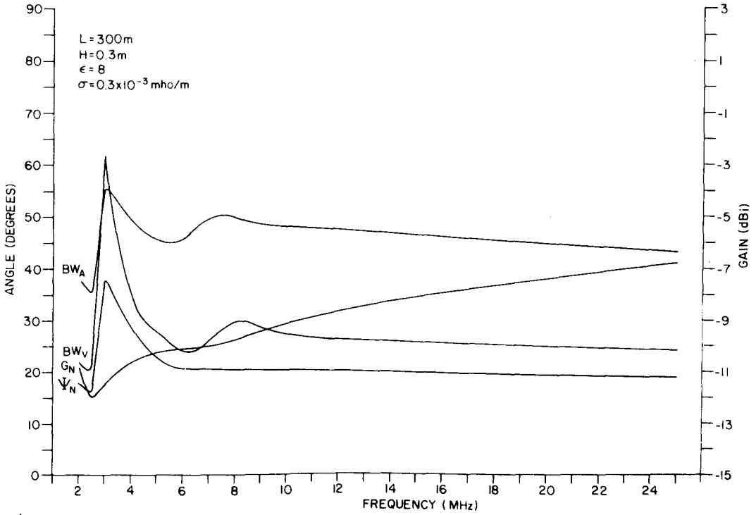
Figure II-3. Design Parameters for Poor Soil (Dry), H = 0.3\text{m} , L = 300\text{m} .
