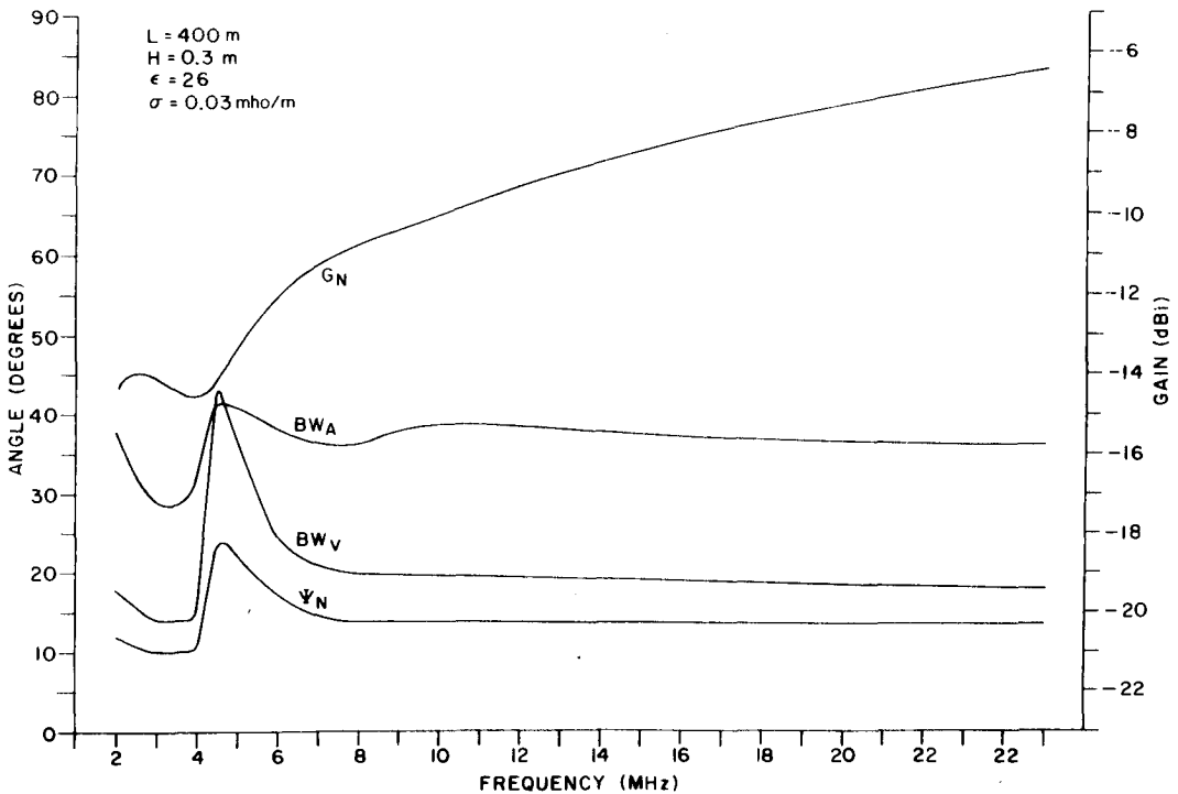
Figure II-36. Design Parameters for Wet Rich Soil, H = 0.3\text{m} , L = 400\text{m} .
