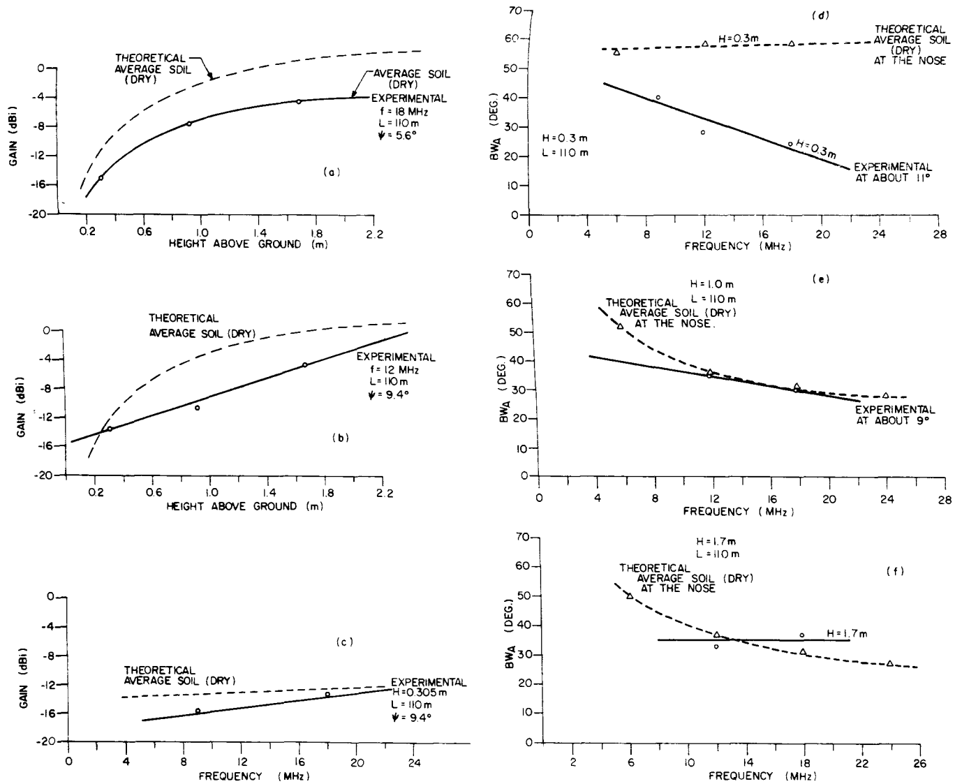
Figure 23. Comparison of Theoretical and Measured Values of Gain G_N and Azimuthal Beamwidth BW_A of a Beverage Antenna. The Measurements were made at Shirley Bay with the Antenna on Average Soil (Dry).
