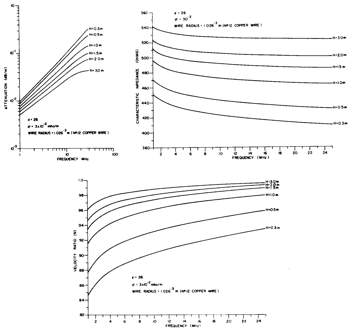
Figure I-7. Theoretical Values of Attenuation, Impedance and Velocity Ratio for a Beverage Antenna on Wet Rich Soil.
