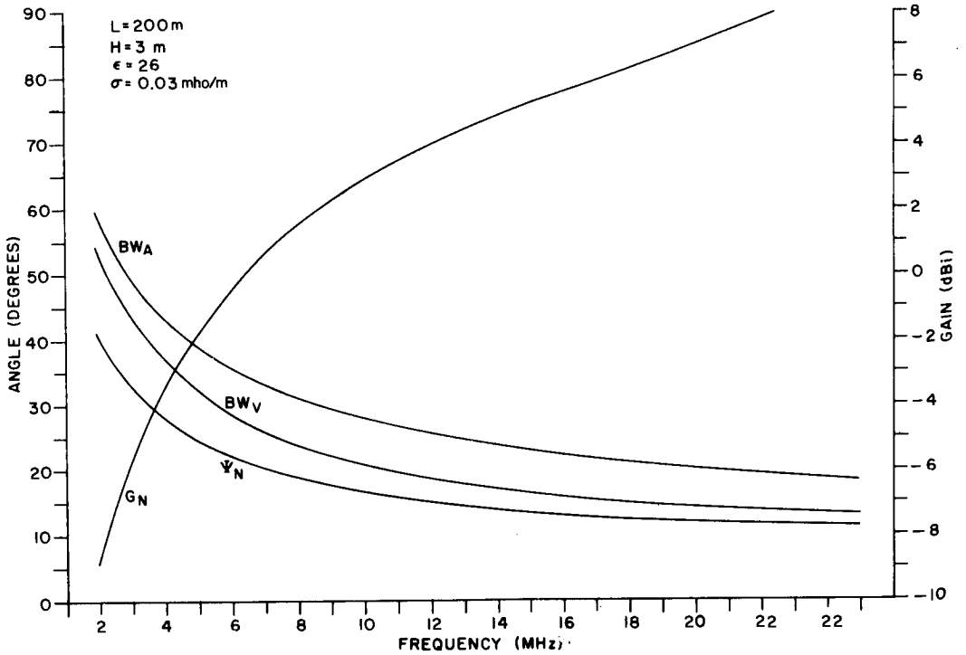
Figure II-42. Design Parameters for Wet Rich Soil, H = 2\text{m} , L = 200\text{m} .
