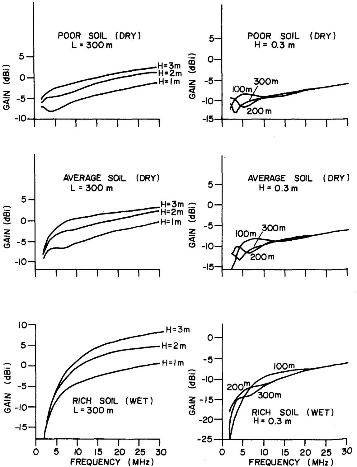
Figure III-2. Theoretical Surface Wave Gain of Beverage Antennas with a Length of 300m, Heights of 1, 2, and 3m over Poor Soil (Dry), Average Soil (Dry) and Rich Soil (Wet). Curves are also Given for a Height of 0.3m, Lengths of 100, 200 and 300m and Poor Soil (Dry), Average Soil (Dry) and Rich Soil (Wet).
