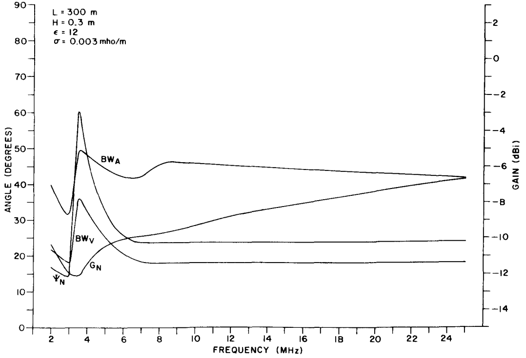
Figure II-19. Design Parameters for Average Soil (Dry), H = 0.3\text{m} , L = 300\text{m} .
