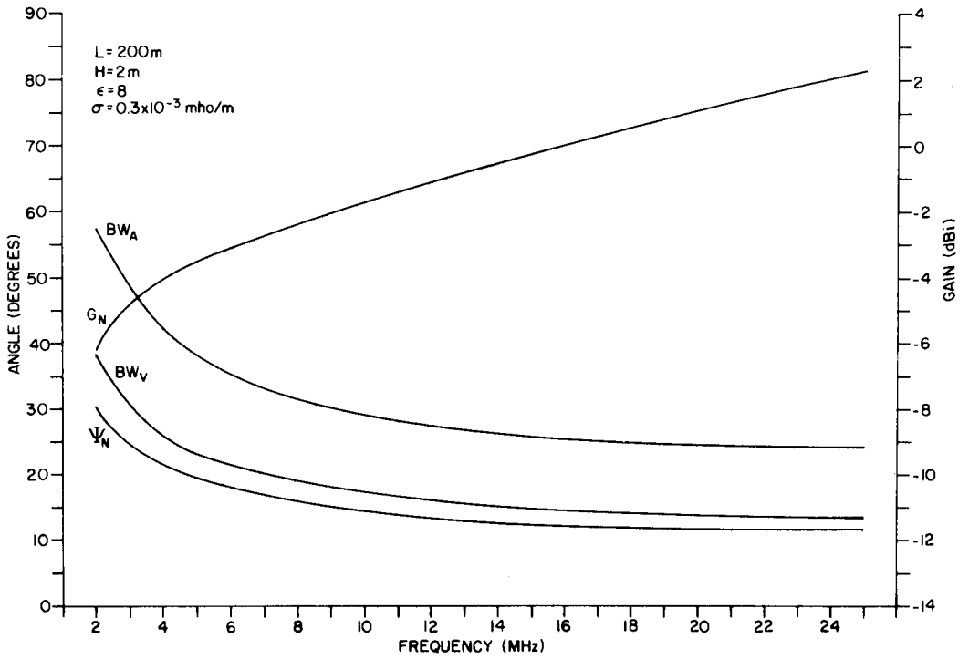
Figure 11-10. Design Parameters for Poor Soil (Dry), H = 2\text{m} , L = 200\text{m} .
