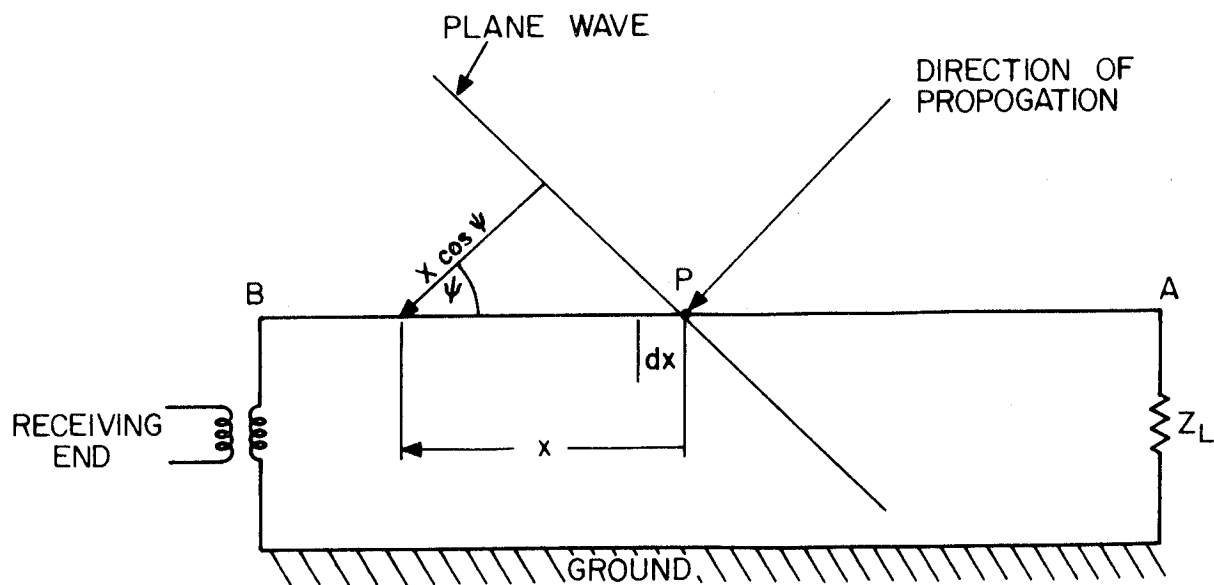
Figure IV-1. Model of the Beverage Antenna
