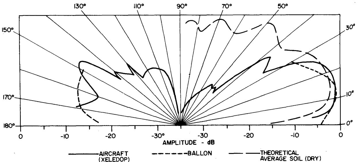
Figure 33. Comparison of theoretical and measured radiation patterns for a Cambridge Bay Beverage pair antenna. The balloon measurements were made at 9.0 MHz and the XELEDOP measurements were made at 9.75 MHz. The theoretical curve was derived for a frequency of 9.5 MHz and average soil (dry).
