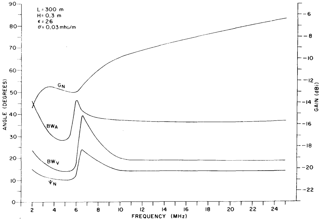
Figure II-35. Design Parameters for Wet Rich Soil, H = 0.3\text{m} , L = 300\text{m} .
