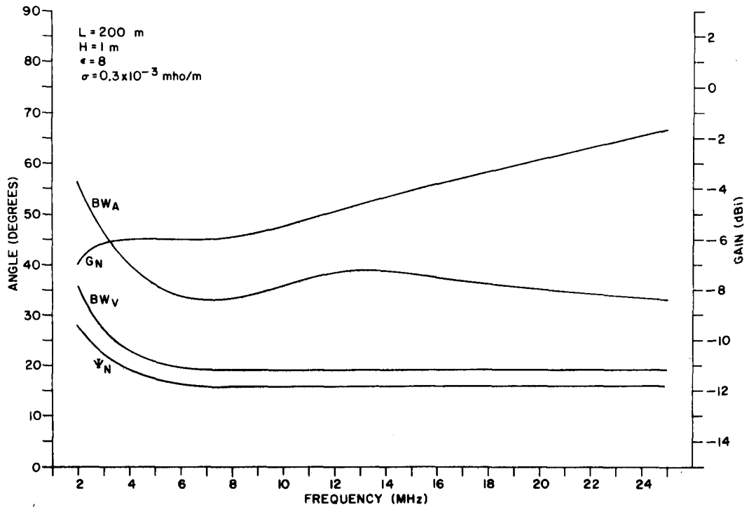
Figure II-6. Design Parameters for Poor Soil (Dry), H = 1\text{m} , L = 200\text{m} .
