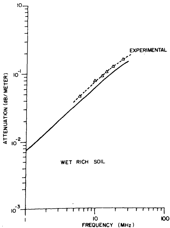
Figure 12. Comparison of experimental current-wave attenuation at Cambridge Bay and theoretical current-wave attenuations for average soil (dry), average soil (wet) and wet rich soil.
