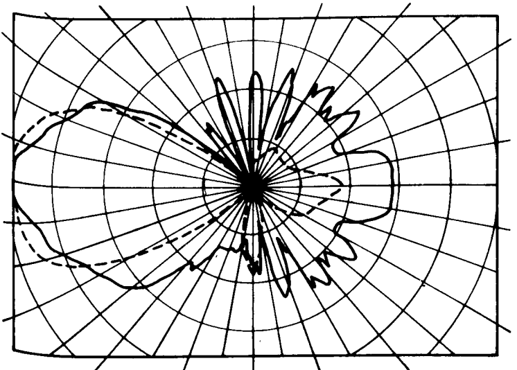
Figure 31. Comparisons of measured azimuthal radiation patterns at 9.75 MHz for a Beverage pair antenna at Cambridge Bay.
