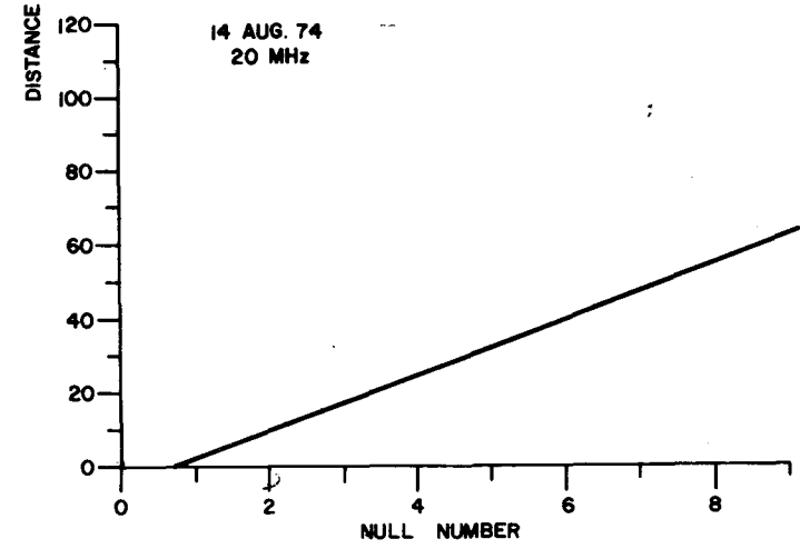
Figure 13. Displacement of Current-wave Null from Terminated End Versus Null Number for 5, 10, 15 and 20 MHz.
