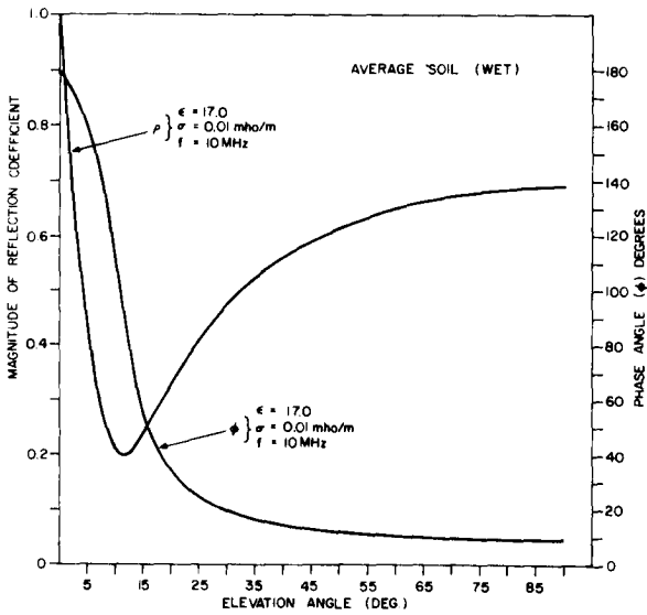
Figure 6. Reflection Coefficients at 10 MHz for Sea Water, Wet Rich Soil, Average Soil (Wet) and Poor Soil.
