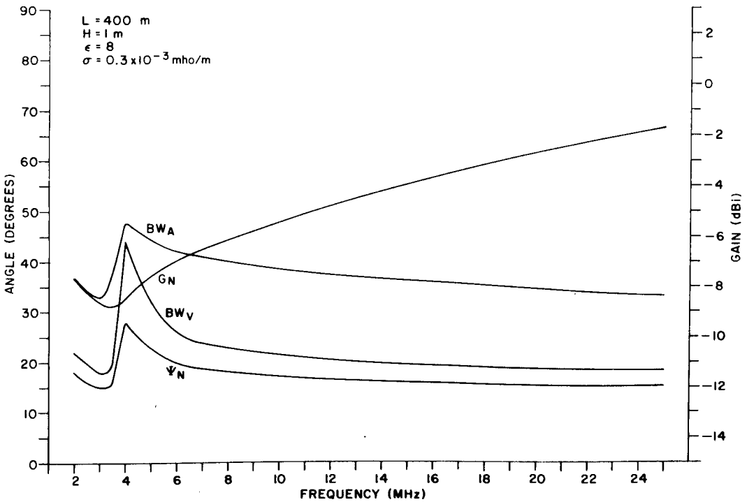
Figure II-8. Design Parameters for Poor Soil (Dry), H = 1 \text{ m} , L = 400 \text{ m} .
