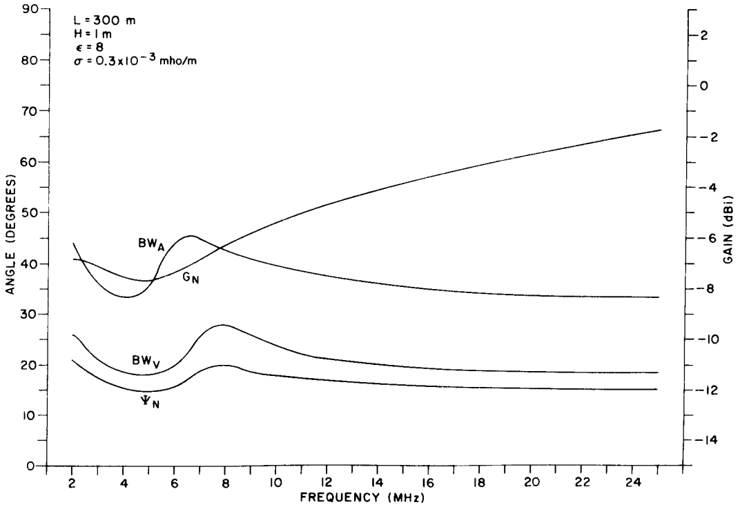
Figure II-7. Design Parameters for Poor Soil (Dry), H = 1 \text{ m} , L = 300 \text{ m} .
