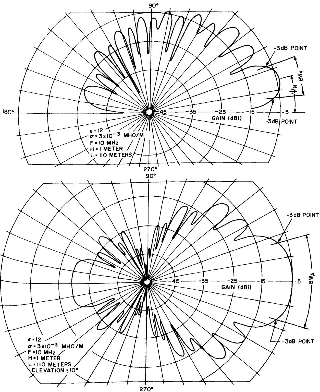
Figure 18. Typical theoretical elevation and azimuthal radiation patterns for a Beverage element situated over average soil (dry) and whose length and height are 110 m and 1 m, respectively. The 3-dB vertical beamwidth BW_V , take-off angle \psi_N , gain G_N and 3-dB azimuthal beamwidth BW_A as defined in Section 3.1 are illustrated.
