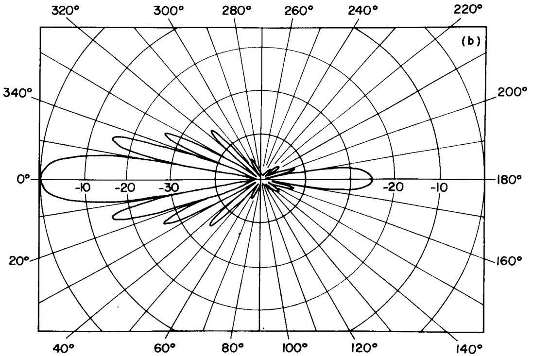
(b) Sixteen-elements
