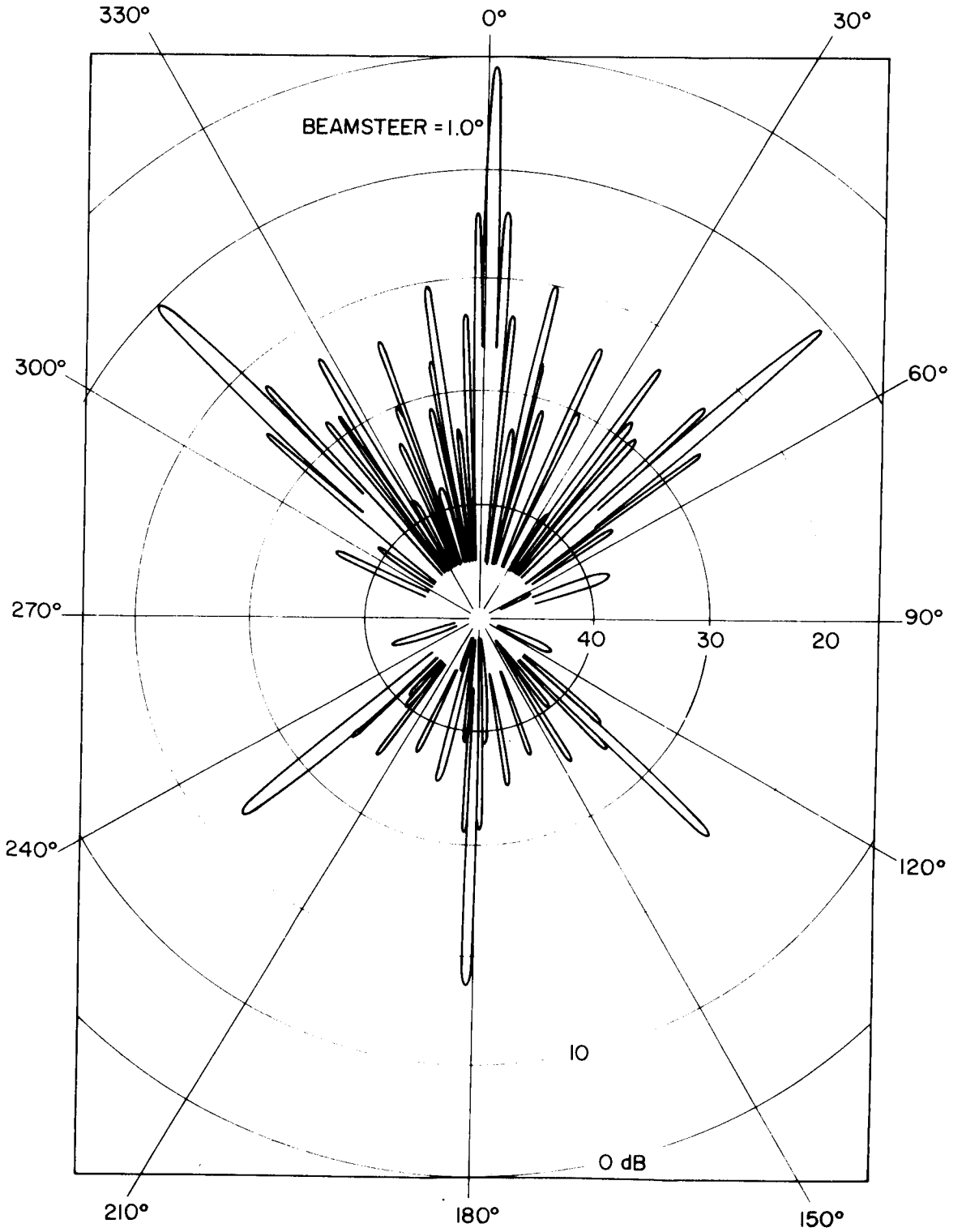
Figure IV-9. Polar Plot for Beamsteer = 1.0°
