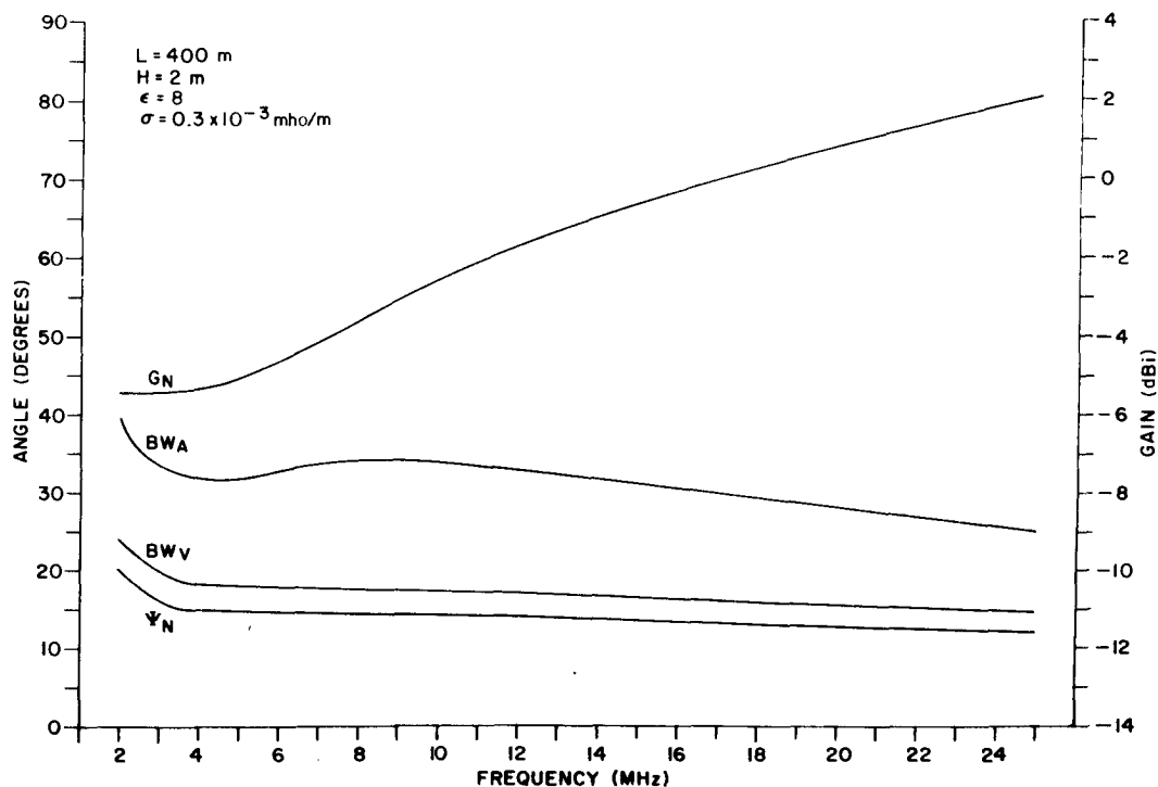
Figure 11-12. Design Parameters for Poor Soil (Dry), H = 2\text{m} , L = 400\text{m} .
