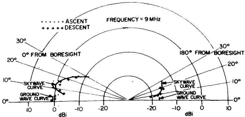
Figure 38. Field Intensity at the Center of the Array From a Balloon-Suspended Transmitter.
