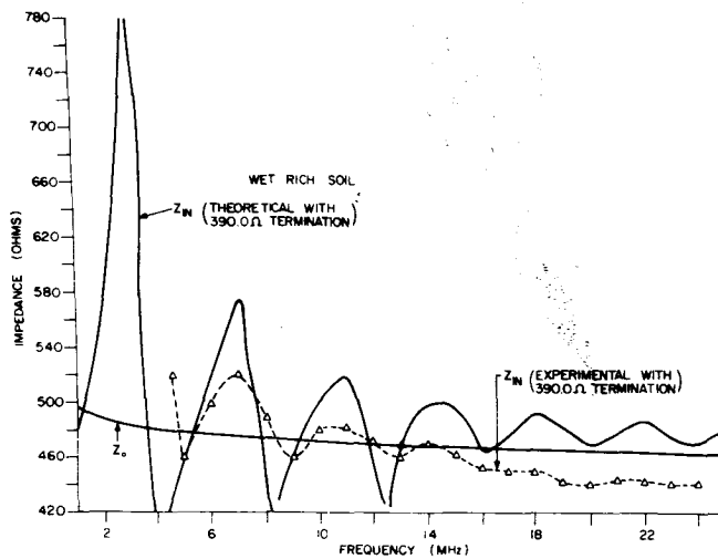
Figure 10. Measured input impedance for a Beverage antenna with a height above ground of 1 meter terminated in 390 ohms. Theoretical curves are included for antennas terminated in 390 ohms and Z_0 over poor soil, average soil (dry), average soil (wet) and wet rich soil.
