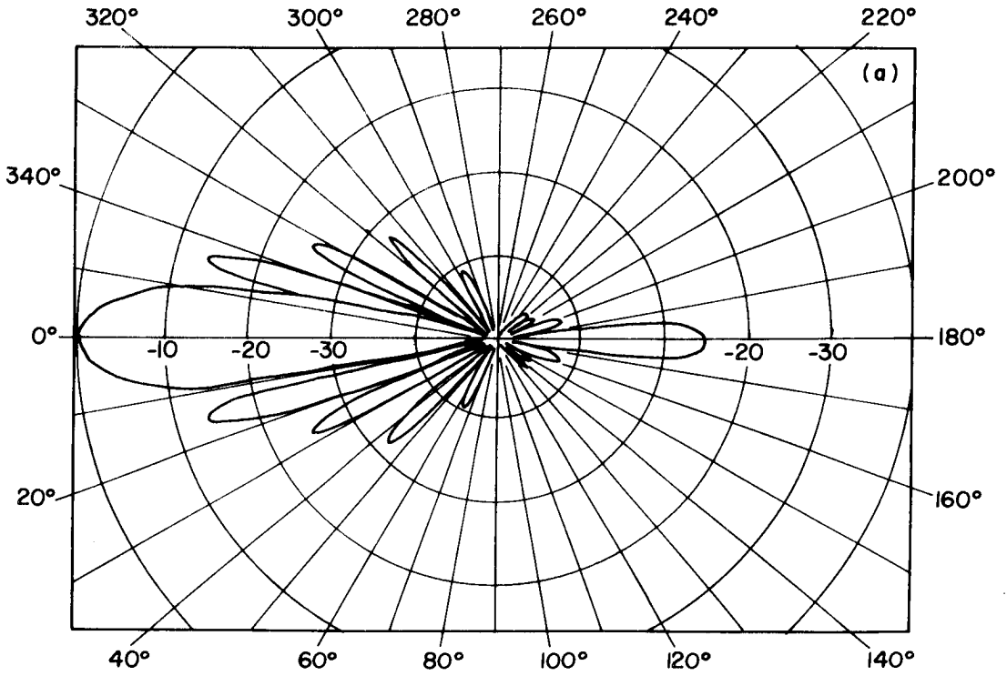
(a) Eight-elements
