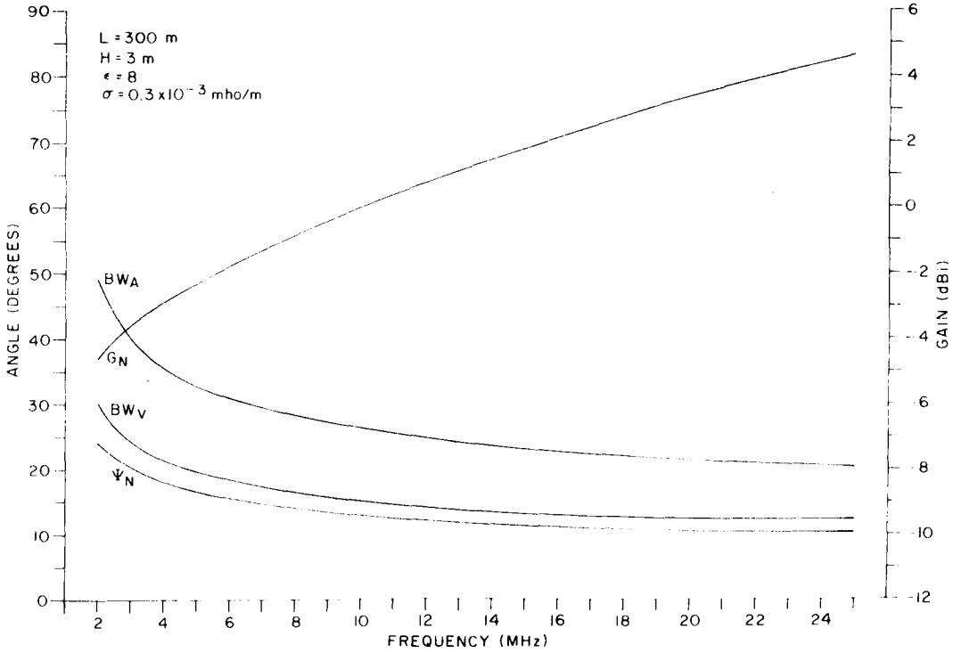
Figure II-15. Design Parameters for Poor Soil (Dry), H = 3\text{m} , L = 300\text{m} .
