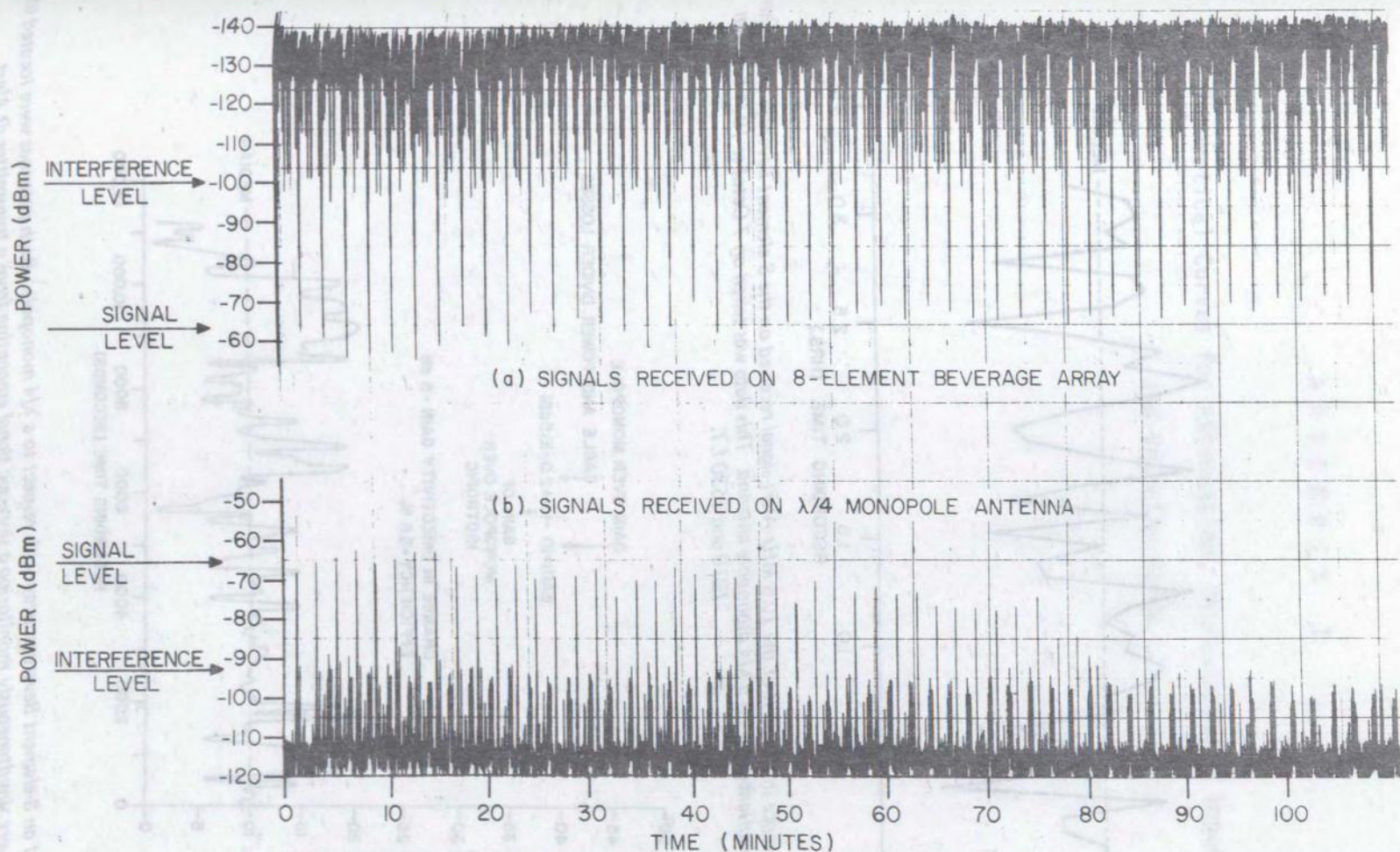
Figure 53. Comparison of signal received by 8-element Beverage array and \lambda/4 monopole antenna the larger amplitude vertical lines separated by 100 sec intervals in both (a) and (b) represent the amplitude of the wanted Alert signal. The other vertical lines represent amplitudes of interfering signals located in the frequency window \pm 25 KHz centered on the frequency of the Alert signal which remained constant throughout.
