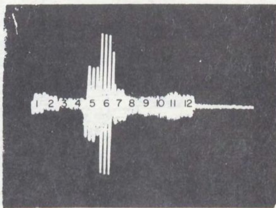
(d) Sequential sampling of the terminal voltages of the 12 Beverage pair antennas at Cambridge Bay, monitoring wvw on 15 MHz, somewhat later in time than (c).
