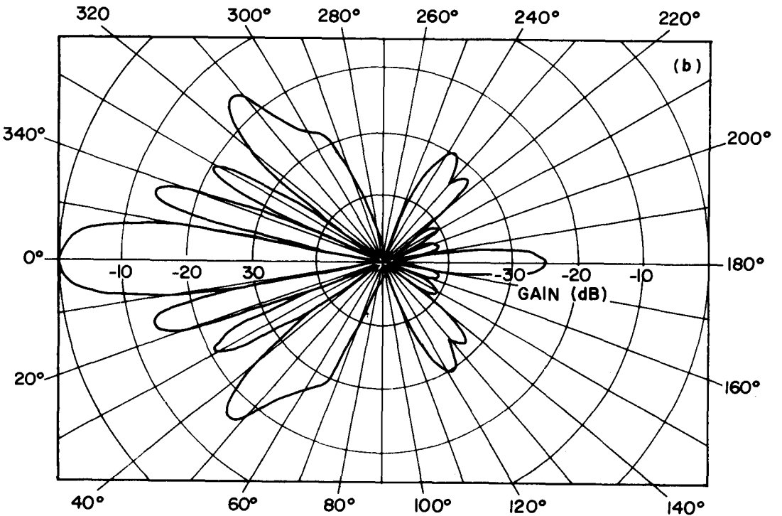
(b) Four-elements
