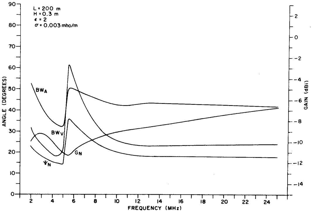
Figure II-18. Design Parameters for Average Soil (Dry), H = 0.3\text{m} , L = 200\text{m} .
