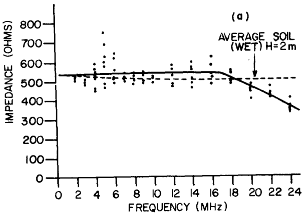
(a) Composite input impedance of 8-elements.
