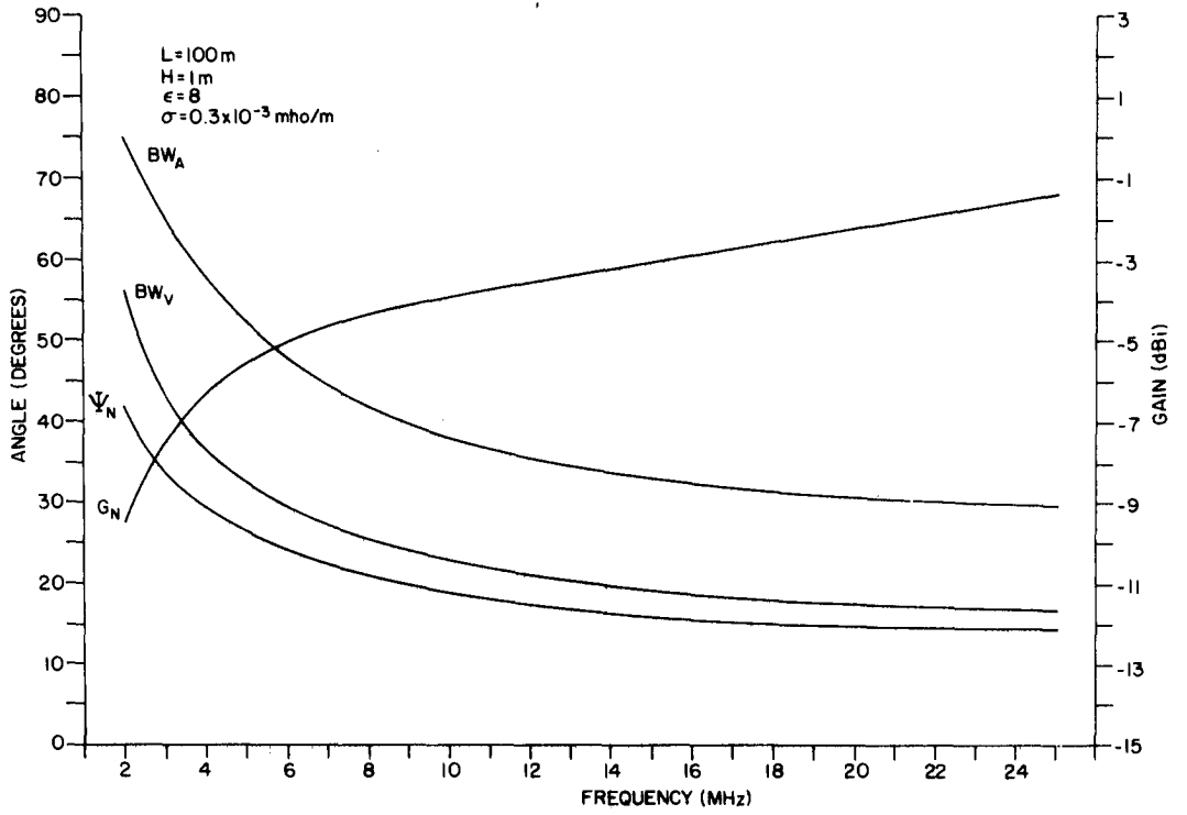
Figure II-5. Design Parameters for Poor Soil (Dry), H = 1\text{m} , L = 100\text{m} .
