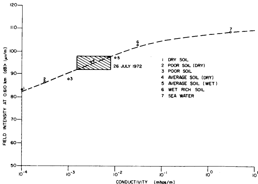
Figure 9. Comparison of field intensity measured at a distance of 0.610 km from position of the center of the rosette array with theoretical values for earth types varying from dry sand to sea water.
