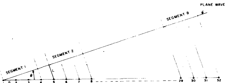
Figure IV-6. Illustration of the Segmentation of the Linear Array.
