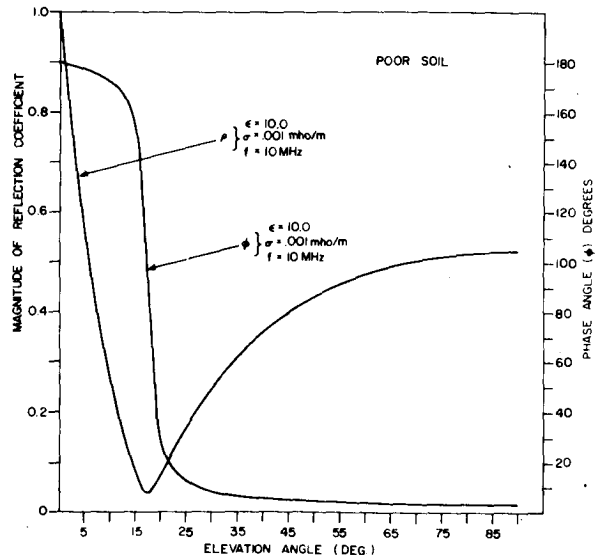
Figure 6. Reflection Coefficients at 10 MHz for Sea Water, Wet Rich Soil, Average Soil (Wet) and Poor Soil.
