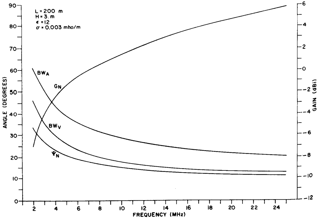
Figure II-30. Design Parameters for Average Soil (Dry), H = 3\text{m} , L = 200\text{m} .
