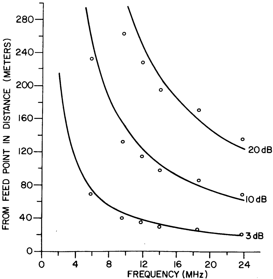
Figure 35. Attenuation Contours for RF Currents on a Beverage Antenna.
