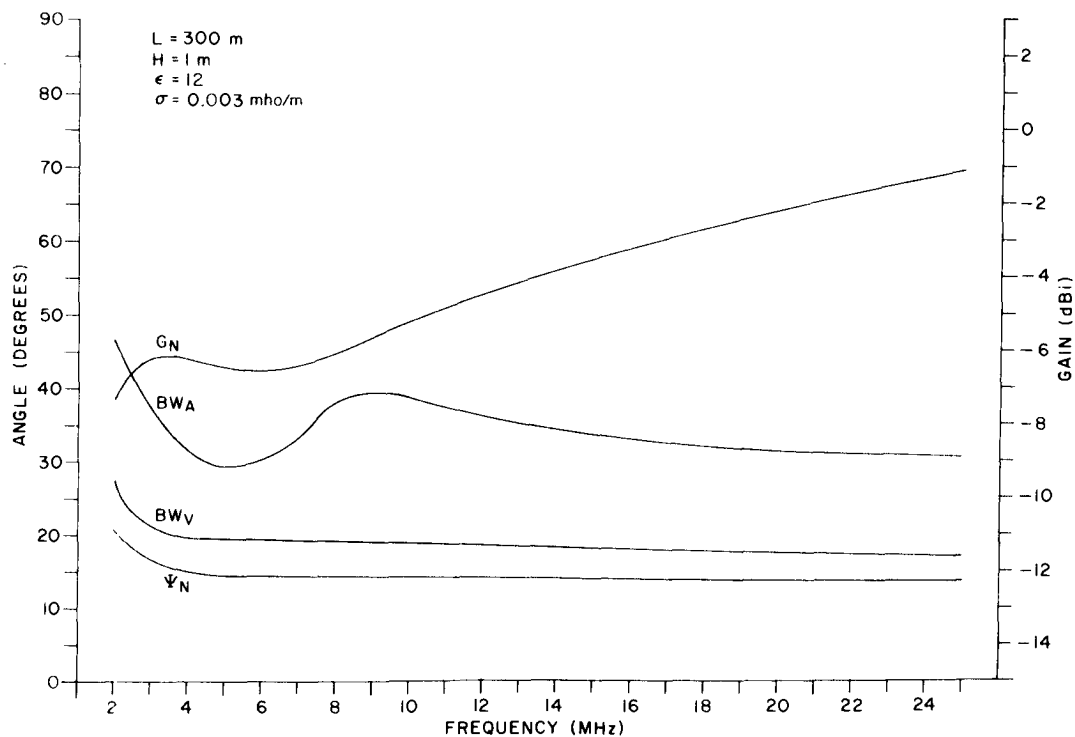
Figure II-23. Design Parameters for Average Soil (Dry), H = 1 \text{ m} , L = 300 \text{ m} .
