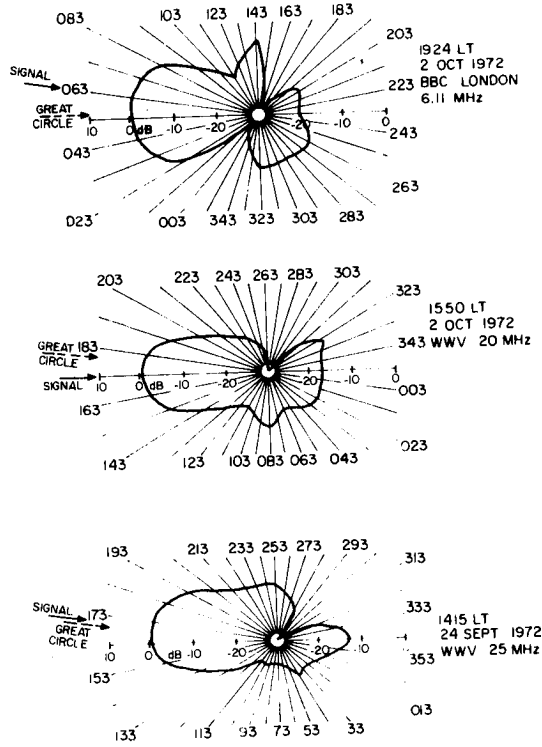
Figure 42. Direction Finding Patterns Obtained With the Beverage Array from Known Transmitters.
