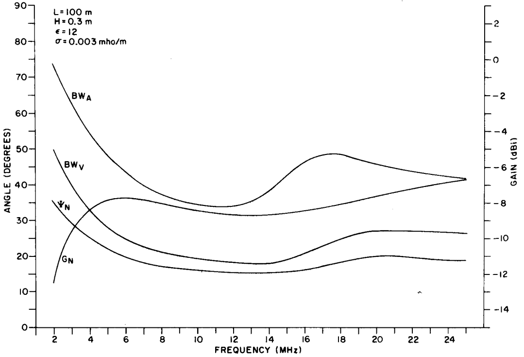
Figure II-17. Design Parameters for Average Soil (Dry), H = 0.3\text{m} , L = 100\text{m} .
