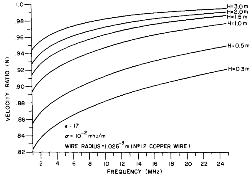
Figure I-6. Theoretical Values of Attenuation, Impedance and Velocity Ratio for a Beverage on Average Soil (Wet).
