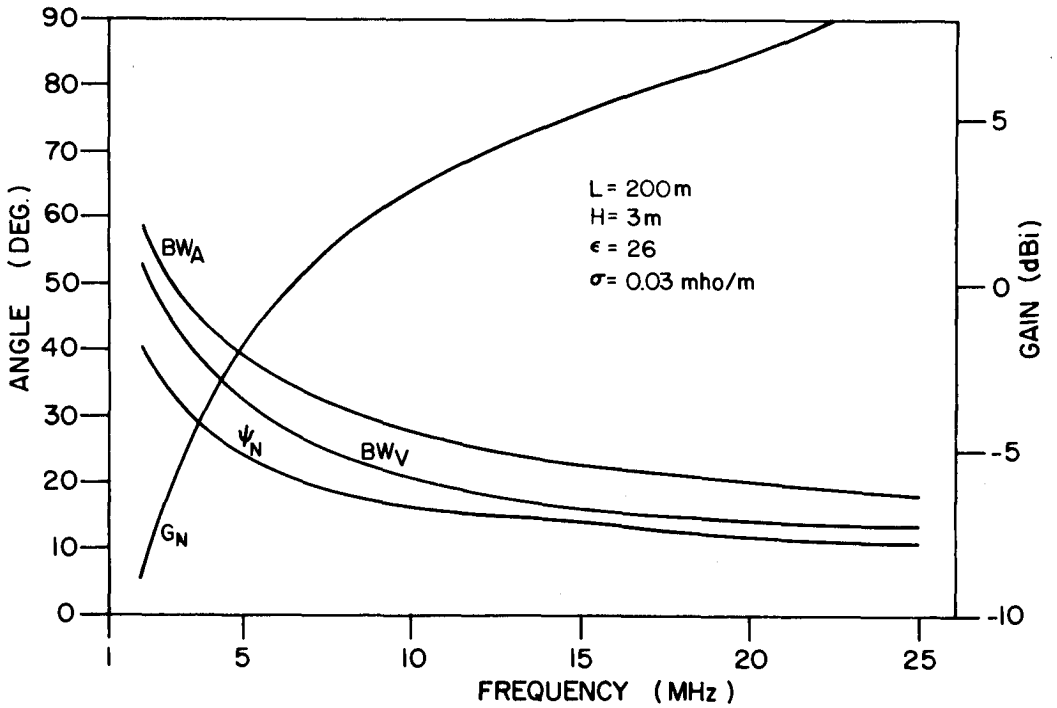
Figure II-46. Design Parameters for Wet Soil, H = 3\text{m} , L = 200\text{m} .
