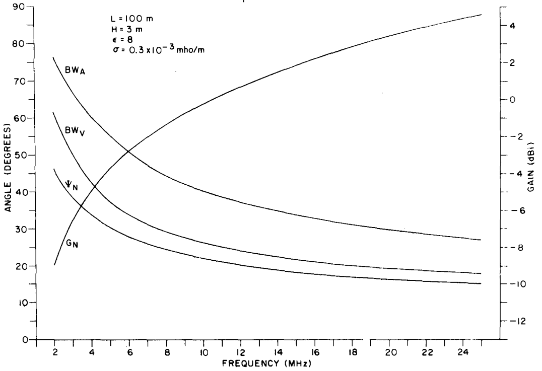
Figure II-13. Design Parameters for Poor Soil (Dry), H = 3\text{m} , L = 100\text{m} .
