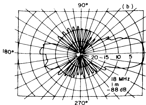
(b) Azimuthal pattern for Beverage antenna L=110\text{m} , H=0.9 and f=18\text{MHz} .
