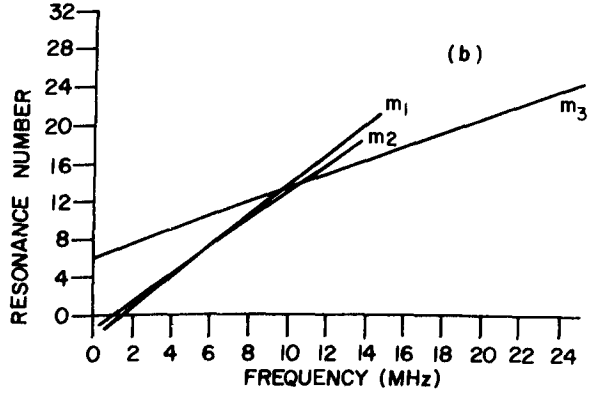
(b) Open and short circuit resonance number versus frequency.
