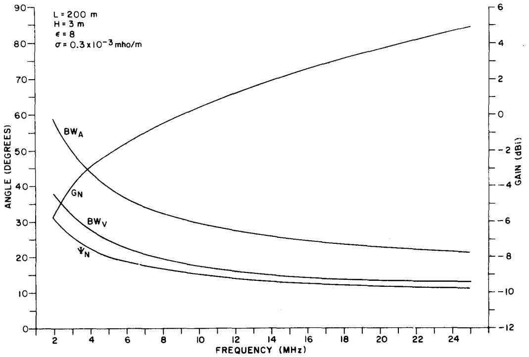
Figure II-14. Design Parameters for Poor Soil (Dry), H = 3\text{m} , L = 200\text{m} .
