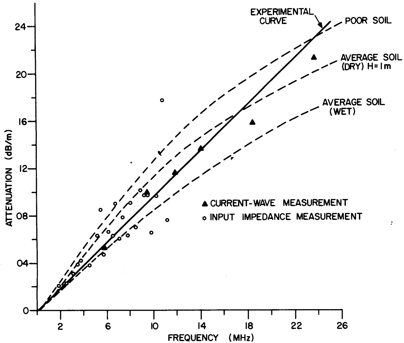
Figure 17. Comparison of Theoretical and Measured Current-wave Attenuation on a Beverage Element at Shirley Bay, 110 m long and 1 m high.
