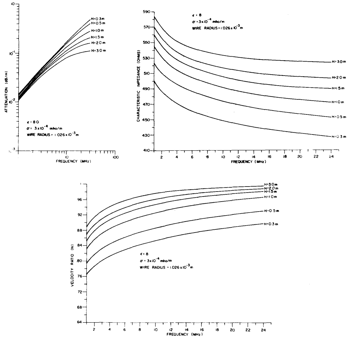
Figure I-3. Theoretical Values for Attenuation, Impedance and Wave Velocity for a Beverage Antenna on Poor Soil (Dry).
