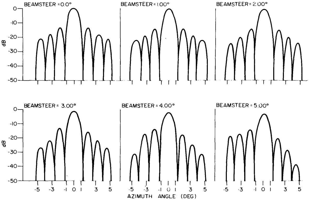
Figure IV-8. Radiation Patterns in the Central Region For the Beamsteers as Shown.
