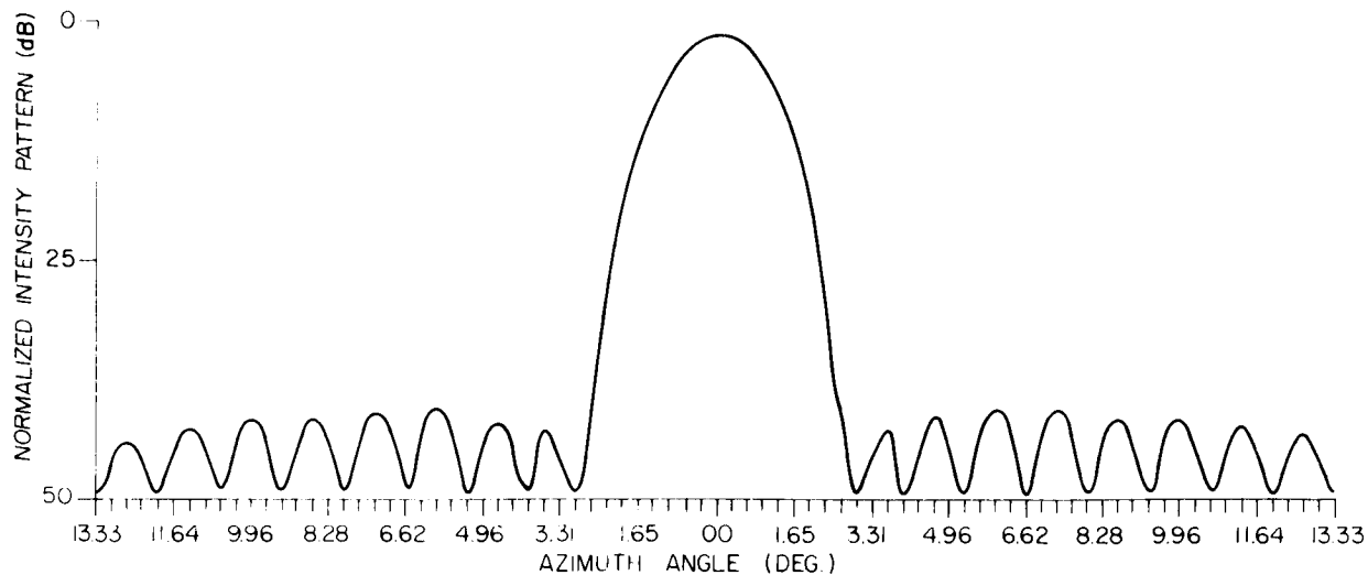
Figure IV-15. Illustration in Linear Form of the Radiation Pattern with Application of Taylor Weighting.
