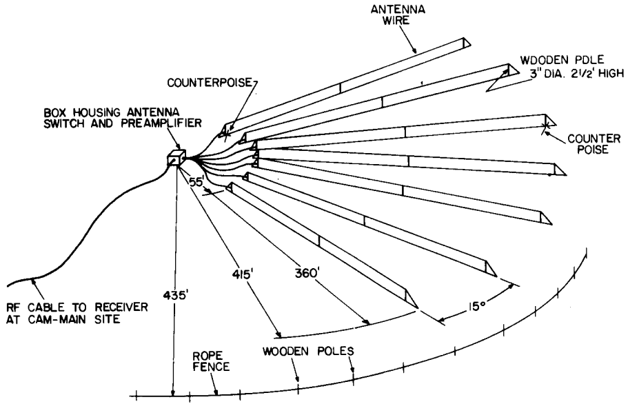
Figure 29. A Portion of the Beverage Rosette Array.
