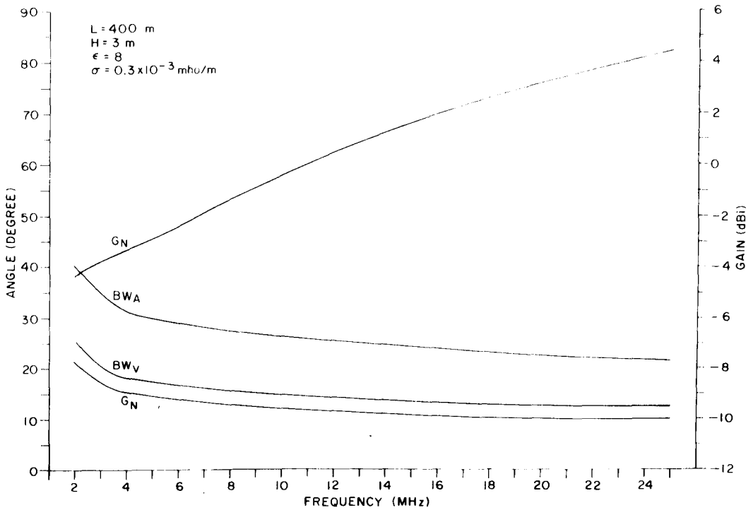
Figure II-16. Design Parameters for Poor Soil (Dry), H = 3\text{m} , L = 400\text{m} .
