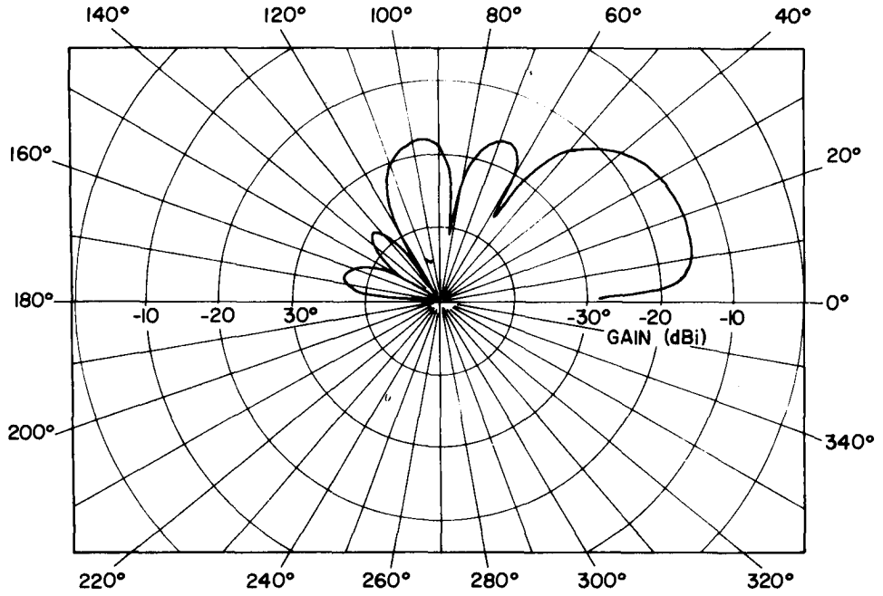
(a) Theoretical vertical radiation pattern for a Beverage antenna at 125 kHz over poor soil (dry).
