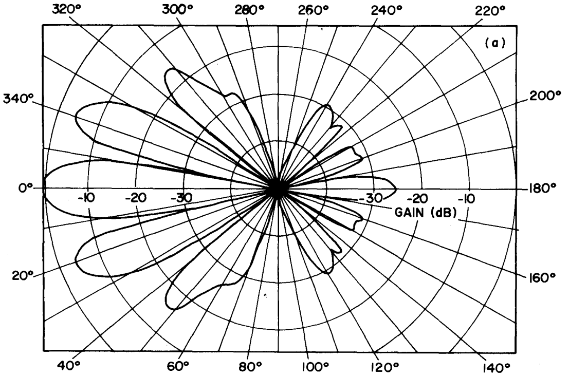
(a) Two-elements
