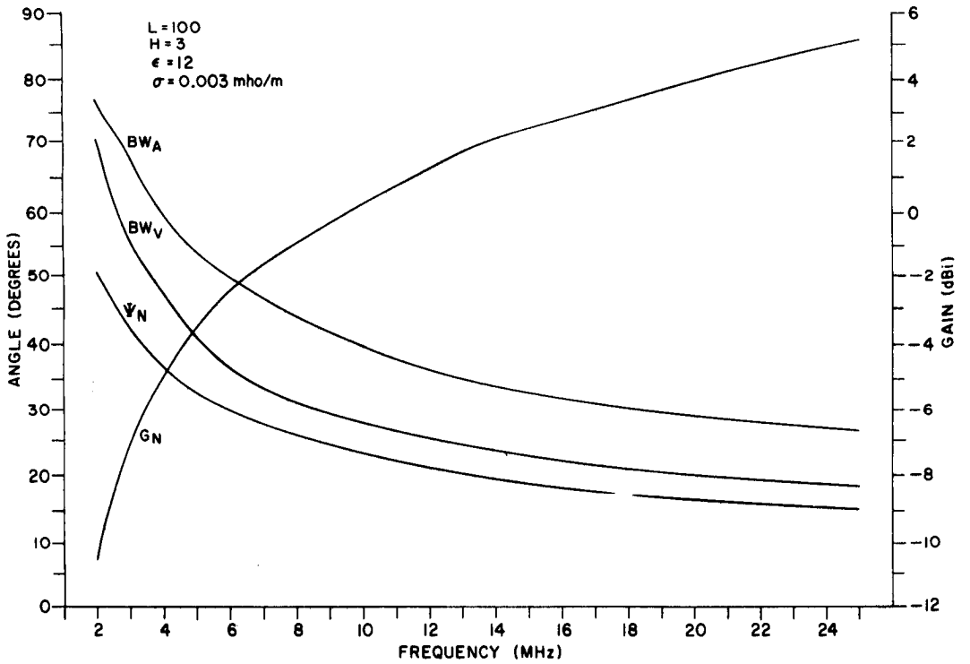
Figure II-29. Design Parameters for Average Soil (Dry), H = 3\text{m} , L = 100\text{m} .
